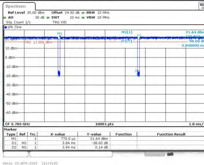
11AC20-BF_Ant2_5785
