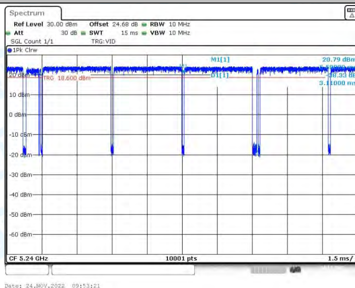
11AX20-BF_Ant2_5240
