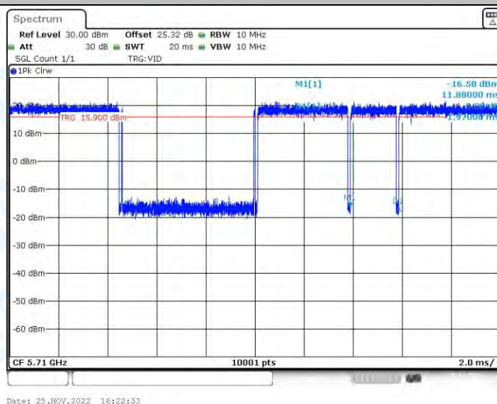
11AC40-BF_Ant2_5710
