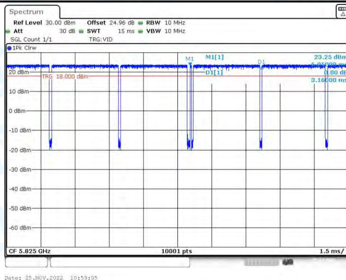
11AX20-BF_Ant2_5825
