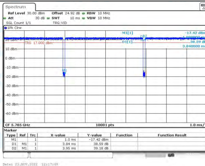
11N20-BF_Ant2_5785
