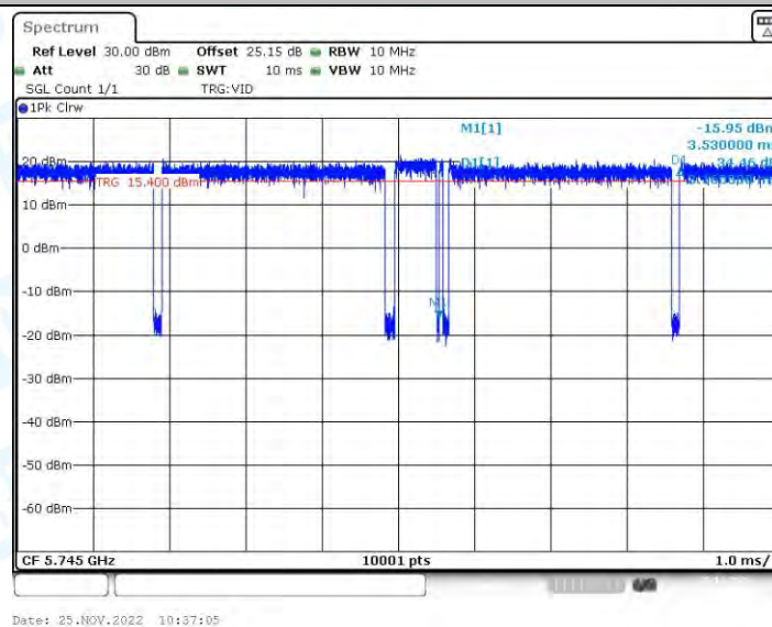
11AX20-BF_Ant2_5745
