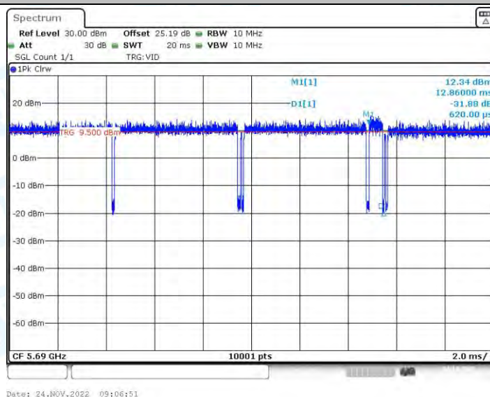
11AC80-BF_Ant2_5690
