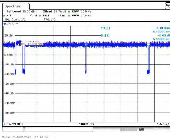
11AC80-BF_Ant2_5290
