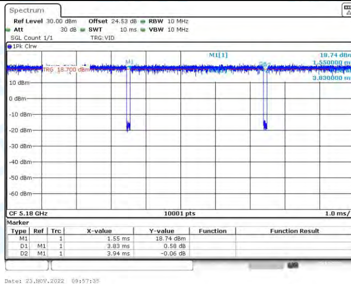
11AC20-BF_Ant2_5180
