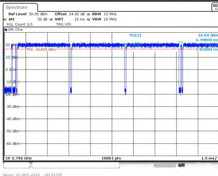
11AC40-BF_Ant2_5795
