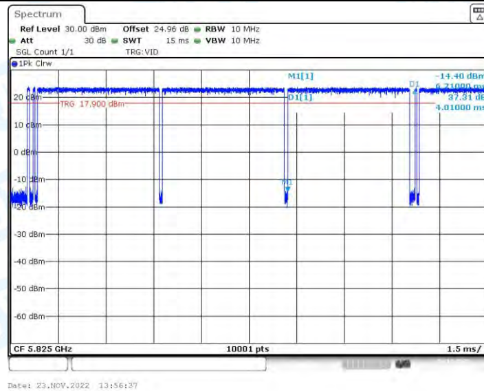
11AC20-BF_Ant2_5825
