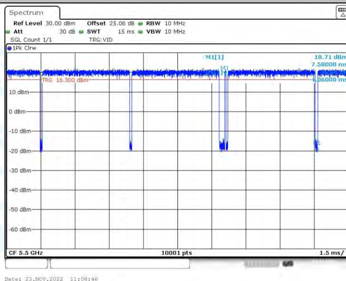
11AC20-BF_Ant2_5500
