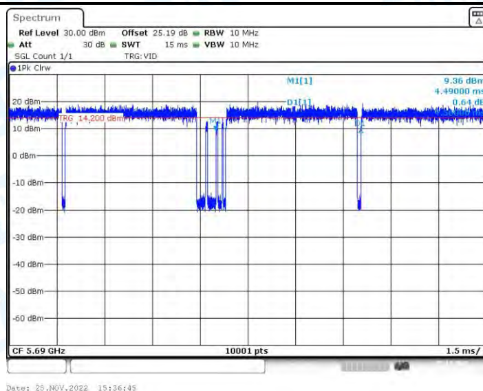
11AX80-BF_Ant2_5690
