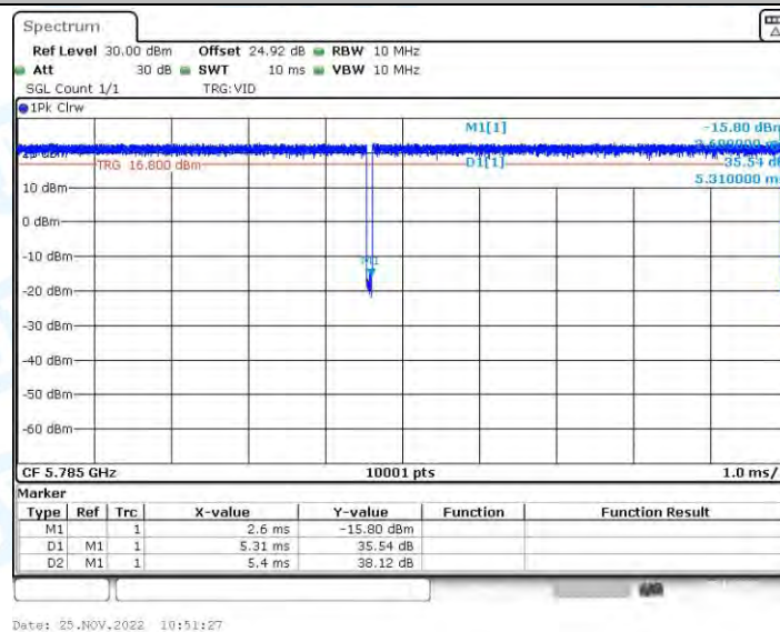
11AX20-BF_Ant2_5785
