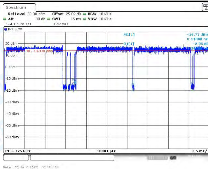
11AX80-BF_Ant2_5775
