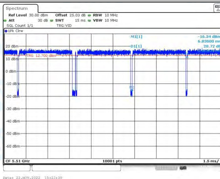
11AC40-BF_Ant2_5510
