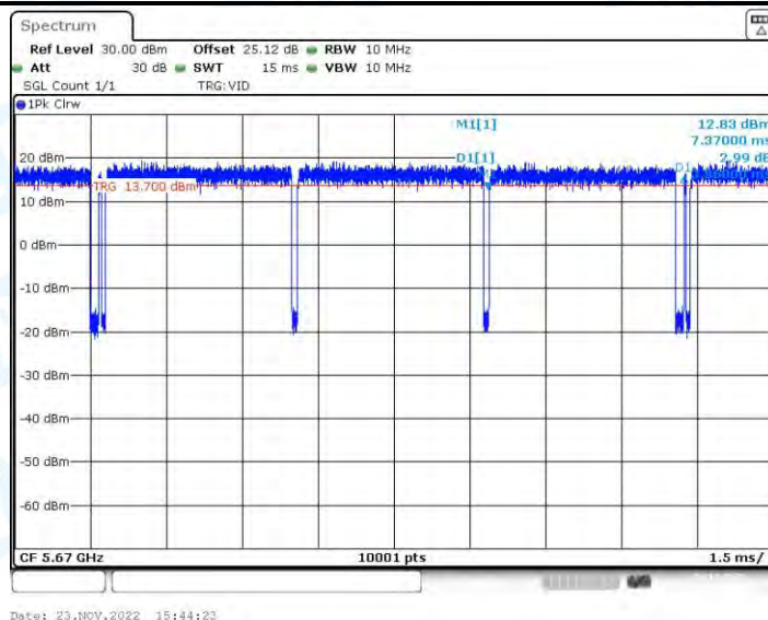
11AC40-BF_Ant2_5670
