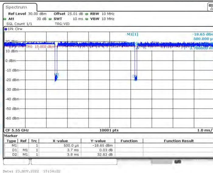
11AC40-BF_Ant2_5550
