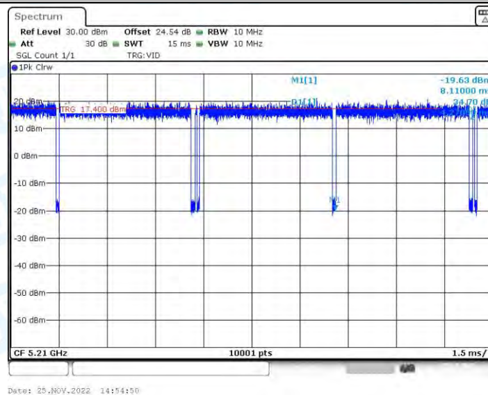
11AX80-BF_Ant2_5210
