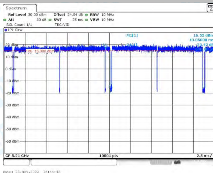
11AC80-BF_Ant2_5210
