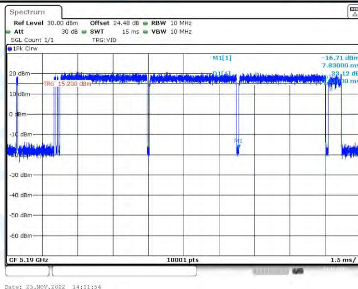
11AC40-BF_Ant2_5190
