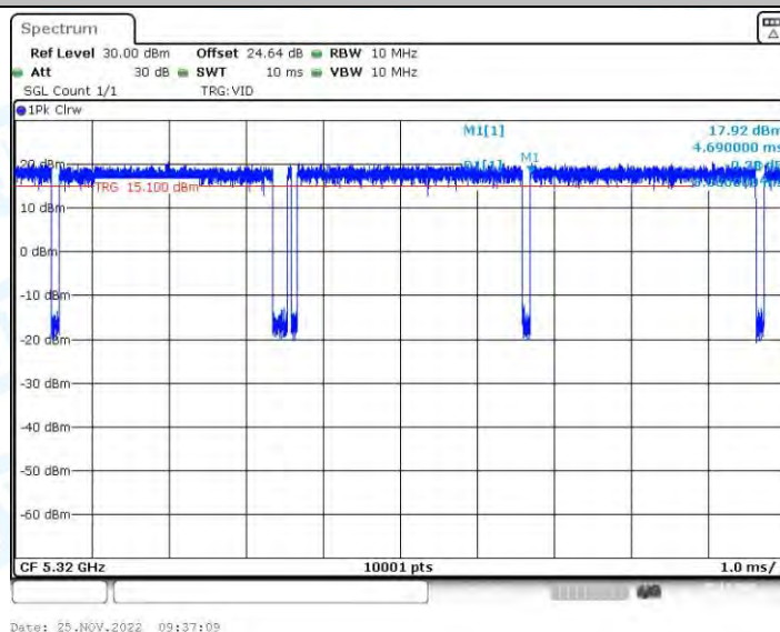
11AX20-BF_Ant2_5320
