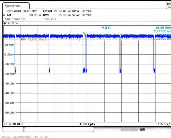
11AX20-BF_Ant2_5180
