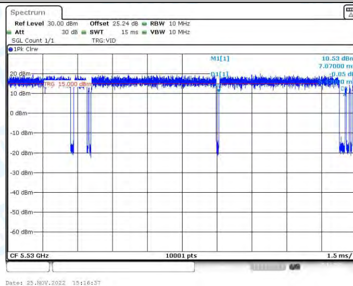
11AX80-BF_Ant2_5530
