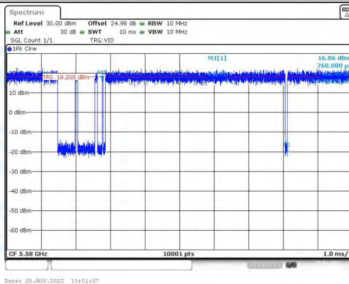
11AX20-BF_Ant2_5580
