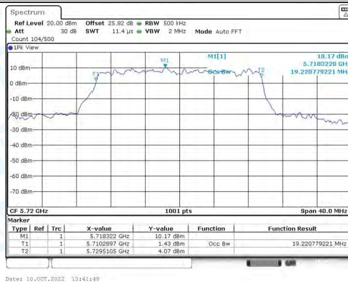
11AX20-SDM_Ant2_5720
