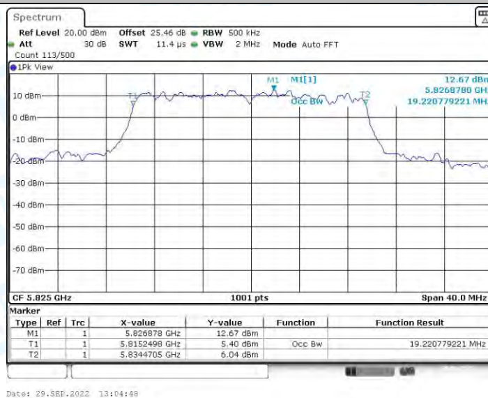
11AX20-SDM_Ant2_5825
