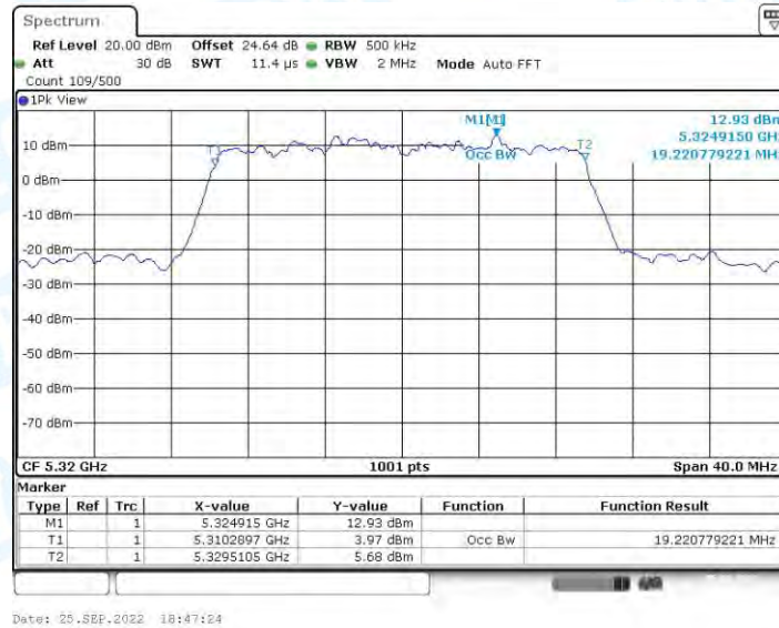
11AX20-SDM_Ant2_5320
