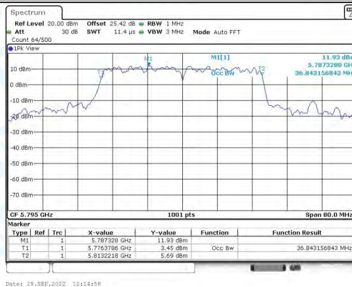
11AC40-SDM_Ant2_5795
