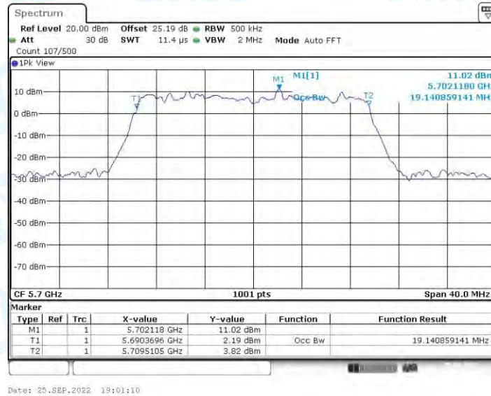
11AX20-SDM_Ant2_5700
