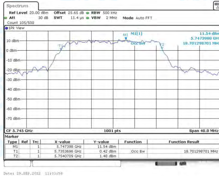
11N20-SDM_Ant2_5745
