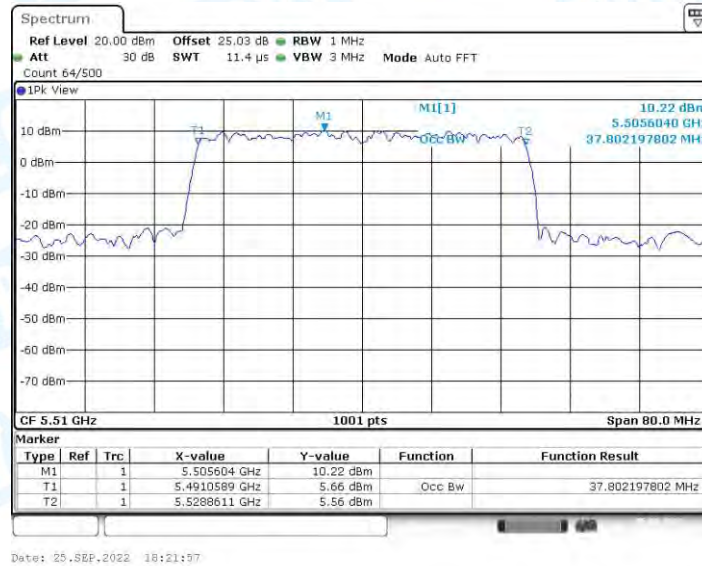
11AX40-SDM_Ant2_5510
