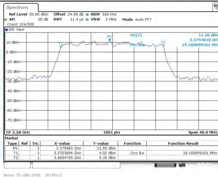
11AX20-SDM_Ant2_5580
