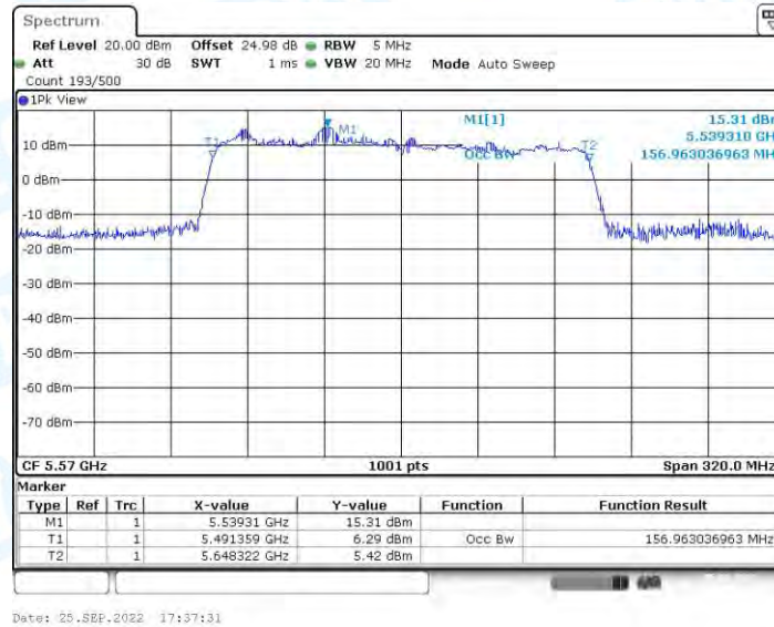
11AC160-SDM_Ant2_5570
