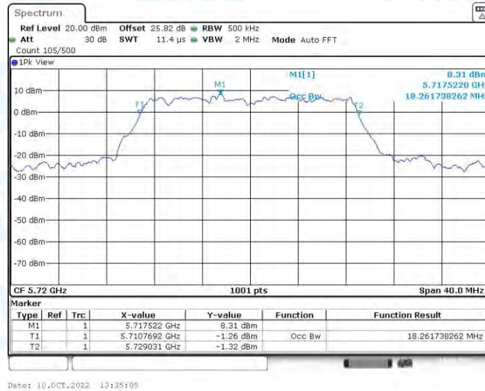
11AC20-SDM_Ant2_5720
