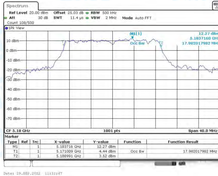
11AC20-SDM_Ant2_5180
