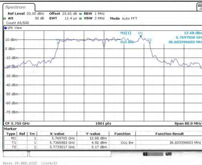
11N40-SDM_Ant2_5755
