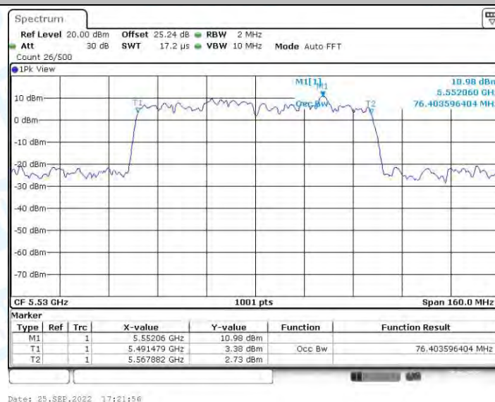
11AC80-SDM_Ant2_5530
