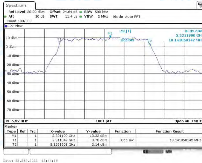
11N20-SDM_Ant2_5320
