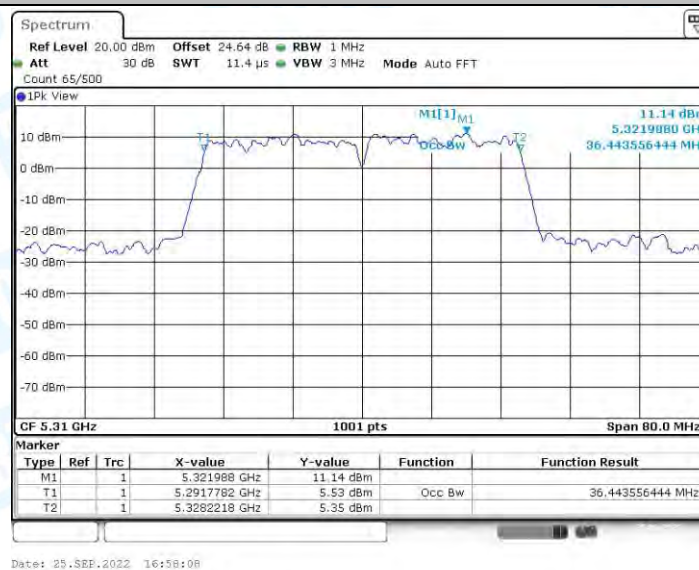
11AC40-SDM_Ant2_5310
