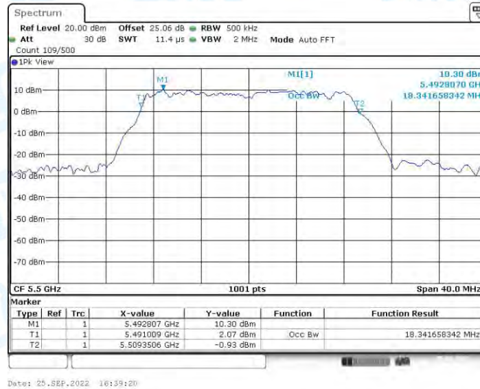
11AC20-SDM_Ant2_5500
