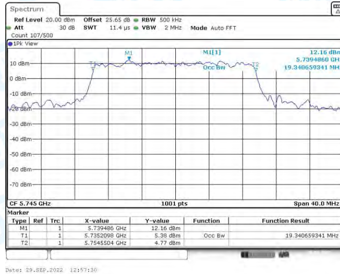
11AX20-SDM_Ant2_5745
