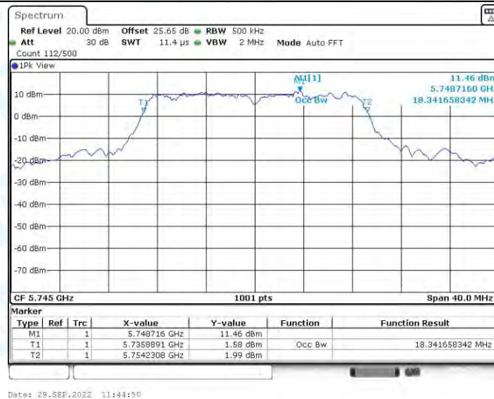
11AC20-SDM_Ant2_5745
