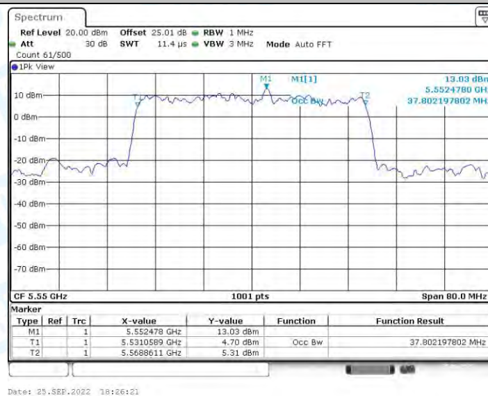
11AX40-SDM_Ant2_5550
