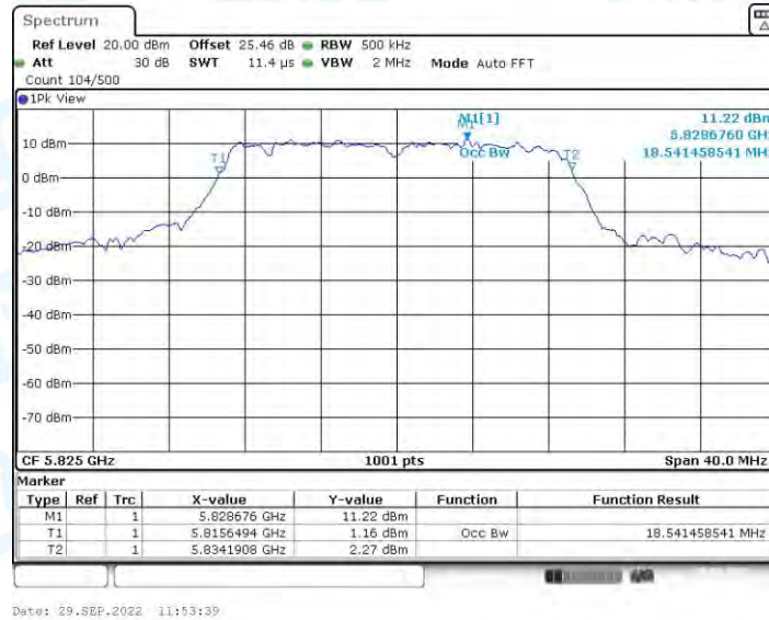
11AC20-SDM_Ant2_5825
