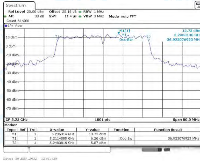
11AC40-SDM_Ant2_5230
