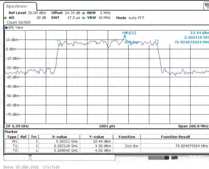
11AC80-SDM_Ant2_5290
