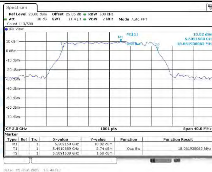
11N20-SDM_Ant2_5500
