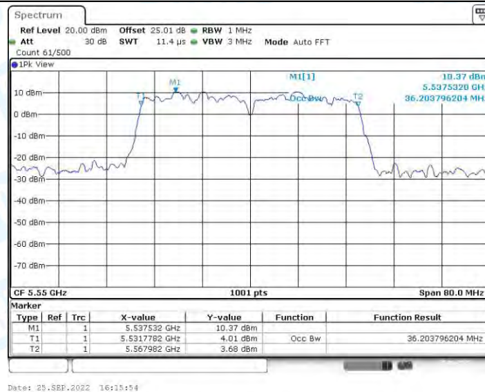
11N40-SDM_Ant2_5550
