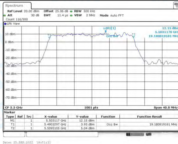
11AX20-SDM_Ant2_5500
