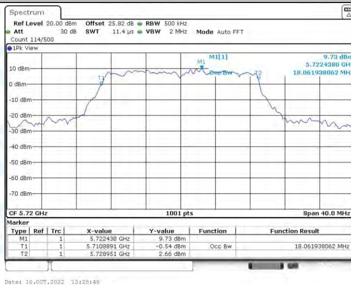
11N20-SDM_Ant2_5720
