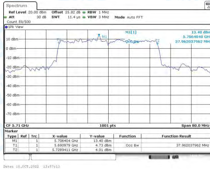
11AX40-SDM_Ant2_5710
