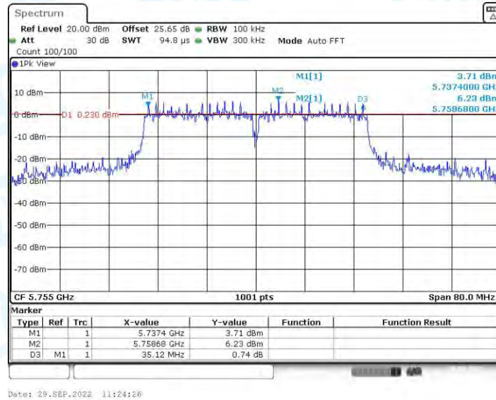
11N40-SDM_Ant2_5755
