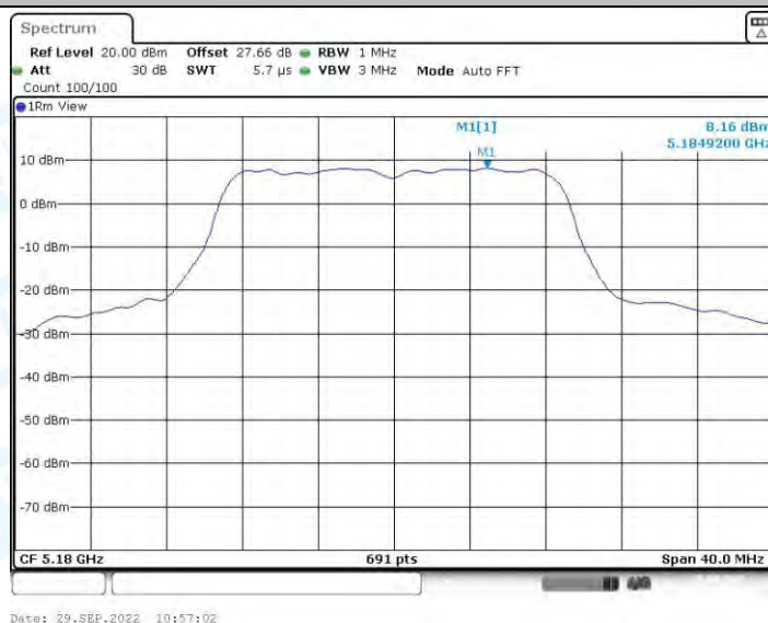
11N20-SDM_Ant2_5180
