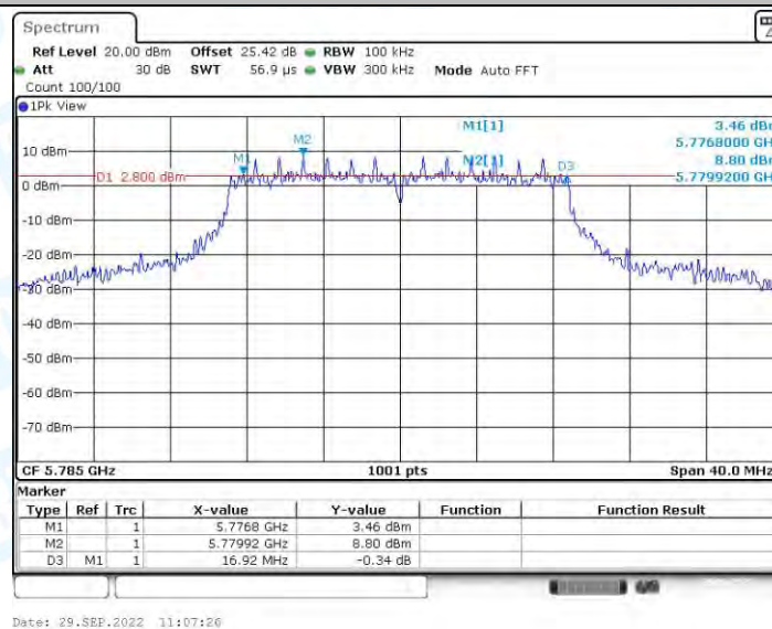
11N20-SDM_Ant2_5785
