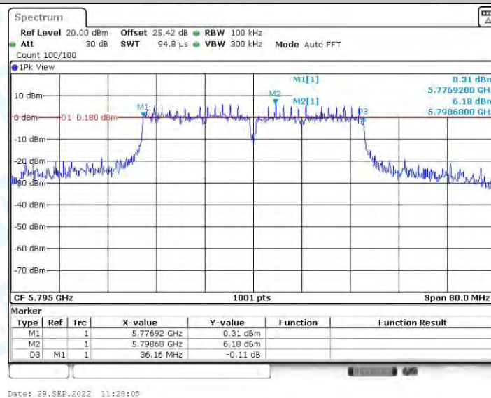
11N40-SDM_Ant2_5795
