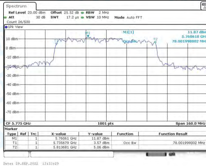
11AX80-SDM_Ant2_5775
