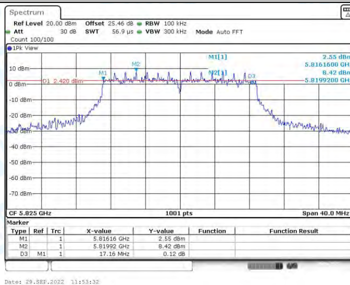
11AC20-SDM_Ant2_5825
