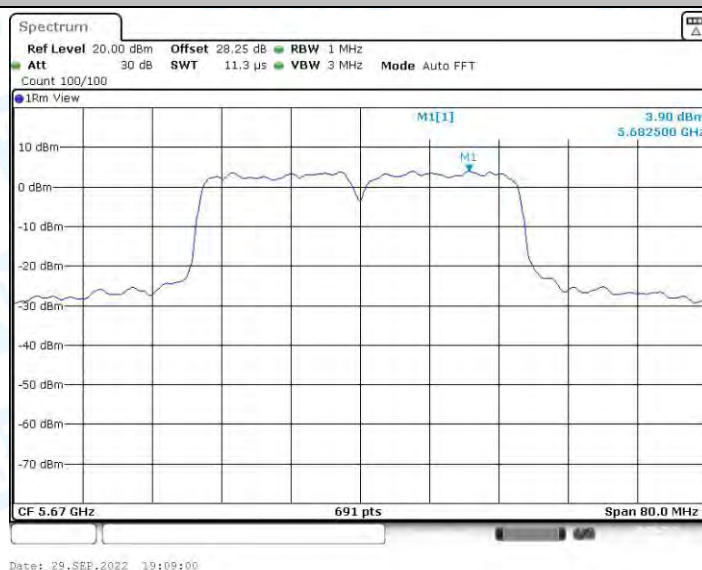
11N40-SDM_Ant2_5670
