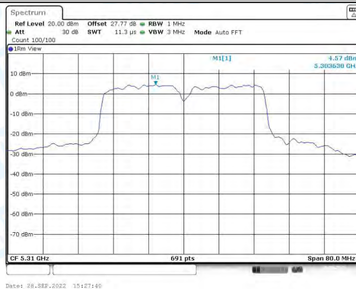
11N40-SDM_Ant2_5310
