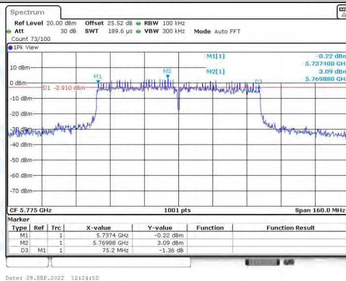
11AC80-SDM_Ant2_5775
