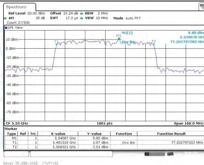
11AX80-SDM_Ant2_5530
