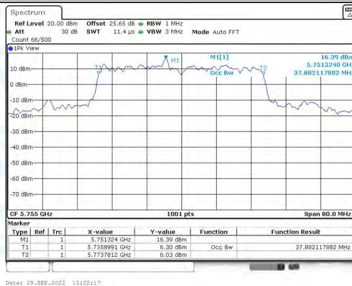
11AX40-SDM_Ant2_5755
