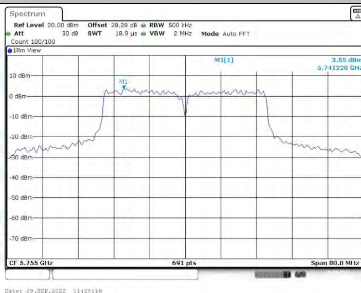
11N40-SDM_Ant2_5755
