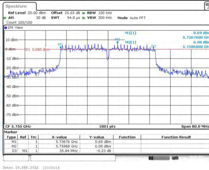
11AC40-SDM_Ant2_5755
