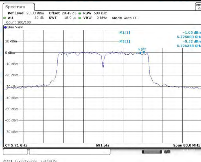
11N40-SDM_Ant2_5710_UNII-3
