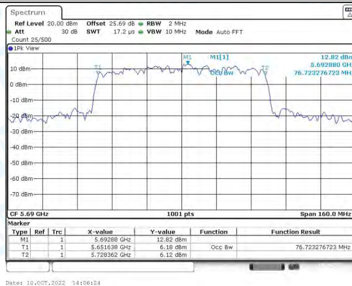
11AX80-SDM_Ant2_5690
