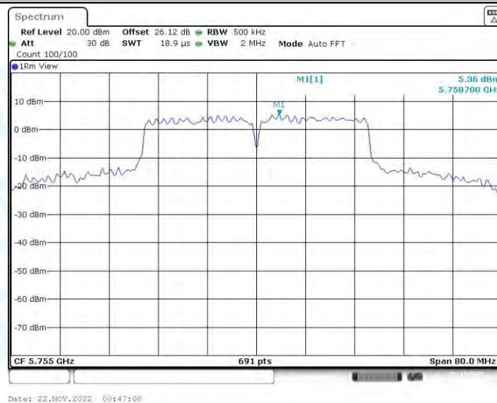
11AC40-CDD_Ant2_5755
