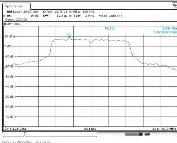
11AC20-CDD_Ant2_5825
