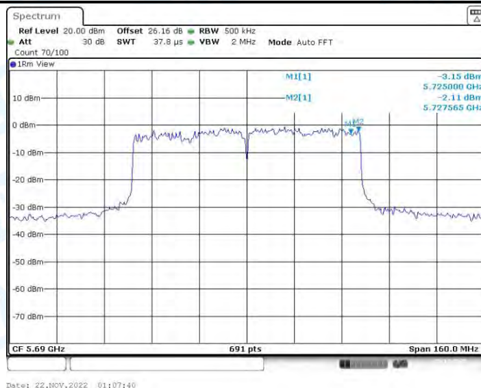
11AC80-CDD_Ant2_5690_UNII-3
