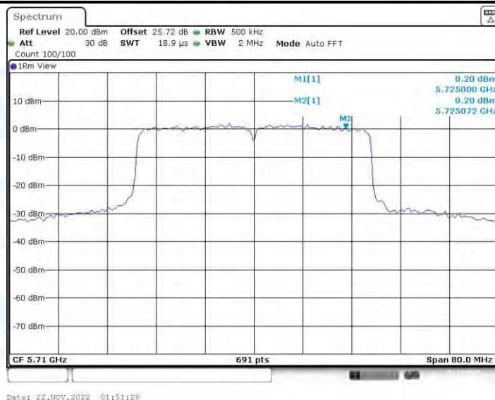
11AX40-CDD_Ant2_5710_UNII-3
