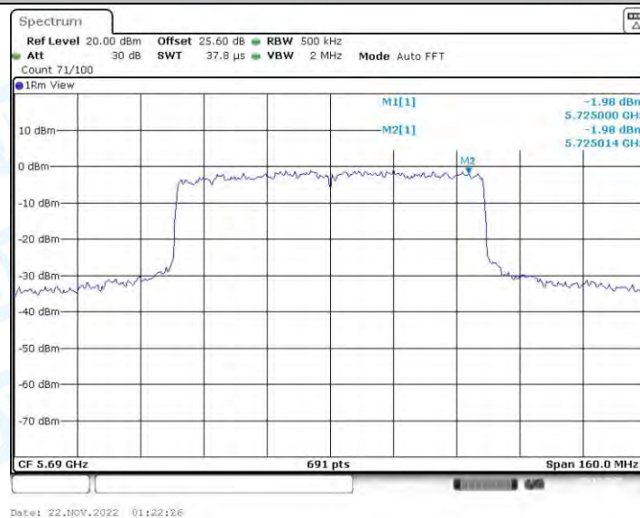
11AX80-CDD_Ant2_5690_UNII-3
