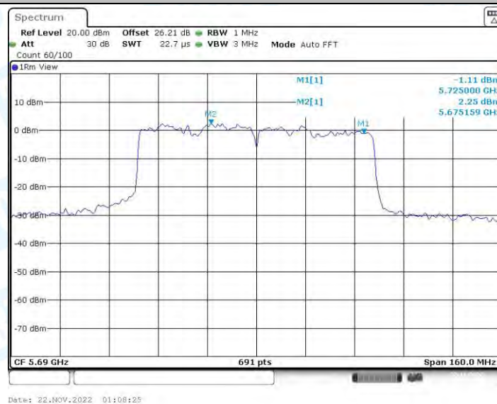
11AC80-CDD_Ant1_5690_UNII-3
