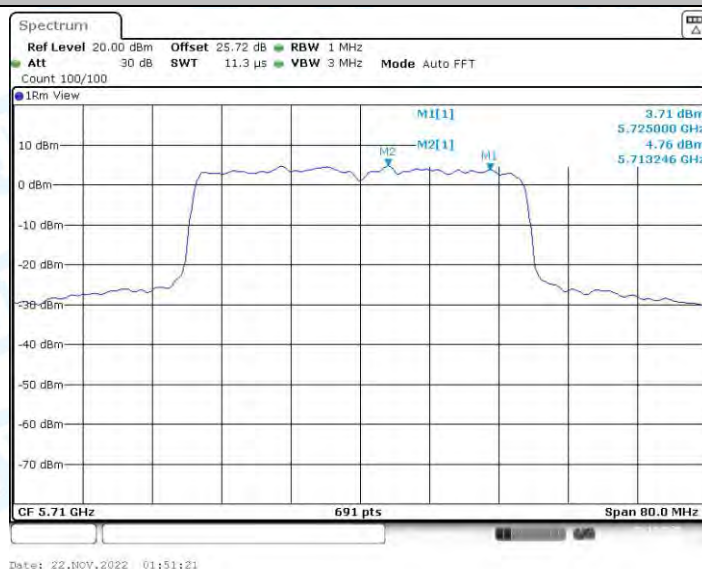
11AX40-CDD_Ant2_5710_UNII-2C
