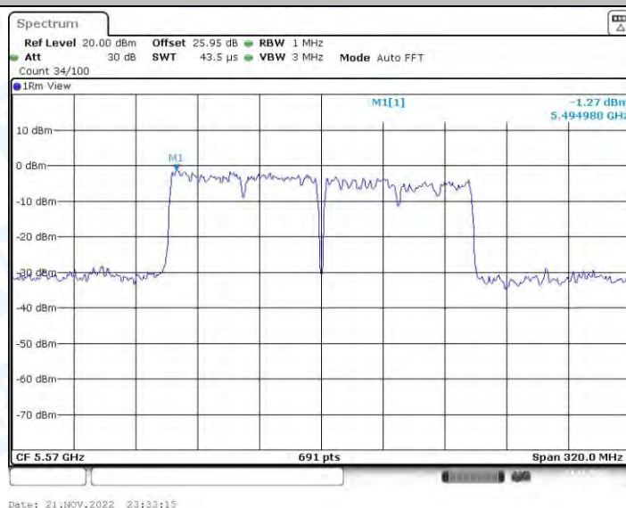
11AC160-CDD_Ant2_5570
