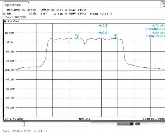
11AC40-CDD_Ant2_5710_UNII-2C
