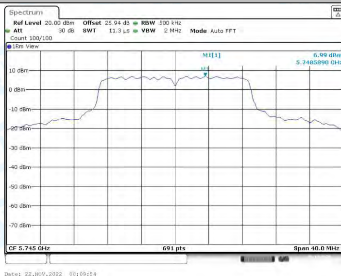
11AC20-CDD_Ant2_5745
