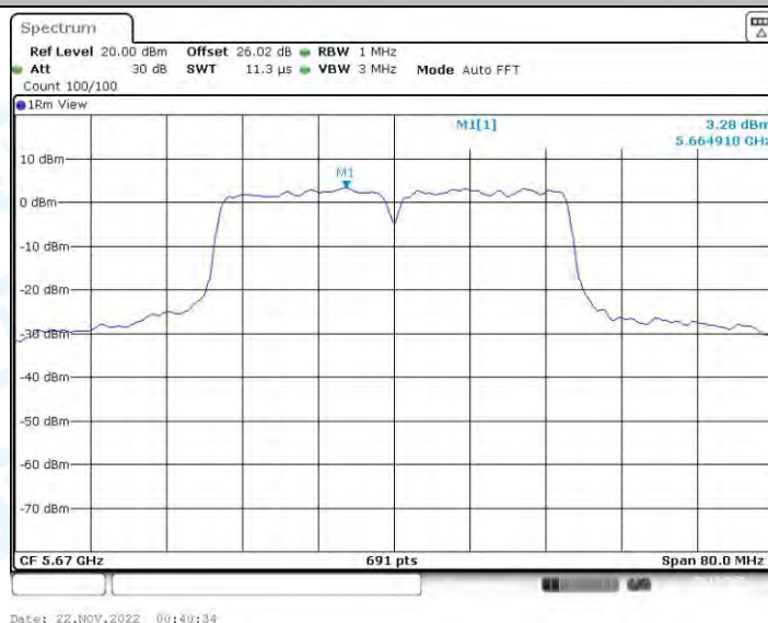
11AC40-CDD_Ant2_5670
