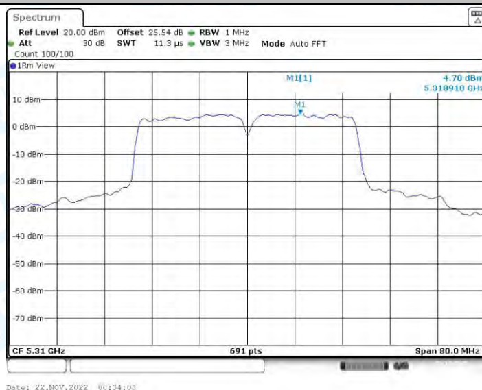
11AC40-CDD_Ant2_5310
