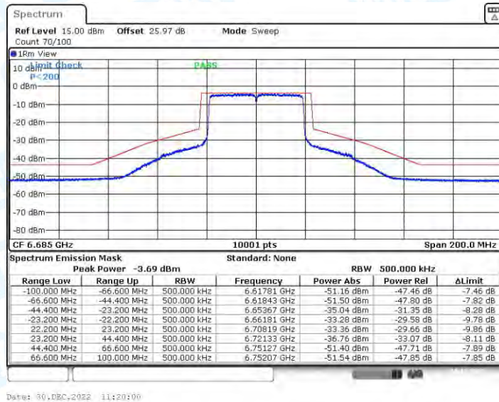
11AX40CDD_Ant2_6685
