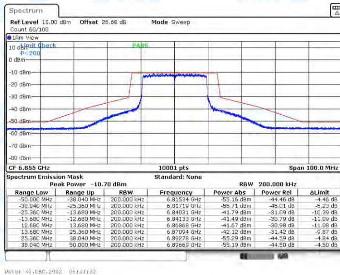
11AX20CDD_Ant2_6855
