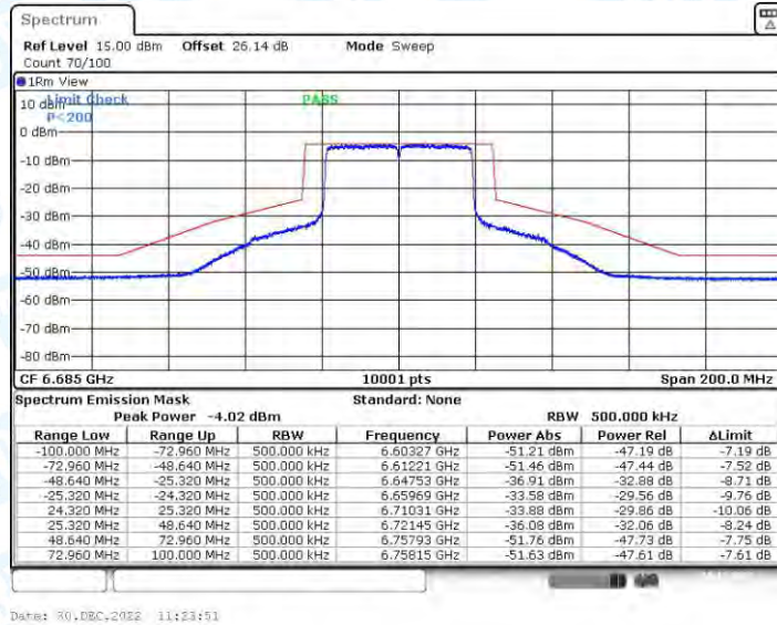
11AX40CDD_Ant4_6685
