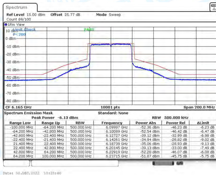
11AX40CDD_Ant3_6165
