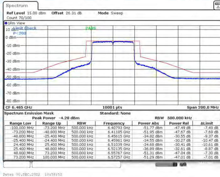
11AX40CDD_Ant4_6485
