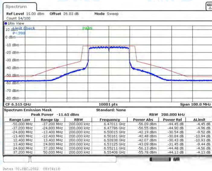
11AX20CDD_Ant2_6515
