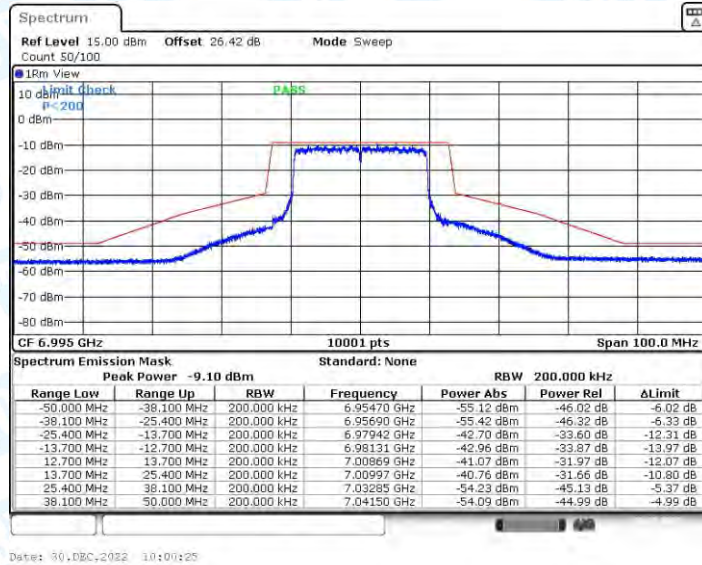
11AX20CDD_Ant4_6995
