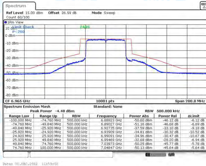
11AX40CDD_Ant4_6965
