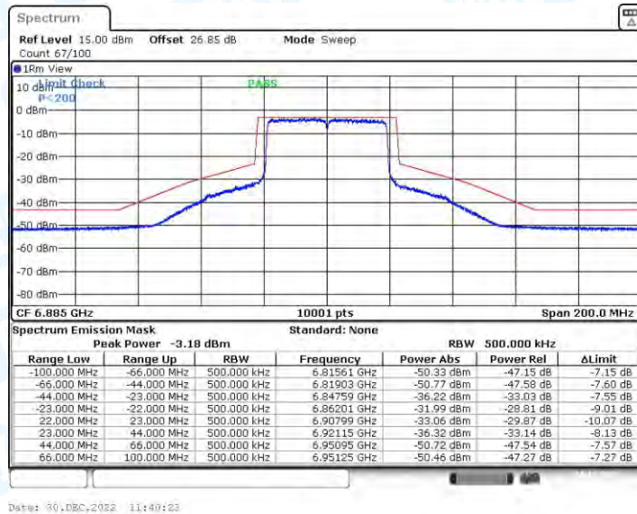
11AX40CDD_Ant3_6885
