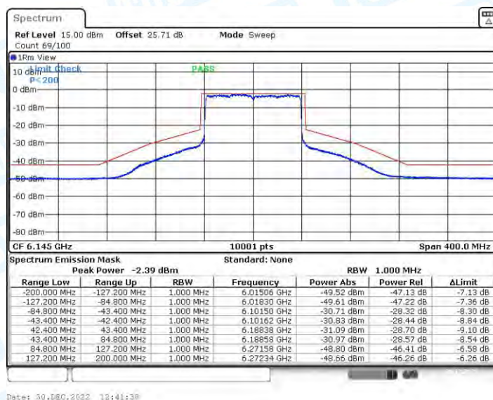
11AX80CDD_Ant2_6145
