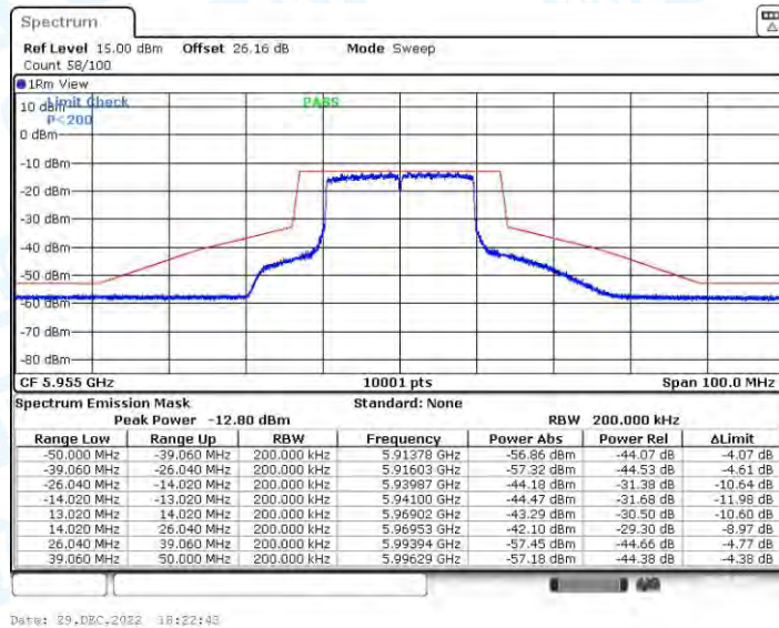
11AX20CDD_Ant4_5955
