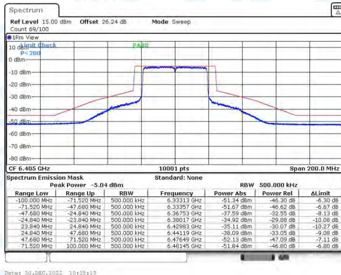
11AX40CDD_Ant2_6405
