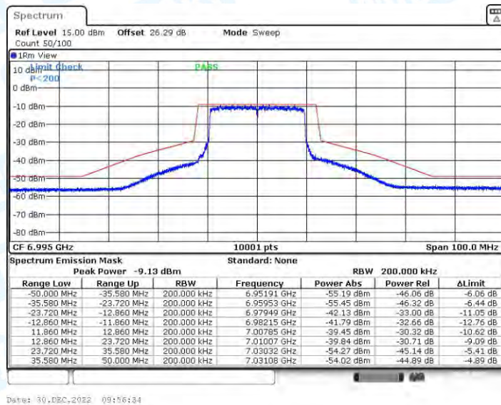
11AX20CDD_Ant2_6995
