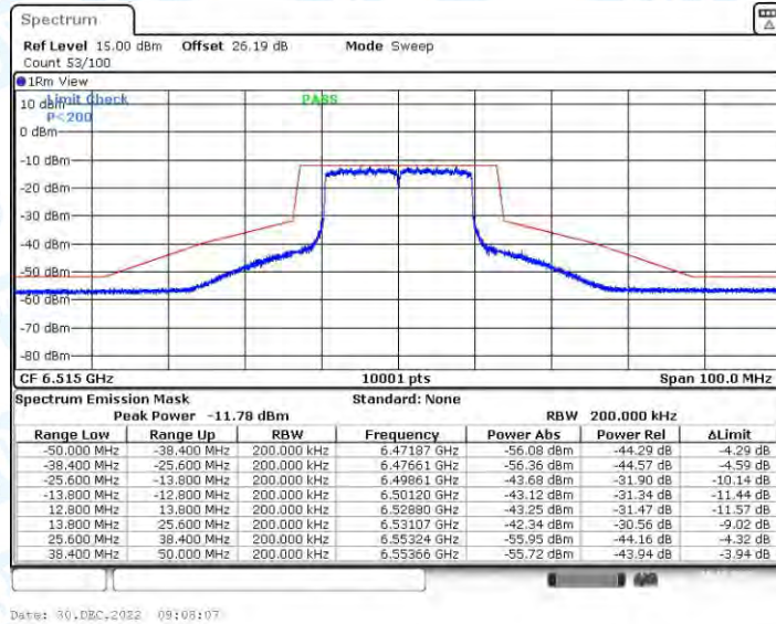
11AX20CDD_Ant4_6515
