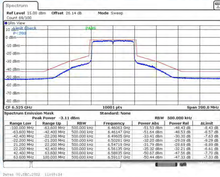
11AX40CDD_Ant3_6525
