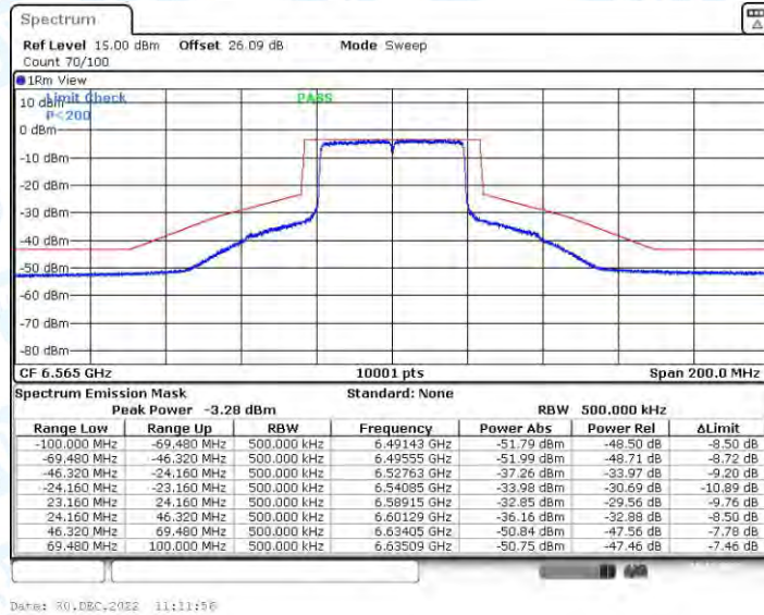
11AX40CDD_Ant2_6565
