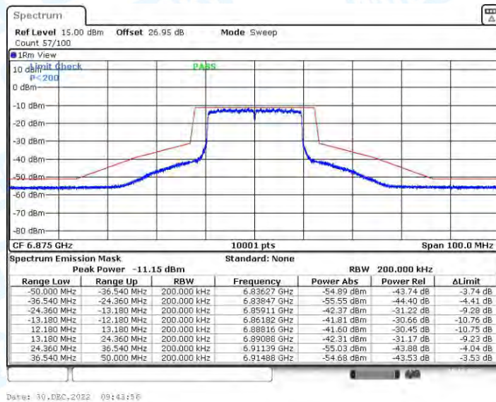
11AX20CDD_Ant4_6875
