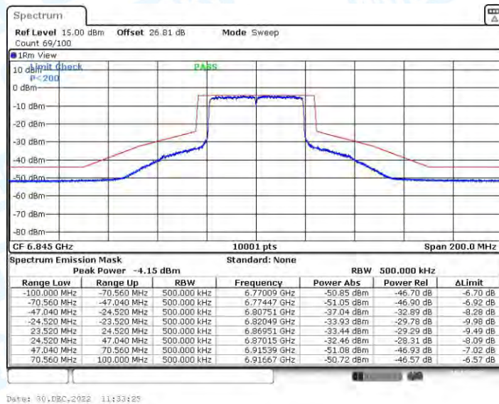
11AX40CDD_Ant4_6845
