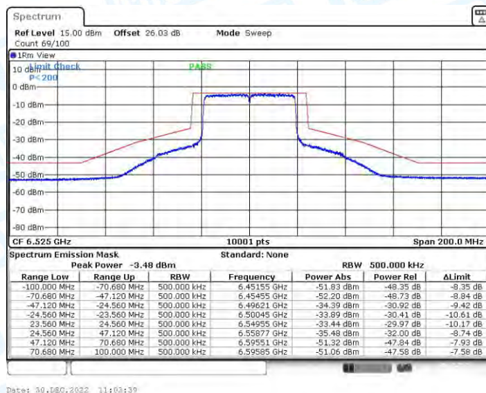
11AX40CDD_Ant2_6525
