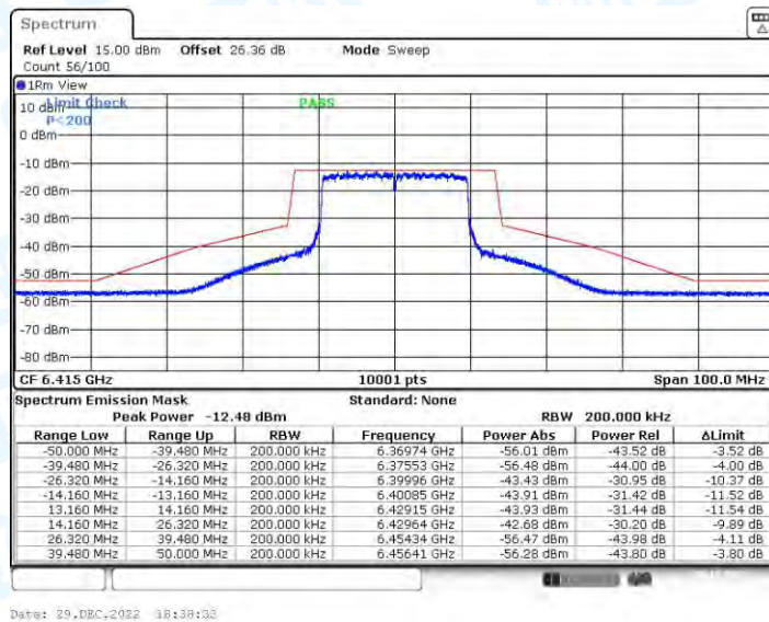
11AX20CDD_Ant2_6415
