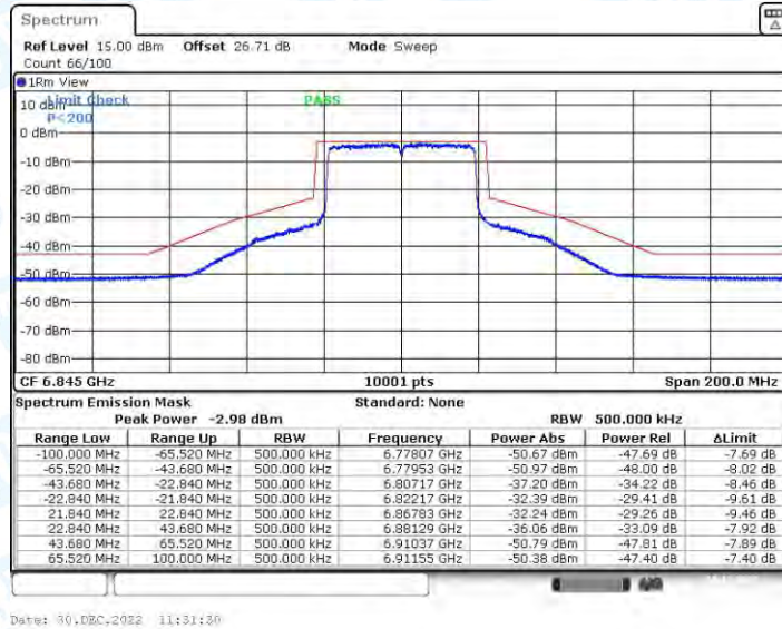
11AX40CDD_Ant3_6845
