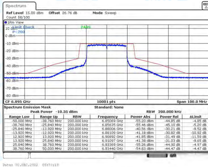
11AX20CDD_Ant3_6895
