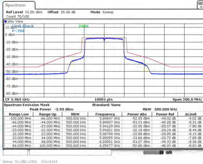
11AX40CDD_Ant2_5965
