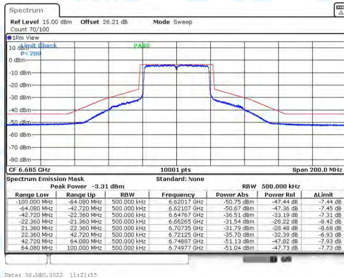
11AX40CDD_Ant3_6685
