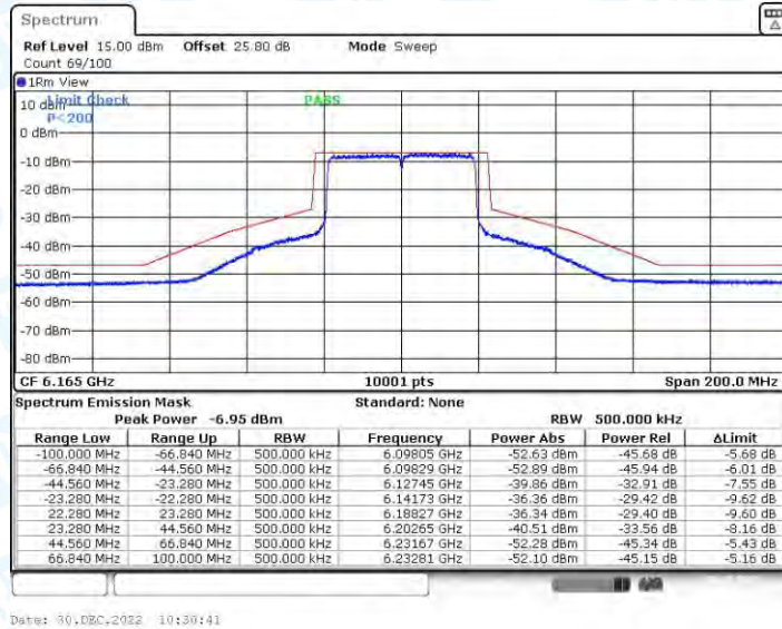
11AX40CDD_Ant4_6165
