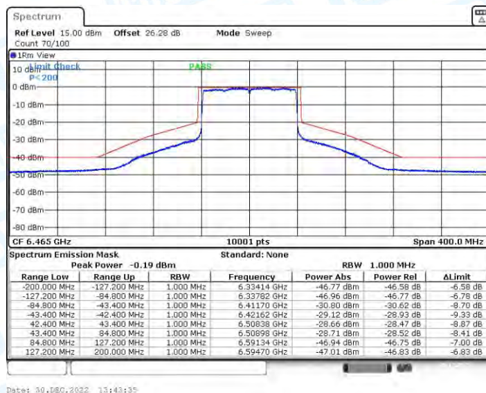
11AX80CDD_Ant3_6465
