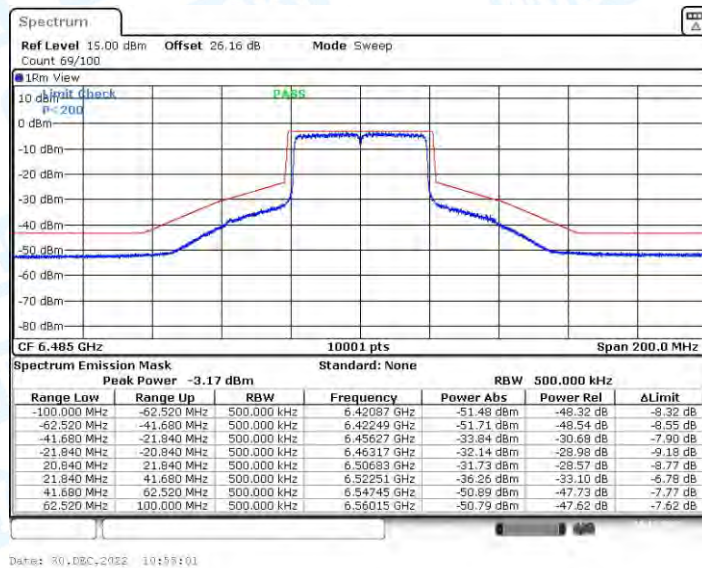
11AX40CDD_Ant2_6485
