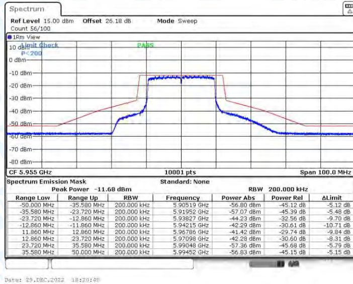
11AX20CDD_Ant3_5955
