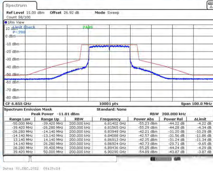
11AX20CDD_Ant4_6855
