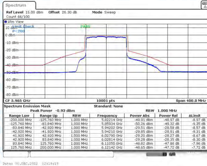
11AX80CDD_Ant4_5985
