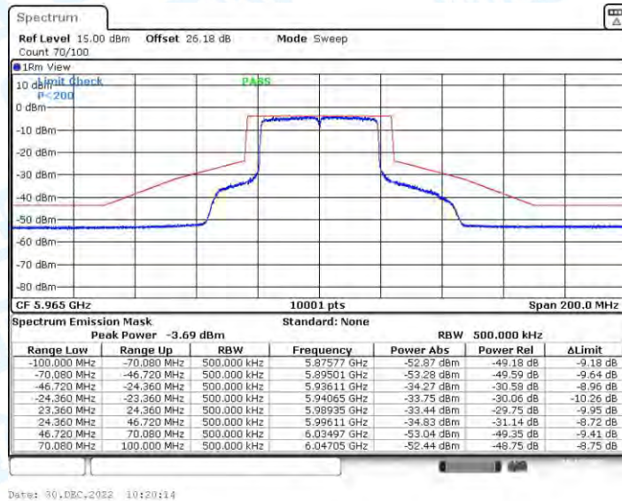
11AX40CDD_Ant3_5965
