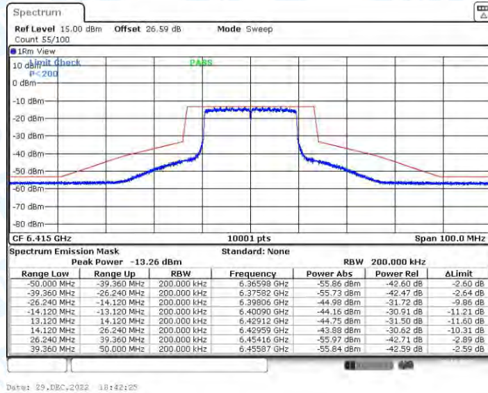
11AX20CDD_Ant4_6415
