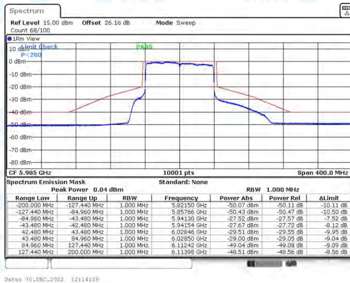
11AX80CDD_Ant2_5985
