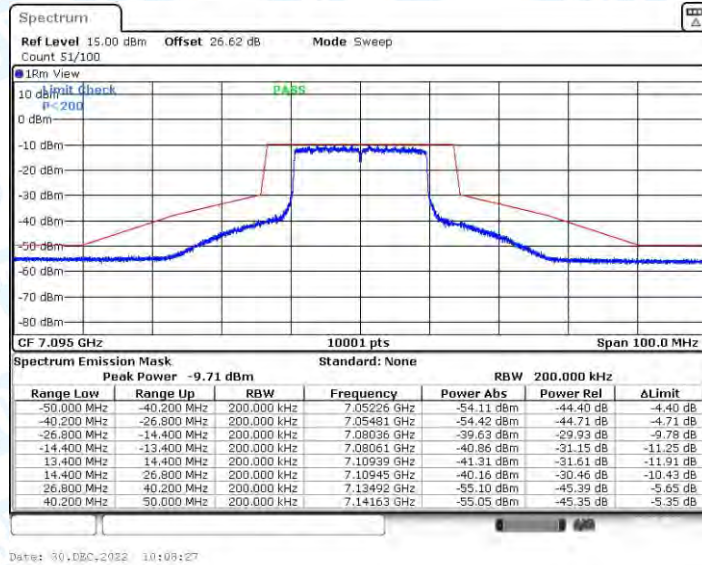
11AX20CDD_Ant3_7095
