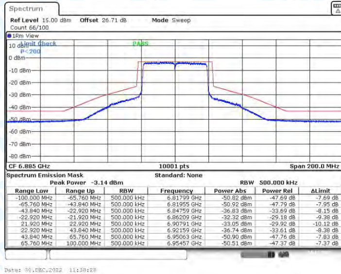
11AX40CDD_Ant2_6885
