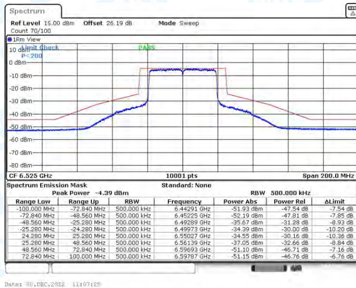
11AX40CDD_Ant4_6525
