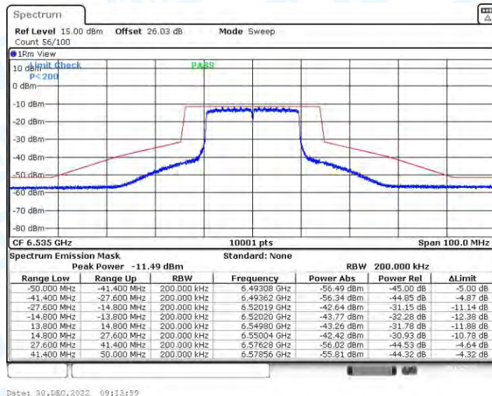
11AX20CDD_Ant2_6535
