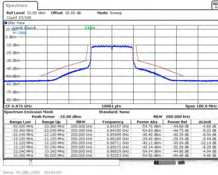
11AX20CDD_Ant3_6875
