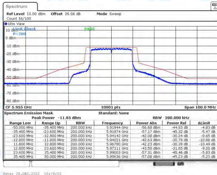
11AX20CDD_Ant2_5955
