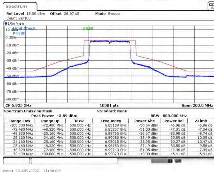
11AX40CDD_Ant3_6925
