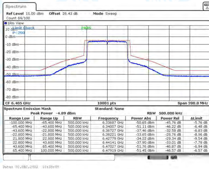
11AX40CDD_Ant4_6405
