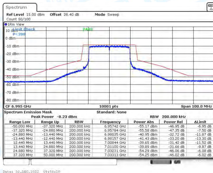
11AX20CDD_Ant3_6995
