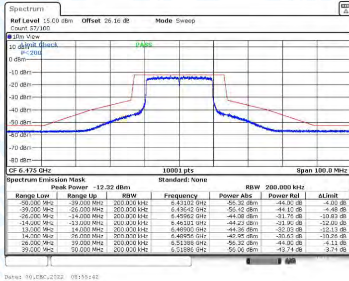
11AX20CDD_Ant2_6475
