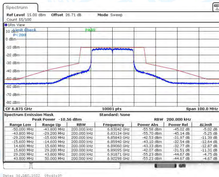
11AX20CDD_Ant2_6875
