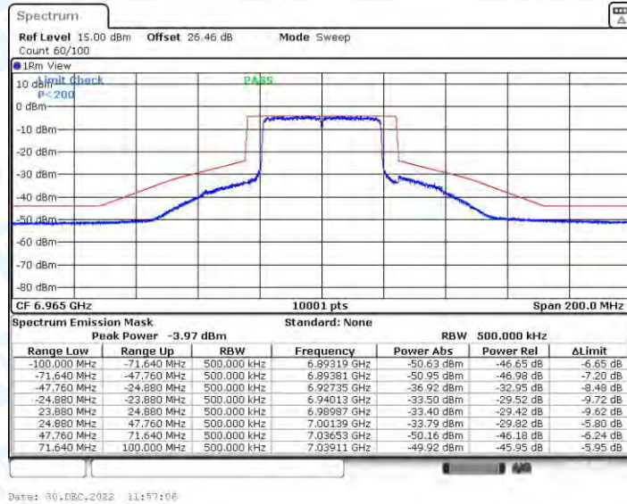
11AX40CDD_Ant3_6965
