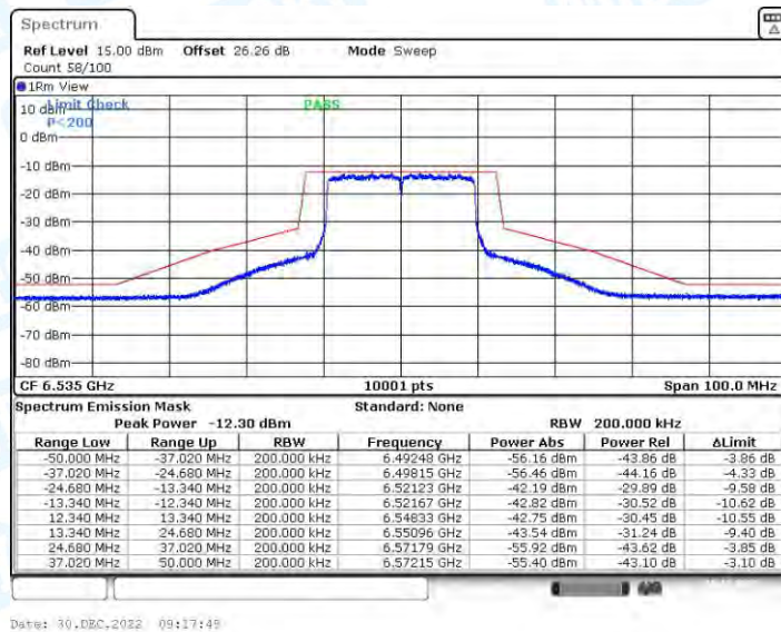
11AX20CDD_Ant4_6535
