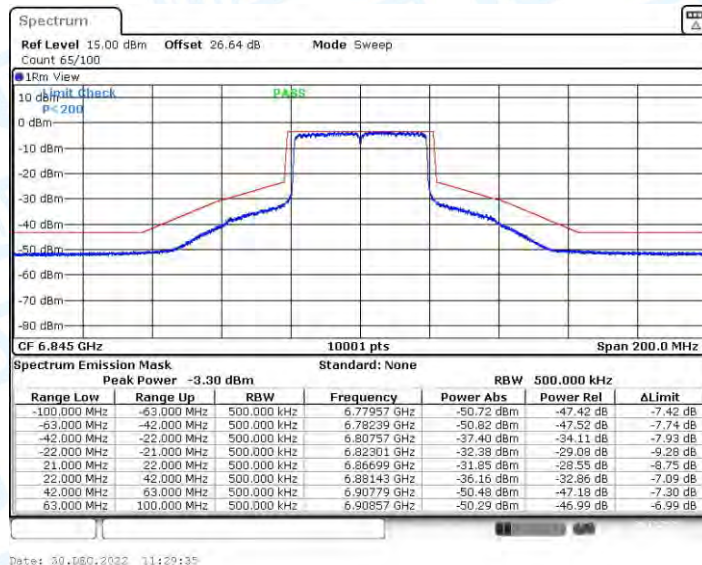
11AX40CDD_Ant2_6845
