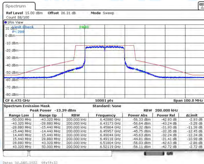
11AX20CDD_Ant4_6475
