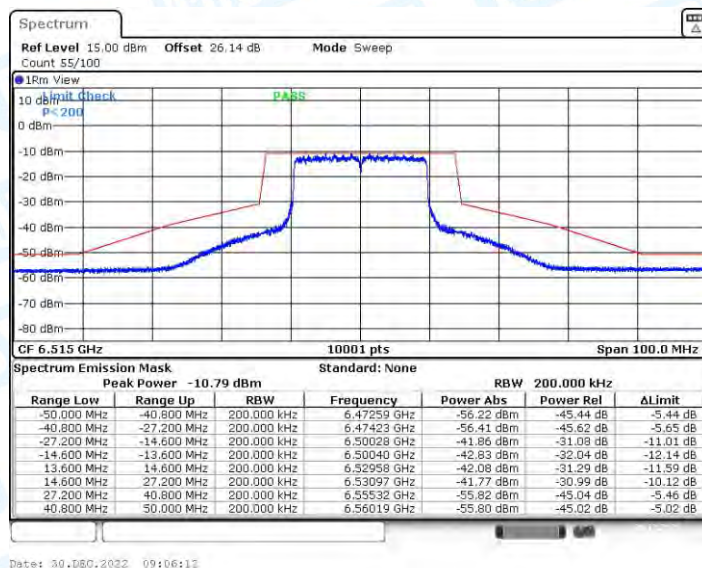
11AX20CDD_Ant3_6515
