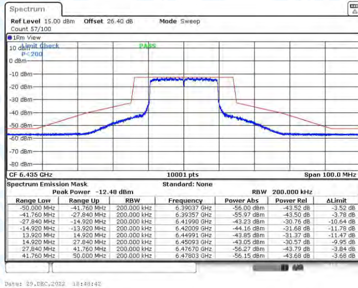
11AX20CDD_Ant3_6435
