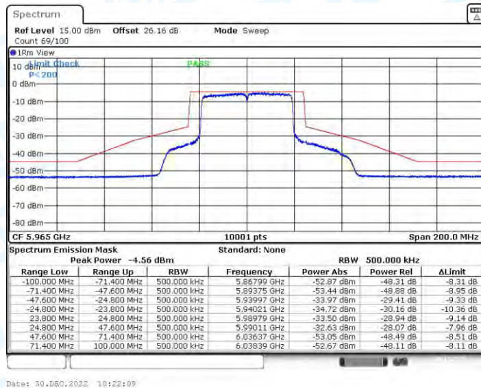
11AX40CDD_Ant4_5965
