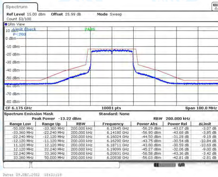
11AX20CDD_Ant3_6175
