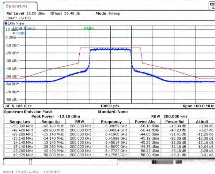
11AX20CDD_Ant4_6435
