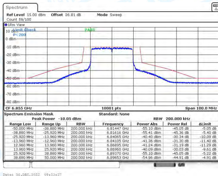
11AX20CDD_Ant3_6855
