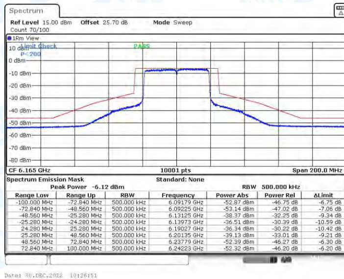
11AX40CDD_Ant2_6165
