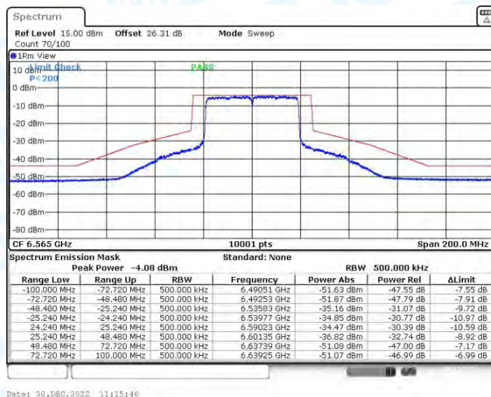
11AX40CDD_Ant4_6565
