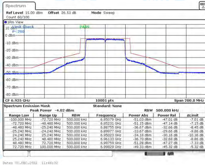
11AX40CDD_Ant2_6925
