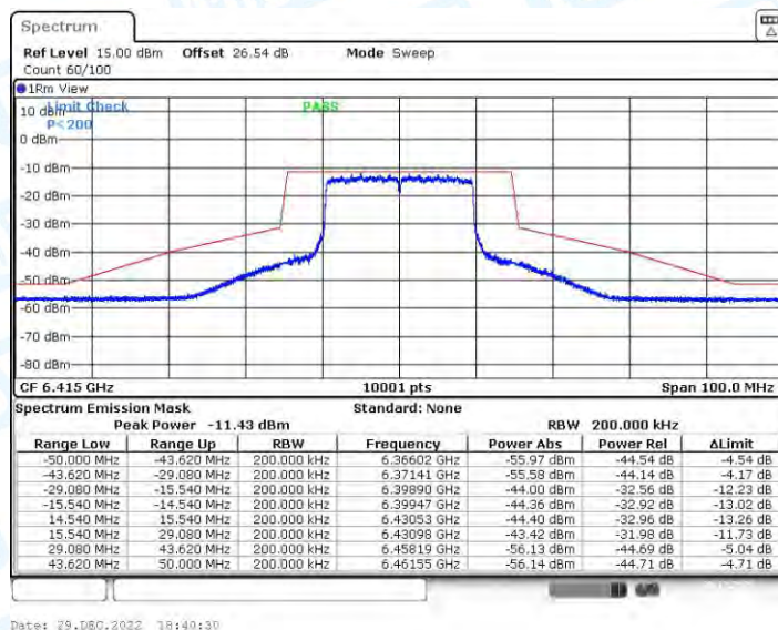
11AX20CDD_Ant3_6415
