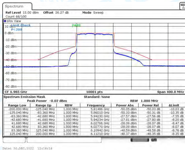
11AX80CDD_Ant3_5985
