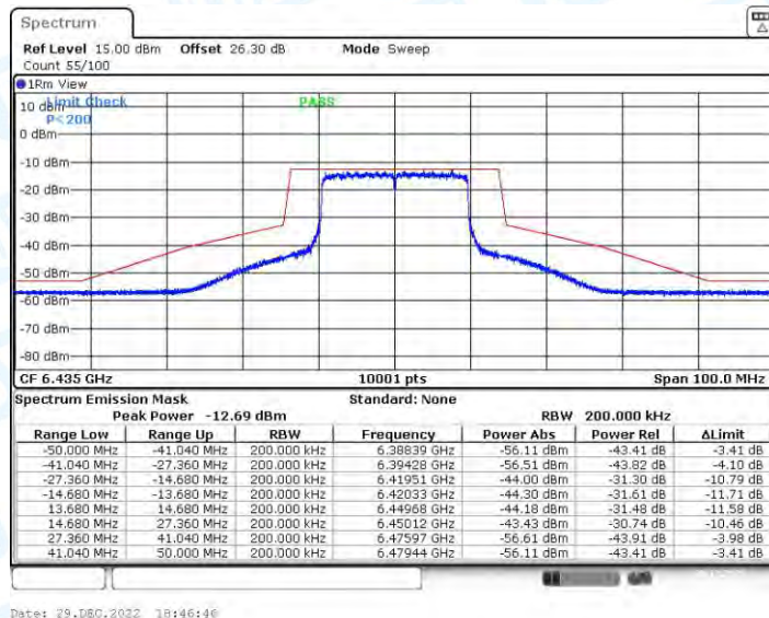
11AX20CDD_Ant2_6435
