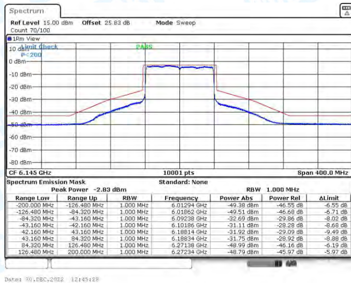
11AX80CDD_Ant4_6145
