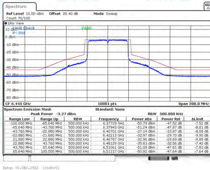
11AX40CDD_Ant3_6445
