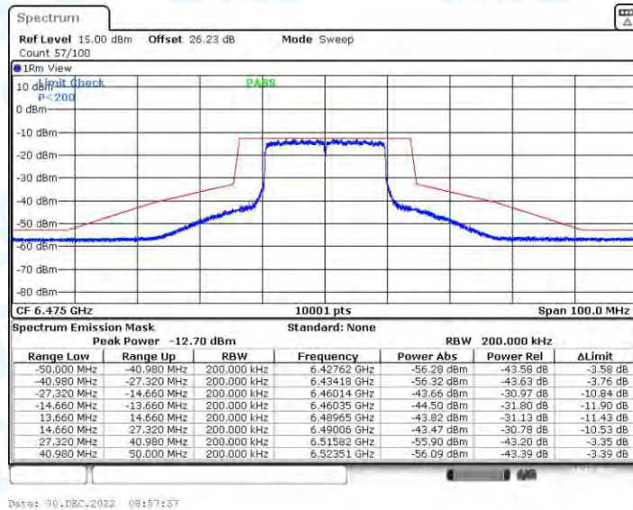
11AX20CDD_Ant3_6475
