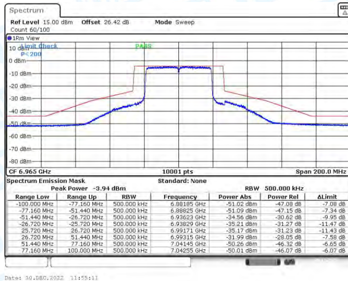
11AX40CDD_Ant2_6965
