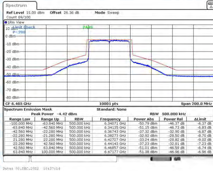
11AX40CDD_Ant3_6405
