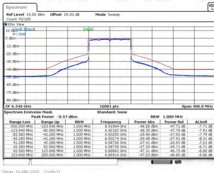
11AX80CDD_Ant2_6545
