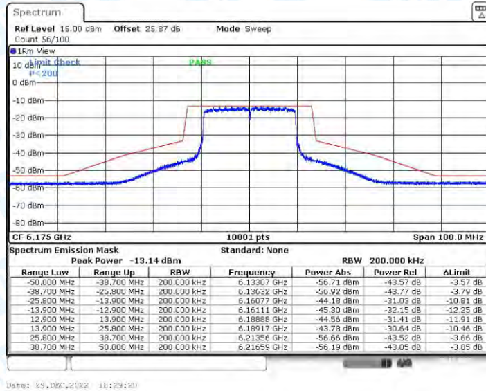
11AX20CDD_Ant2_6175
