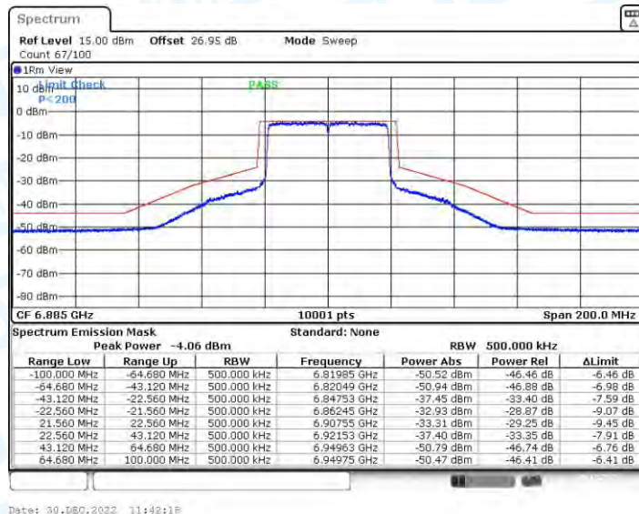
11AX40CDD_Ant4_6885
