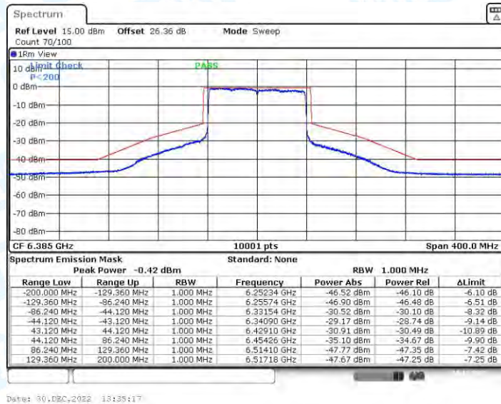
11AX80CDD_Ant3_6385
