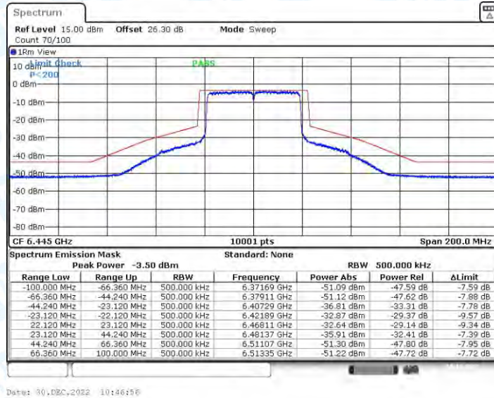
11AX40CDD_Ant2_6445
