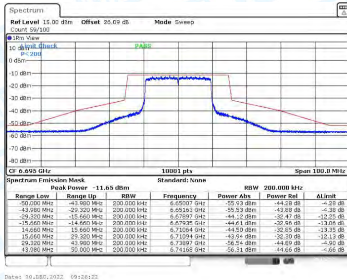
11AX20CDD_Ant4_6695
