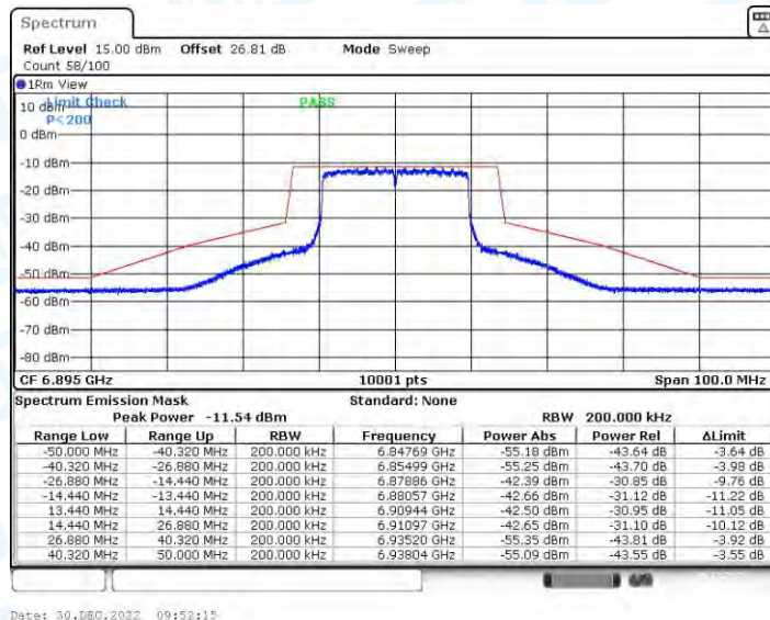
11AX20CDD_Ant4_6895
