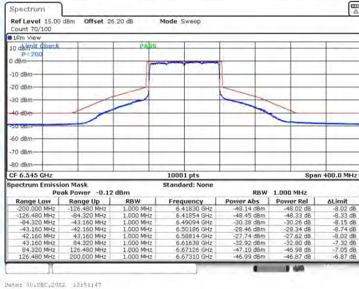
11AX80CDD_Ant3_6545
