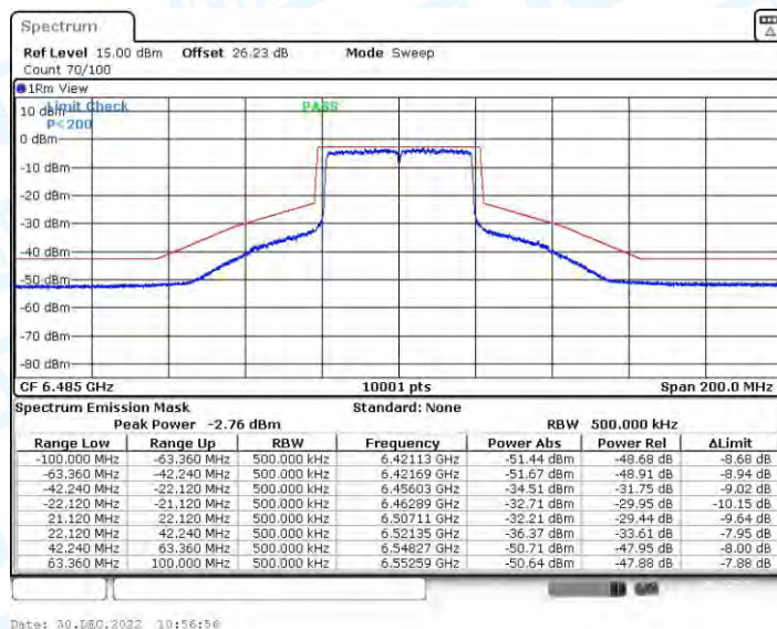
11AX40CDD_Ant3_6485
