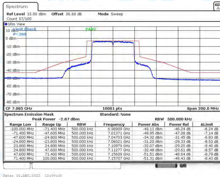
11AX40CDD_Ant4_7085
