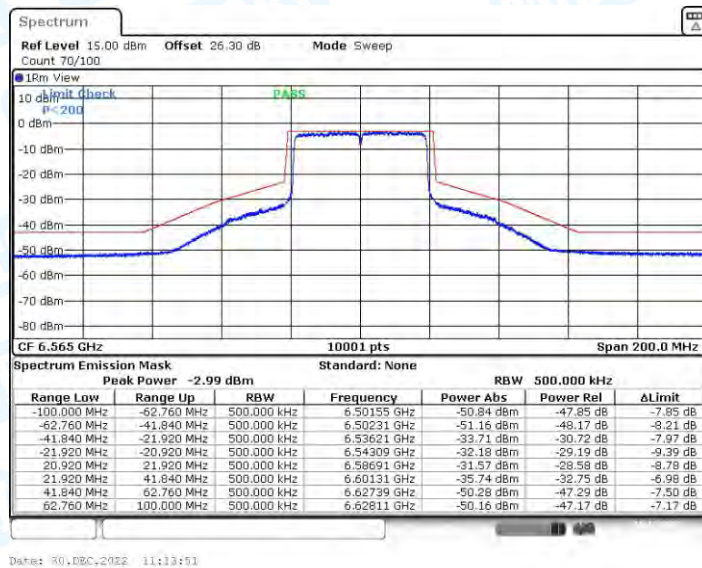
11AX40CDD_Ant3_6565
