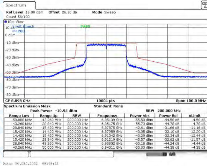
11AX20CDD_Ant2_6895
