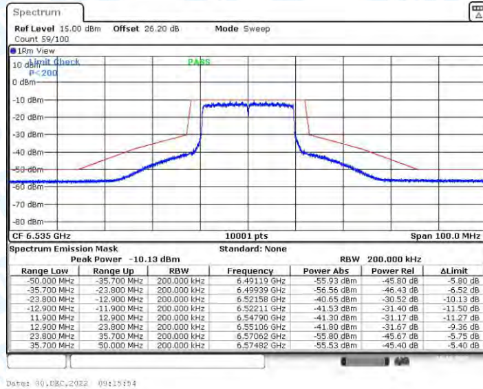
11AX20CDD_Ant3_6535
