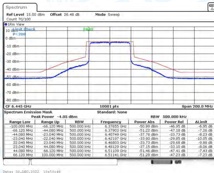
11AX40CDD_Ant4_6445
