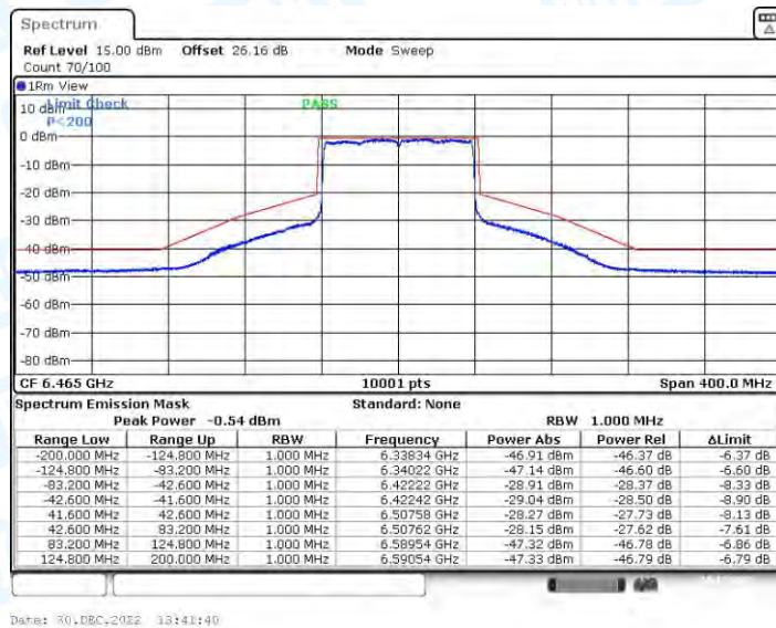
11AX80CDD_Ant2_6465
