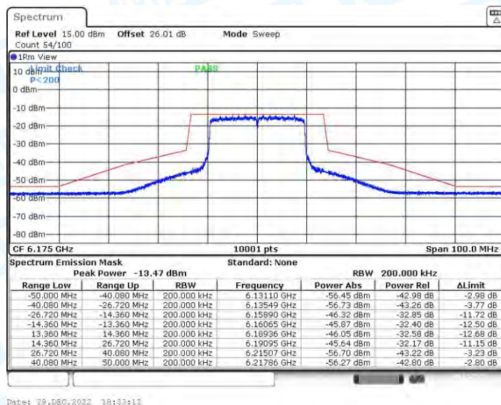
11AX20CDD_Ant4_6175
