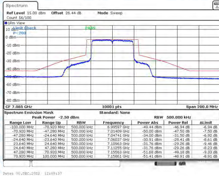
11AX40CDD_Ant2_7085
