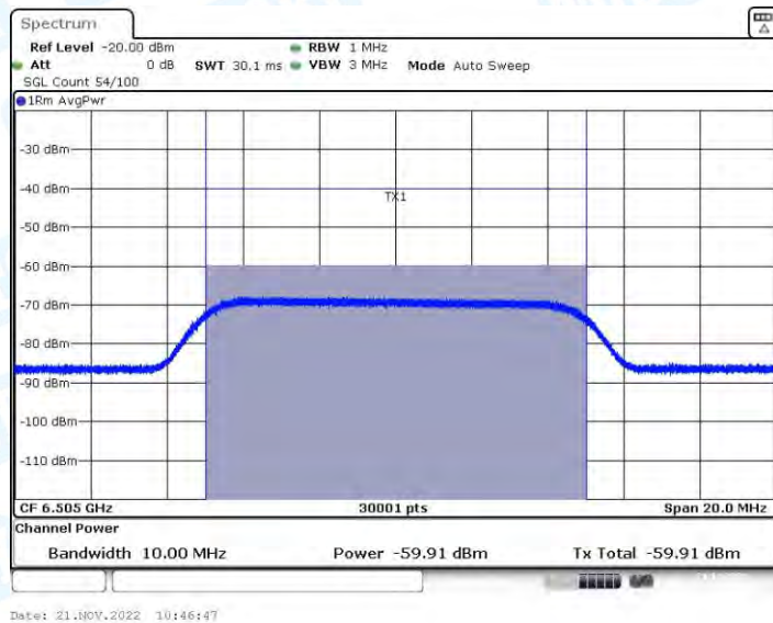
11AX160_Ant1_6505_Center_6505_OFF
