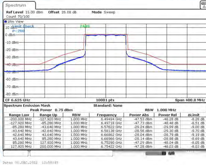
11AX80CDD_Ant2_6625
