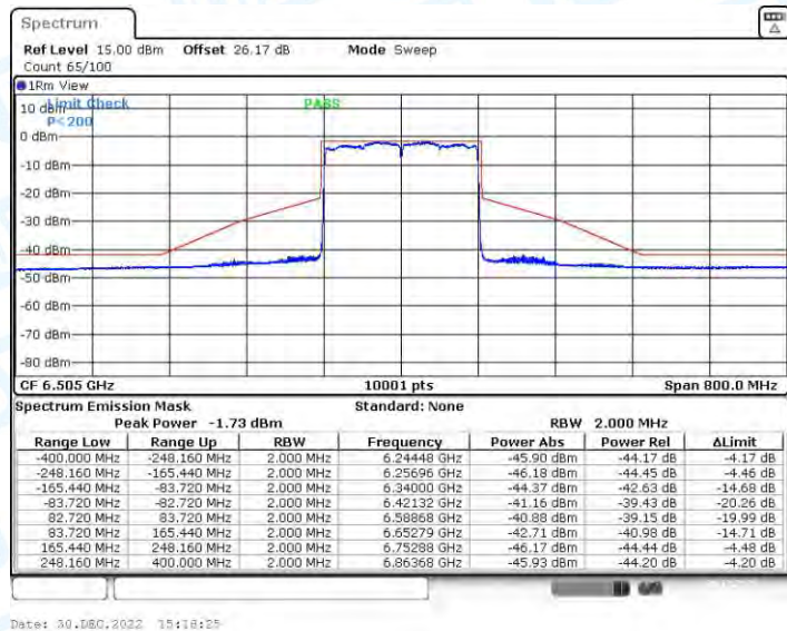
11AX160CDD_Ant4_6505
