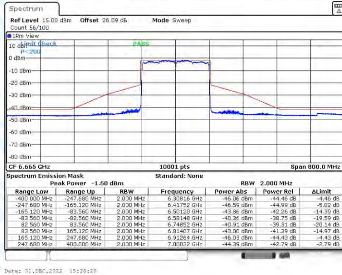
11AX160CDD_Ant4_6665
