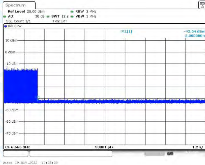
11AX160_Ant1_6665_Center_6665_OFF
