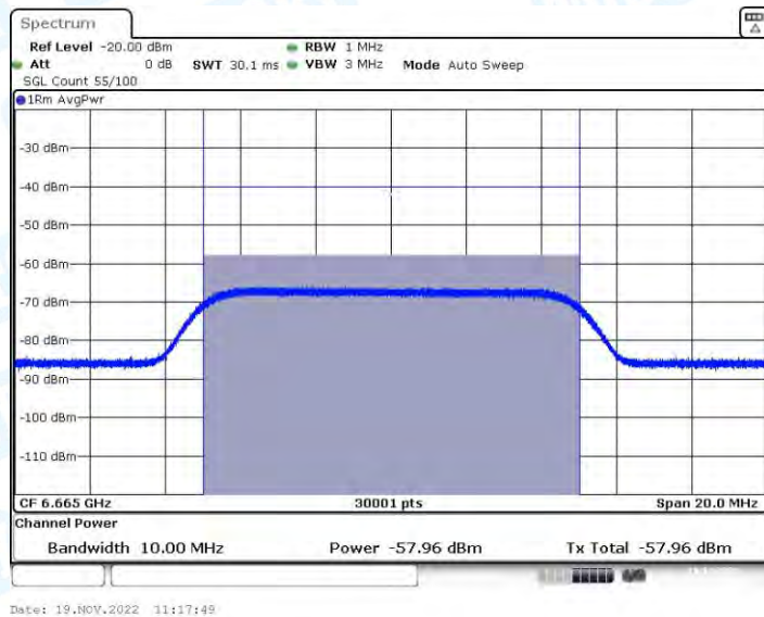
11AX160_Ant1_6665_Center_6665_OFF
