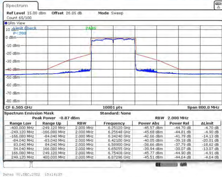
11AX160CDD_Ant2_6505
