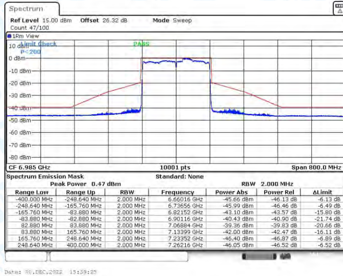
11AX160CDD_Ant2_6985
