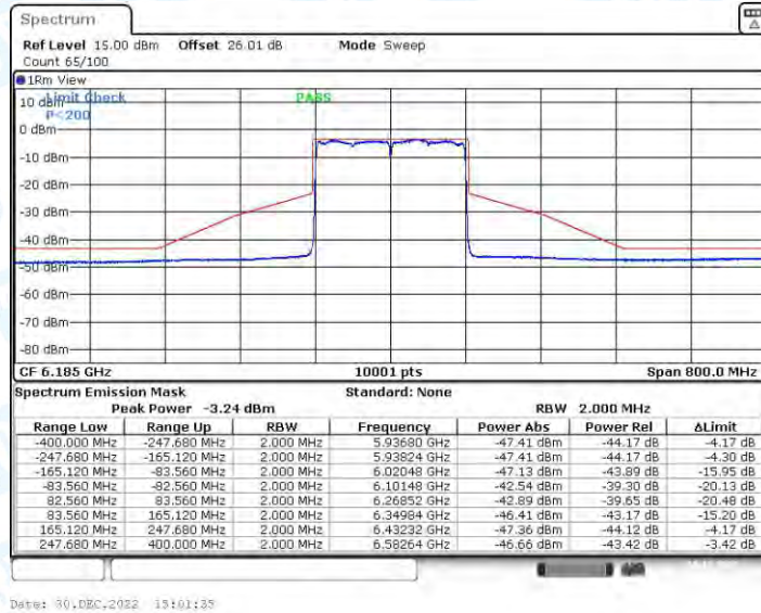
11AX160CDD_Ant4_6185
