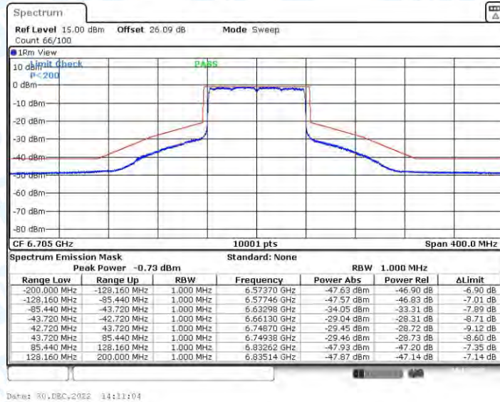
11AX80CDD_Ant4_6705
