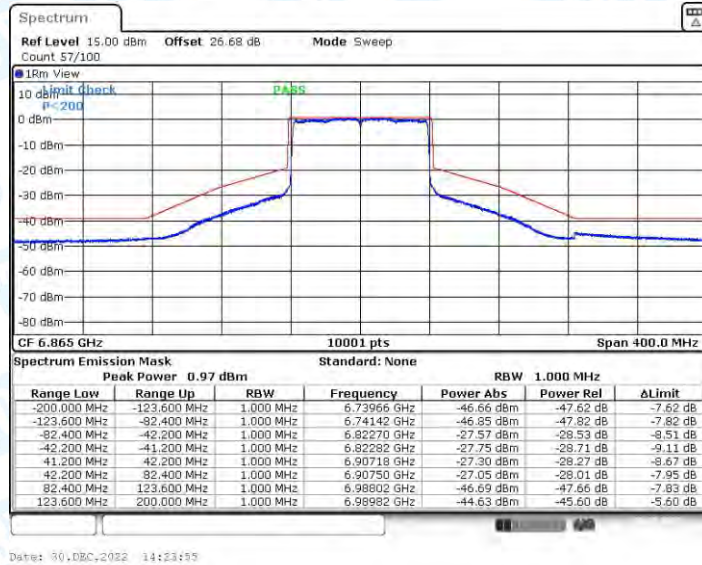
11AX80CDD_Ant2_6865
