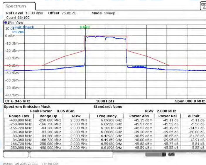
11AX160CDD_Ant2_6345
