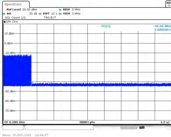
11AX160_Ant1_6505_Center_6505_OFF
