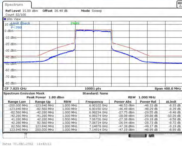
11AX80CDD_Ant3_7025
