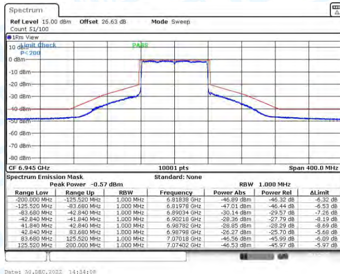
11AX80CDD_Ant3_6945
