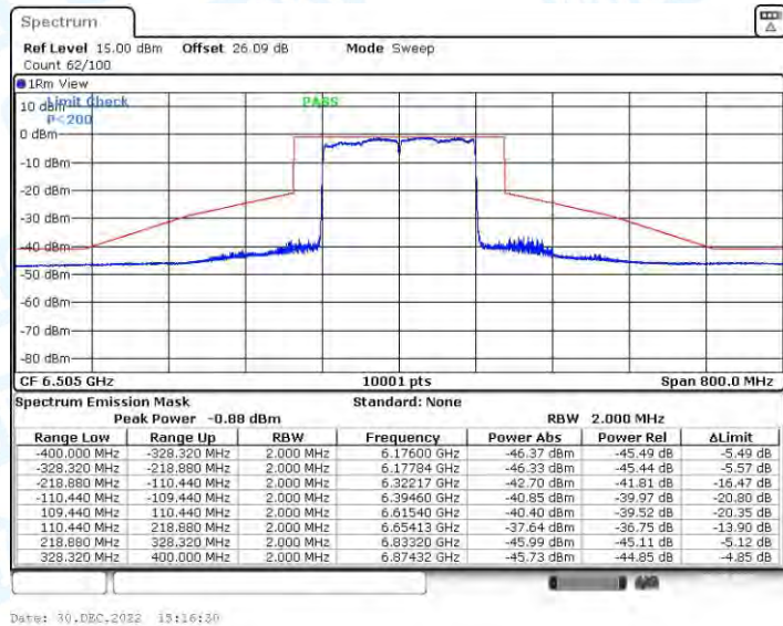
11AX160CDD_Ant3_6505
