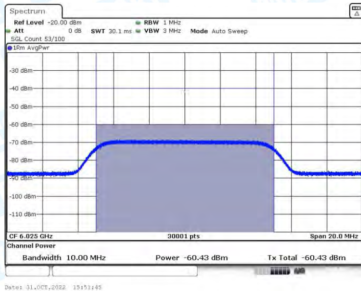
11AX160_Ant1_6025_Center_6025_OFF
