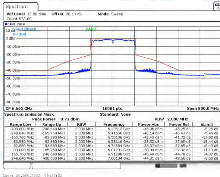
11AX160CDD_Ant3_6665
