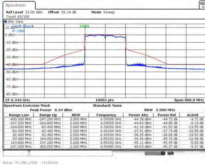
11AX160CDD_Ant3_6345
