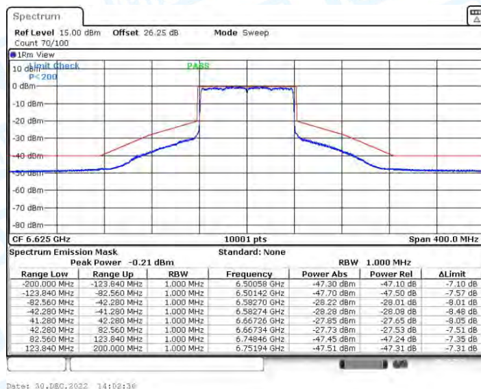
11AX80CDD_Ant4_6625
