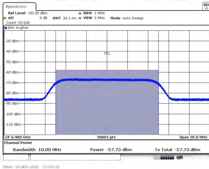
11AX160_Ant1_6985_Center_6985_OFF
