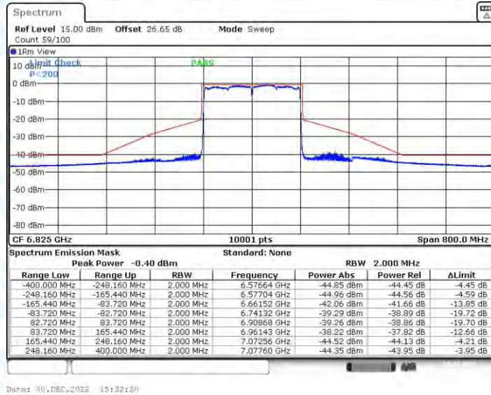
11AX160CDD_Ant3_6825
