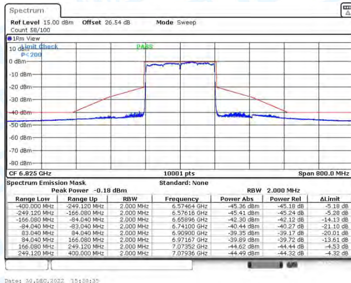
11AX160CDD_Ant2_6825
