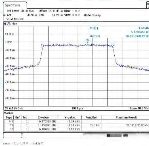
11AX40_CDD-Ant4-6165
