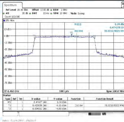
11AX80_CDD-Ant3-6465
