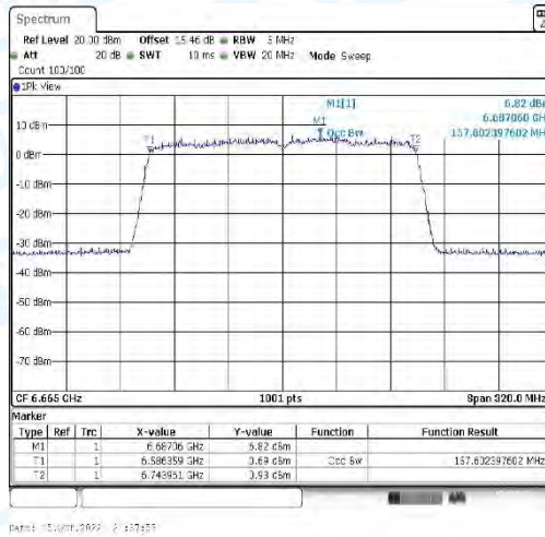
11AX160_CDD-Ant1-6665
