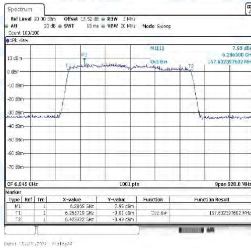
11AX160_CDD-Ant1-6345
