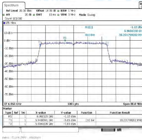
11AX40_CDD-Ant4-6965
