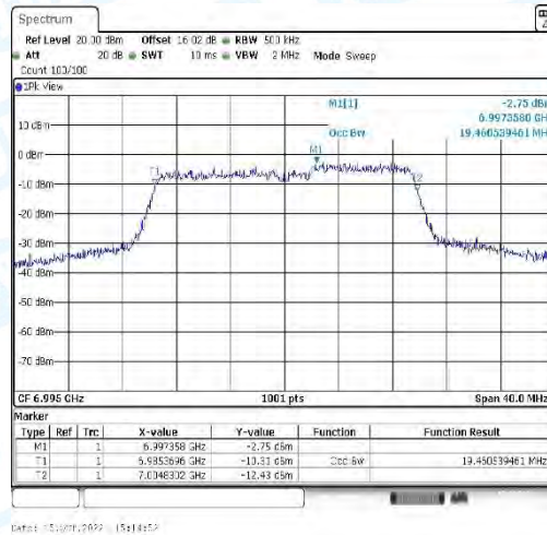
11AX20_CDD-Ant4-6995
