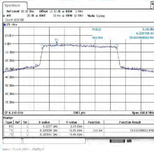
11AX80_CDD-Ant3-6145
