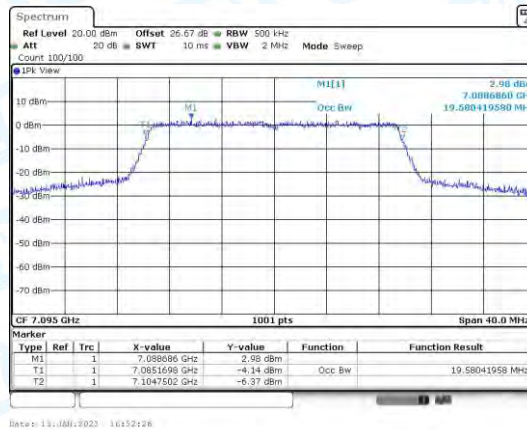
11AX20_CDD-Ant4-7095
