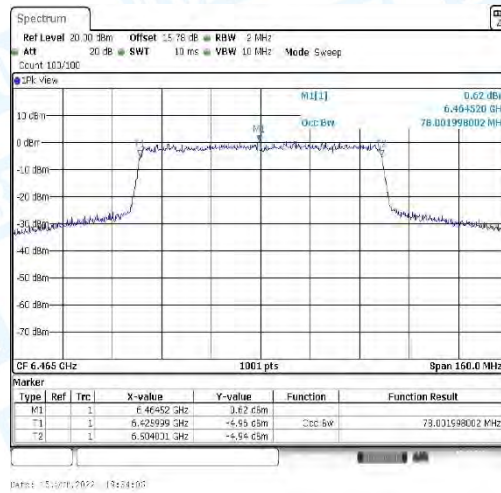
11AX80_CDD-Ant2-6465
