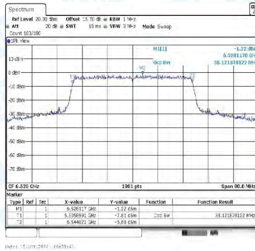
11AX40_CDD-Ant4-6525
