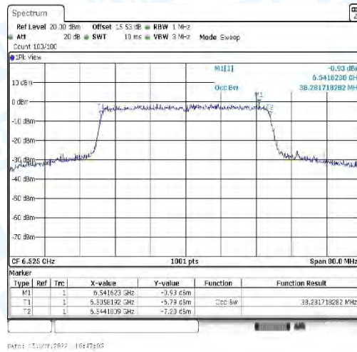
11AX40_CDD-Ant1-6525
