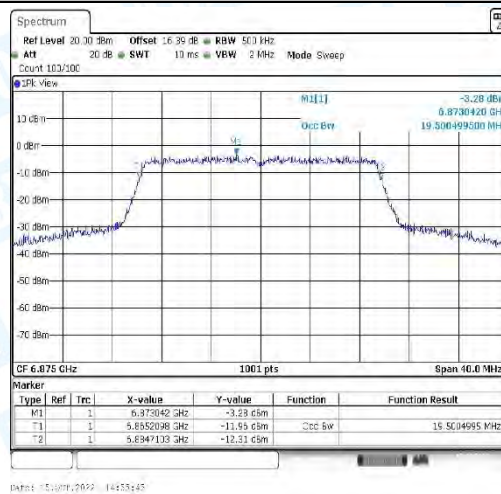
11AX20_CDD-Ant4-6875
