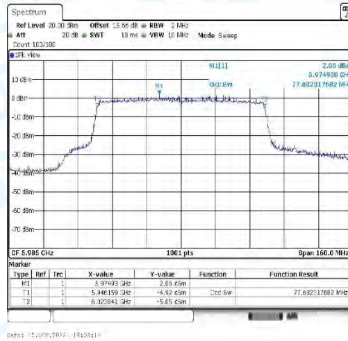
11AX80_CDD-Ant1-5985
