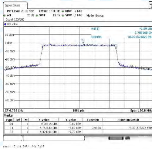
11AX80_CDD-Ant3-6785
