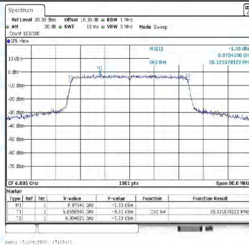
11AX40_CDD-Ant4-6885
