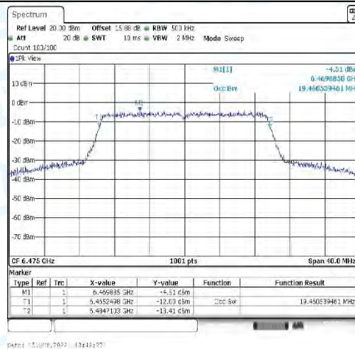
11AX20_CDD-Ant4-6475
