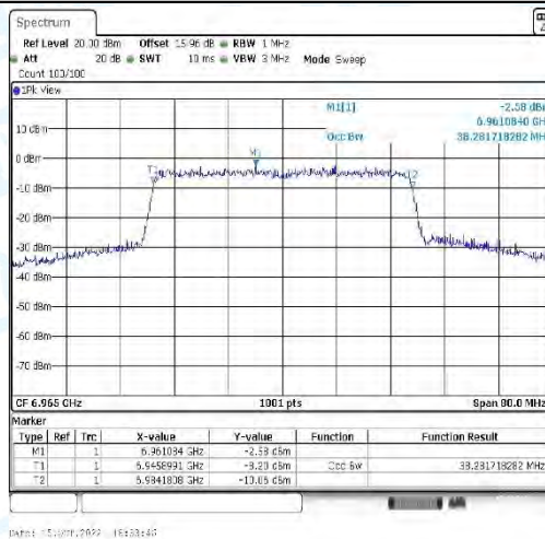
11AX40_CDD-Ant2-6965
