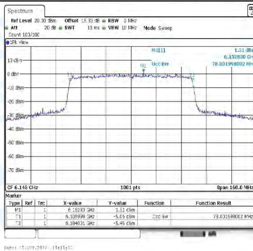
11AX80_CDD-Ant4-6145
