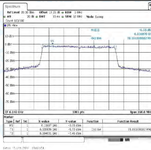
11AX80_CDD-Ant1-6145
