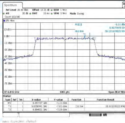
11AX40_CDD-Ant2-6845
