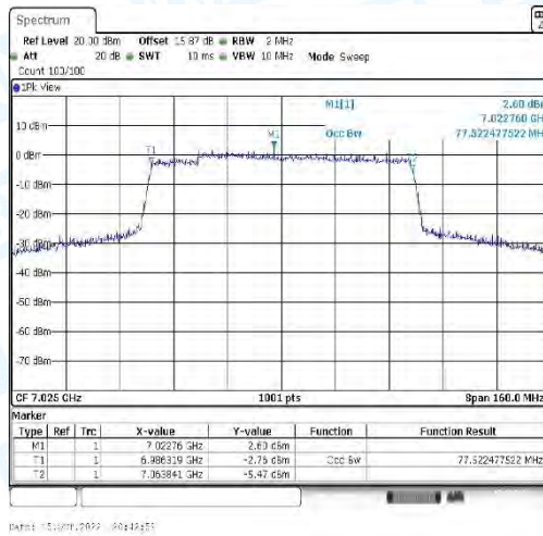
11AX80_CDD-Ant1-7025
