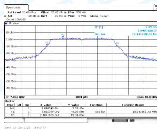
11A-CDD -Ant3-7095
