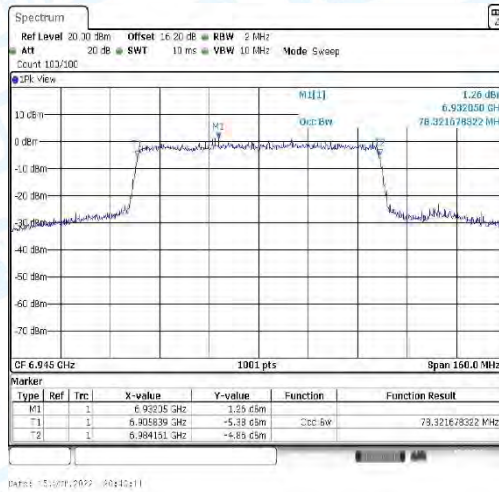
11AX80_CDD-Ant4-6945
