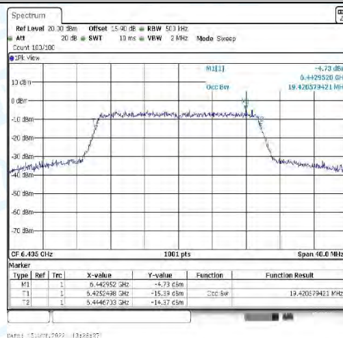
11AX20_CDD-Ant2-6435
