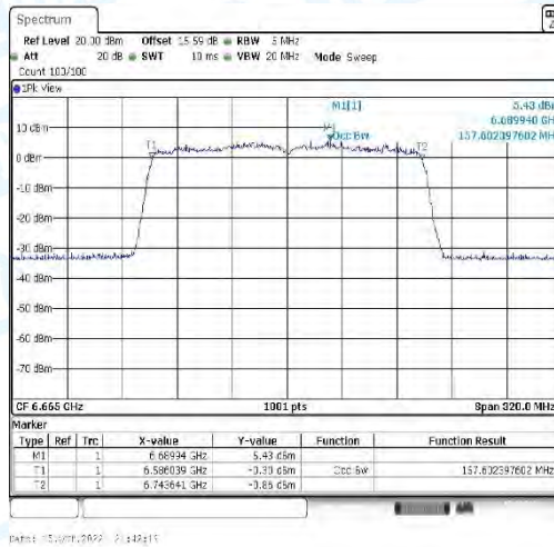
11AX160_CDD-Ant3-6665
