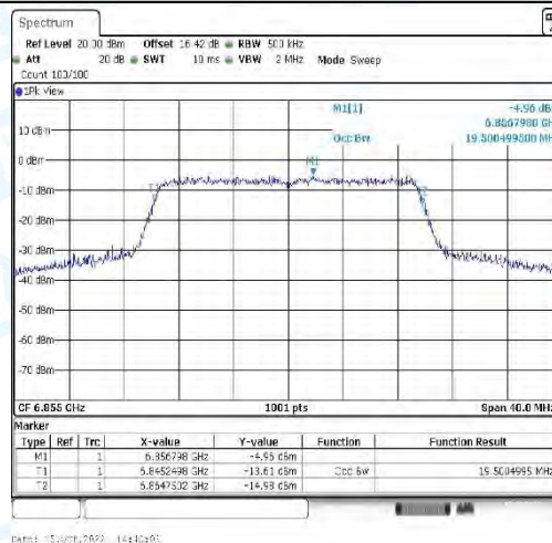
11AX20_CDD-Ant3-6855
