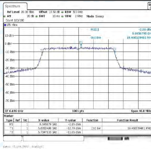
11AX20_CDD-Ant4-6695
