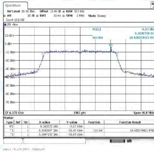
11AX20_CDD-Ant2-6175
