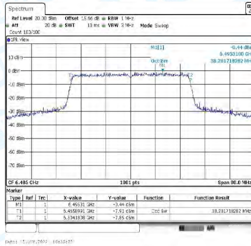
11AX40_CDD-Ant1-6485
