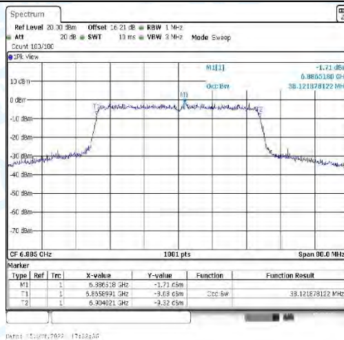
11AX40_CDD-Ant1-6885
