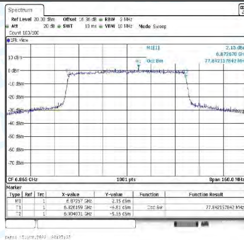
11AX80_CDD-Ant4-6865
