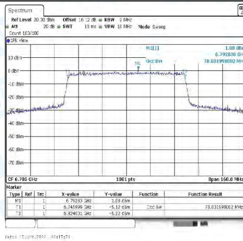
11AX80_CDD-Ant4-6785
