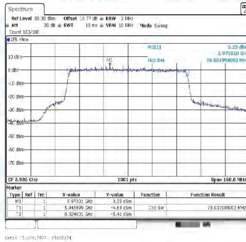
11AX80_CDD-Ant2-5985
