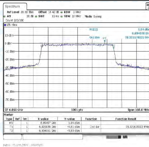
11AX80_CDD-Ant3-6865
