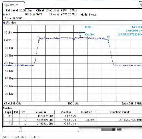
11AX160_CDD-Ant4-6665
