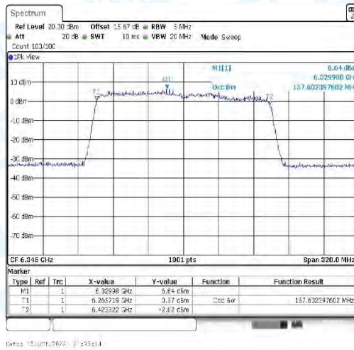
11AX160_CDD-Ant4-6345
