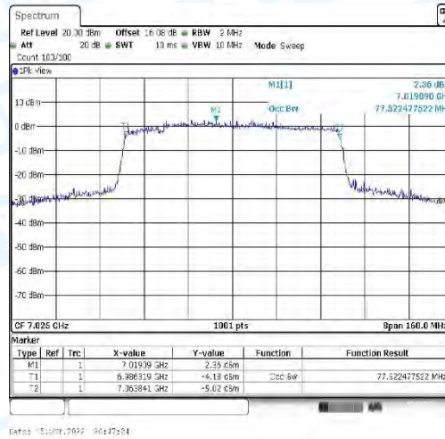
11AX80_CDD-Ant3-7025
