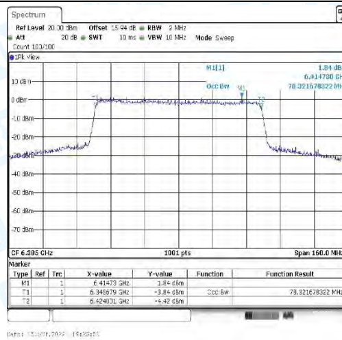
11AX80_CDD-Ant3-6385
