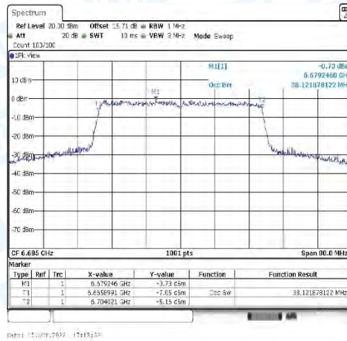
11AX40_CDD-Ant2-6685
