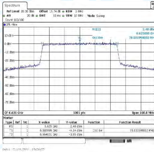
11AX80_CDD-Ant2-6625
