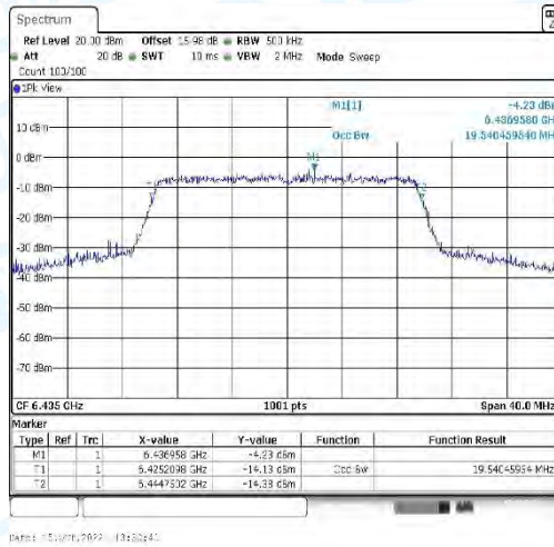
11AX20_CDD-Ant3-6435
