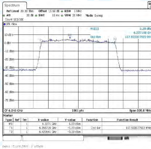
11AX160_CDD-Ant3-6345
