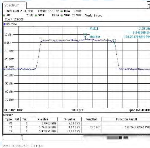
11AX160_CDD-Ant2-6825
