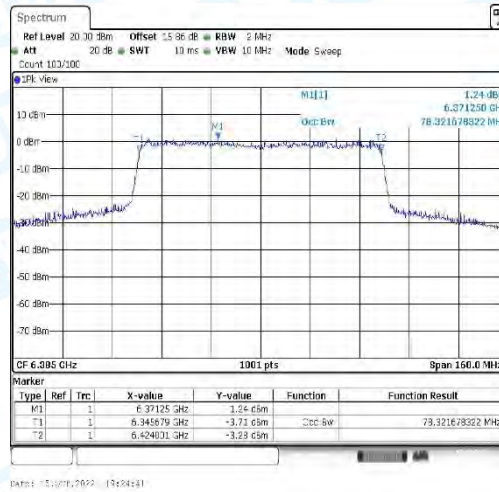
11AX80_CDD-Ant2-6385
