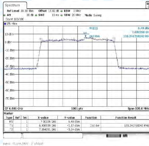
11AX160_CDD-Ant1-6985
