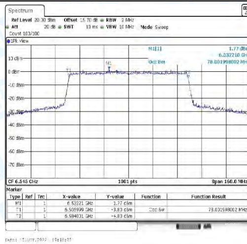
11AX80_CDD-Ant4-6545
