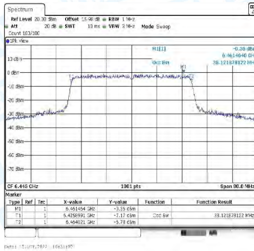
11AX40_CDD-Ant3-6445
