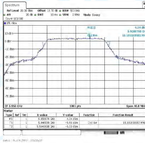
11A-CDD -Ant4-5955
