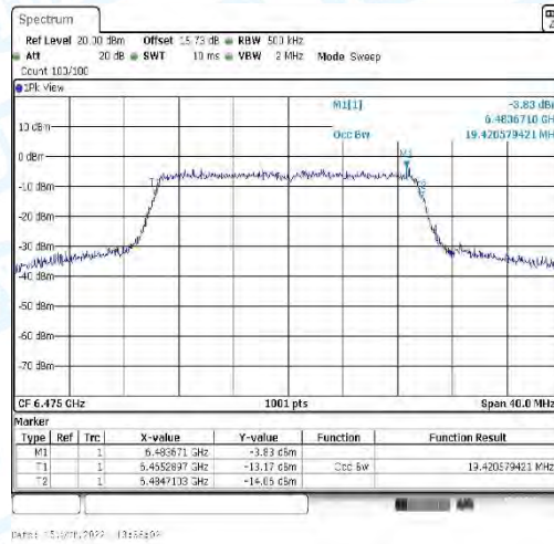
11AX20_CDD-Ant2-6475
