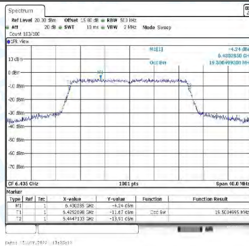
11AX20_CDD-Ant1-6435
