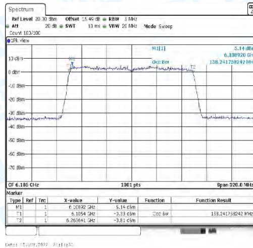
11AX160_CDD-Ant2-6185
