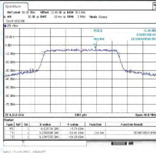
11AX20_CDD-Ant3-6515
