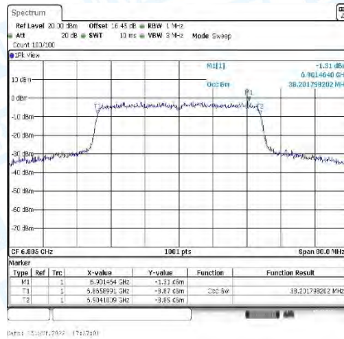
11AX40_CDD-Ant3-6885
