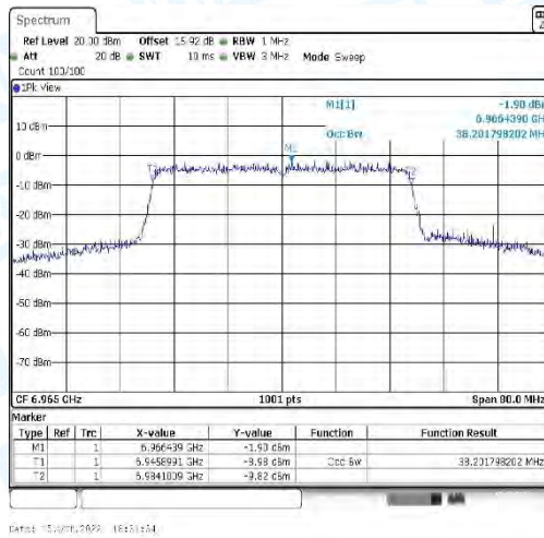
11AX40_CDD-Ant1-6965
