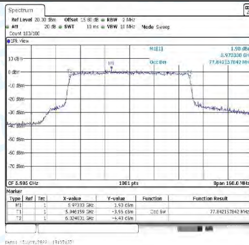
11AX80_CDD-Ant3-5985
