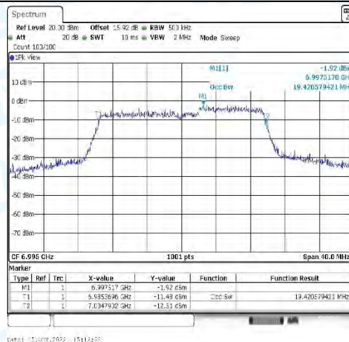
11AX20_CDD-Ant3-6995
