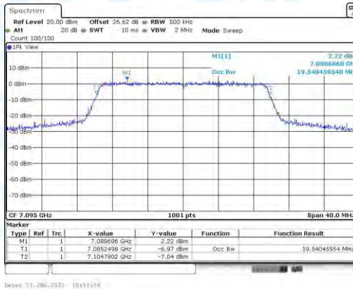
11AX20_CDD-Ant2-7095
