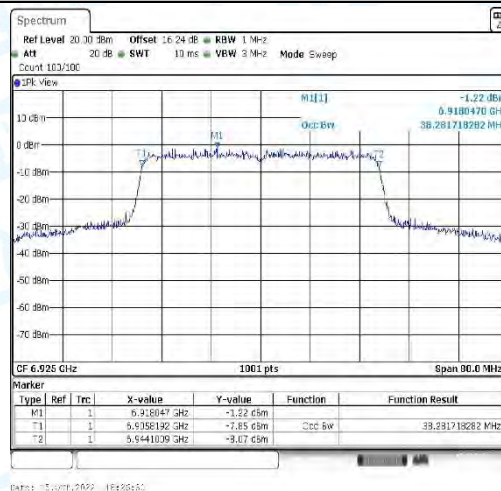
11AX40_CDD-Ant3-6925
