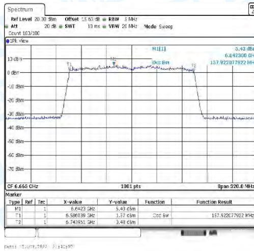
11AX160_CDD-Ant2-6665
