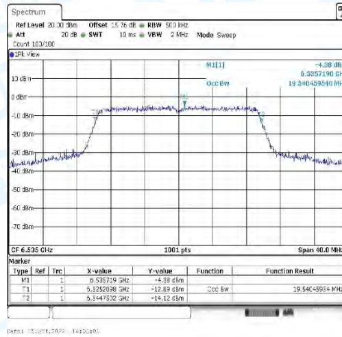
11AX20_CDD-Ant3-6535
