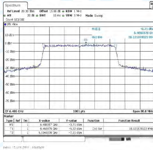
11AX40_CDD-Ant4-6485
