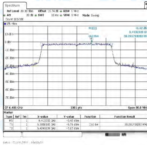
11AX40_CDD-Ant1-6405
