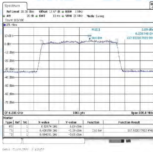
11AX160_CDD-Ant3-6505
