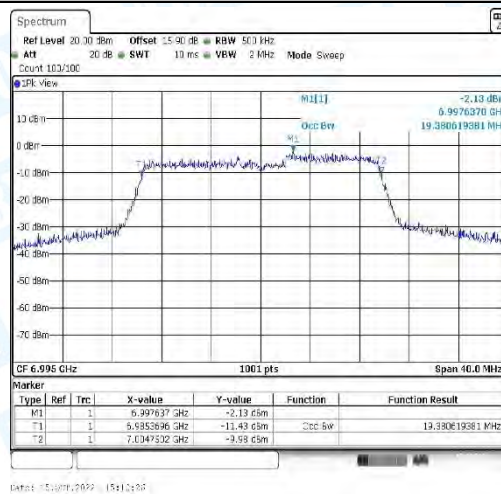
11AX20_CDD-Ant2-6995
