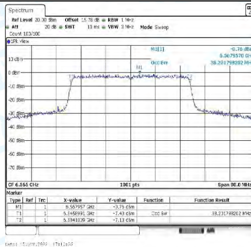
11AX40_CDD-Ant4-6565
