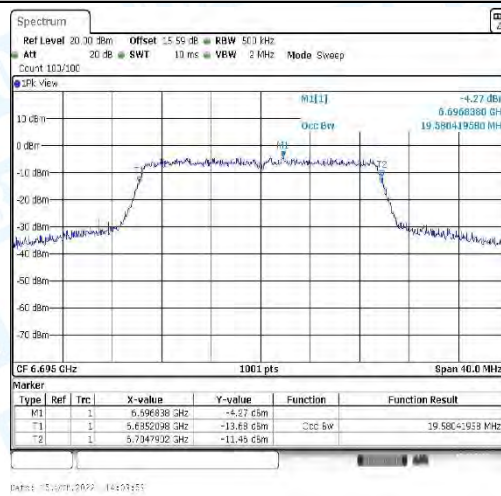
11AX20_CDD-Ant3-6695
