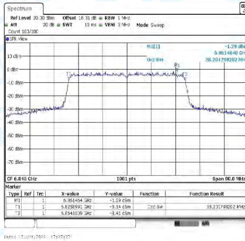
11AX40_CDD-Ant3-6845
