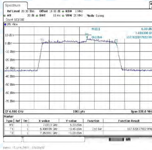
11AX160_CDD-Ant4-6985
