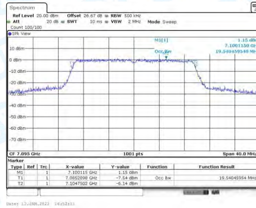
11AX20_CDD-Ant3-7095
