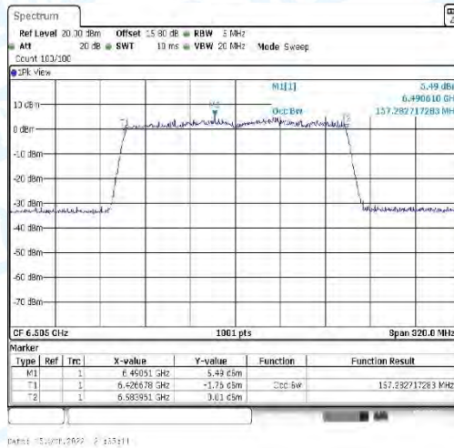
11AX160_CDD-Ant4-6505
