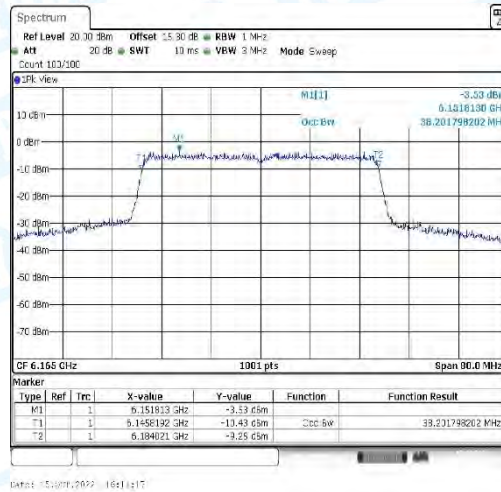
11AX40_CDD-Ant3-6165
