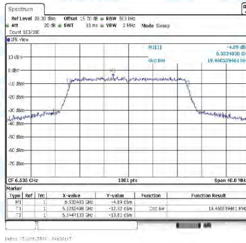
11AX20_CDD-Ant4-6535
