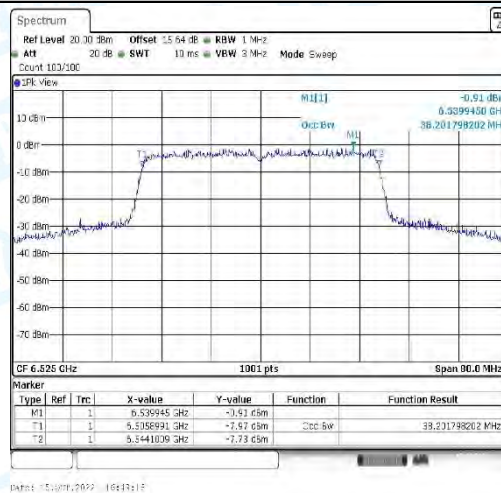
11AX40_CDD-Ant2-6525
