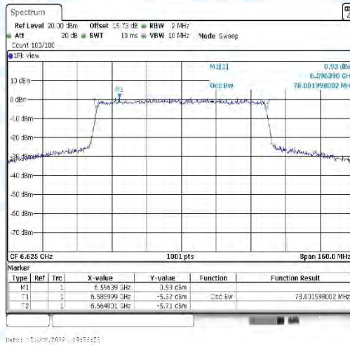
11AX80_CDD-Ant4-6625
