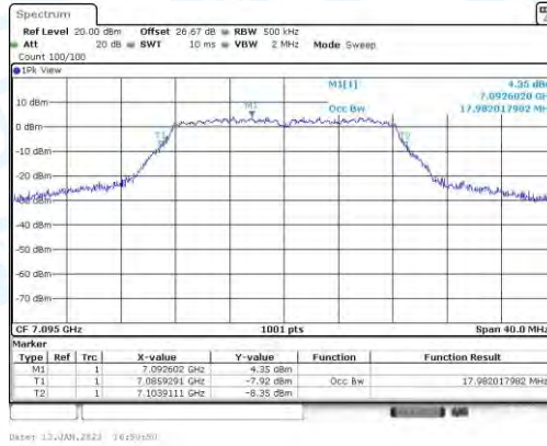
11A-CDD-Ant4-7095
