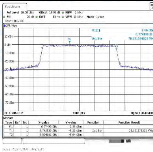
11AX80_CDD-Ant1-6785
