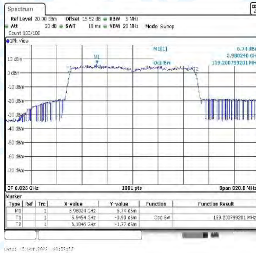
11AX160_CDD-Ant4-6025
