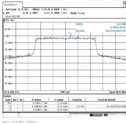
11AX40_CDD-Ant4-6405
