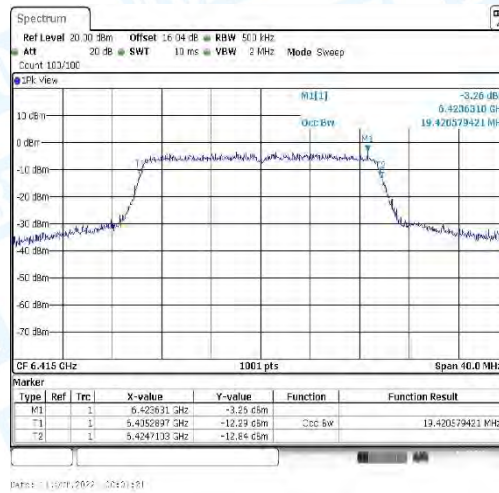
11AX20_CDD-Ant2-6415
