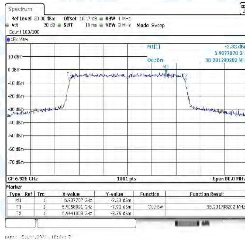
11AX40_CDD-Ant2-6925
