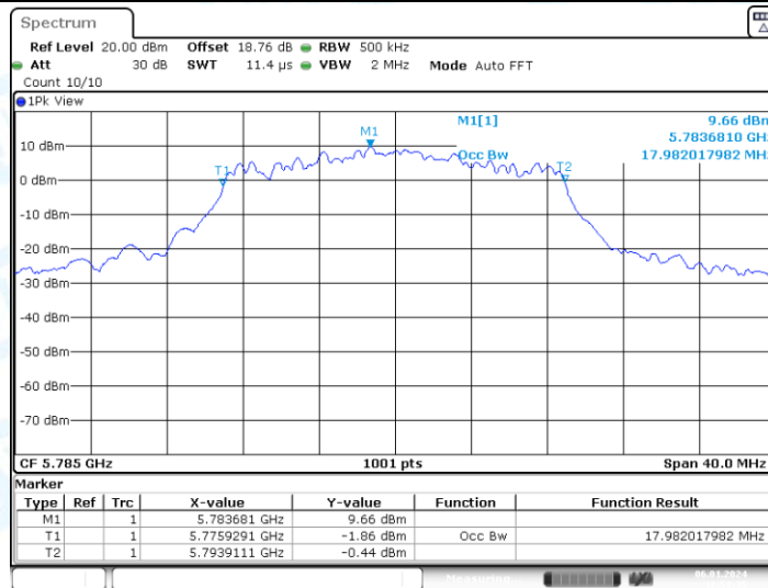
11AC20-CDD_Ant2_5785
