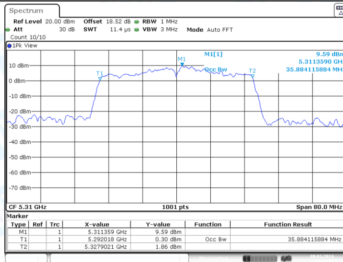
11AC40-CDD_Ant2_5310
