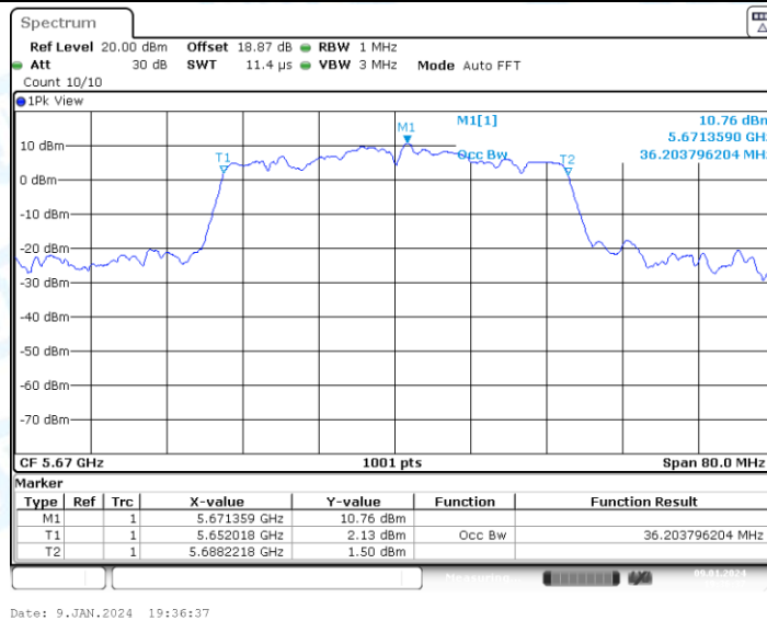
11AC40-CDD_Ant2_5670
