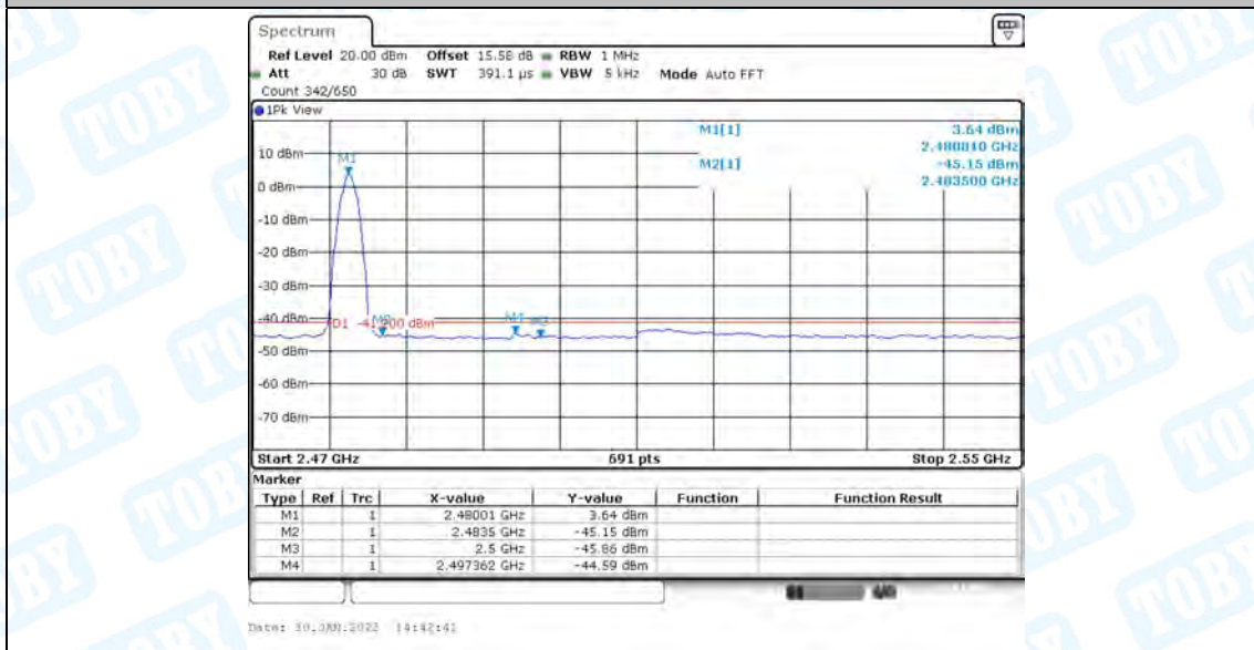
2DH5_AntA_High_2480_Peak
