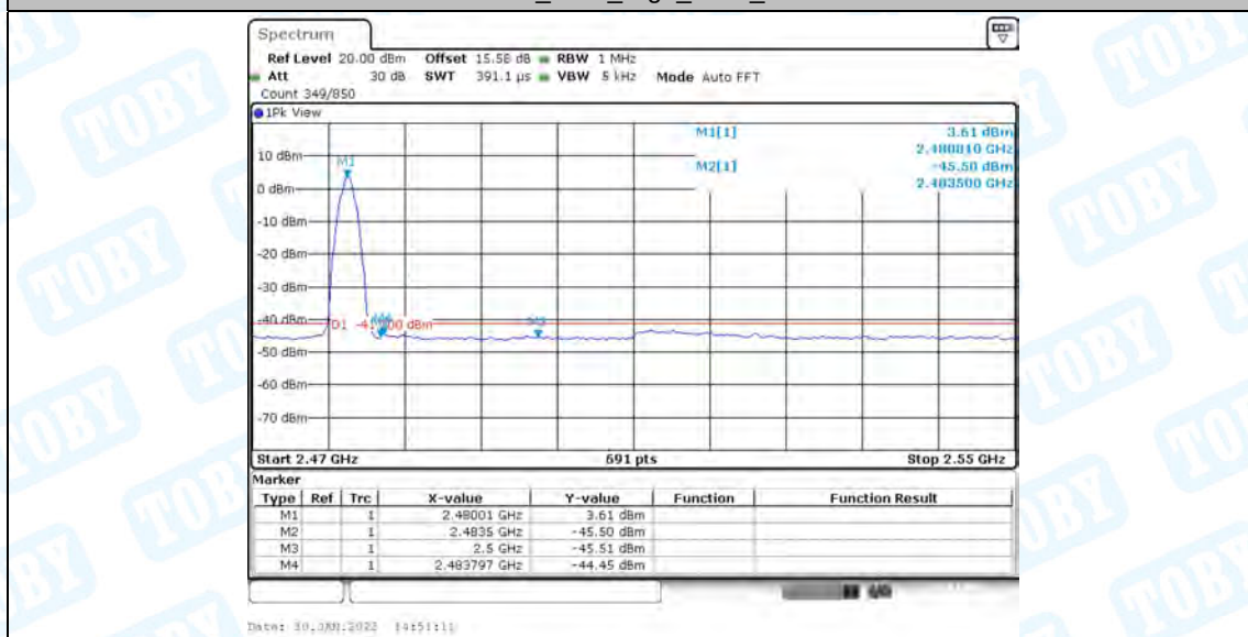
3DH5_AntA_High_2480_Peak
