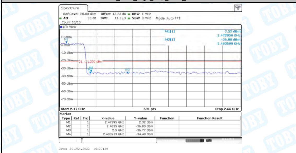
3DH5_AntA_High_Hop_2480_Peak
