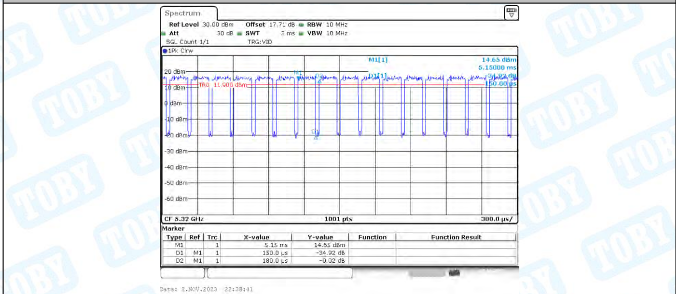
11AC20_Ant2_5320
