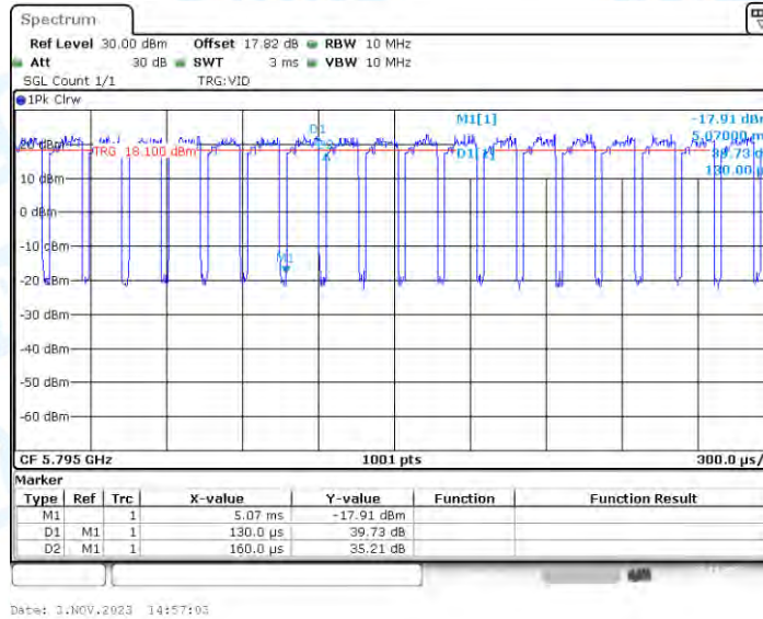
11AC40_Ant4_5795
