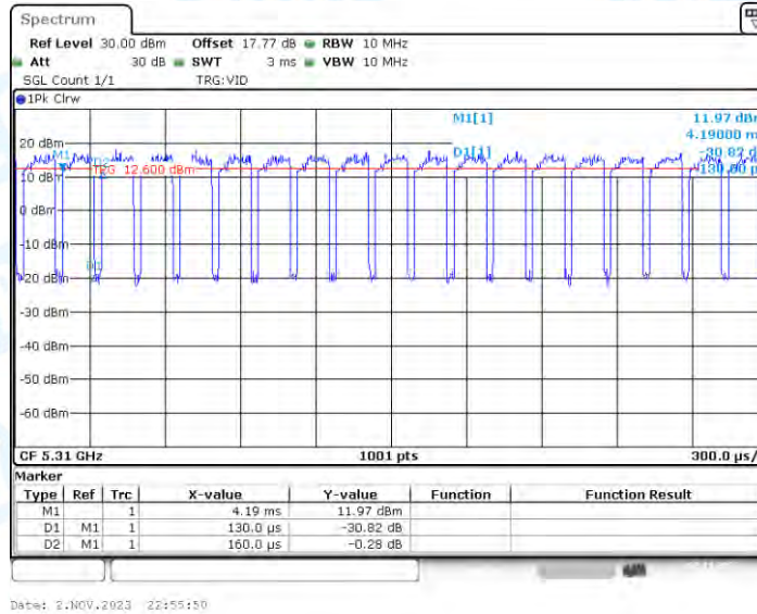
11AC40_Ant4_5310
