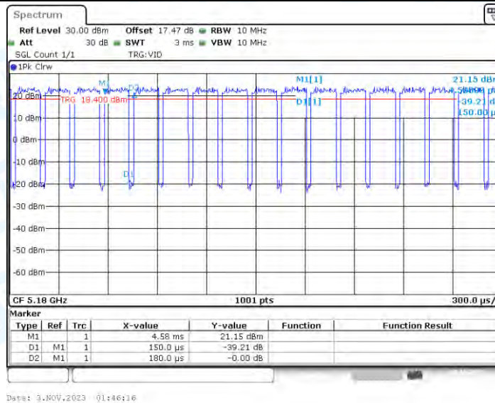
11AC20_Ant3_5180
