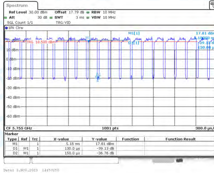
11AC40_Ant3_5755
