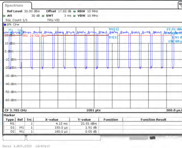
11AC20_Ant4_5785
