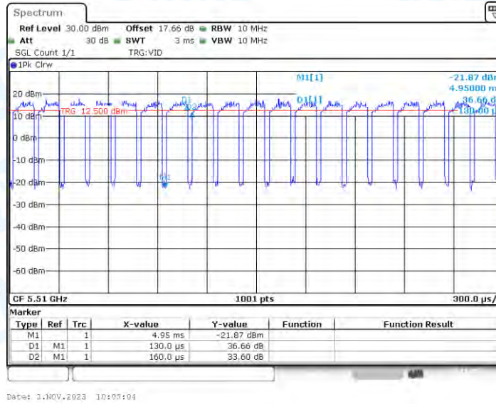
11AC40_Ant3_5510
