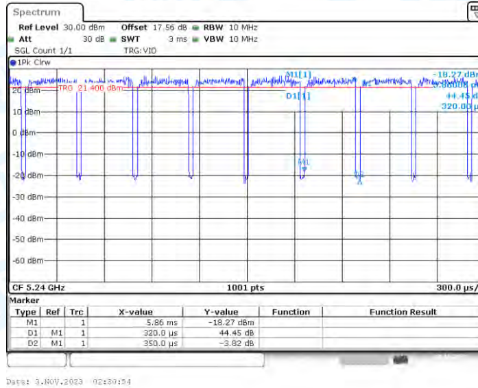
11AX20_Ant3_5240
