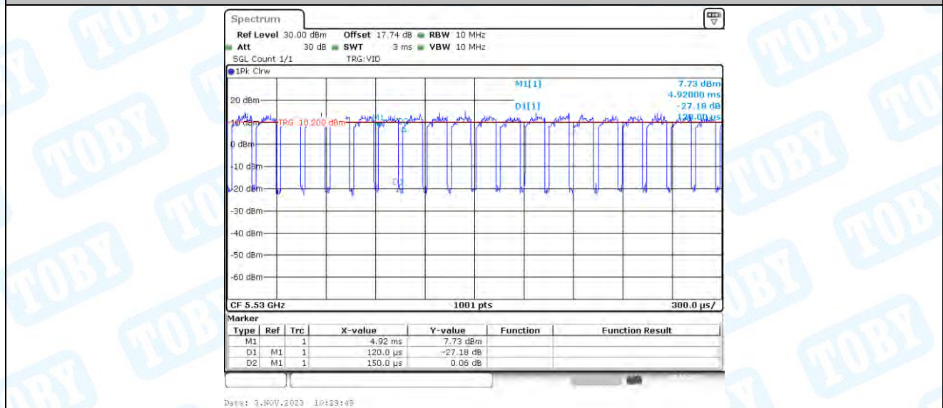
11AC80_Ant2_5530
