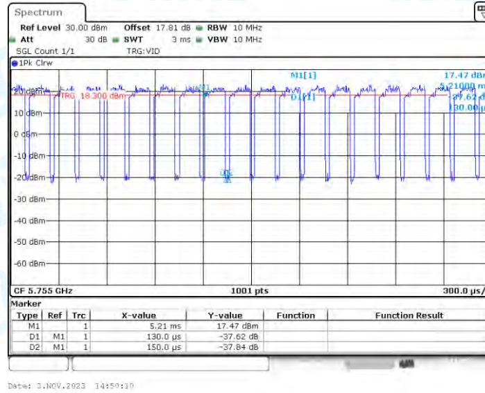
11AC40_Ant2_5755
