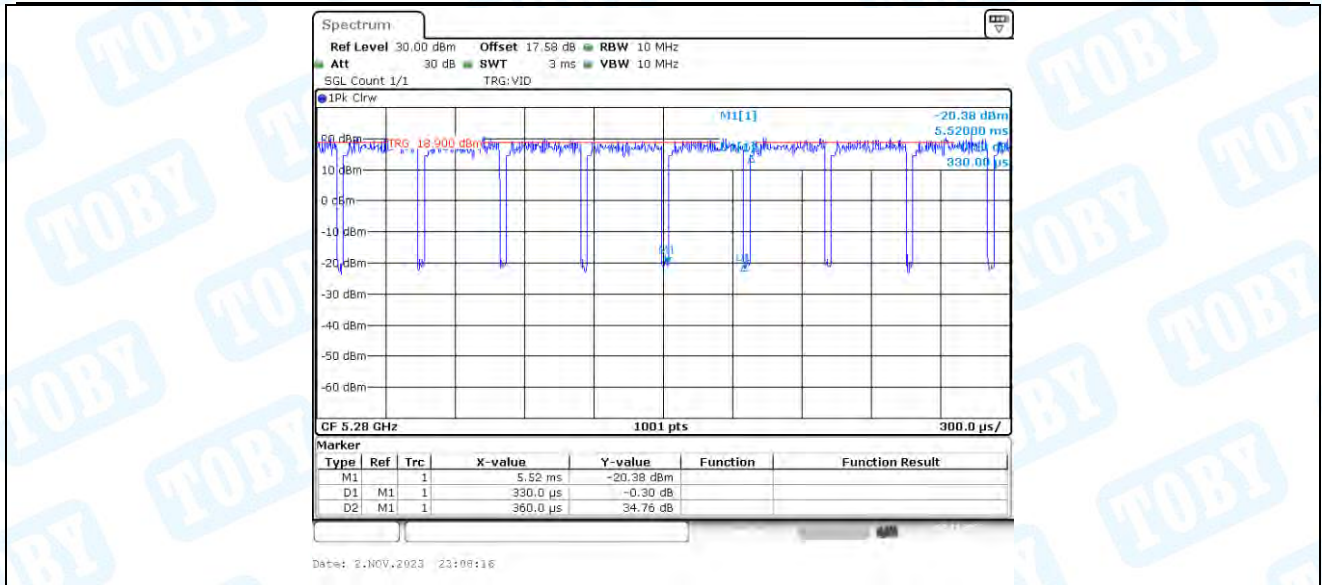
11AX20_Ant3_5280
