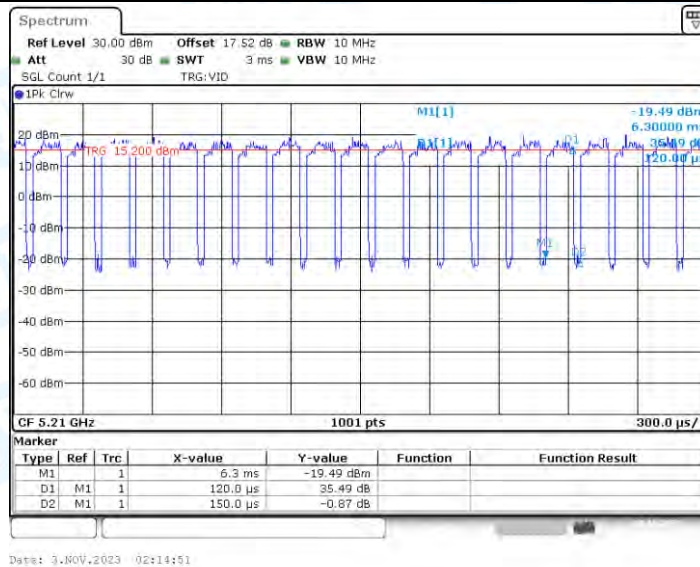
11AC80_Ant4_5210
