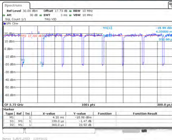
11AX20_Ant3_5720
