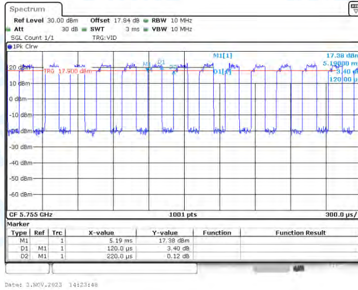
11N40_Ant4_5755
