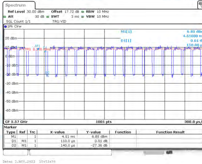
11AC160_Ant2_5570
