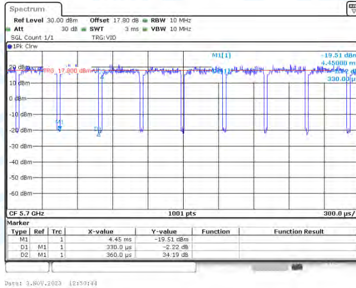
11AX20_Ant3_5700
