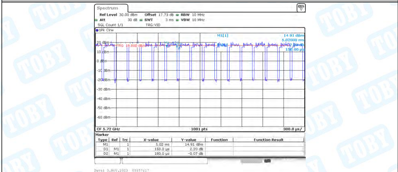
11AC20_Ant3_5720
