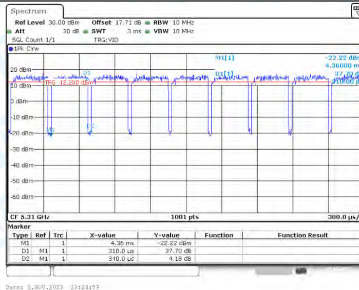
11AX40_Ant2_5310
