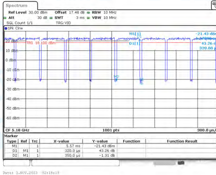
11AX20_Ant2_5180
