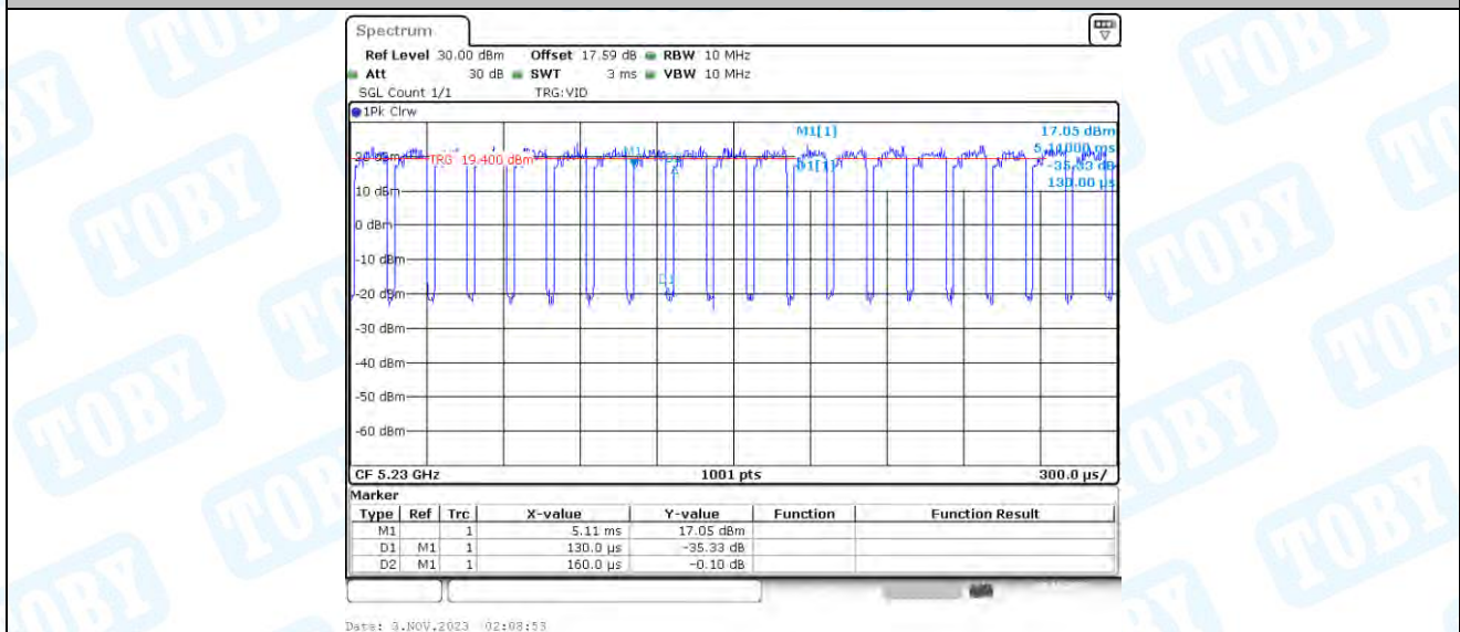
11AC40_Ant2_5230
