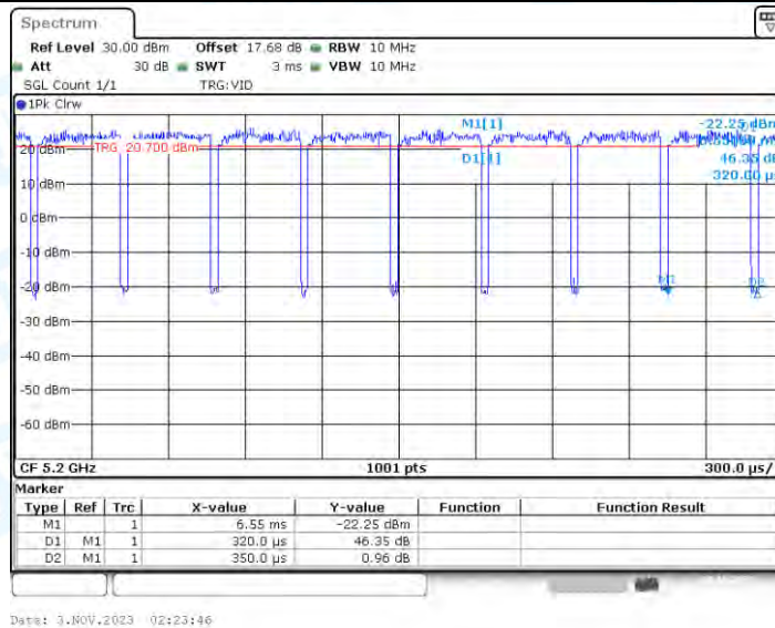
11AX20_Ant4_5200
