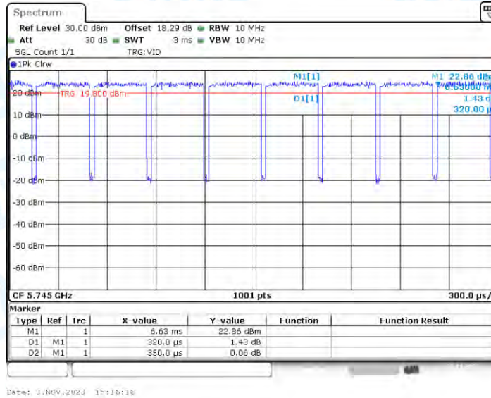
11AX20_Ant3_5745
