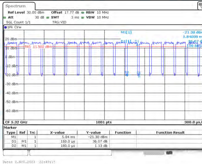
11AC20_Ant4_5320
