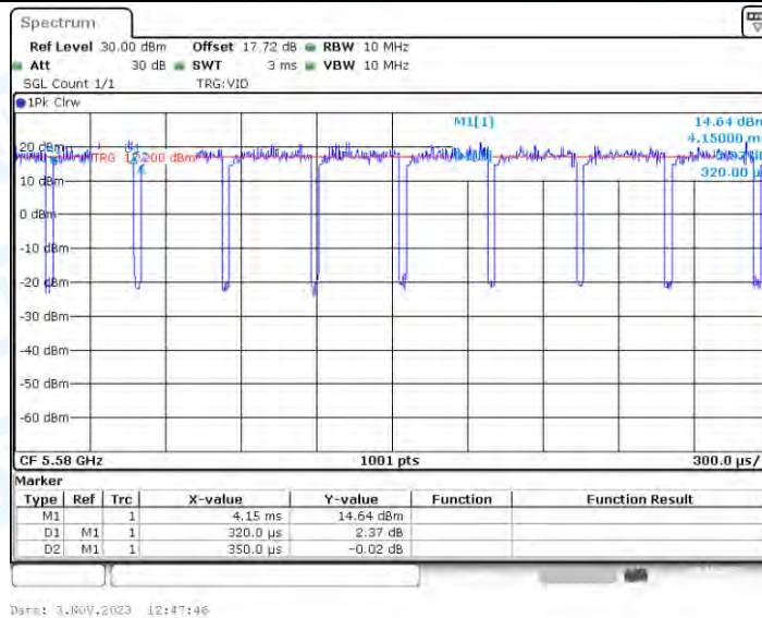
11AX20_Ant4_5580
