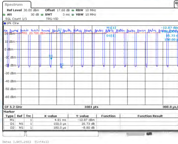
11AC20_Ant4_5200
