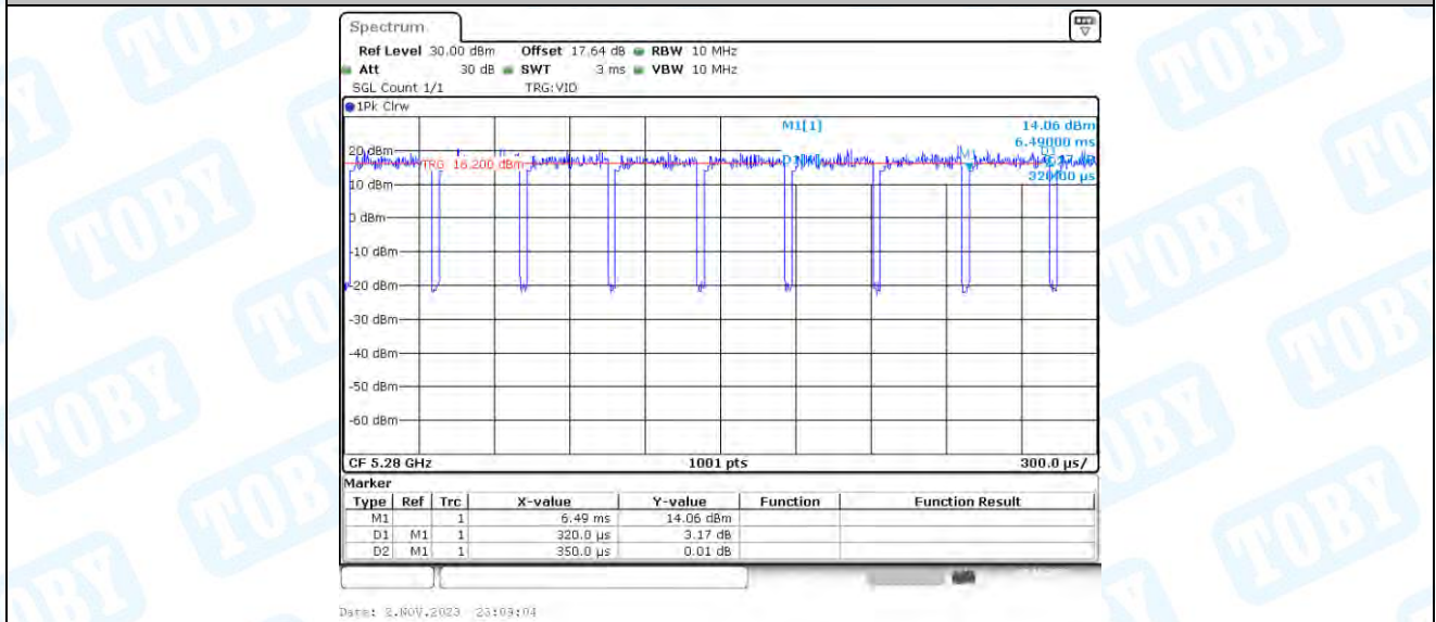
11AX20_Ant4_5280
