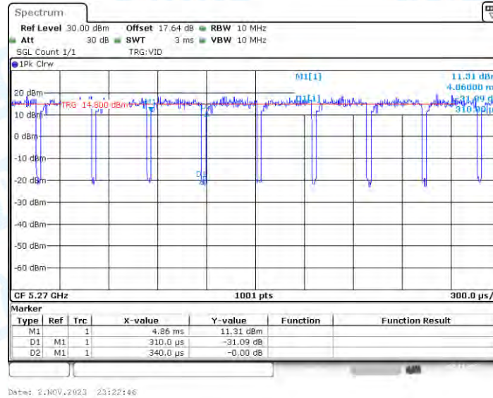
11AX40_Ant4_5270
