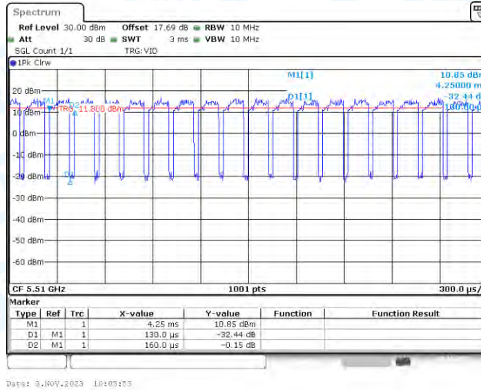
11AC40_Ant4_5510
