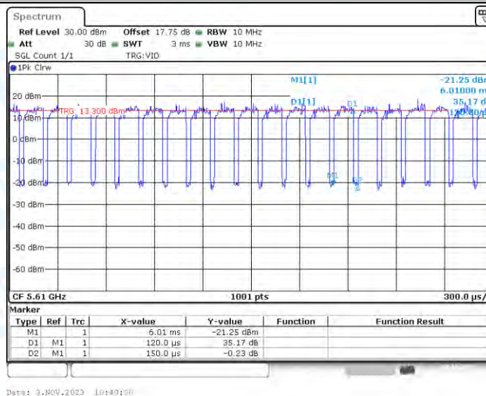
11AC80_Ant2_5610
