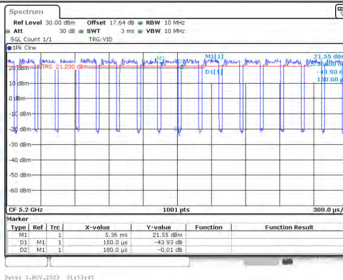
11AC20_Ant3_5200
