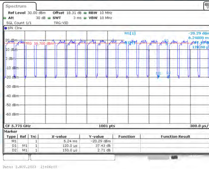
11AC80_Ant2_5775
