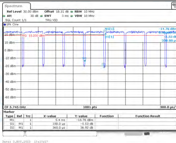
11AX20_Ant2_5745
