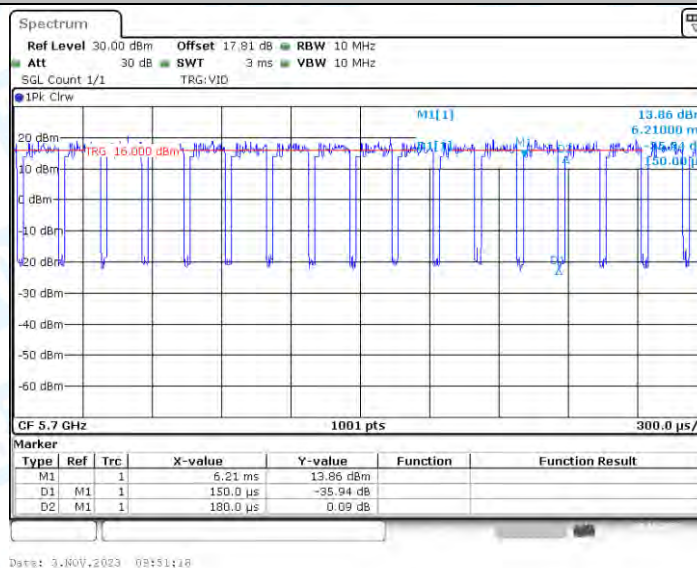
11AC20_Ant2_5700
