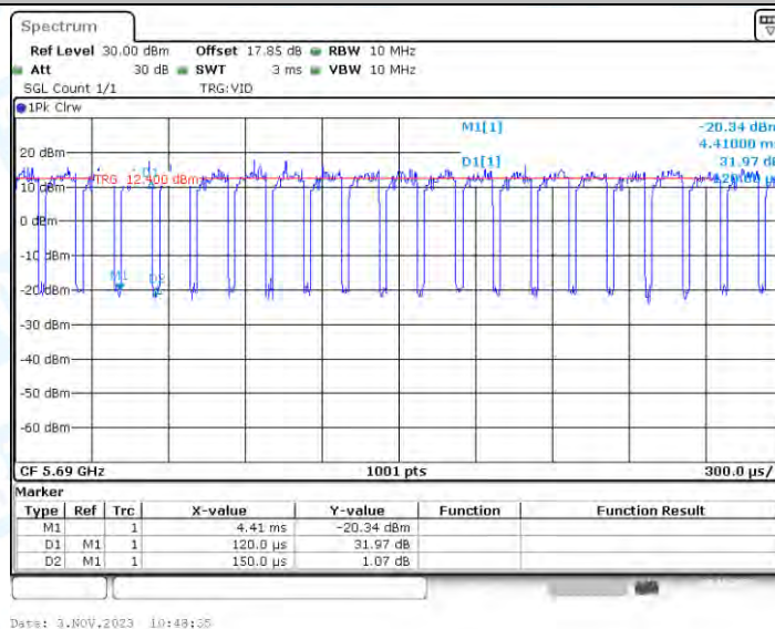
11AC80_Ant4_5690
