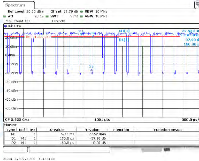
11AC20_Ant2_5825
