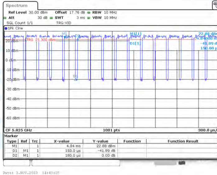
11AC20_Ant3_5825
