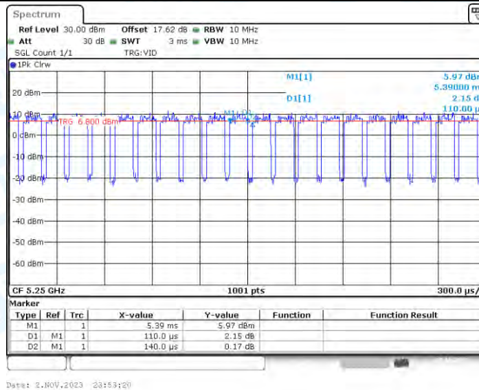
11AC160_Ant4_5250
