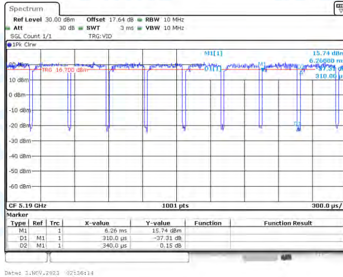
11AX40_Ant3_5190
