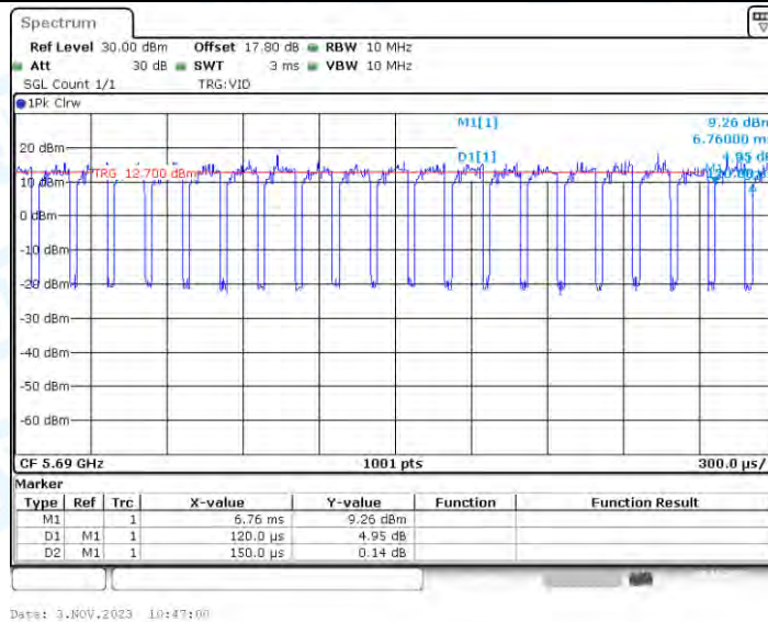
11AC80_Ant3_5690
