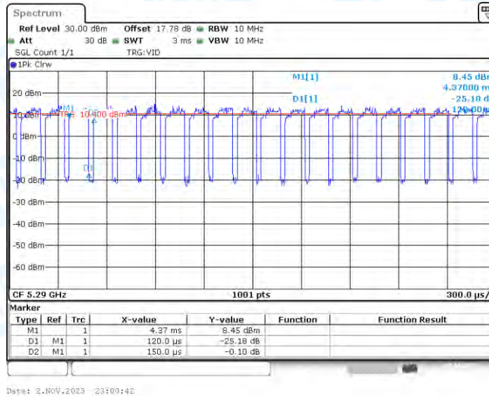
11AC80_Ant4_5290
