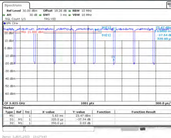
11AX20_Ant3_5825
