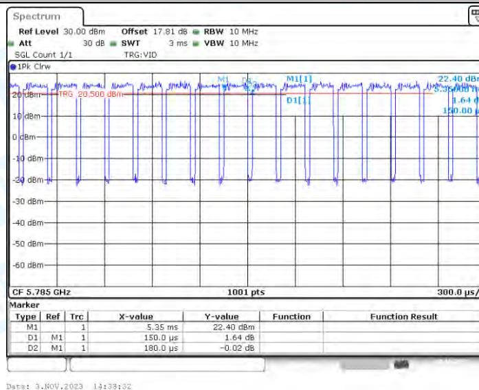
11AC20_Ant2_5785
