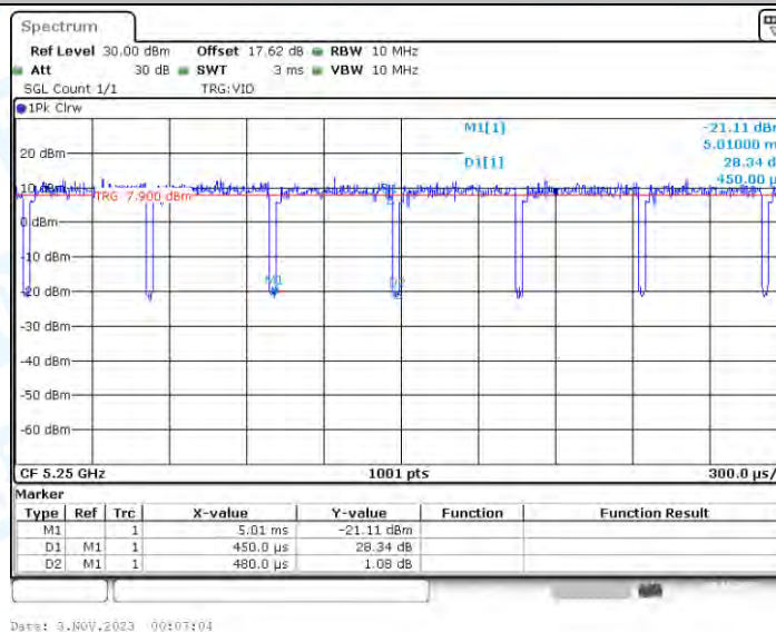
11AX160_Ant4_5250
