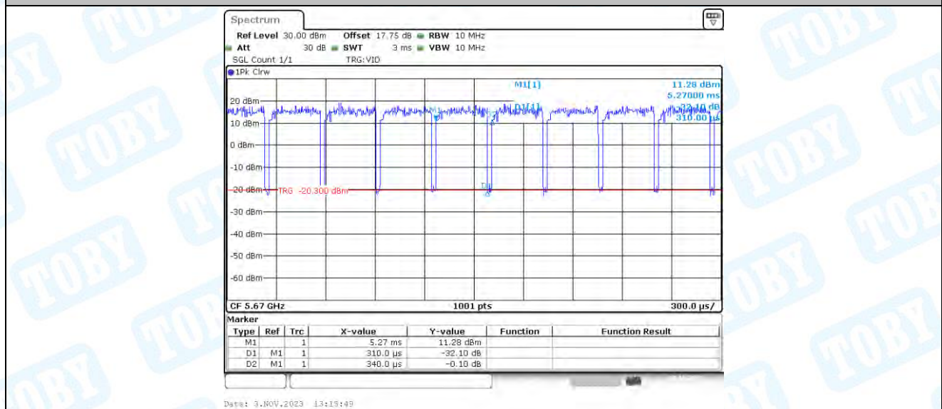
11AX40_Ant2_5670
