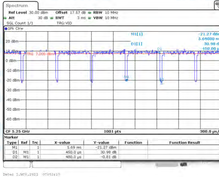
11AX160_Ant2_5250
