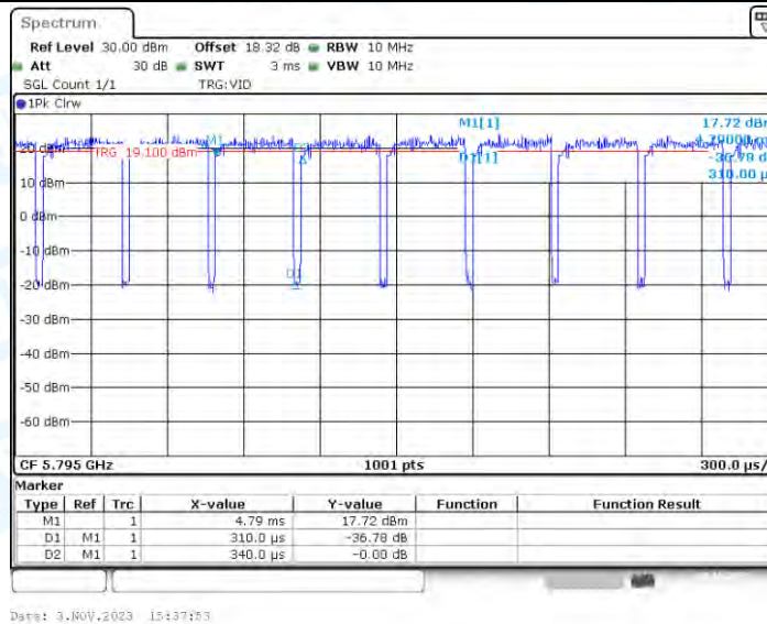
11AX40_Ant4_5795
