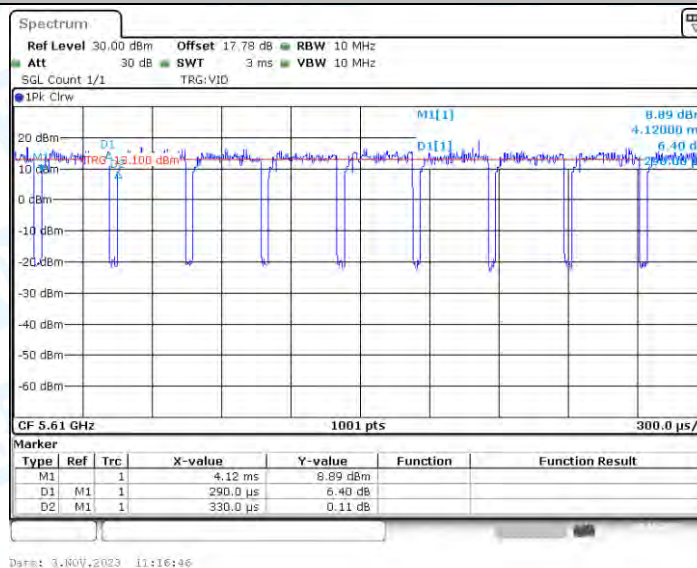
11AX80_Ant4_5610
