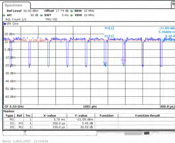
11AX80_Ant4_5530
