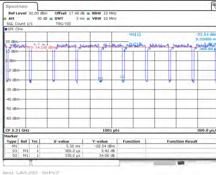
11AX80_Ant3_5210
