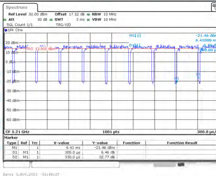
11AX80_Ant4_5210
