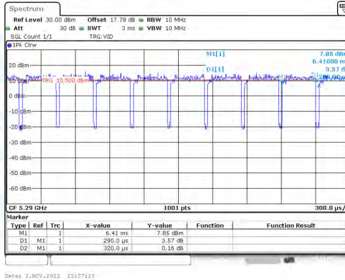
11AX80_Ant4_5290
