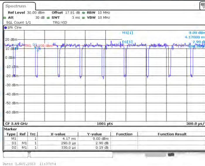
11AX80_Ant2_5690
