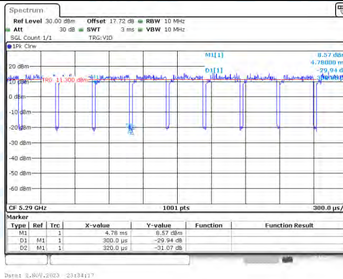
11AX80_Ant2_5290
