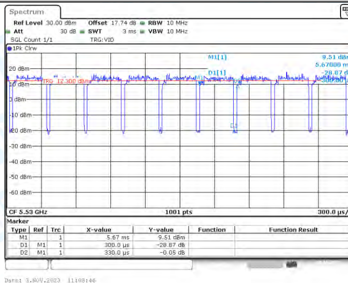
11AX80_Ant2_5530
