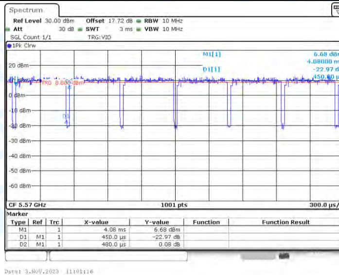
11AX160_Ant2_5570
