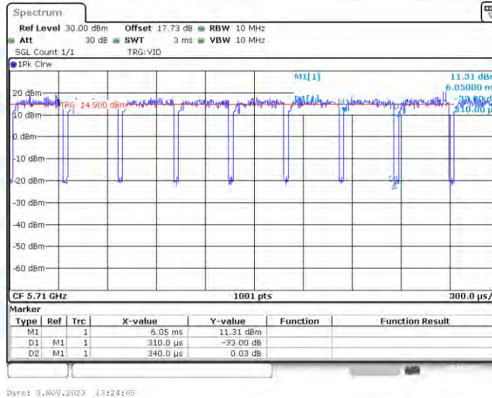
11AX40_Ant3_5710
