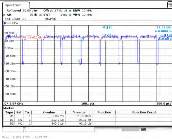
11AX40_Ant4_5670
