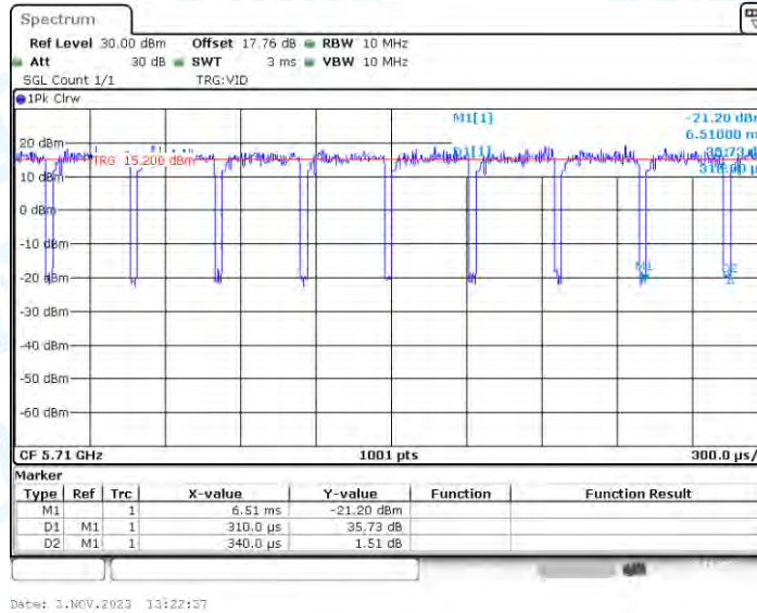
11AX40_Ant2_5710
