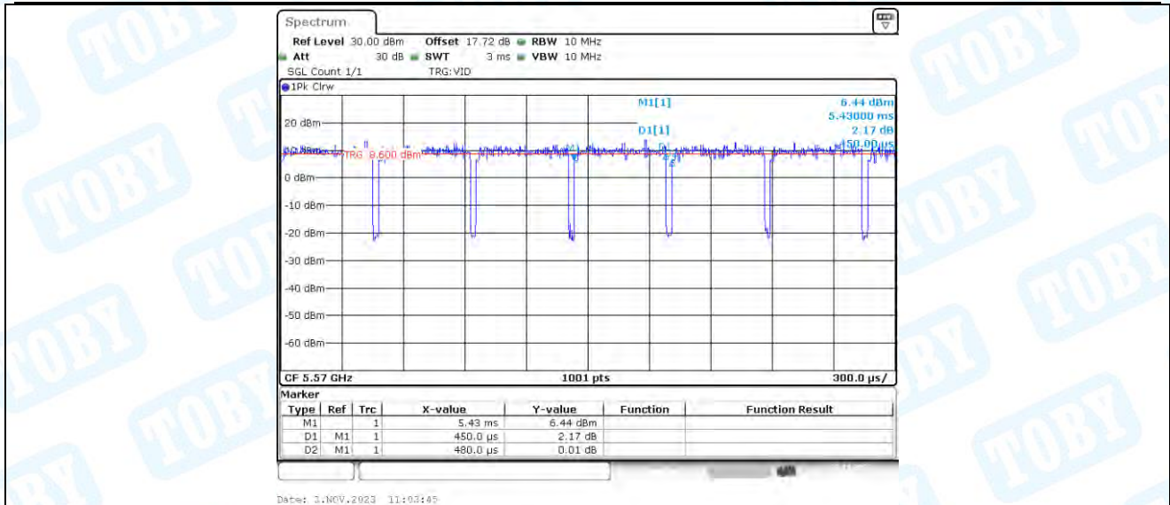
11AX160_Ant4_5570
