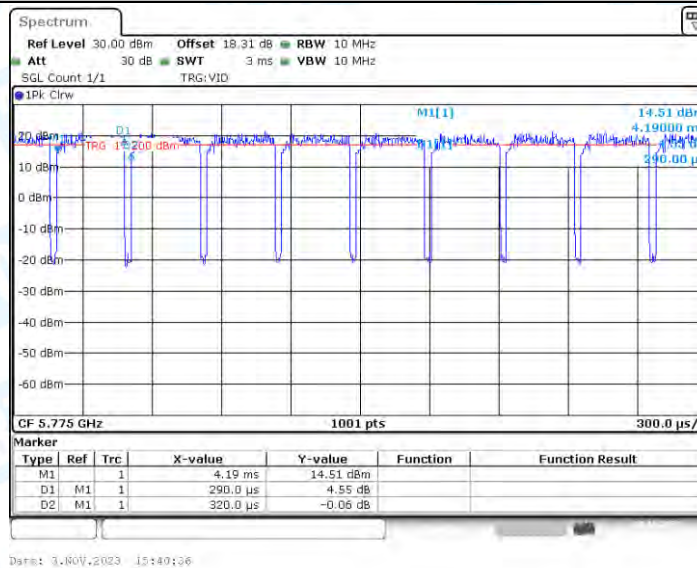
11AX80_Ant2_5775
