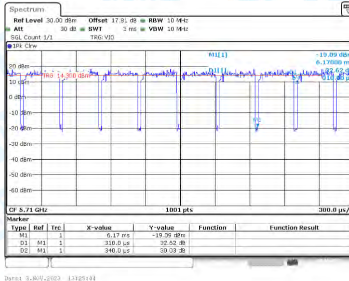
11AX40_Ant4_5710
