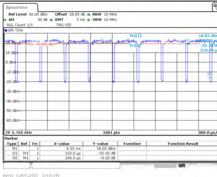
11AX40_Ant3_5755
