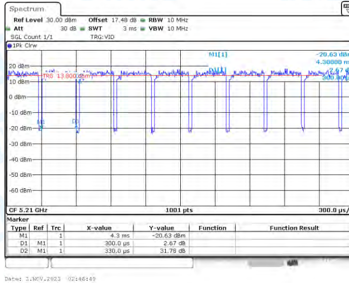
11AX80_Ant2_5210
