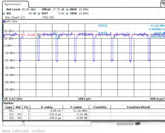
11AX40_Ant3_5670
