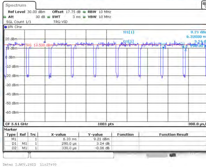
11AX80_Ant2_5610
