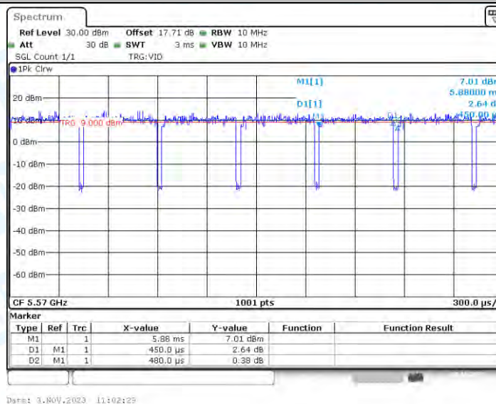
11AX160_Ant3_5570
