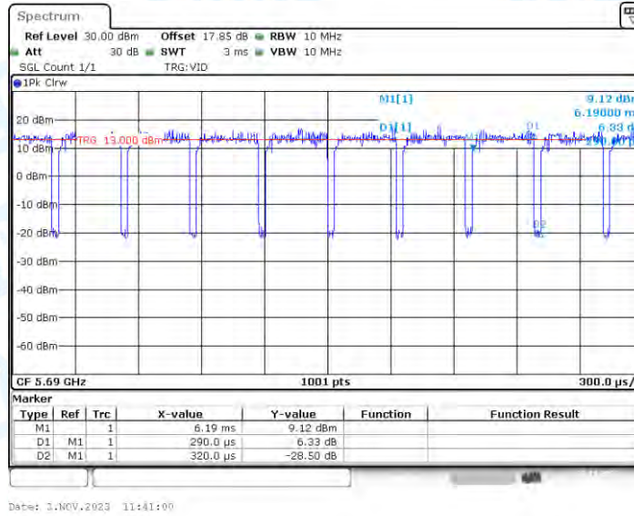
11AX80_Ant4_5690
