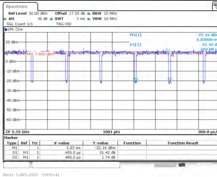
11AX160_Ant3_5250
