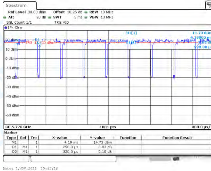
11AX80_Ant3_5775
