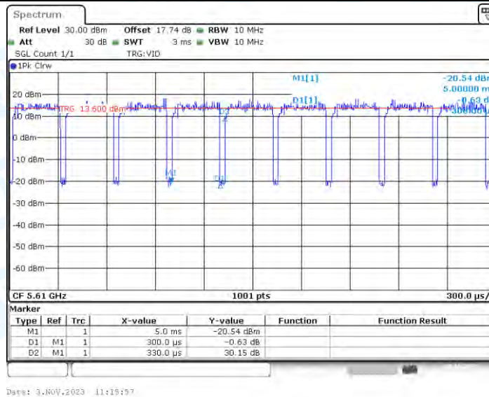
11AX80_Ant3_5610
