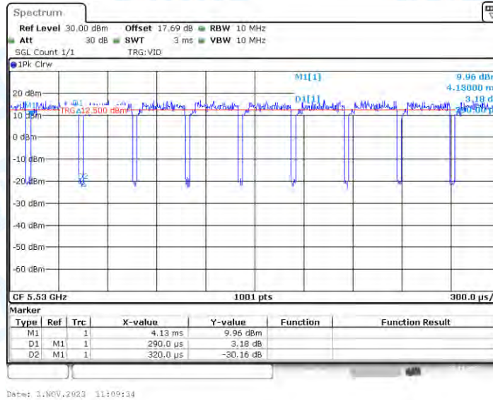
11AX80_Ant3_5530
