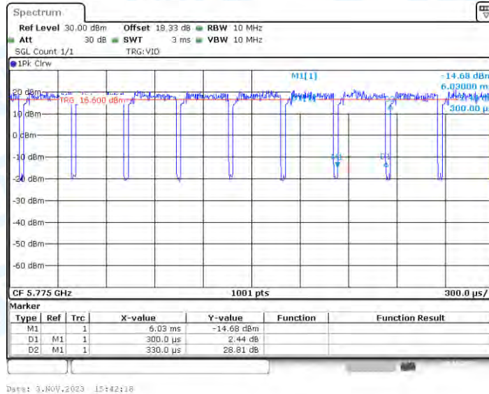
11AX80_Ant4_5775
