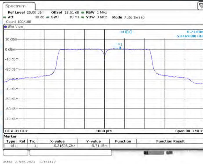
11AC40-CDD_Ant2_5310
