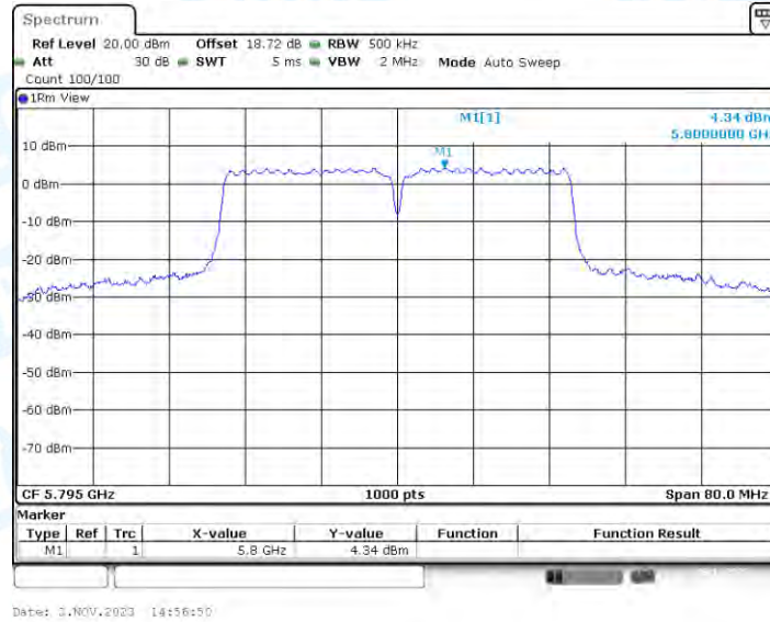
11AC40-CDD_Ant3_5795
