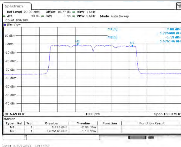
11AC80-CDD_Ant3_5690_UNII-2C
