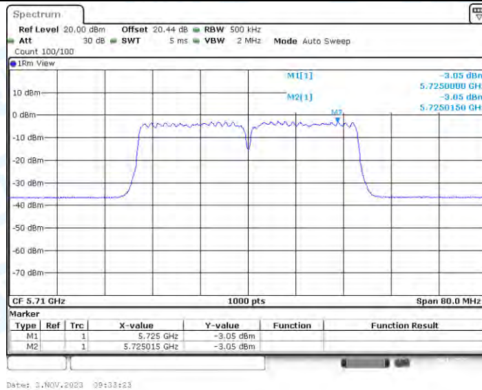
11N40-CDD_Ant4_5710_UNII-3
