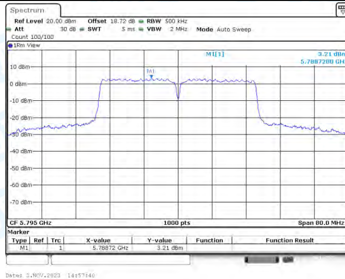
11AC40-CDD_Ant4_5795
