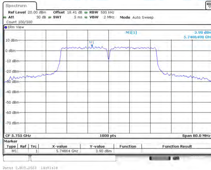
11AC40-CDD_Ant3_5755
