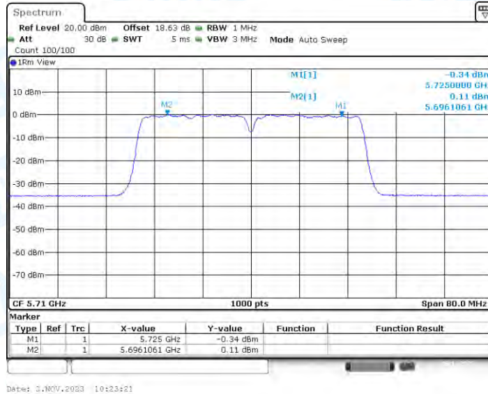
11AC40-CDD_Ant3_5710_UNII-2C
