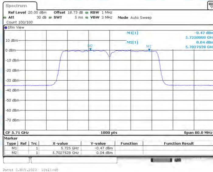
11AC40-CDD_Ant2_5710_UNII-2C
