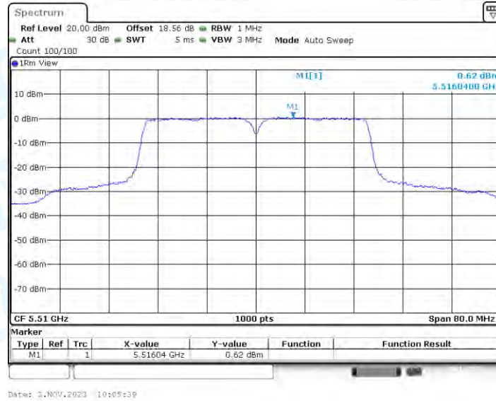
11AC40-CDD_Ant3_5510
