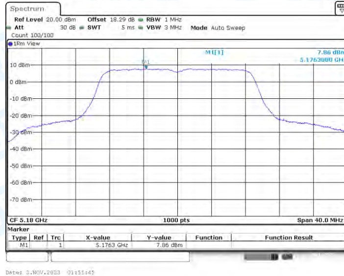
11AC20-CDD_Ant4_5180
