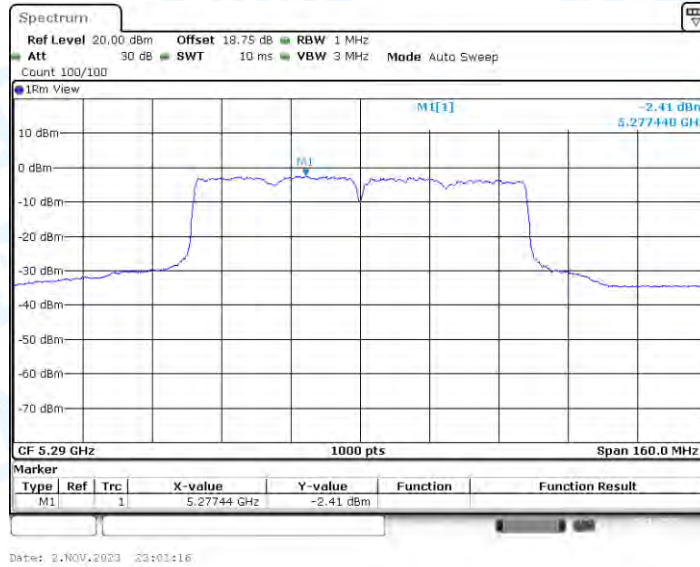
11AC80-CDD_Ant4_5290
