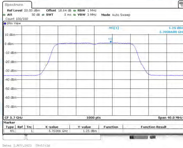
11AC20-CDD_Ant4_5700
