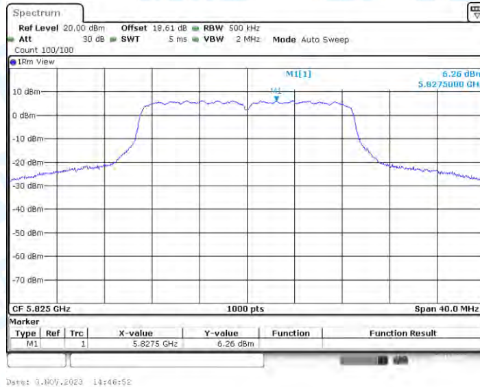
11AC20-CDD_Ant4_5825
