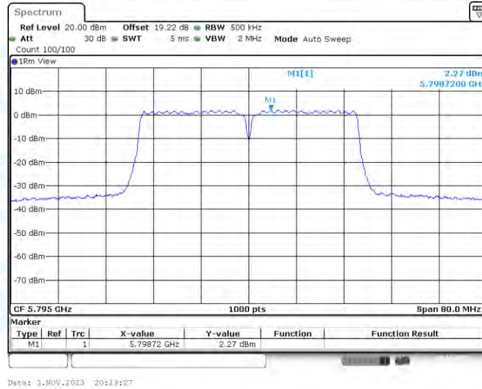
11AC40-BF_Ant3_5795
