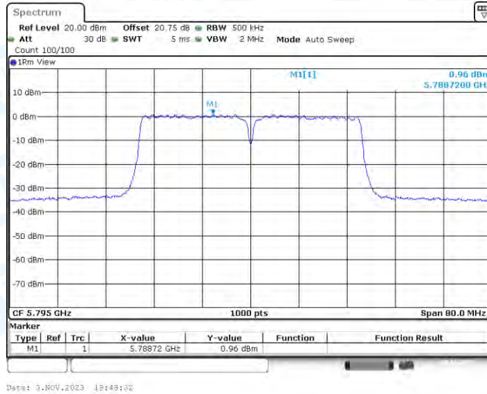
11N40-BF_Ant4_5795
