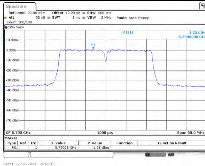
11AC40-BF_Ant4_5795
