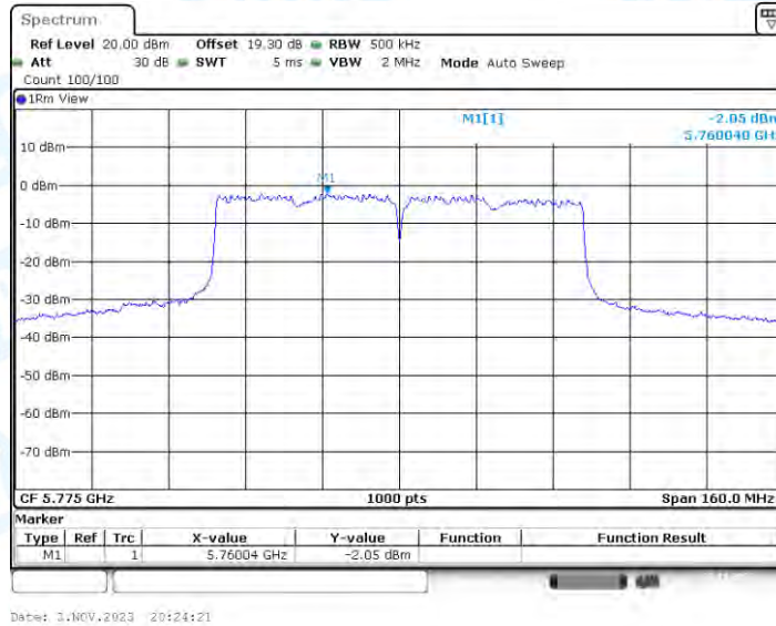
11AC80-BF_Ant4_5775
