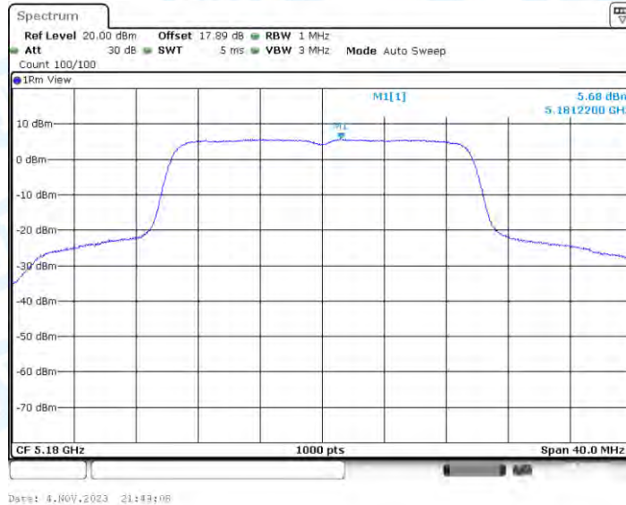
11AX20-BF_Ant4_5180
