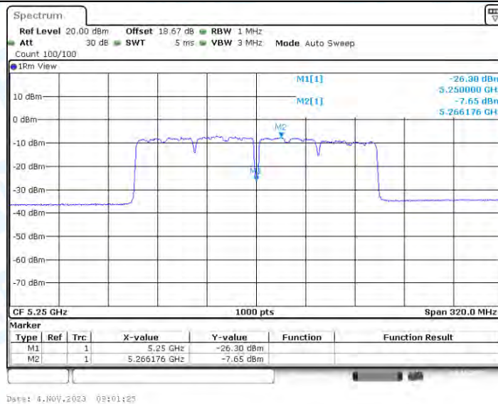
11AC160-BF_Ant4_5250_UNII-2A
