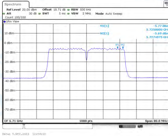
11AC40-BF_Ant4_5710_UNII-3
