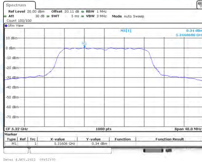
11N20-BF_Ant4_5320
