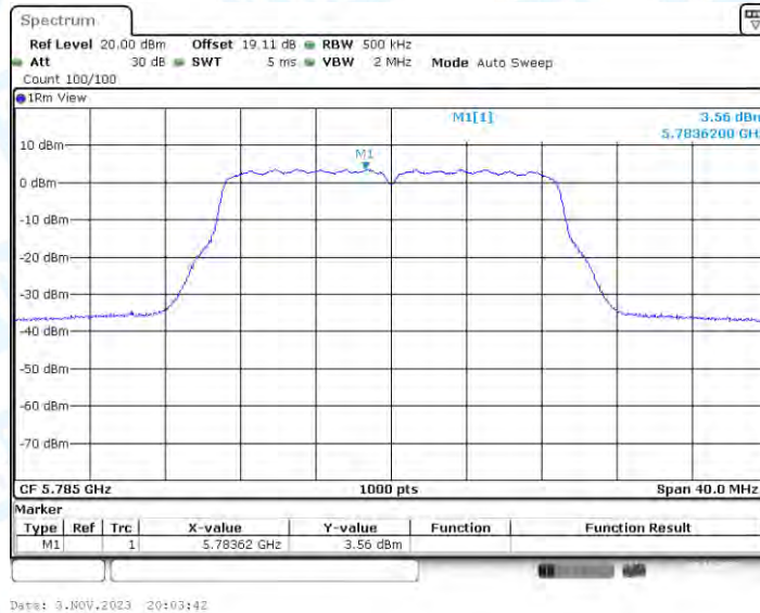
11AC20-BF_Ant4_5785
