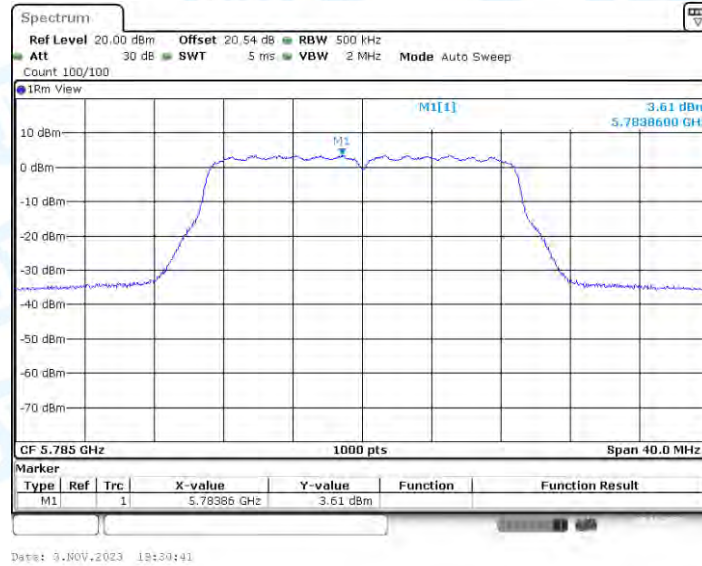
11N20-BF_Ant4_5785
