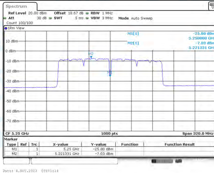
11AC160-BF_Ant4_5250_UNII-1
