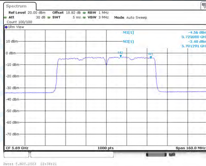
11AC80-BF_Ant4_5690_UNII-2C
