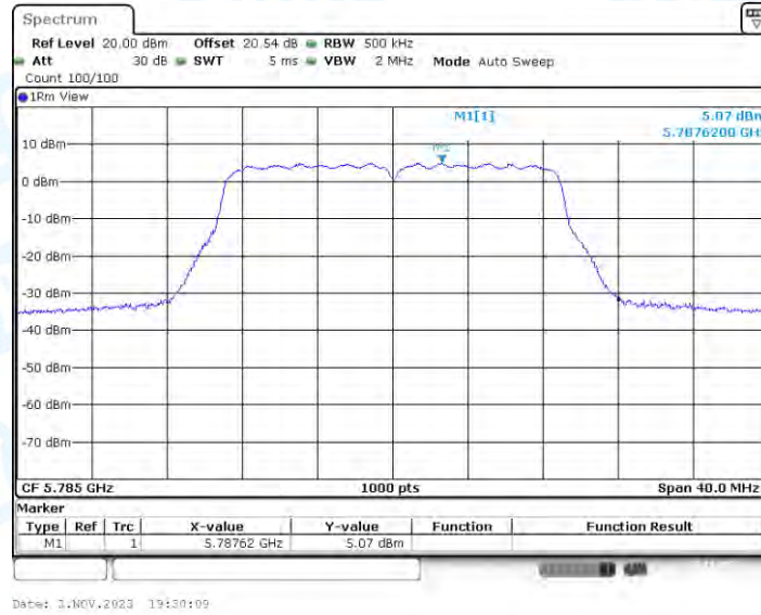
11N20-BF_Ant3_5785
