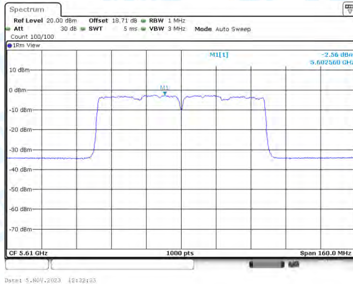
11AC80-BF_Ant3_5610
