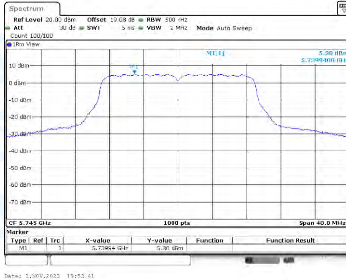
11AC20-BF_Ant3_5745
