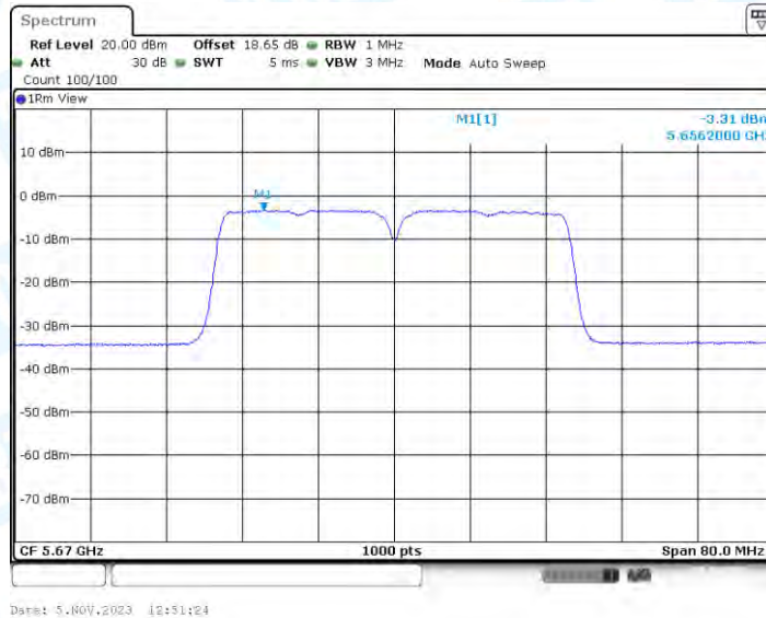
11AC40-BF_Ant2_5670
