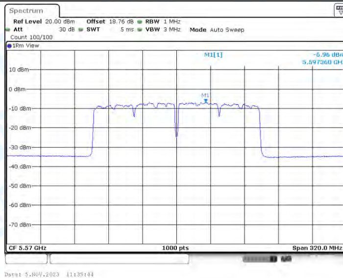
11AC160-BF_Ant3_5570
