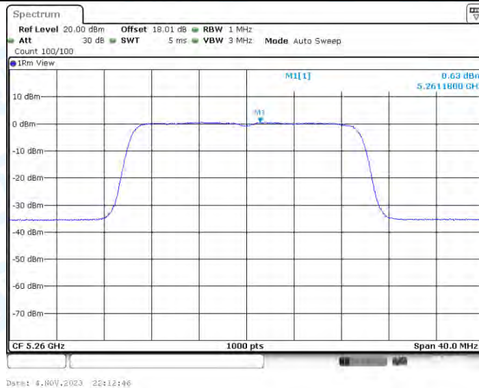
11AX20-BF_Ant4_5260
