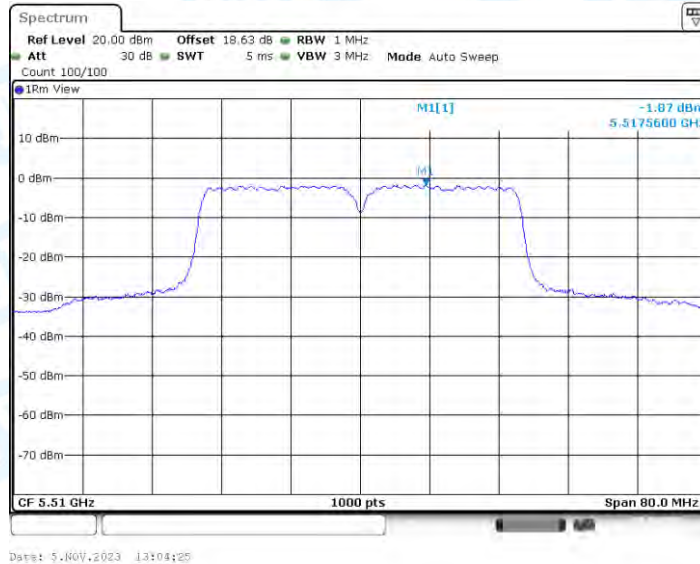
11AC40-BF_Ant3_5510
