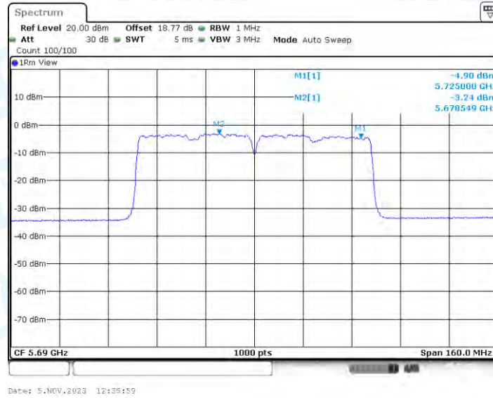
11AC80-BF_Ant3_5690_UNII-2C
