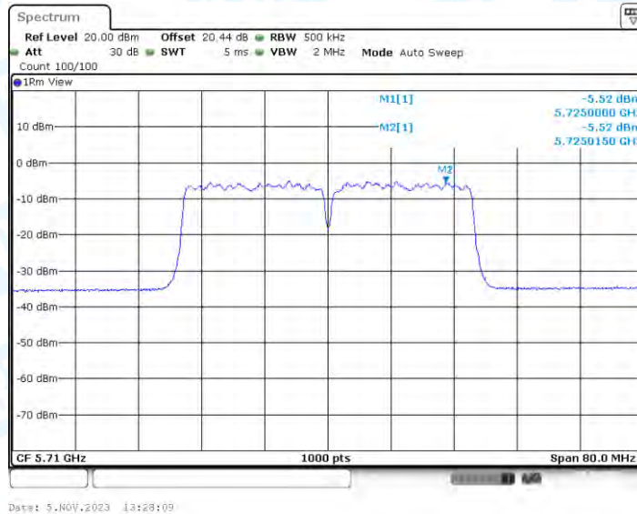
11N40-BF_Ant4_5710_UNII-3
