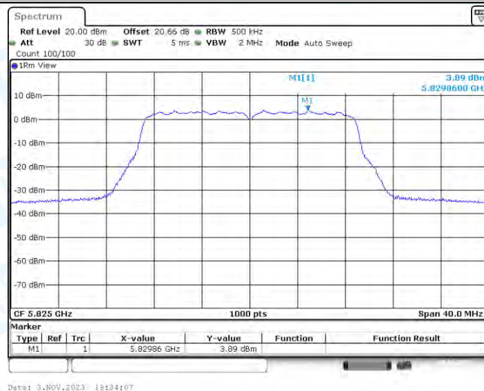
11N20-BF_Ant4_5825
