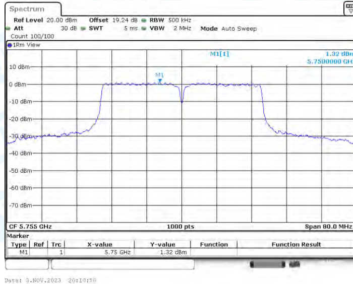
11AC40-BF_Ant4_5755
