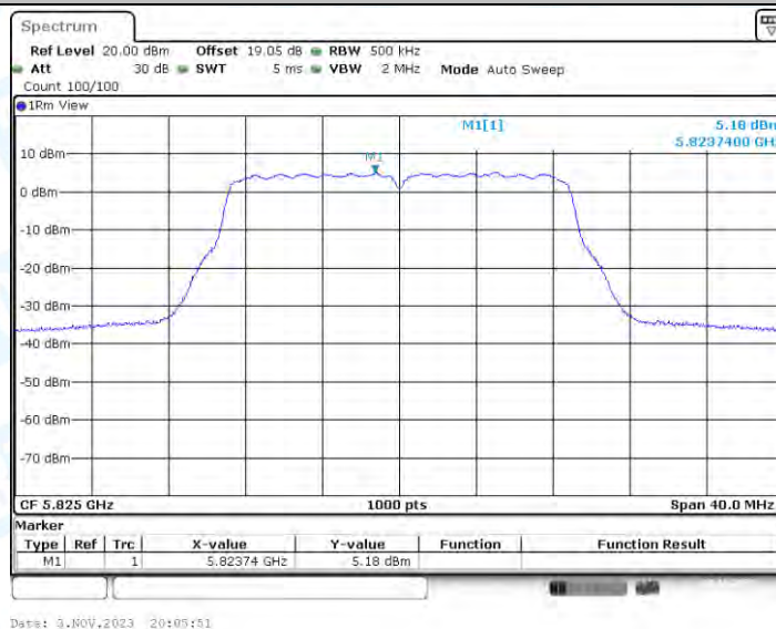
11AC20-BF_Ant3_5825
