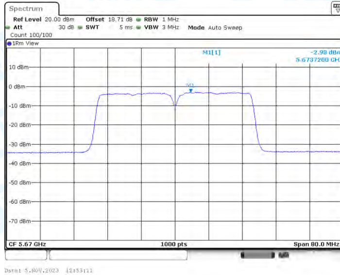
11AC40-BF_Ant4_5670
