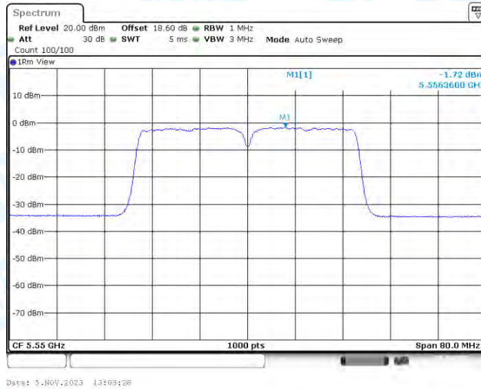
11AC40-BF_Ant3_5550
