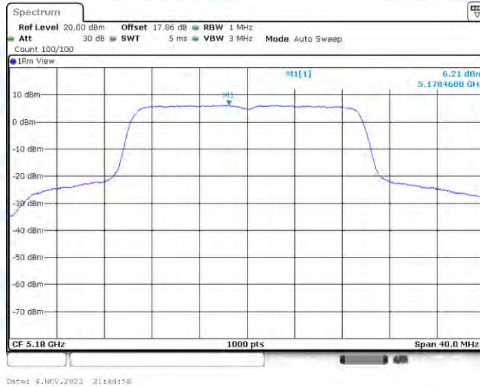
11AX20-BF_Ant3_5180
