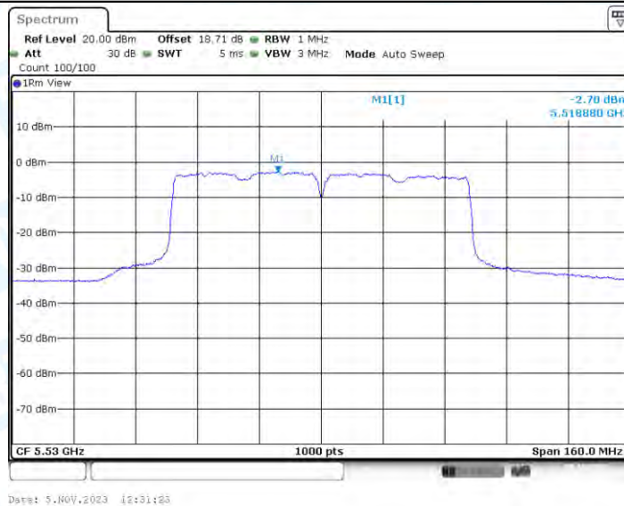
11AC80-BF_Ant4_5530
