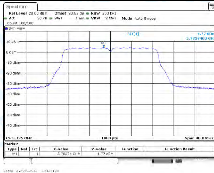
11N20-BF_Ant2_5785
