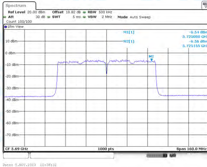
11AC80-BF_Ant4_5690_UNII-3
