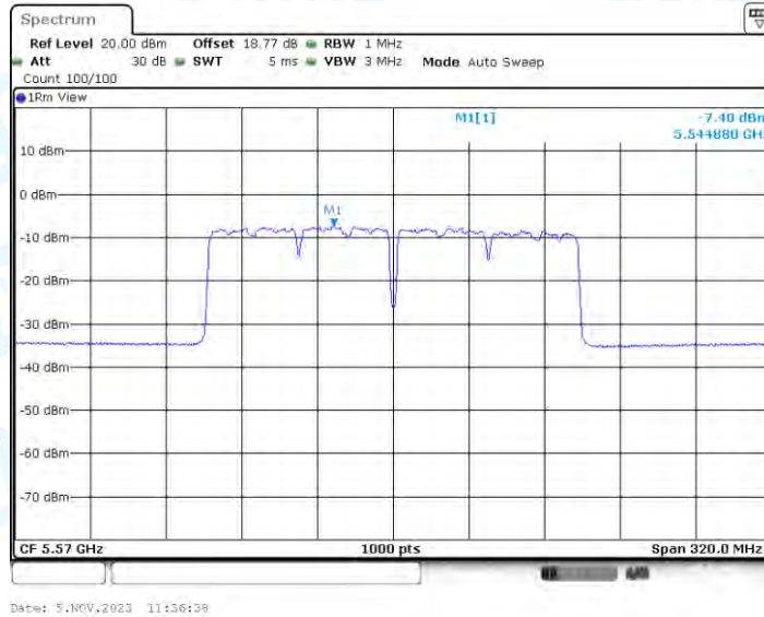
11AC160-BF_Ant4_5570
