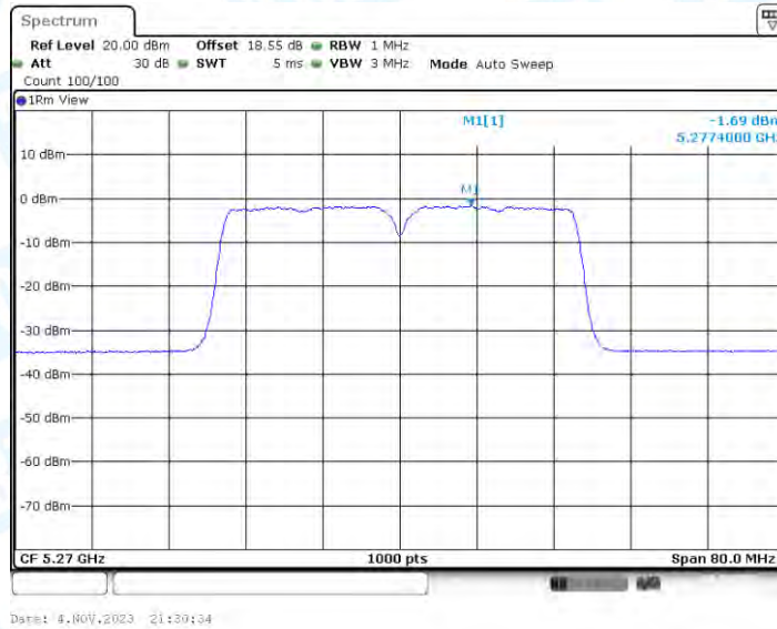
11AC40-BF_Ant3_5270
