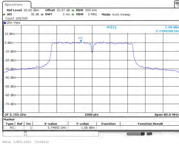
11N40-BF_Ant4_5755
