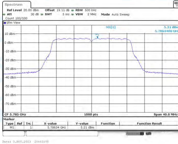
11AC20-BF_Ant3_5785
