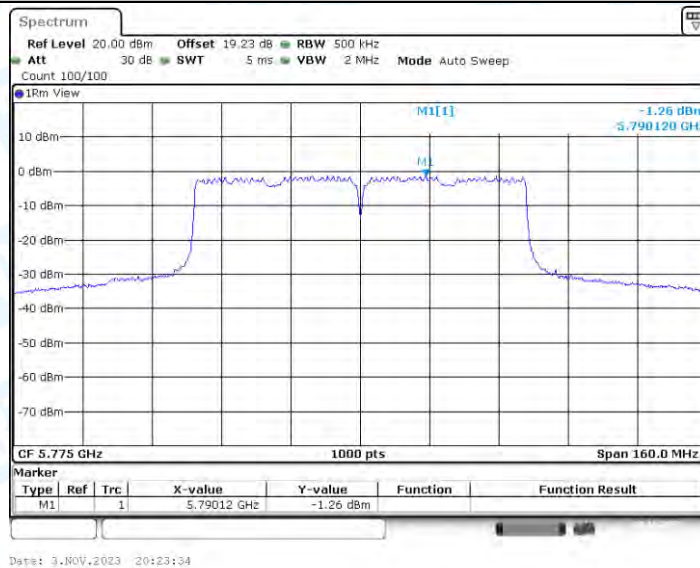
11AC80-BF_Ant3_5775
