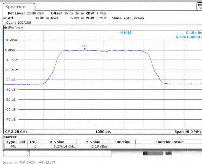
11N20-BF_Ant4_5280
