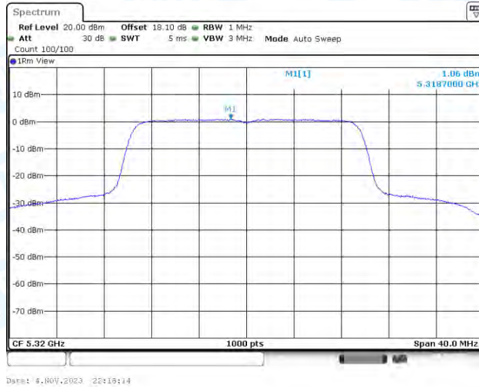
11AX20-BF_Ant2_5320
