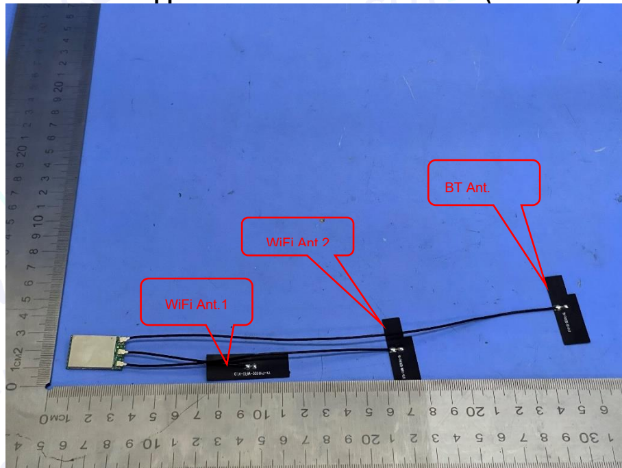
Photo 2 Appearance of EUT with Antenna(XINGHE)
