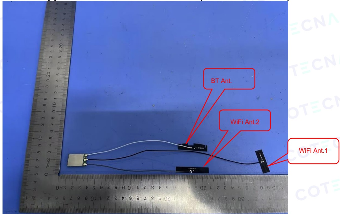
Photo 2 Appearance of EUT with Antenna(XINGHE)
