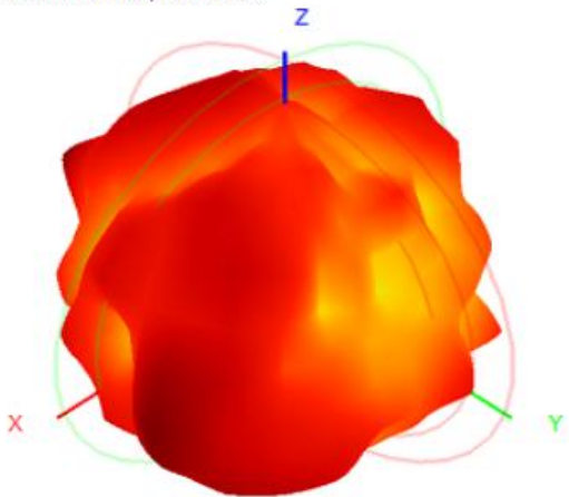
5350.0MHz H+V, Eff. 52.6%
