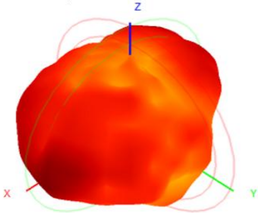
2460.0MHz H+V, Eff. 50.8%
