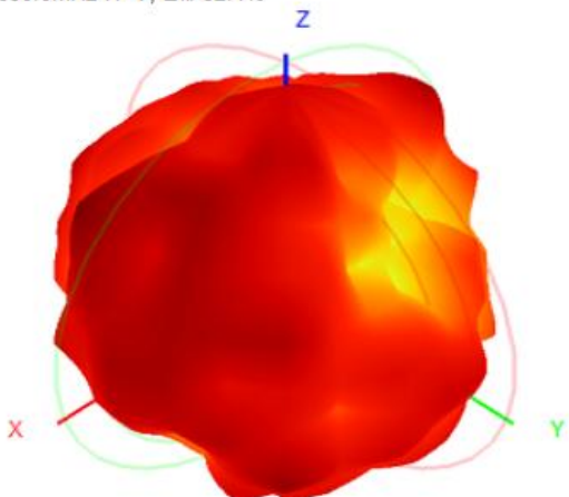
5850.0MHz H+V, Eff. 52.4%
