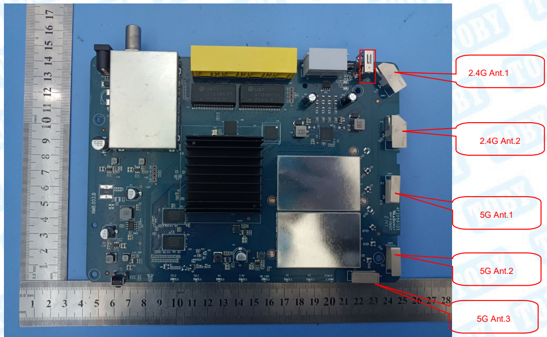
Photo 13 Appearance of PCB without USB
