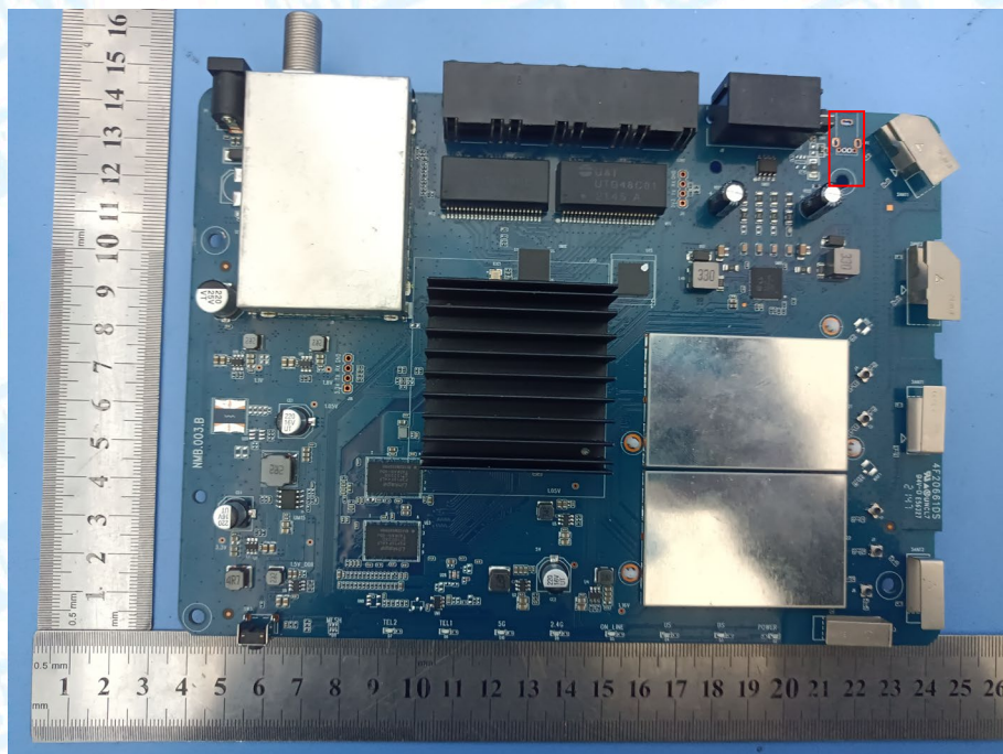
Photo 13 Appearance of PCB without USB
