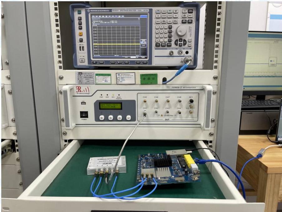
Photo of Setup for DFS Test
