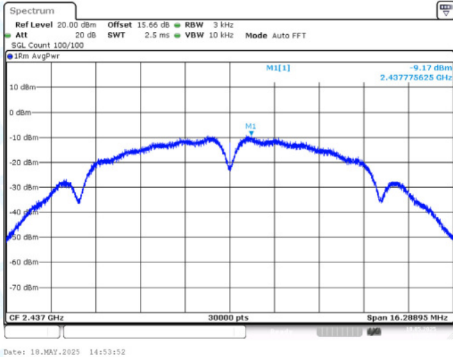
11B-Ant1-2437-PASS
