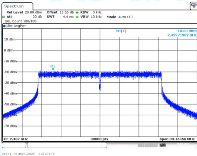
11AX20-CDD-Ant1-2437-PASS
