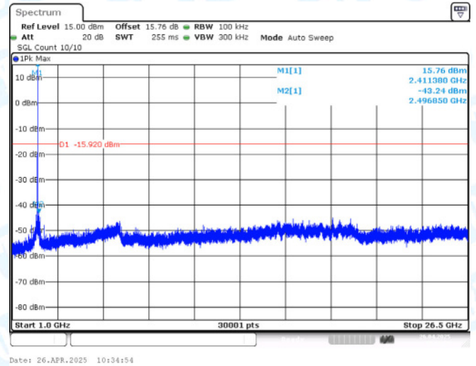
11B-Ant2-2412-1000~26500-PASS
