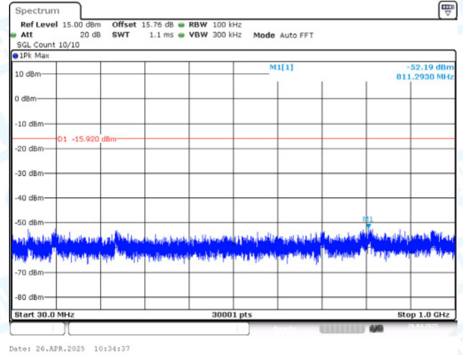
11B-Ant2-2412-30~1000-PASS
