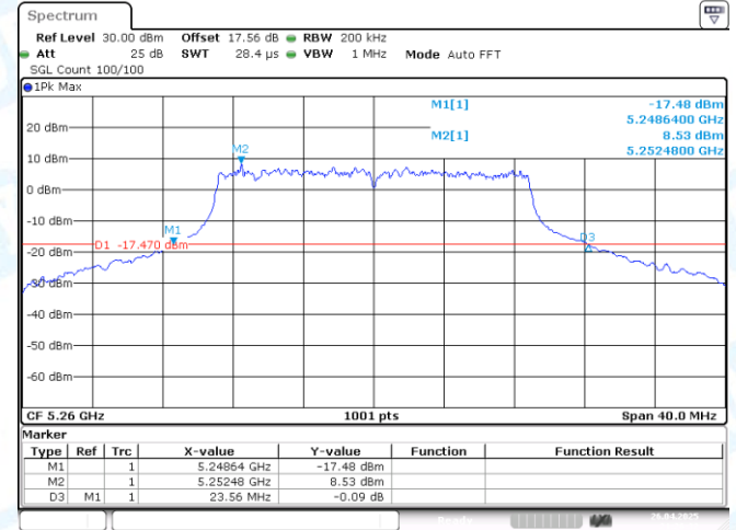
11N20-CDD-Ant2-5260
