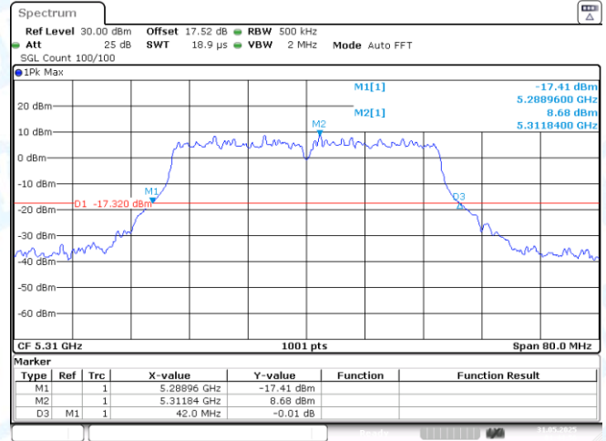
11N40-CDD-Ant2-5310
