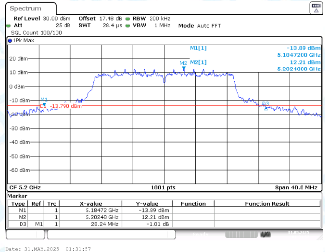
11N20-CDD-Ant2-5200
