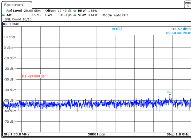
11AC40-CDD-Ant1-5310-30~1000-PASS
