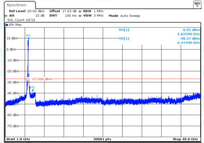
11AC160-CDD-Ant2-5570-1000~40000-PASS
