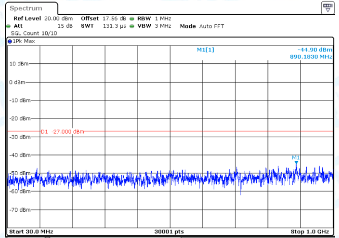
11AC160-CDD-Ant2-5250-30~1000-PASS
