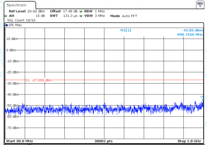
11AX20-CDD-Ant2-5200-30~1000-PASS
