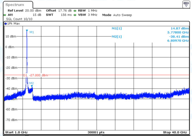
11AX80-CDD-Ant2-5775-1000~40000-PASS
