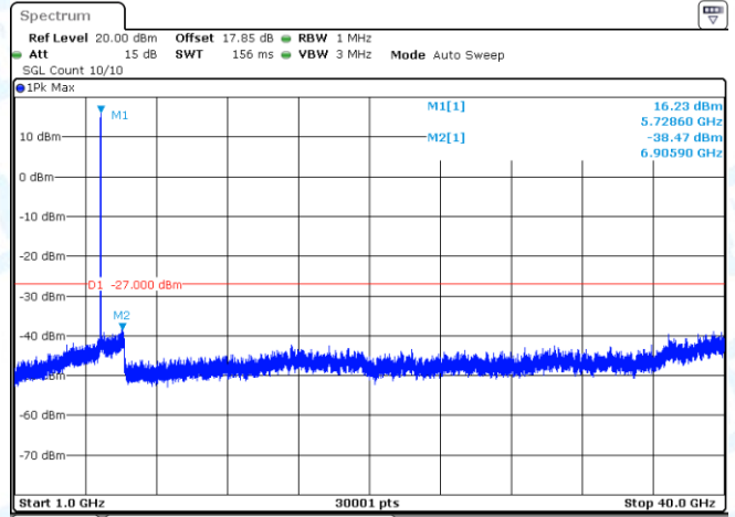
11AX20-CDD-Ant2-5720-1000~40000-PASS
