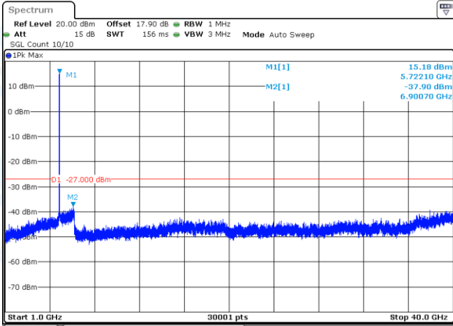
11AX20-CDD-Ant1-5720-1000~40000-PASS
