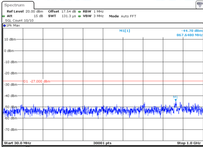
11AX40-CDD-Ant1-5510-30~1000-PASS
