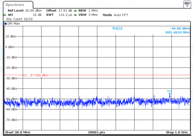
11AX40-CDD-Ant2-5510-30~1000-PASS
