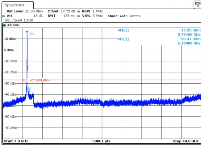
11AX80-CDD-Ant1-5775-1000~40000-PASS
