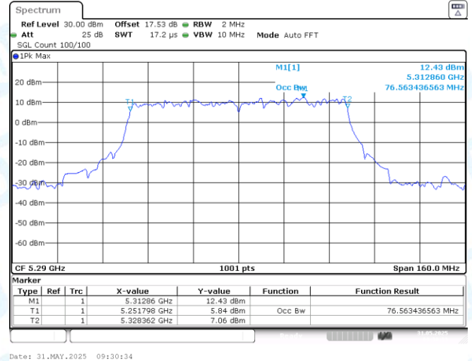
11AC80-CDD-Ant2-5290
