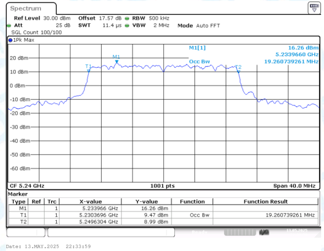
11AX20-CDD-Ant2-5240
