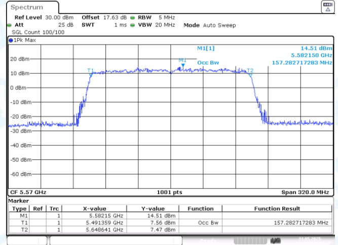
11AX160-CDD-Ant2-5570
