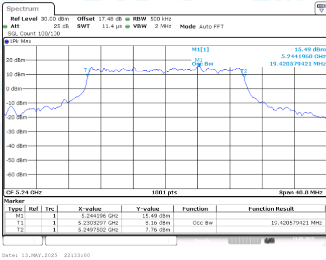
11AX20-CDD-Ant1-5240
