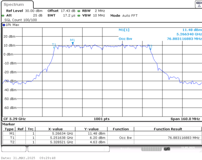
11AC80-CDD-Ant1-5290
