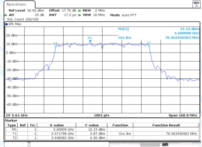
11AC80-CDD-Ant2-5610
