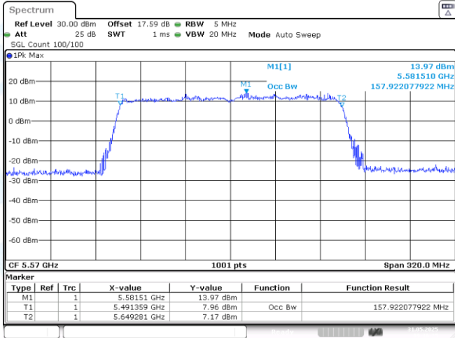
11AX160-CDD-Ant1-5570
