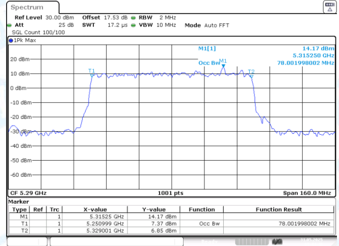
11AX80-CDD-Ant2-5290
