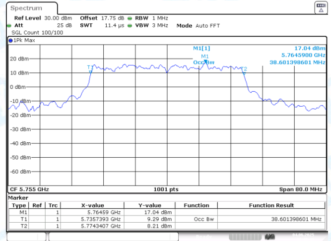
11AX40-CDD-Ant2-5755
