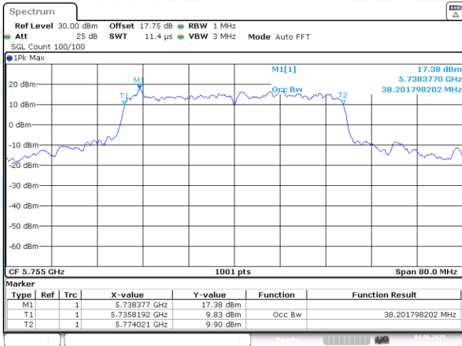
11AX40-CDD-Ant1-5755
