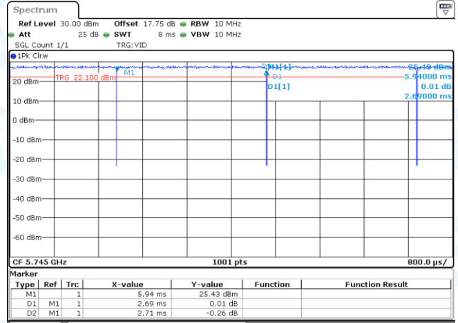
NTNV-11A-Ant2-5745
