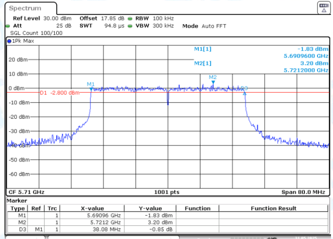
11AX40-CDD-Ant2-5710
