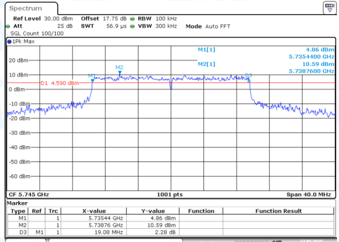
11AX20-CDD-Ant2-5745-PASS
