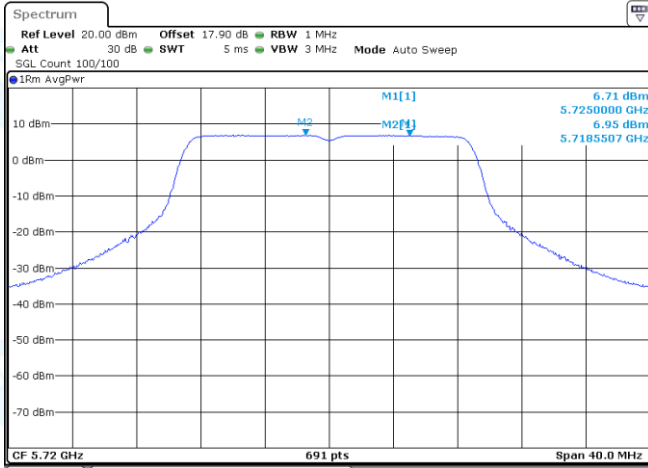
11N20-CDD-Ant1-5720_UNII-2C-PASS
