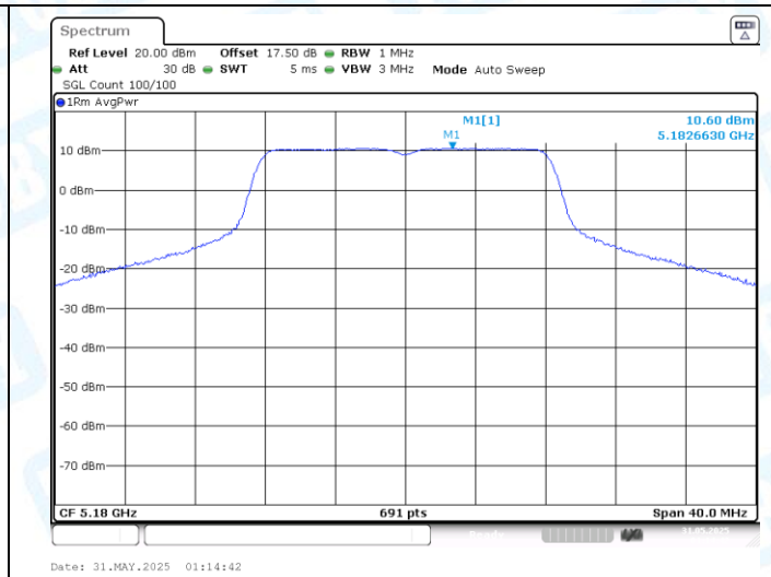
11A-Ant2-5180-PASS
