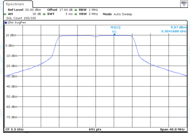
11A-Ant2-5500-PASS
