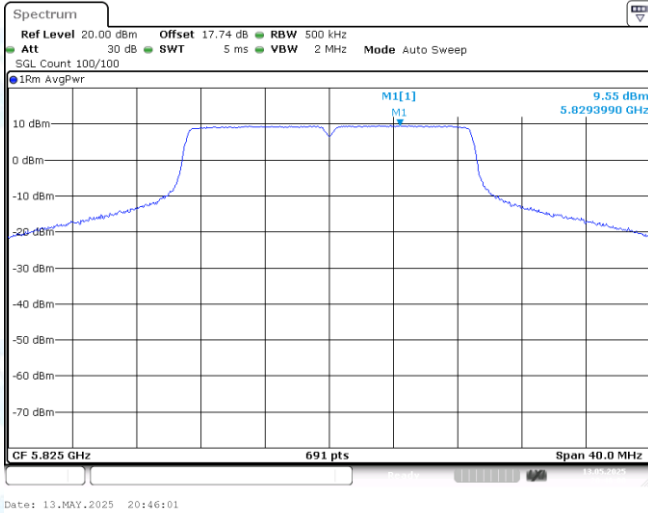
11AC20-CDD-Ant1-5825-PASS
