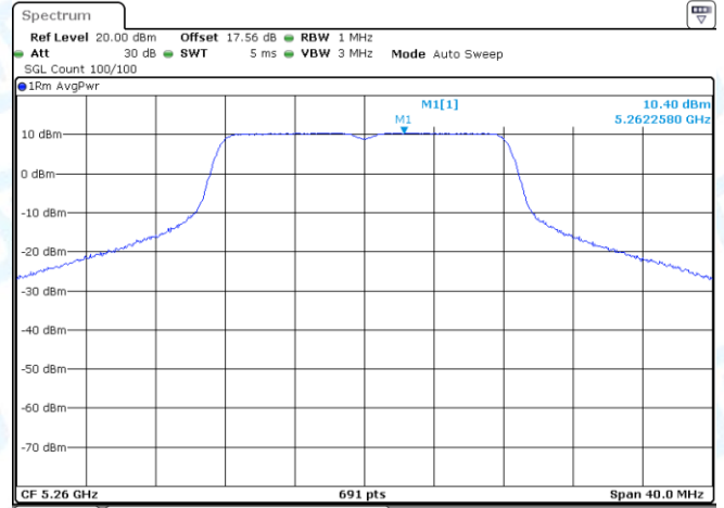
11A-Ant2-5260-PASS
