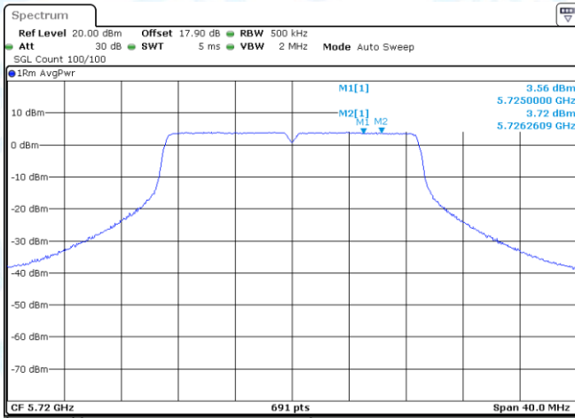
11N20-CDD-Ant1-5720_UNII-2C-PASS
