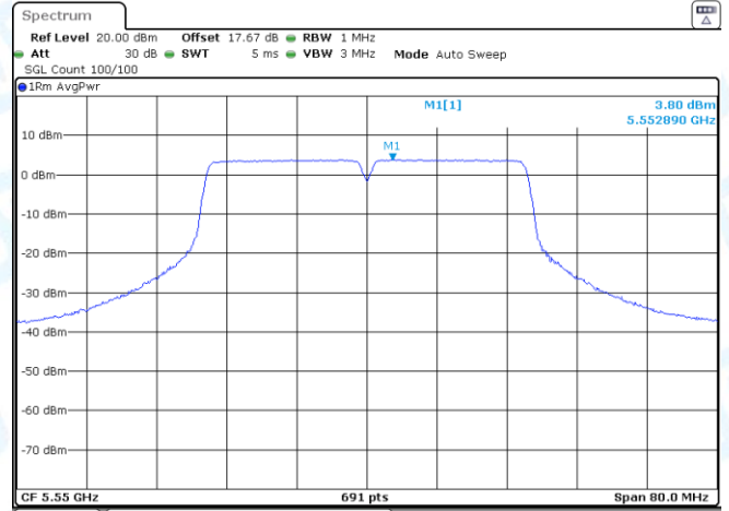
11AC40-CDD-Ant2-5550-PASS
