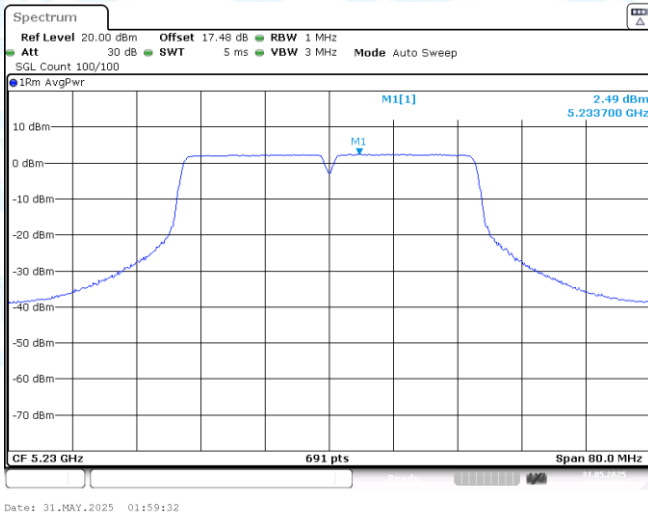
11AC40-CDD-Ant1-5230-PASS
