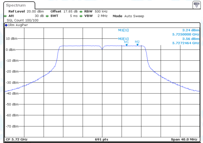
11N20-CDD-Ant2-5720_UNII-2C-PASS
