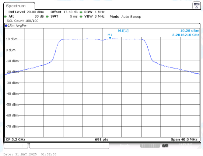
11N20-CDD-Ant2-5200-PASS
