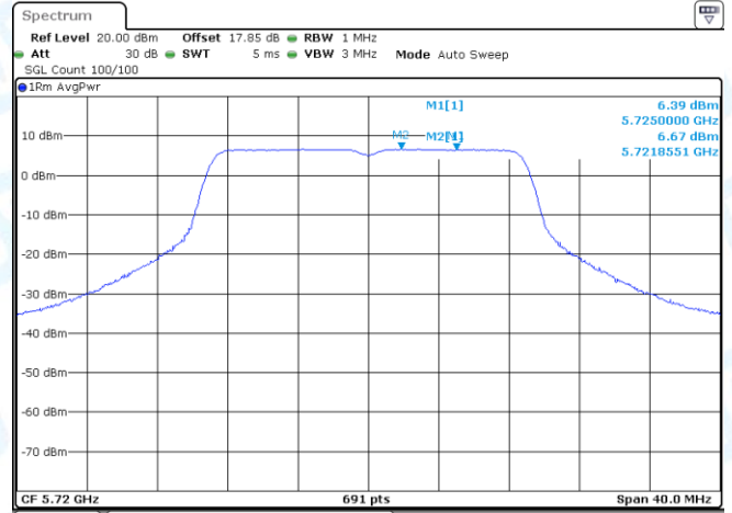
11N20-CDD-Ant2-5720_UNII-2C-PASS
