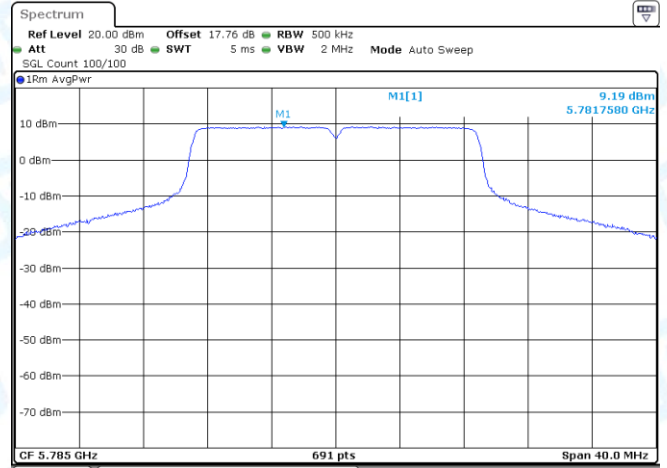
11N20-CDD-Ant2-5785-PASS
