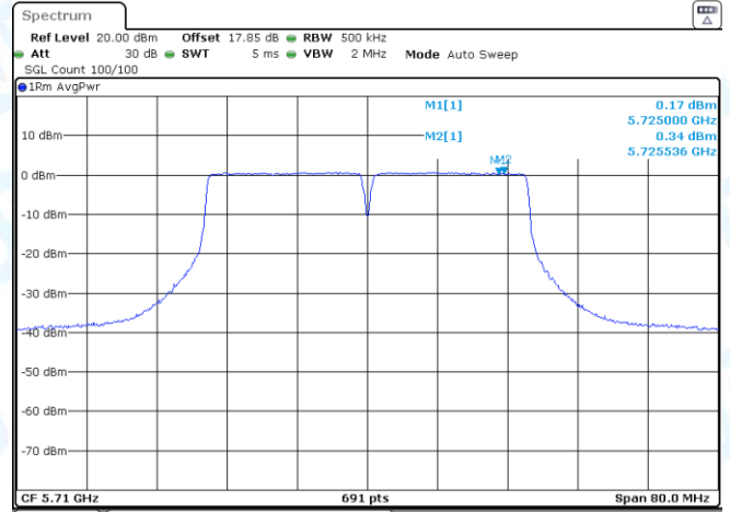
11N40-CDD-Ant2-5710_UNII-3-PASS
