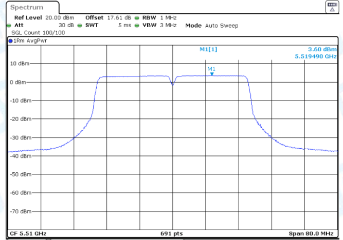
11N40-CDD-Ant2-5510-PASS
