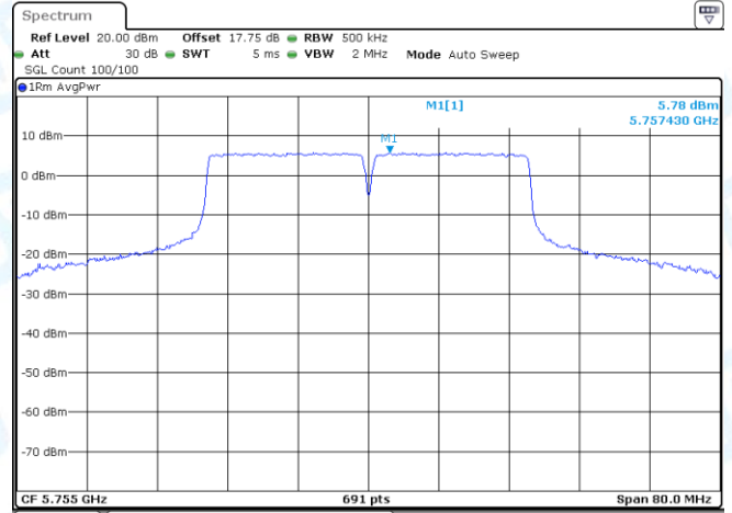
11AC40-CDD-Ant2-5755-PASS
