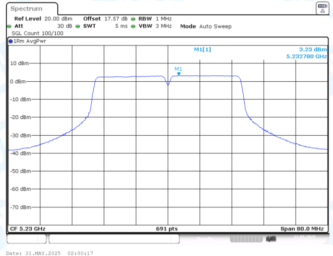
11AC40-CDD-Ant2-5230-PASS
