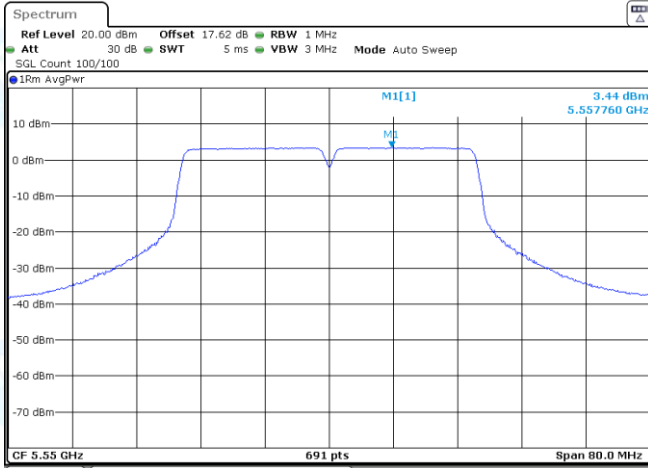
11AC40-CDD-Ant1-5550-PASS
