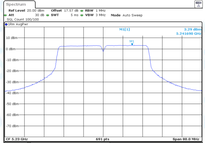
11N40-CDD-Ant2-5230-PASS
