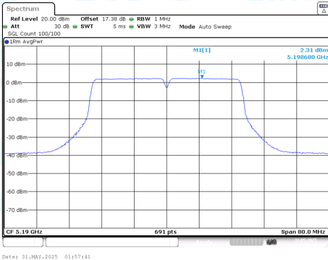
11AC40-CDD-Ant1-5190-PASS
