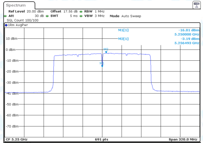
11AX160-CDD-Ant2-5250_UNII-1-PASS
