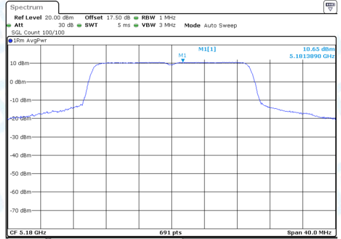
11AX20-CDD-Ant2-5180-PASS
