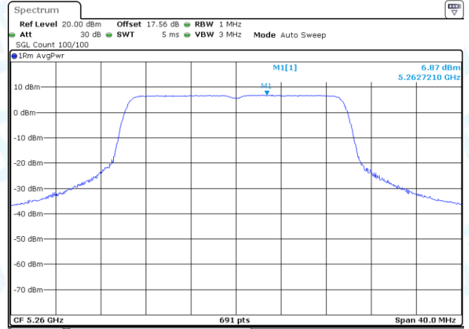
11AX20-CDD-Ant2-5260-PASS
