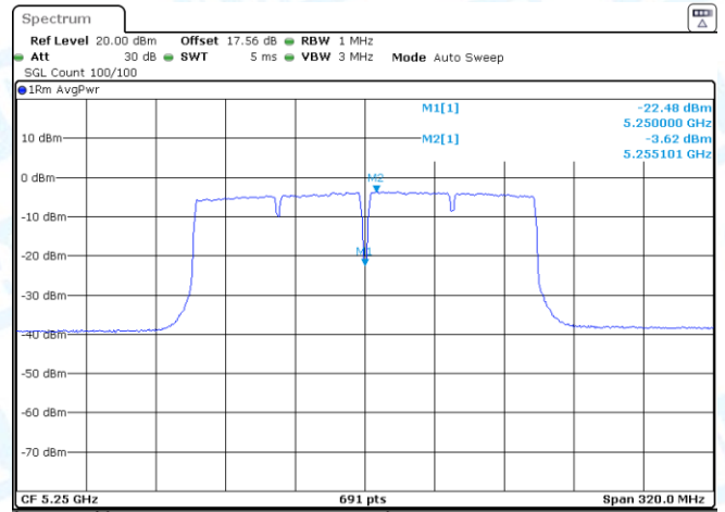
11AC160-CDD-Ant2-5250_UNII-1-PASS
