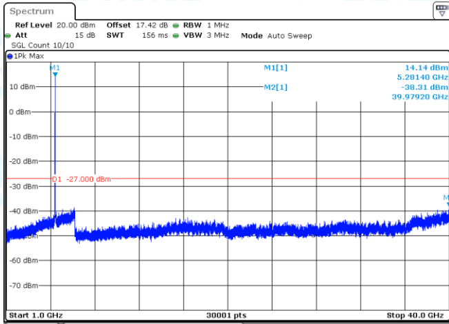
11N20-CDD-Ant1-5280-1000~40000-PASS
