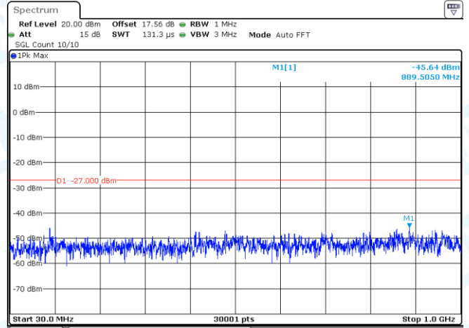
11N20-CDD-Ant2-5260-30~1000-PASS
