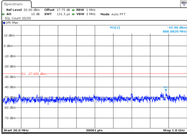
11N20-CDD-Ant1-5745-30~1000-PASS
