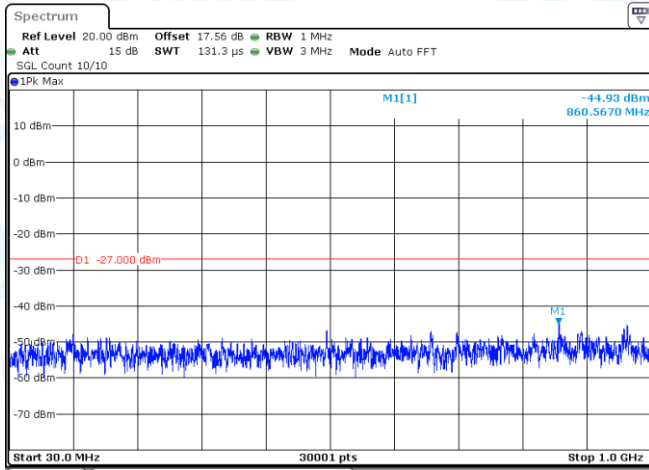
11N20-CDD-Ant1-5500-30~1000-PASS
