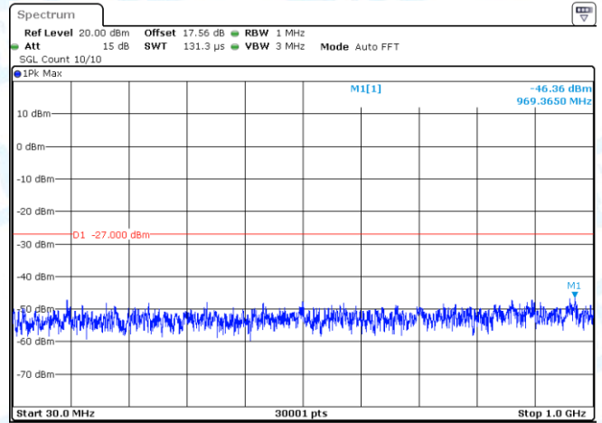
11A-Ant2-5260-30~1000-PASS
