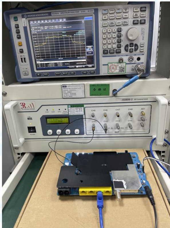
Photo of Setup for RF Conducted Measurements
