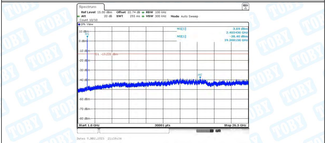
11G_Ant4_2412_0~Reference
