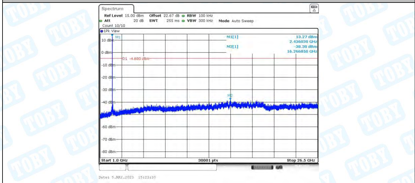
11B_Ant3_2437_0~Reference
