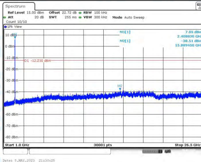
11G_Ant3_2412_0~Reference
