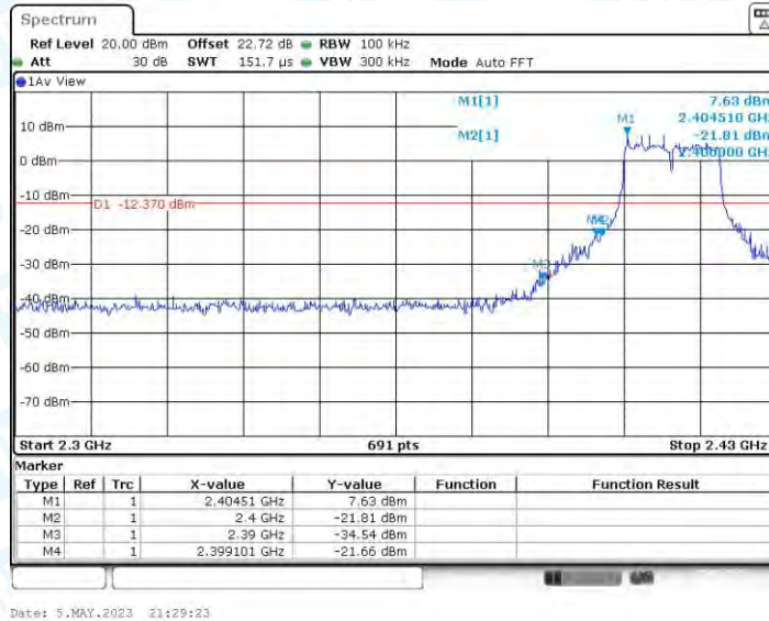
11G_Ant3_Low_2412
