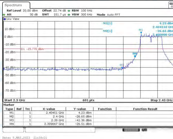
11G_Ant4_Low_2412
