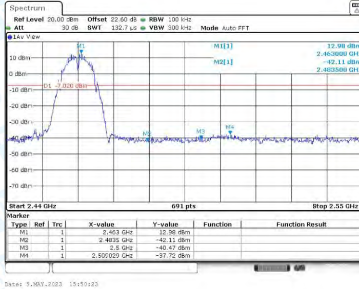
11B_Ant4_High_2462
