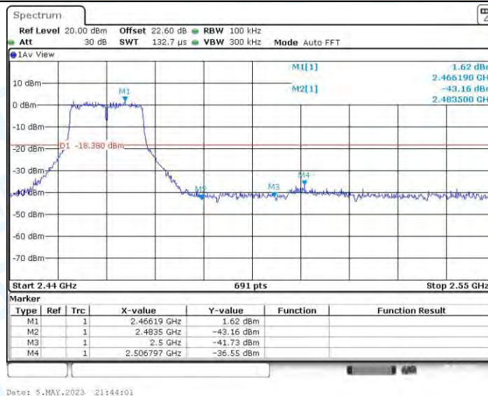
11G_Ant4_High_2462
