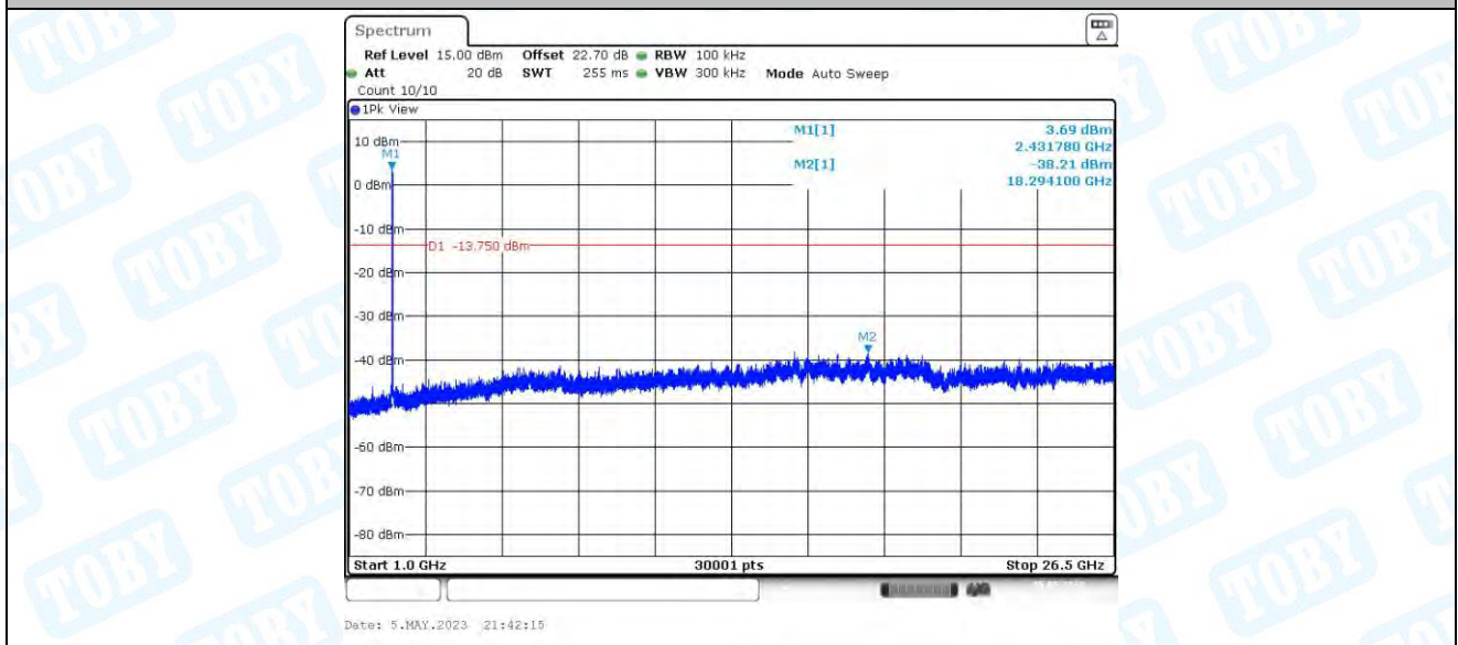
11G_Ant4_2437_0~Reference
