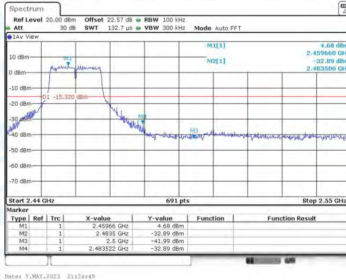
11G_Ant3_High_2462
