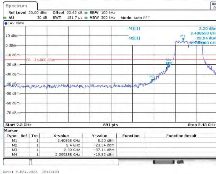
11G_Ant2_Low_2412
