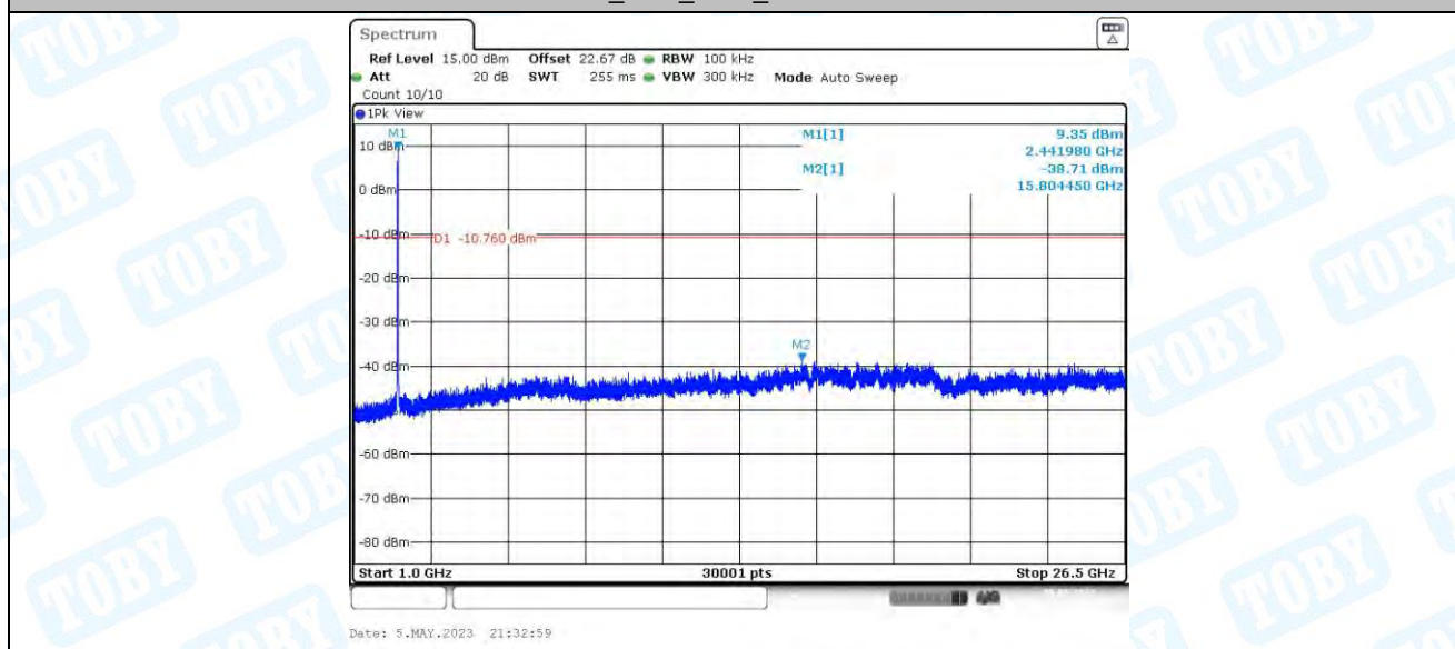
11G_Ant3_2437_0~Reference
