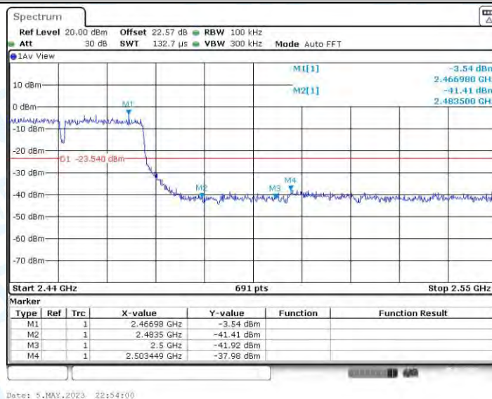
11N40MIMO_Ant3_High_2452
