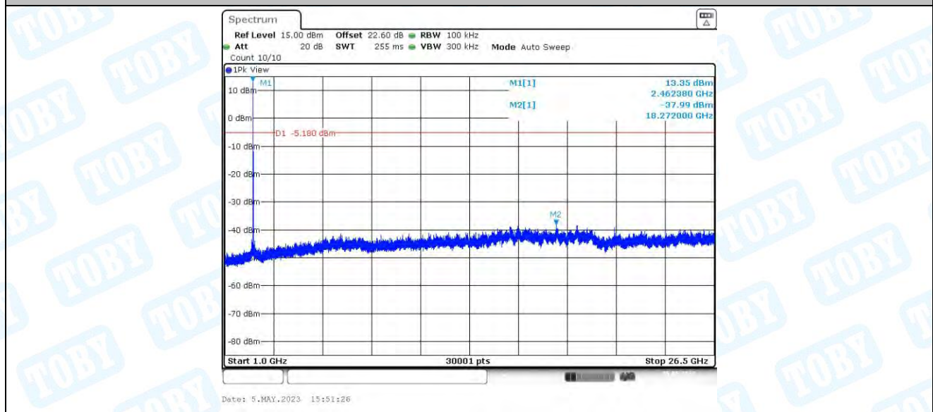
11B_Ant4_2462_0~Reference
