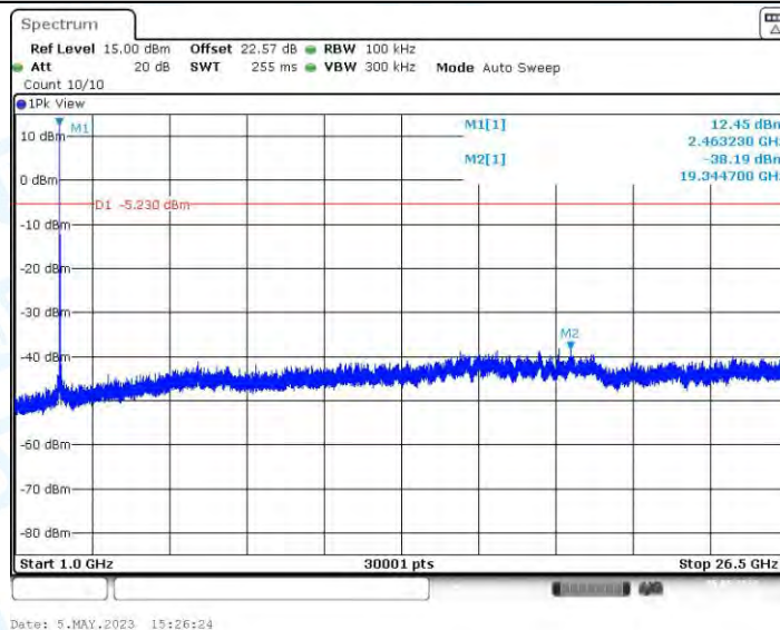
11B_Ant3_2462_0~Reference
