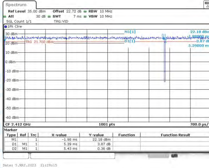
11G_Ant3_2412
