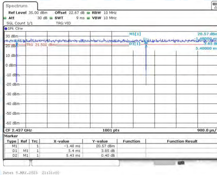
11G_Ant3_2437
