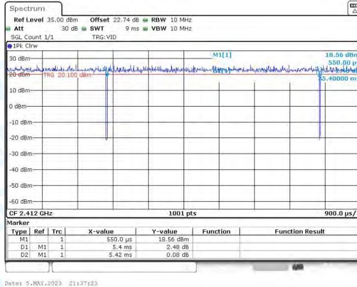
11G_Ant4_2412
