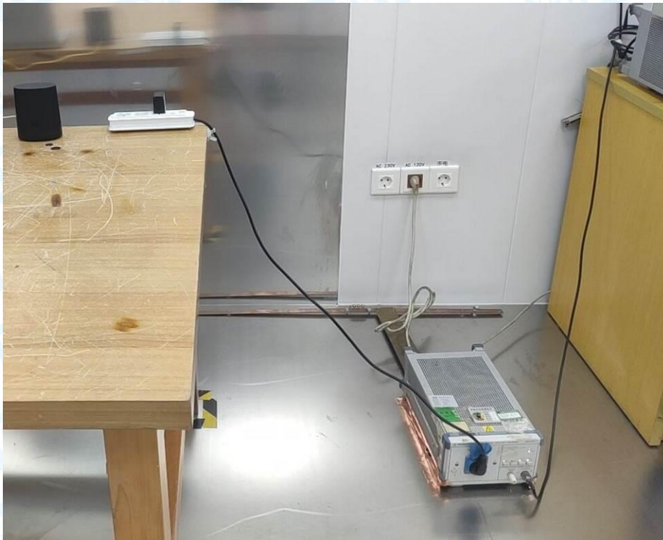
Photo of Setup for Conducted Emission
