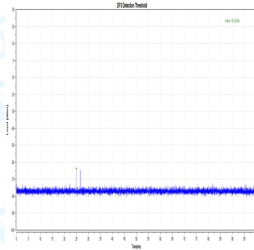
11AC80-5290-Type5
