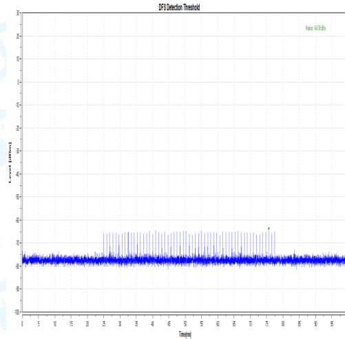
11AC80-5530-Type1
