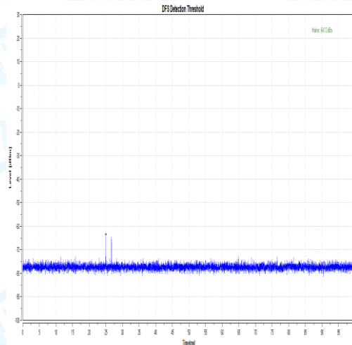
11AC40-5510-Type5
