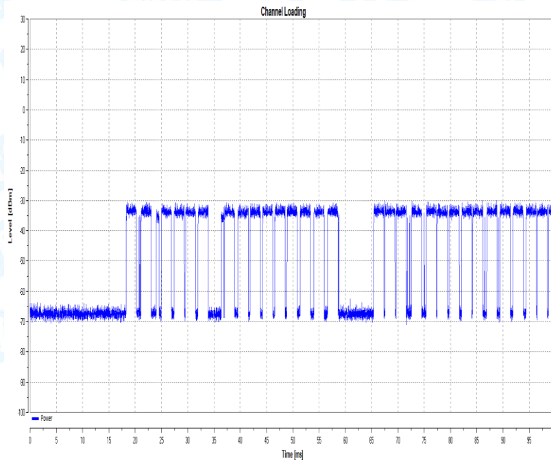
11AC80_5290
