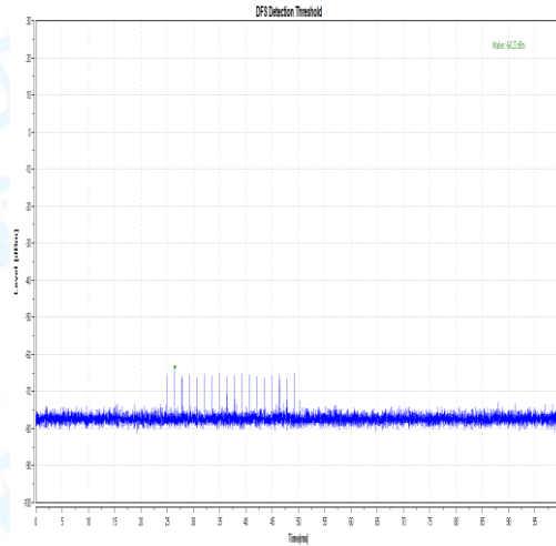
11AC40-5510-Type0
