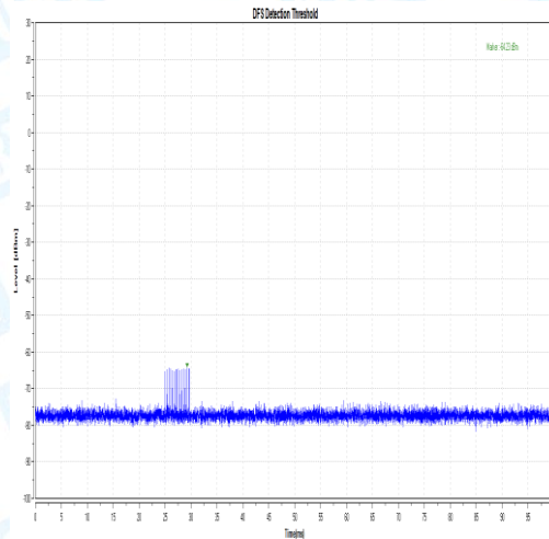
11AC40-5510-Type4
