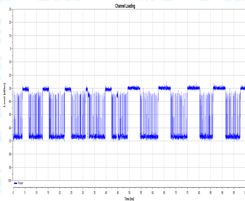
11AC80_5530
