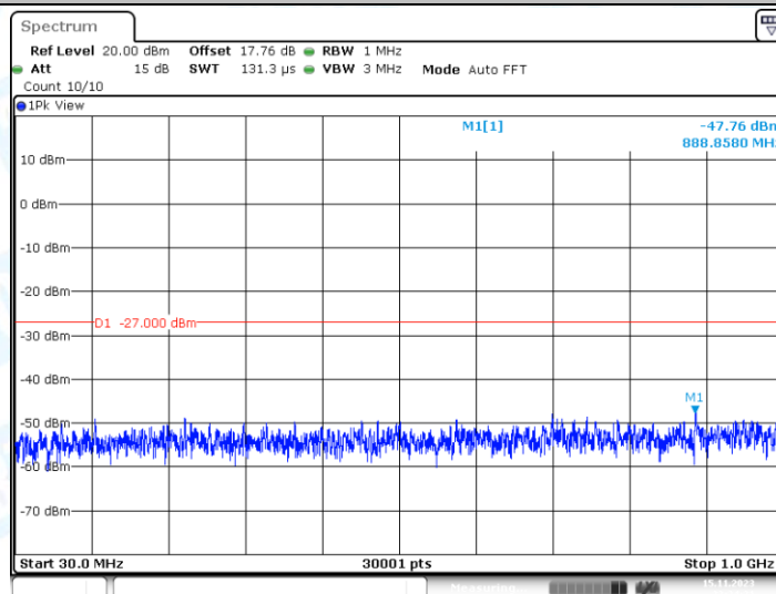
11A_Ant2_5825_30~1000
