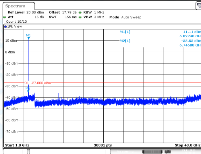
11A_Ant1_5825_1000~40000
