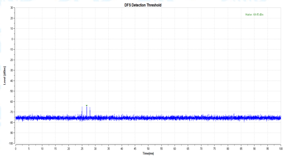
11AC80_5530_Type6
