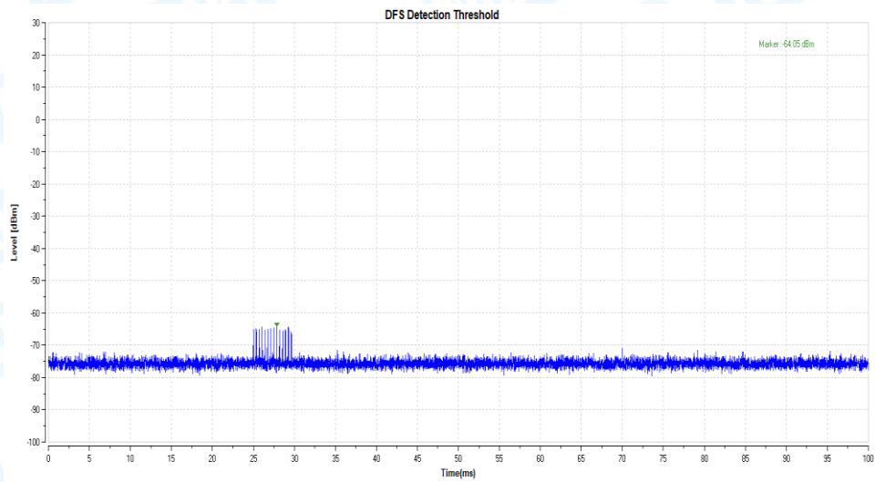
11AC80_5530_Type5
