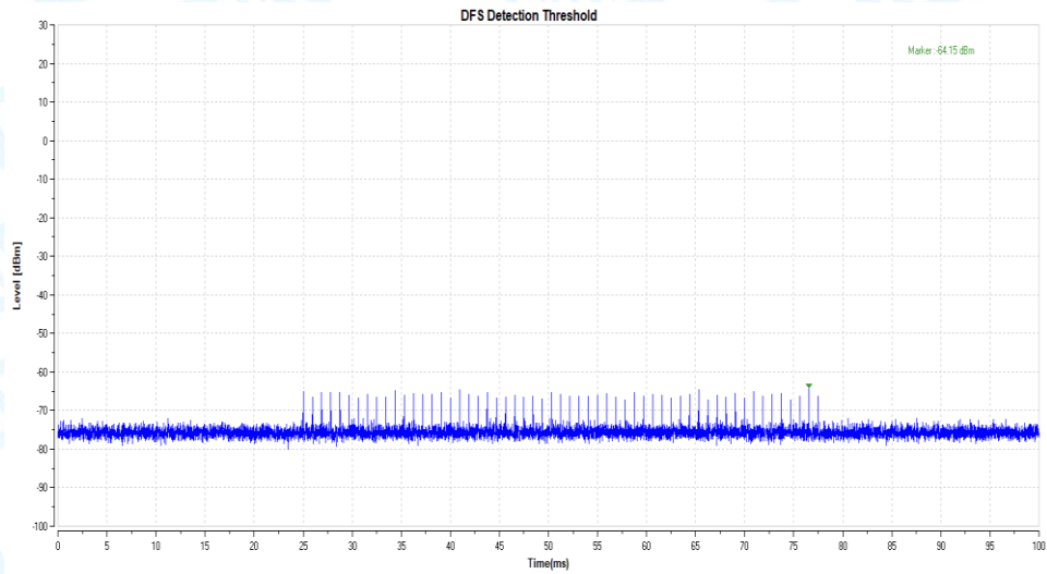
11AC80_5530_Type2
