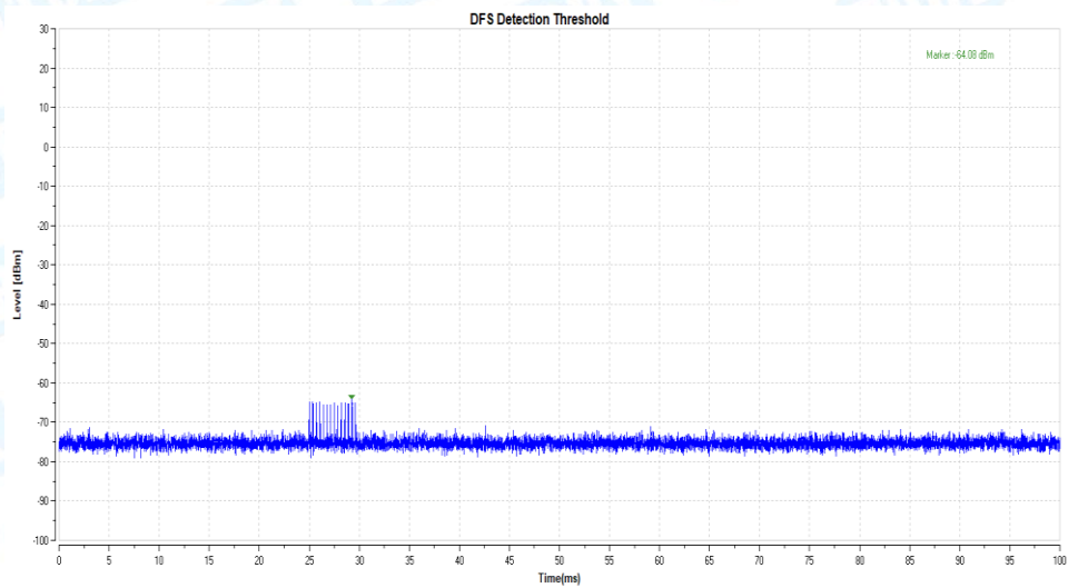
11A_5260_Type5
