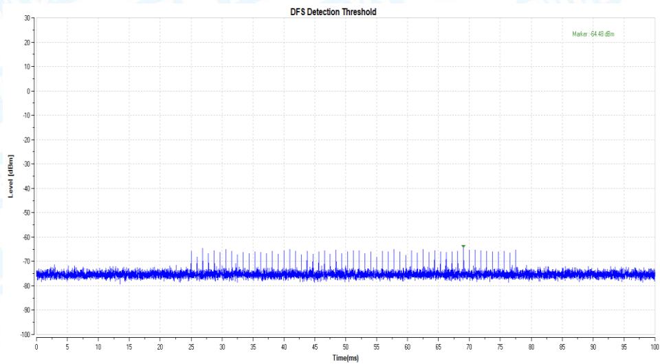
11A_5260_Type2
