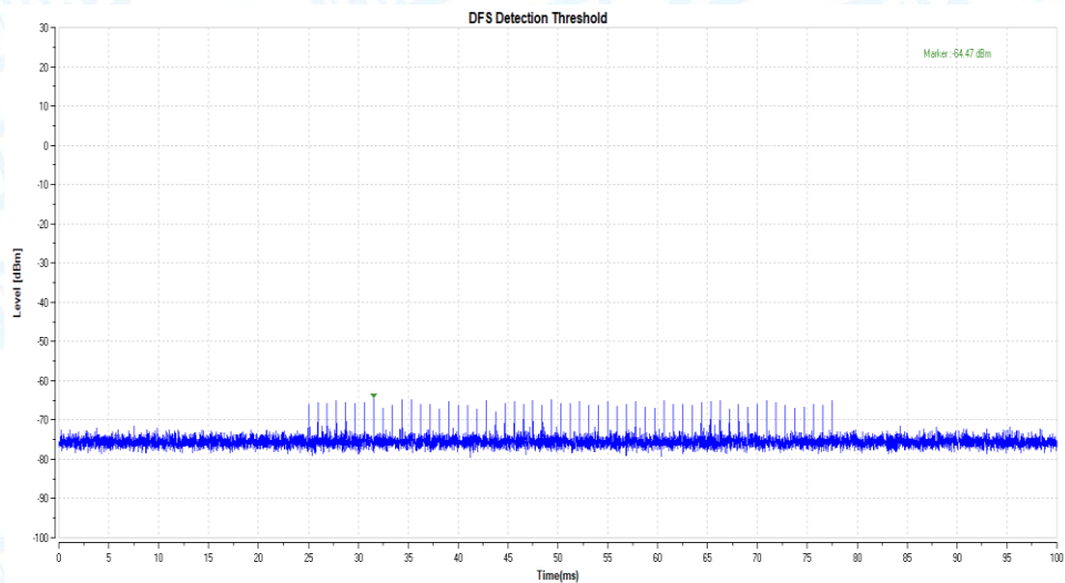
11A_5500_Type1
