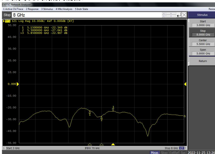
Isolation of antenna A and 5G antenna
