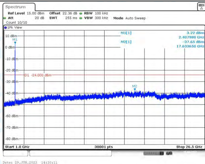
11G-CDD_Ant2_2412_0~Reference
