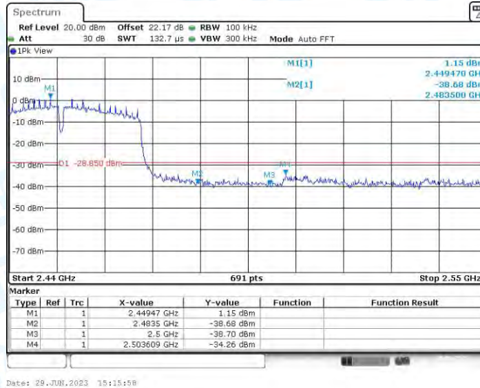
11N40-CDD_Ant2_High_2452
