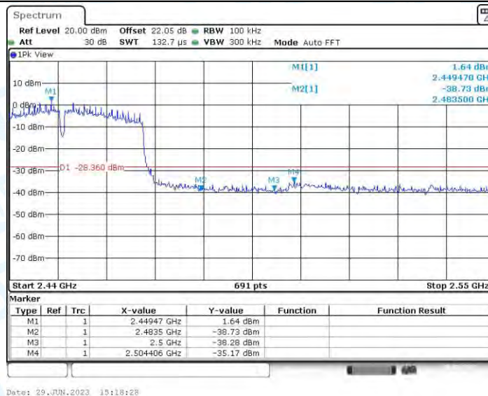
11N40-CDD_Ant2_High_2452
