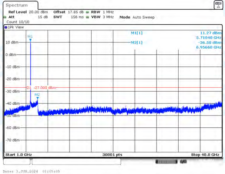
11AX40-CDD-Ant2-5710-1000~40000-PASS
