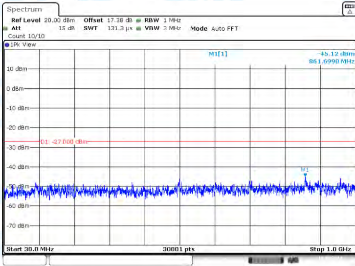
11AX40-CDD-Ant3-5795-30~1000-PASS
