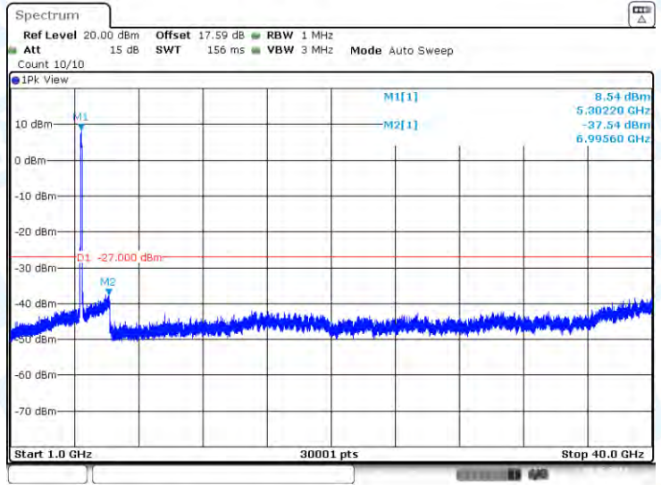
11AX80-CDD-Ant2-5290-1000~40000-PASS
