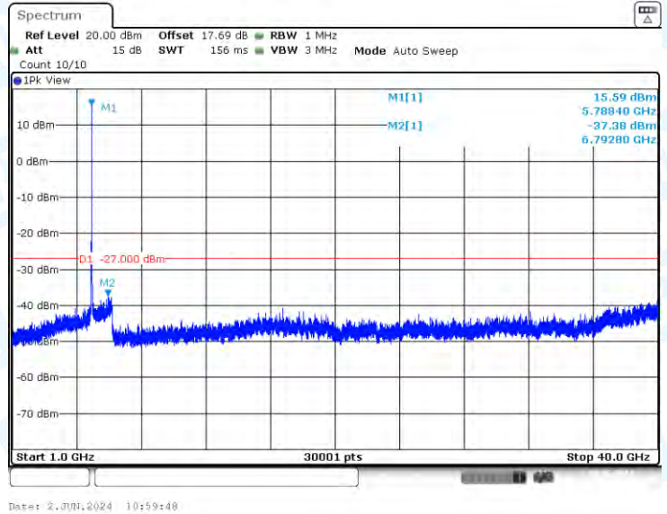
11AX20-CDD-Ant1-5785-1000~40000-PASS
