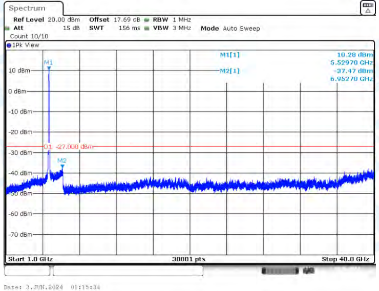
11AX80-CDD-Ant3-5530-1000~40000-PASS
