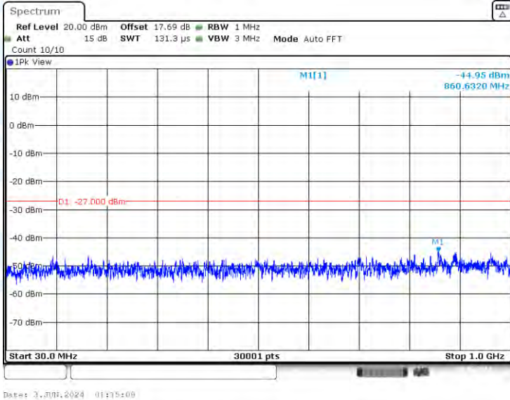
11AX80-CDD-Ant3-5530-30~1000-PASS
