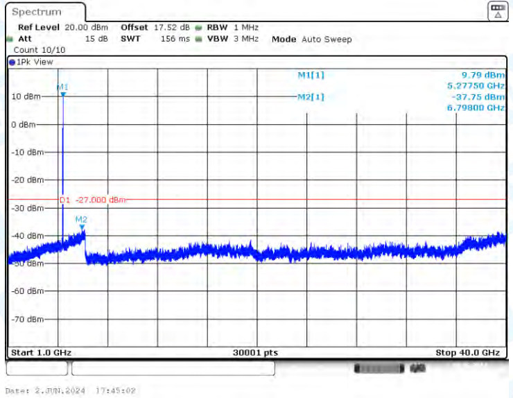
11AX20-CDD-Ant2-5280-1000~40000-PASS
