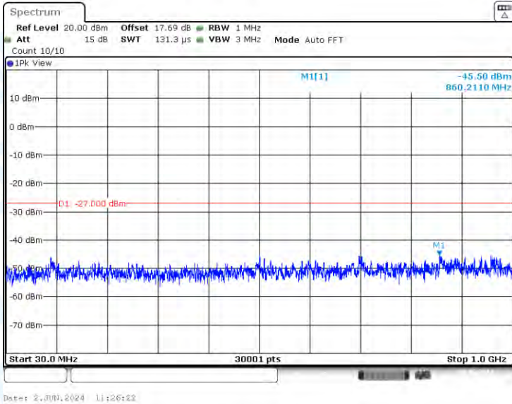
11AX40-CDD-Ant1-5795-30~1000-PASS
