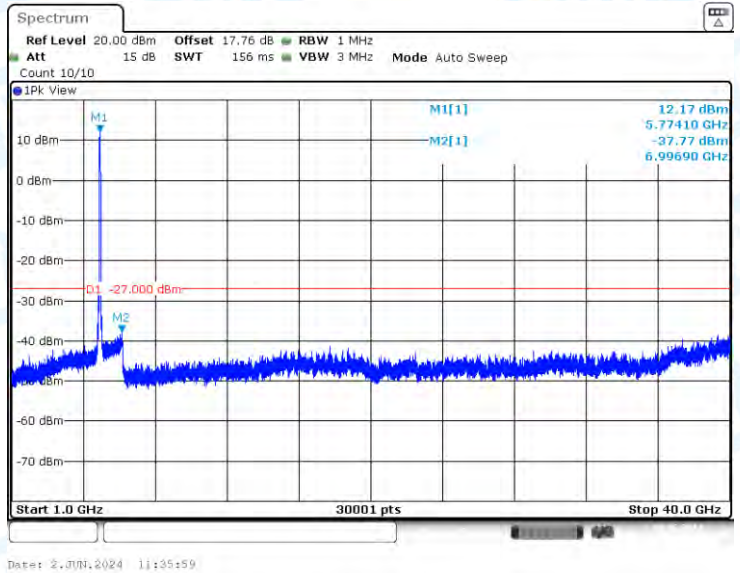
11AX80-CDD-Ant2-5775-1000~40000-PASS
