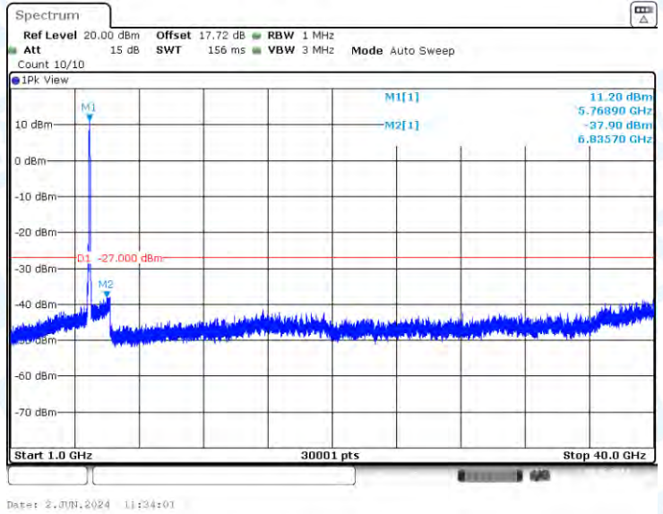
11AX80-CDD-Ant1-5775-1000~40000-PASS
