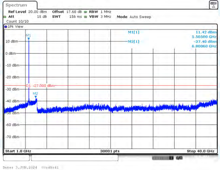
11AX40-CDD-Ant3-5510-1000~40000-PASS
