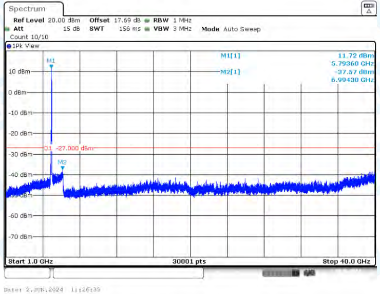
11AX40-CDD-Ant1-5795-1000~40000-PASS
