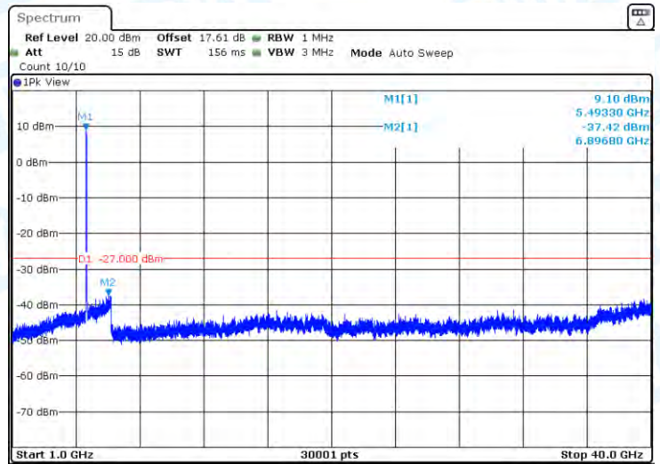
11AX40-CDD-Ant1-5510-1000~40000-PASS
