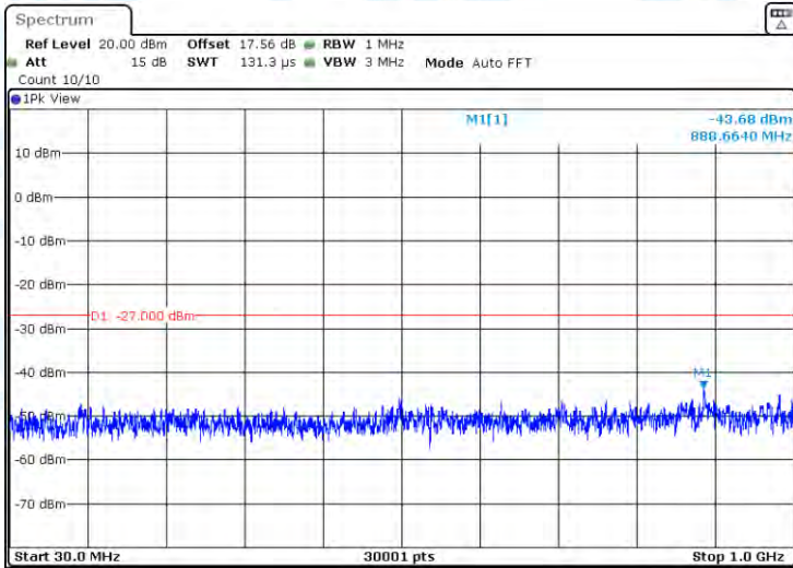
11AX80-CDD-Ant3-5290-30~1000-PASS
