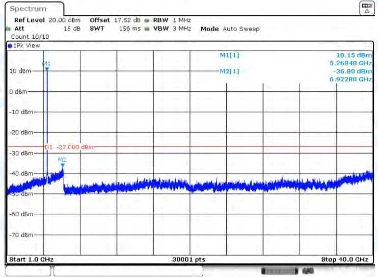
11AX40-CDD-Ant1-5270-1000~40000-PASS
