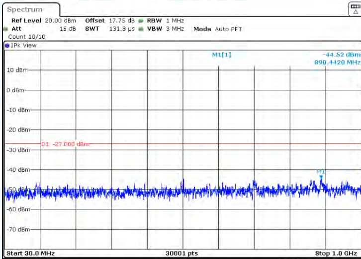
11AX40-CDD-Ant1-5755-30~1000-PASS
