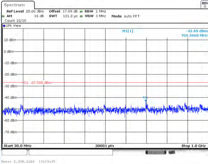
11AX20-CDD-Ant1-5785-30~1000-PASS
