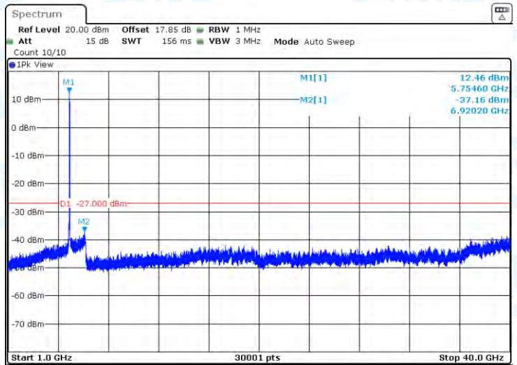
11AX40-CDD-Ant2-5755-1000~40000-PASS
