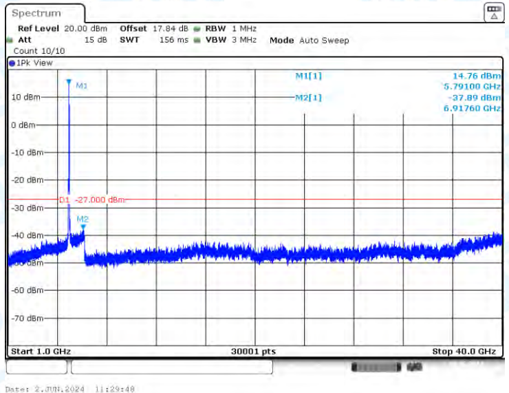
11AX40-CDD-Ant2-5795-1000~40000-PASS
