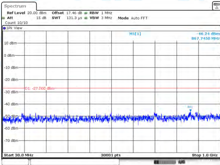
11AX80-CDD-Ant1-5210-30~1000-PASS
