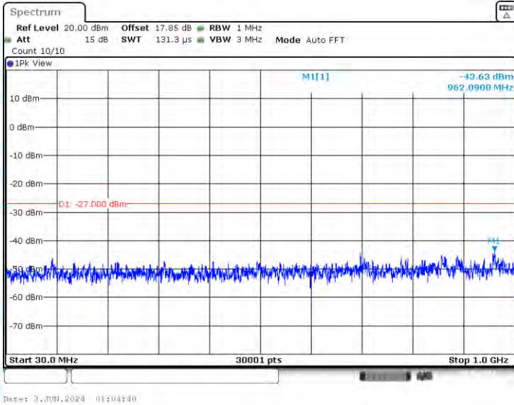
11AX40-CDD-Ant2-5710-30~1000-PASS
