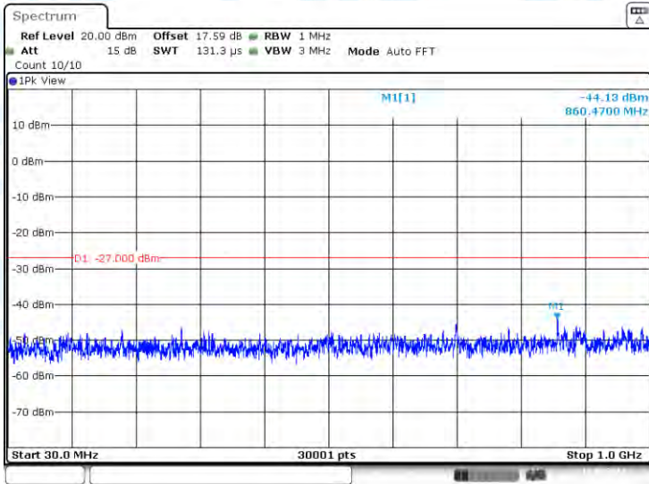
11AX160-CDD-Ant3-5250-30~1000-PASS
