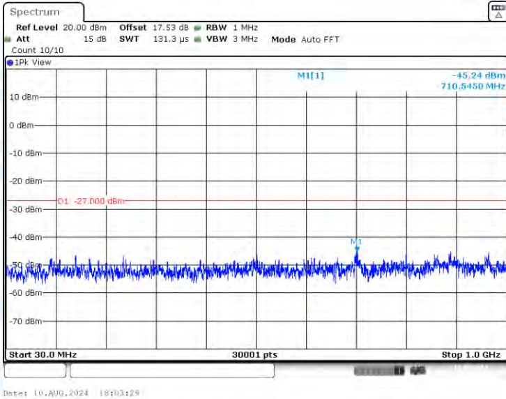
11AX80-CDD-Ant3-5210-30~1000-PASS
