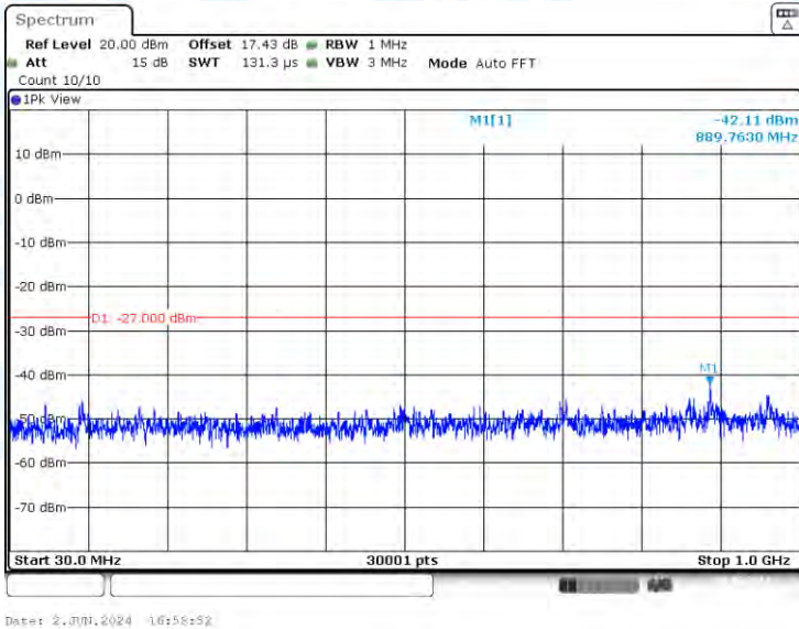
11AX80-CDD-Ant1-5290-30~1000-PASS
