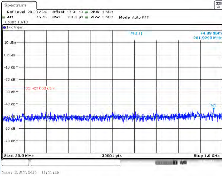
11AX20-CDD-Ant3-5825-30~1000-PASS
