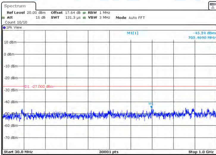
11AX20-CDD-Ant1-5500-30~1000-PASS
