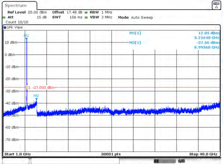
11AX40-CDD-Ant3-5190-1000~40000-PASS
