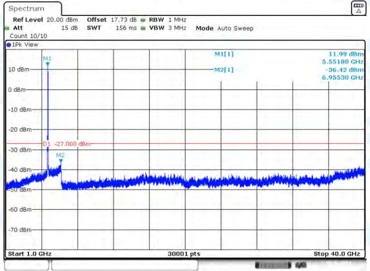
11AX40-CDD-Ant2-5550-1000~40000-PASS
