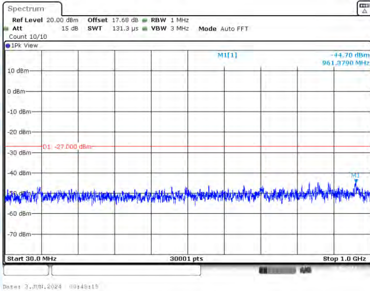
11AX40-CDD-Ant3-5510-30~1000-PASS
