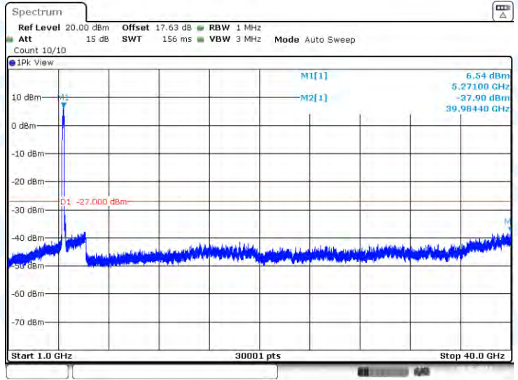
11AX160-CDD-Ant2-5250-1000~40000-PASS
