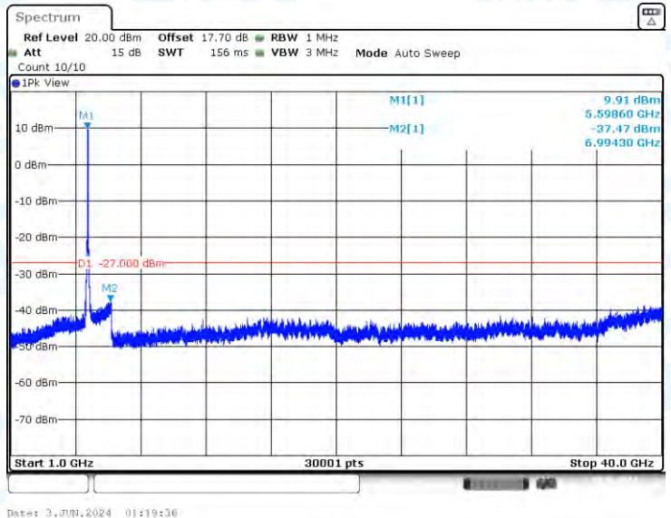
11AX80-CDD-Ant3-5530-1000~40000-PASS
