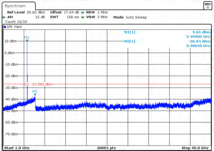
11AX20-CDD-Ant1-5500-1000~40000-PASS
