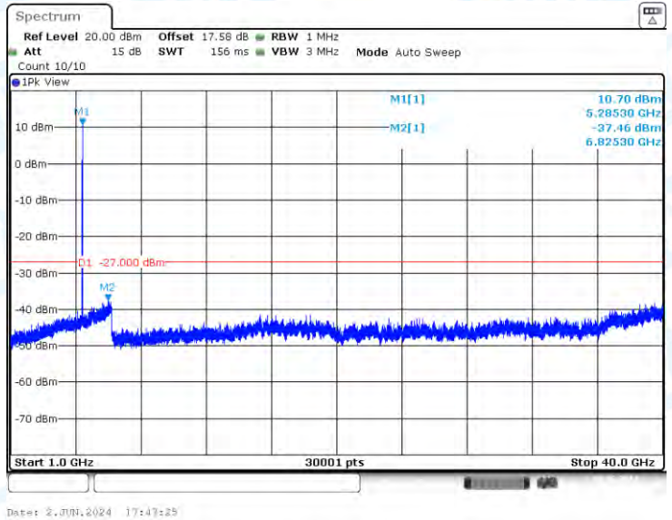
11AX20-CDD-Ant3-5280-1000~40000-PASS
