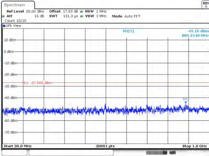
11AX160-CDD-Ant2-5250-30~1000-PASS
