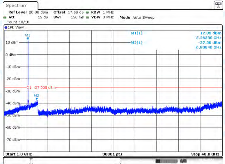
11AX40-CDD-Ant2-5270-1000~40000-PASS
