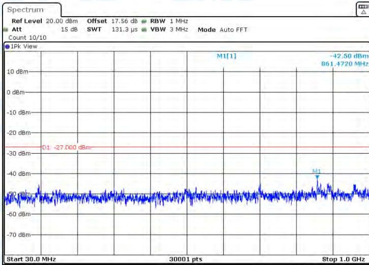
11AX20-CDD-Ant3-5320-30~1000-PASS
