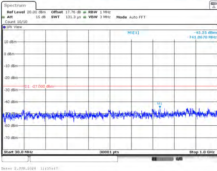
11AX80-CDD-Ant2-5775-30~1000-PASS
