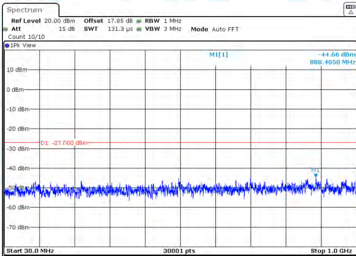
11AX40-CDD-Ant2-5755-30~1000-PASS
