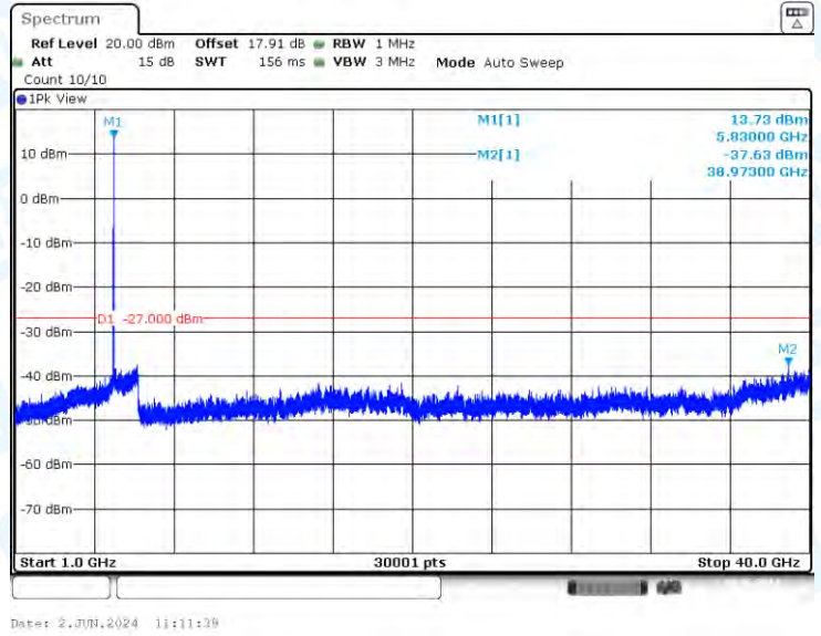
11AX20-CDD-Ant3-5825-1000~40000-PASS
