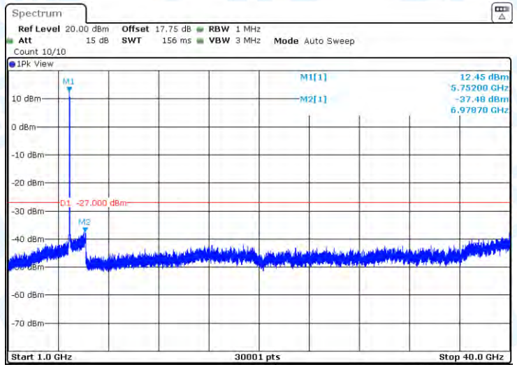
11AX40-CDD-Ant1-5755-1000~40000-PASS
