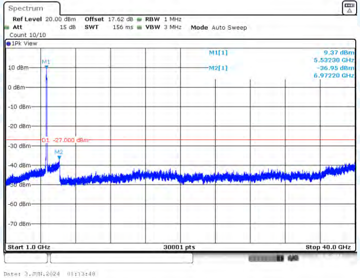
11AX80-CDD-Ant2-5530-1000~40000-PASS
