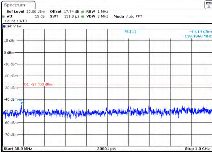
11AX20-CDD-Ant3-5785-30~1000-PASS
