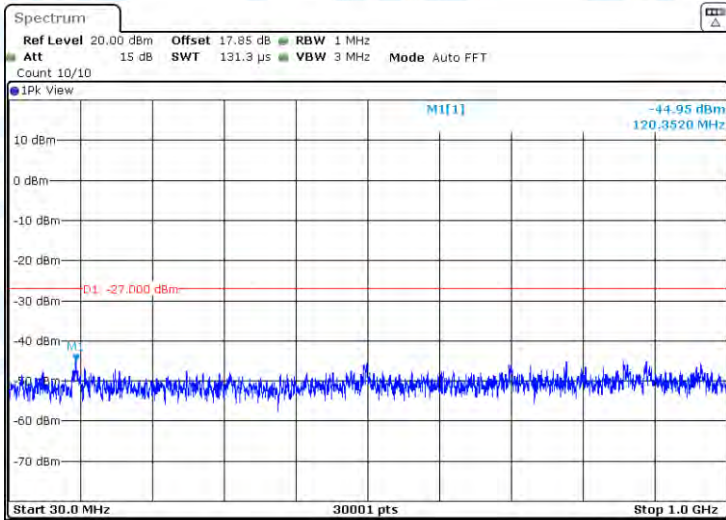
11AX20-CDD-Ant1-5825-30~1000-PASS
