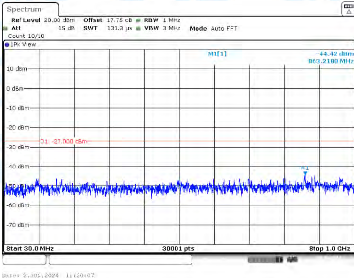
11AX40-CDD-Ant3-5710-30~1000-PASS
