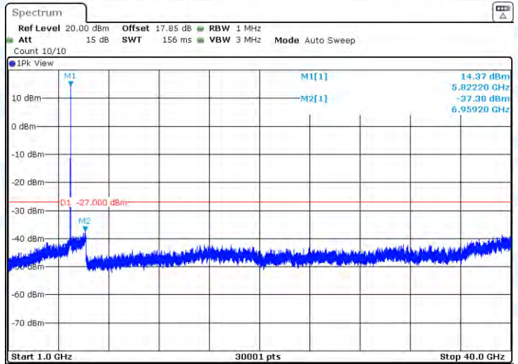
11AX20-CDD-Ant1-5825-1000~40000-PASS
