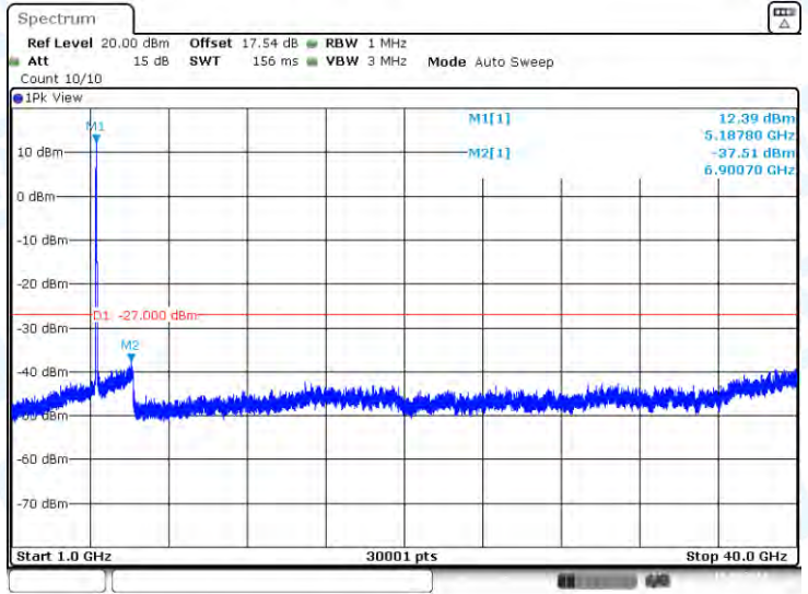
11AX40-CDD-Ant2-5190-1000~40000-PASS
