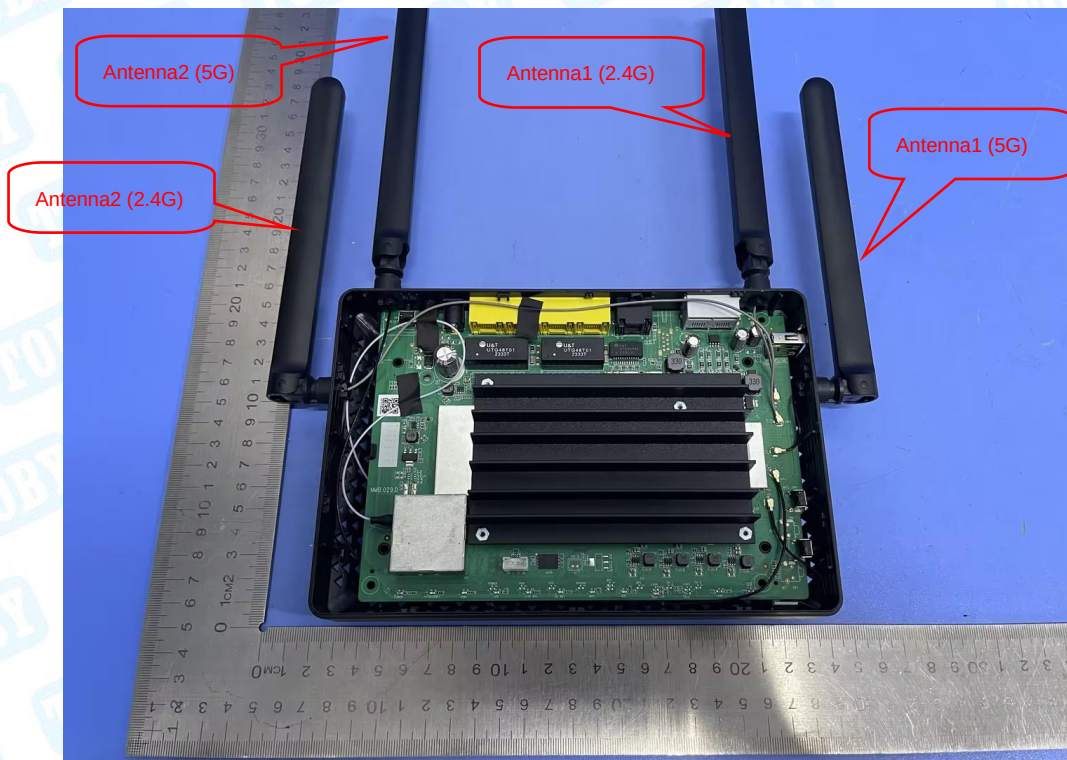
Photo 9 Internal of EUT
