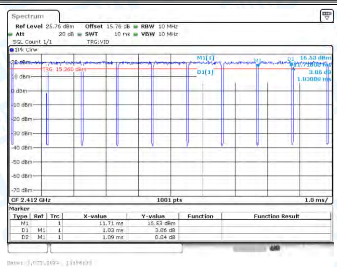
NTNV-11AX20-CDD-Ant2-2412
