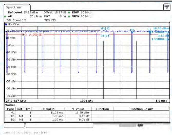
NTNV-11AX20-CDD-Ant2-2437
