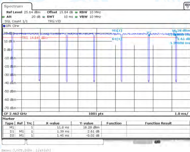
NTNV-11G-Ant1-2462
