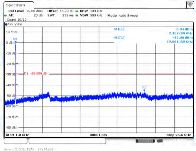
11AX40-CDD-Ant2-2452-1000~26500-PASS
