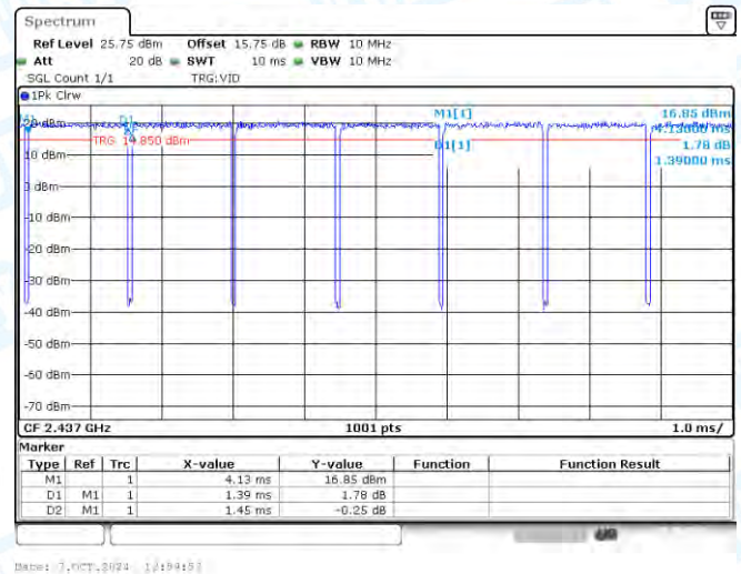
NTNV-11G-Ant2-2437
