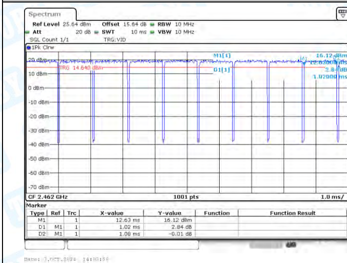
NTNV-11AX20-CDD-Ant1-2462
