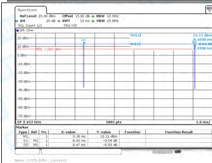
NTNV-11B-CDD-Ant1-2412
