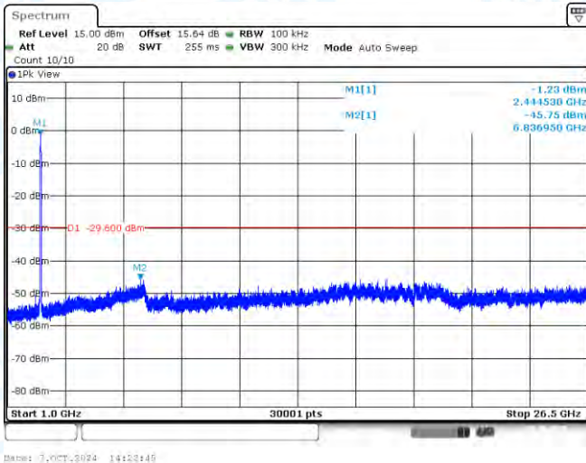
11AX40-CDD-Ant1-2452-1000~26500-PASS
