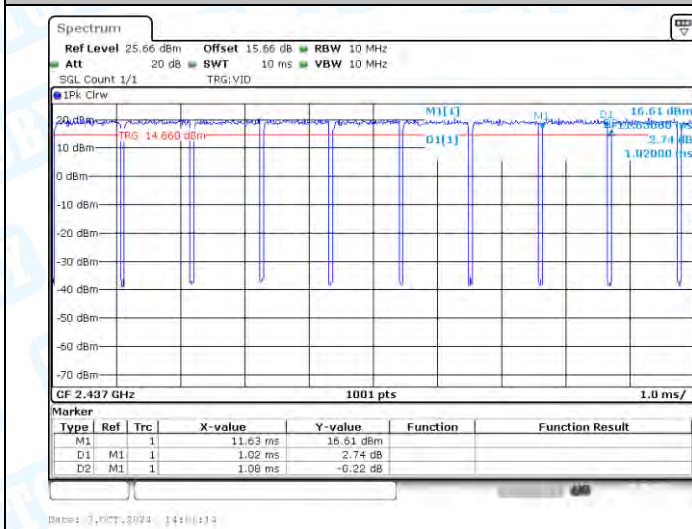
NTNV-11AX20-CDD-Ant1-2437
