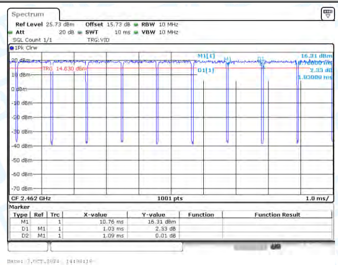
NTNV-11AX20-CDD-Ant2-2462
