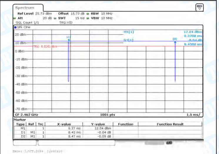
NTNV-11B-CDD-Ant2-2462
