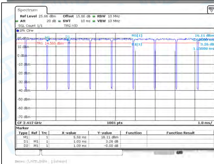
NTNV-11AX20-CDD-Ant1-2412
