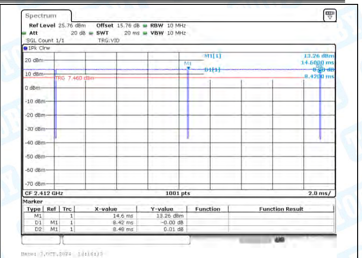
NTNV-11B-CDD-Ant2-2412
