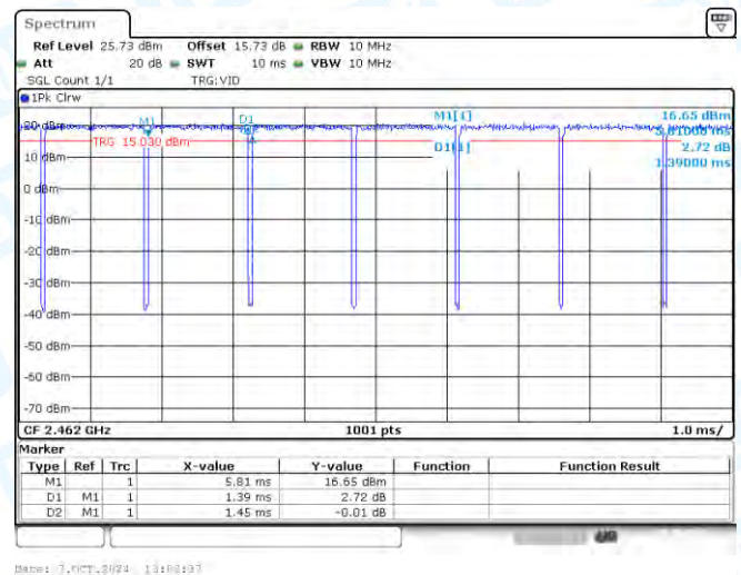
NTNV-11G-Ant2-2462
