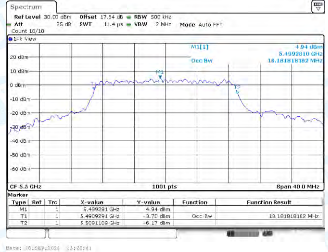
11N20-CDD-Ant2-5500
