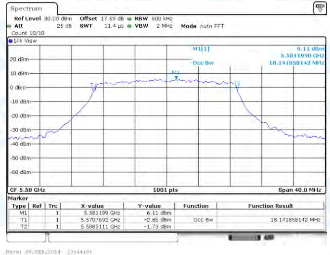
11N20-CDD-Ant1-5580
