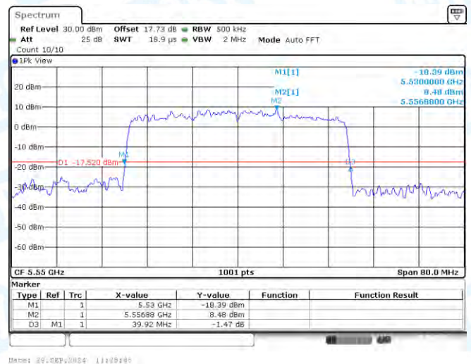
11AX40-CDD-Ant3-5550
