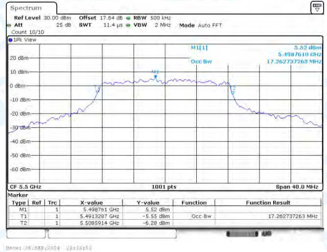
11A-CDD-Ant2-5500
