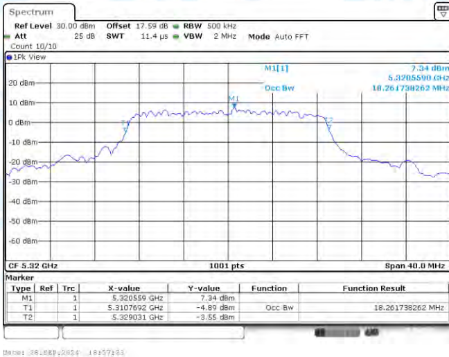
11AC20-CDD-Ant3-5320
