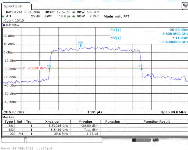
11AX40-CDD-Ant2-5550
