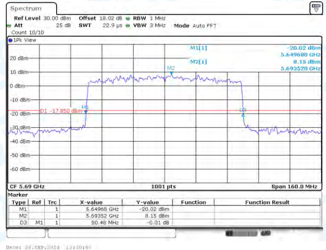
11AX80-CDD-Ant3-5690
