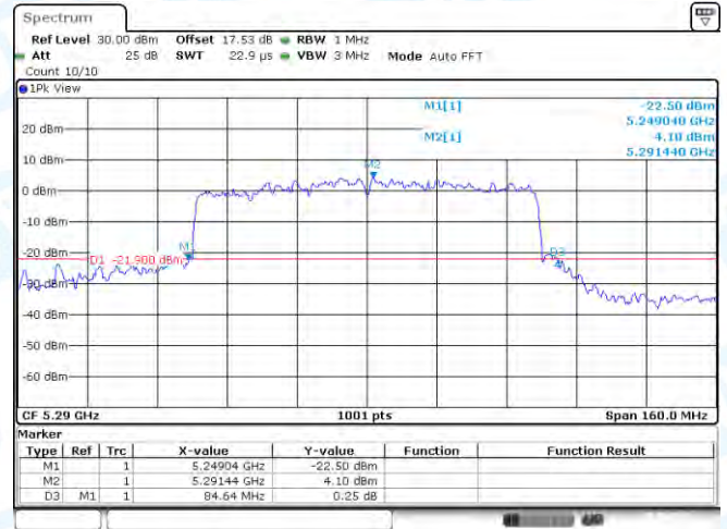
11AX80-CDD-Ant2-5290
