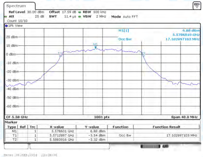
11A-CDD-Ant1-5580
