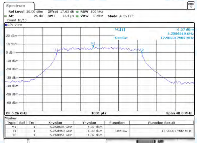
11N20-CDD-Ant1-5260
