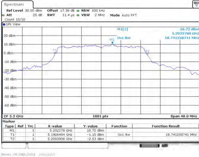
11AC20-CDD-Ant1-5200
