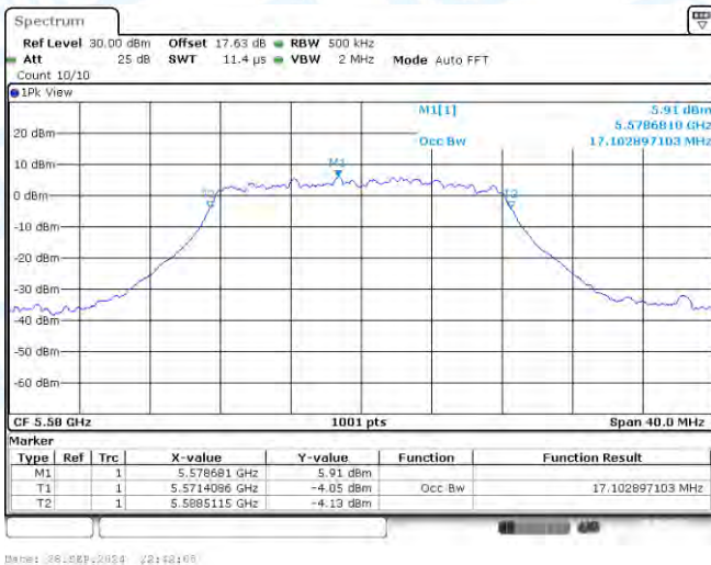
11A-CDD-Ant2-5580
