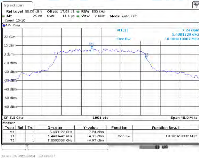
11N20-CDD-Ant3-5500
