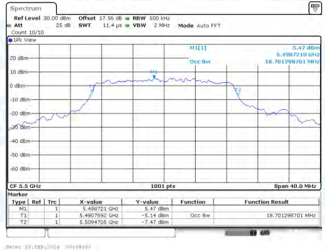
11AC20-CDD-Ant1-5500
