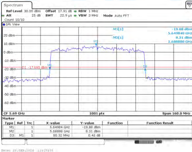
11AX80-CDD-Ant2-5690
