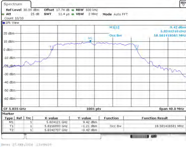
11AC20-CDD-Ant1-5825
