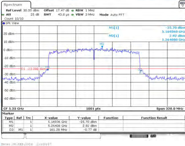
11AX160-CDD-Ant1-5250
