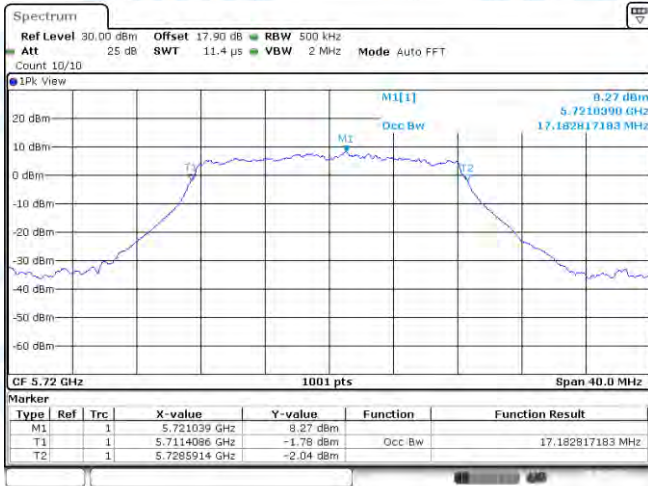
11A-CDD-Ant1-5720
