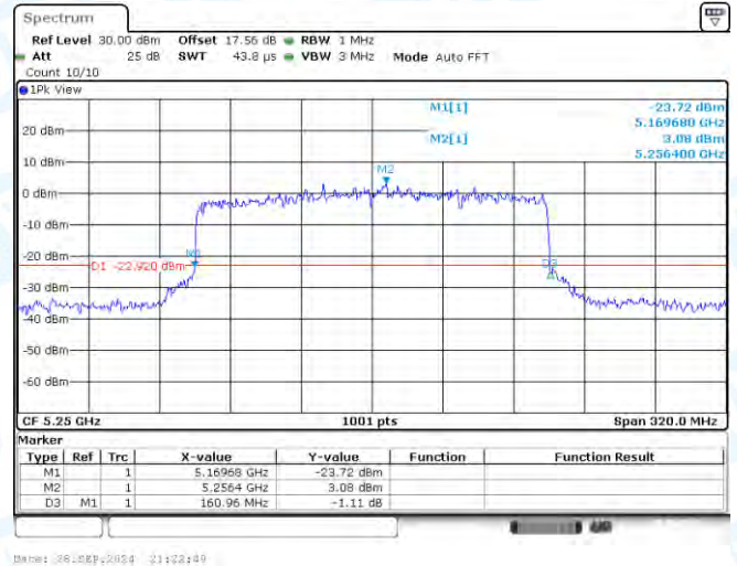
11AX160-CDD-Ant2-5250
