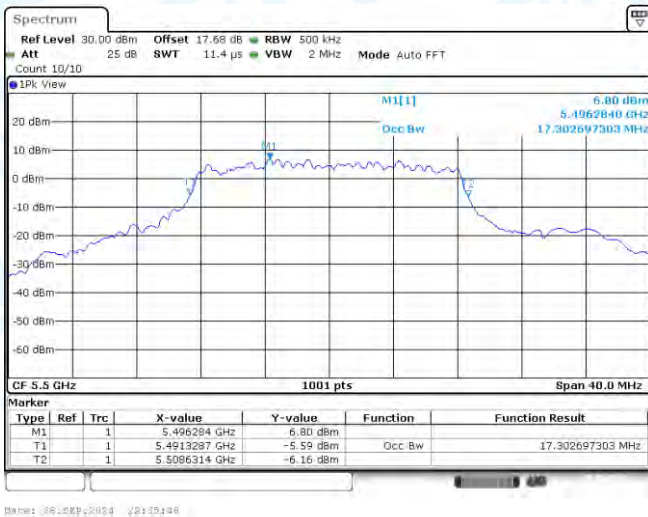
11A-CDD-Ant3-5500
