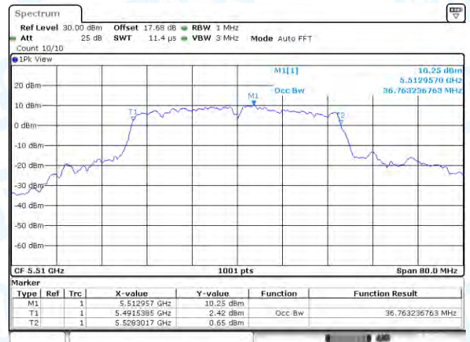
11AC40-CDD-Ant1-5510
