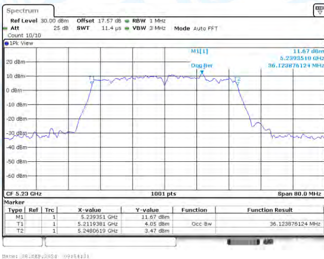
11N40-CDD-Ant2-5230
