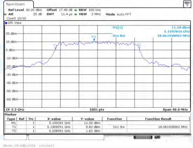
11AC20-CDD-Ant2-5200
