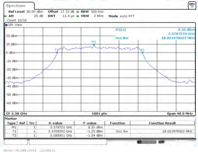
11N20-CDD-Ant3-5580
