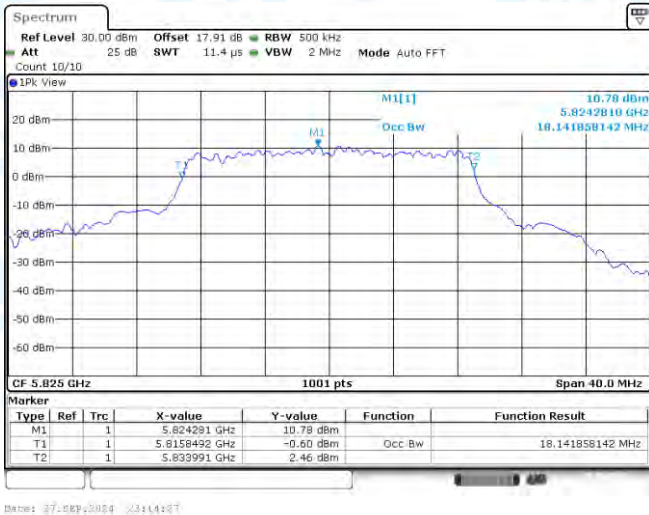
11AC20-CDD-Ant3-5825
