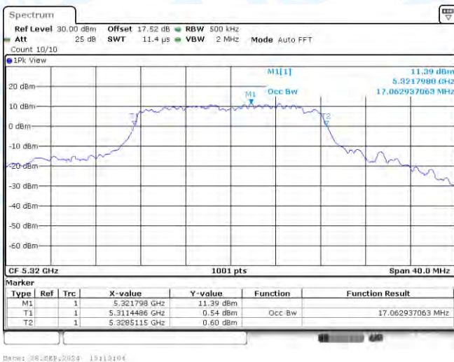
11A-Ant2-5320
