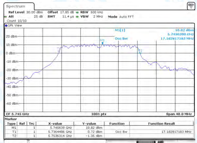
11A-CDD-Ant1-5745
