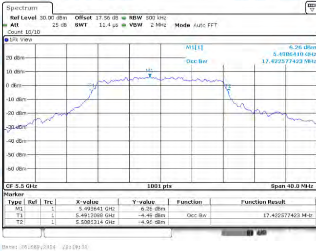
11A-CDD-Ant1-5500
