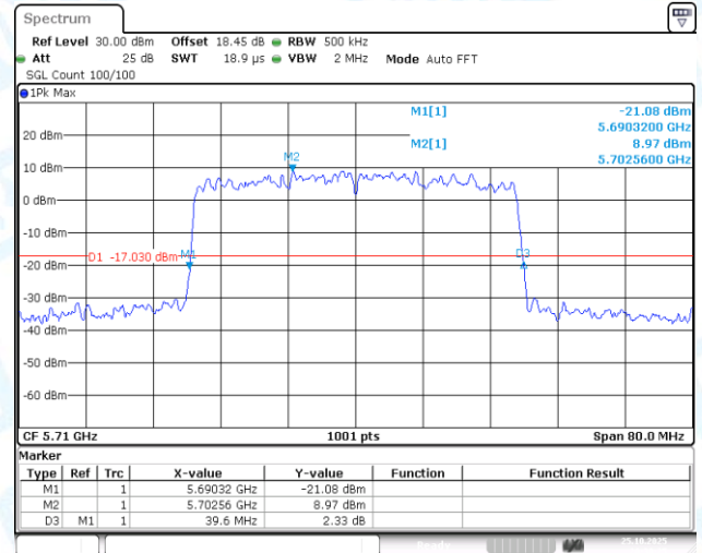
11AX40-CDD-Ant1-5710
