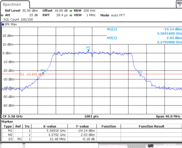
11AC20-CDD-Ant1-5580
