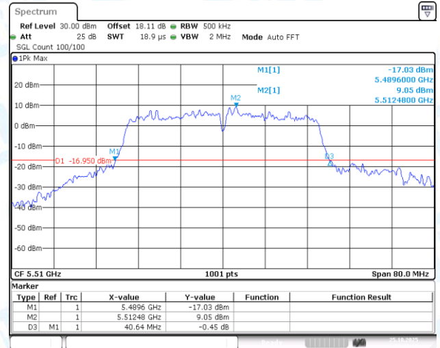
11AC40-CDD-Ant2-5510
