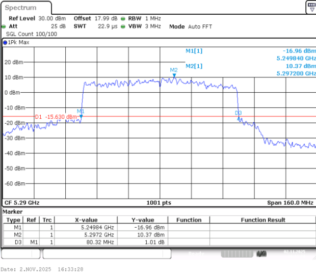
11AX80-CDD-Ant2-5290
