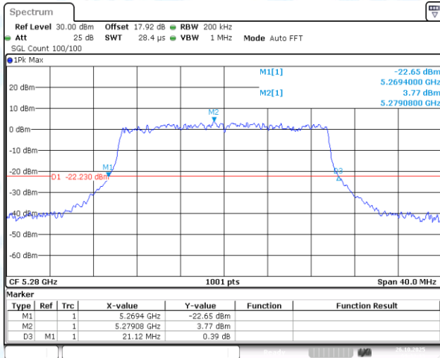
11AX20-CDD-Ant1-5280
