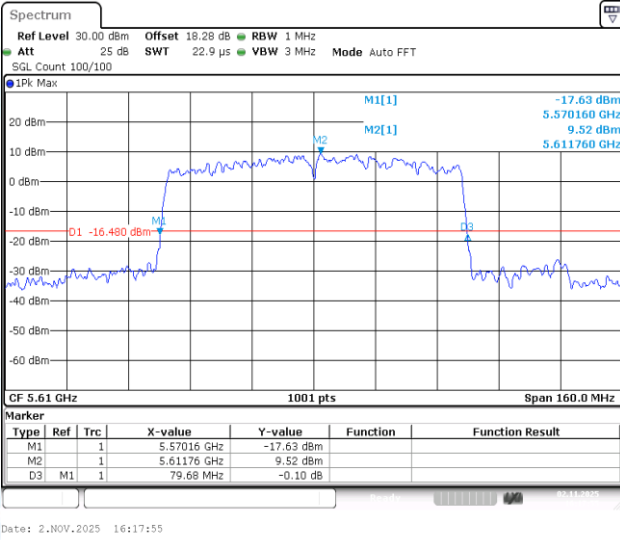
11AC80-CDD-Ant1-5610
