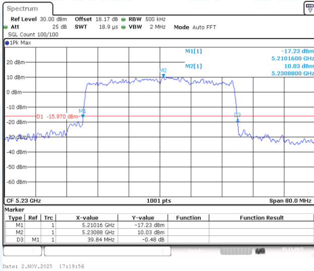
11AX40-CDD-Ant3-5230
