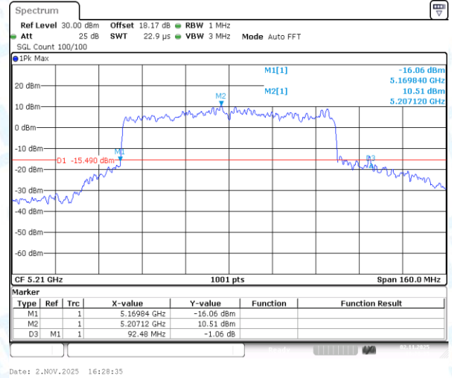
11AX80-CDD-Ant2-5210
