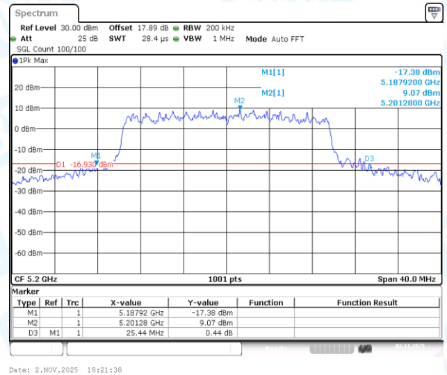
11AX20-CDD-Ant3-5200
