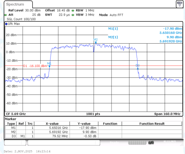
11AC80-CDD-Ant2-5690
