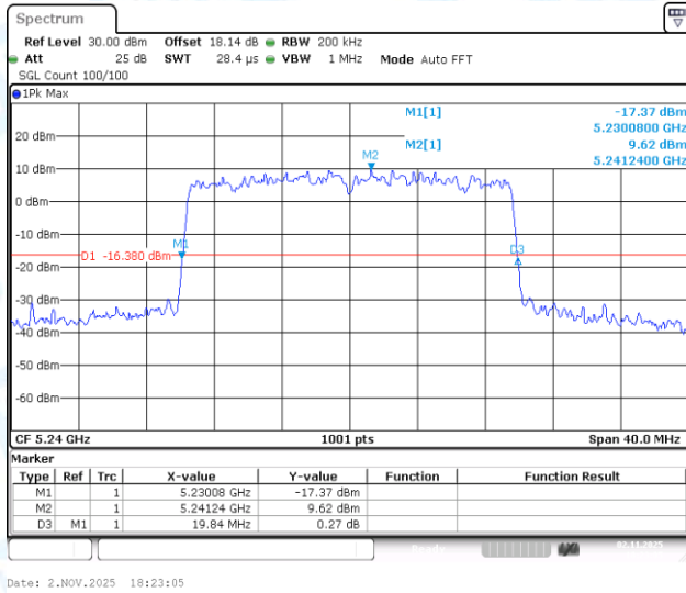
11AX20-CDD-Ant1-5240
