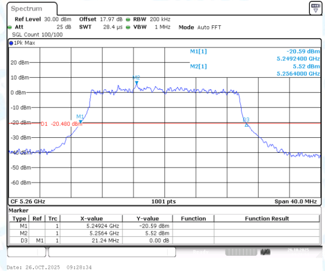
11AX20-CDD-Ant1-5260
