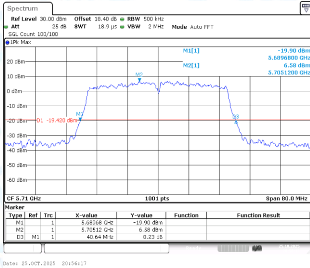
11AC40-CDD-Ant1-5710
