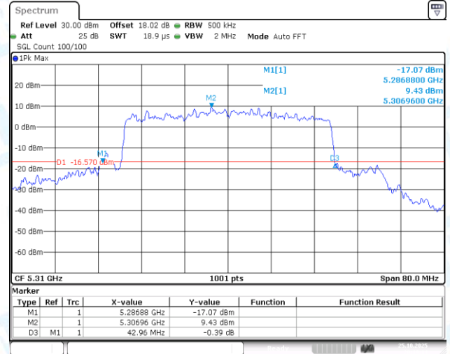
11AX40-CDD-Ant2-5310
