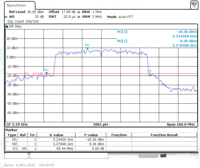
11AC80-CDD-Ant2-5290
