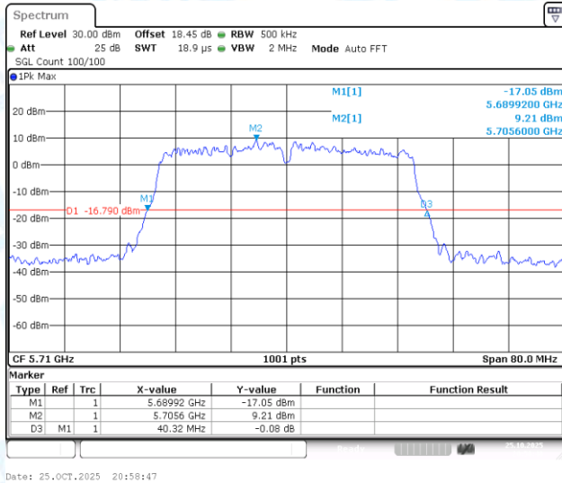
11AC40-CDD-Ant3-5710
