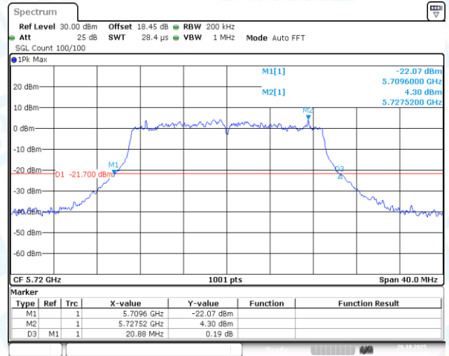
11AC20-CDD-Ant1-5720
