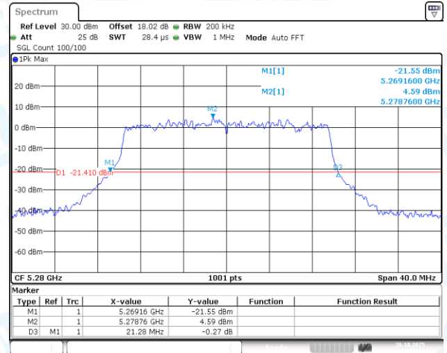
11AX20-CDD-Ant2-5280
