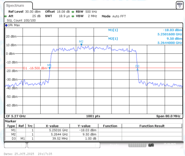
11AX40-CDD-Ant3-5270
