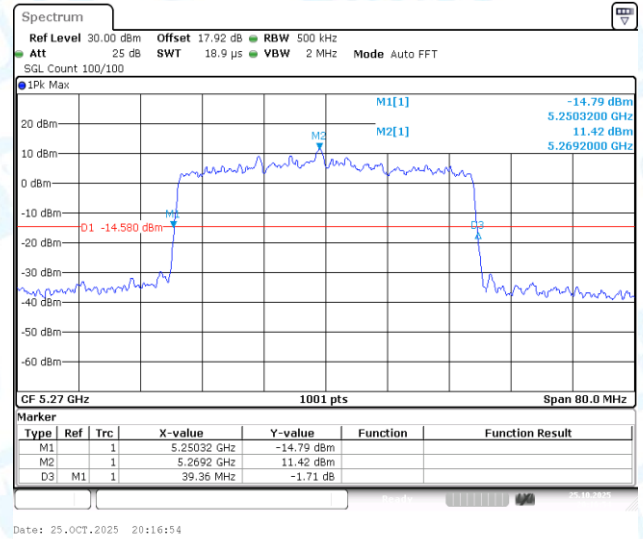
11AX40-CDD-Ant1-5270
