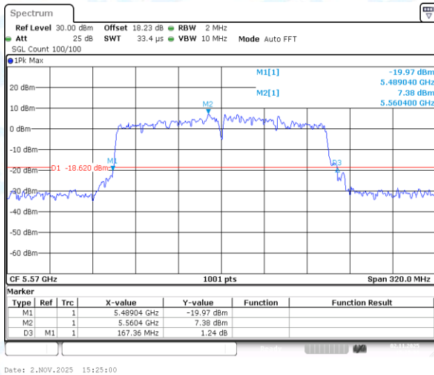
11AC160-CDD-Ant2-5570
