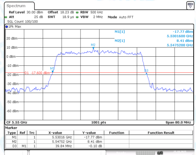
11AC40-CDD-Ant1-5550
