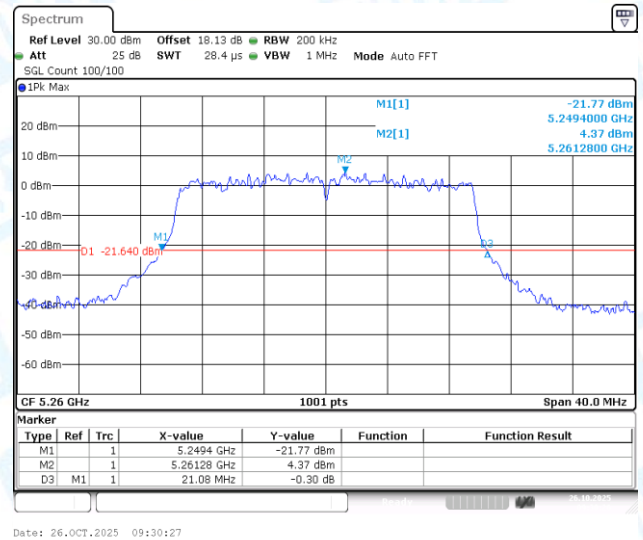
11AX20-CDD-Ant3-5260
