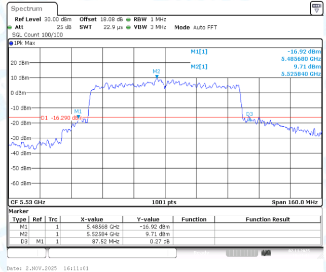
11AC80-CDD-Ant1-5530
