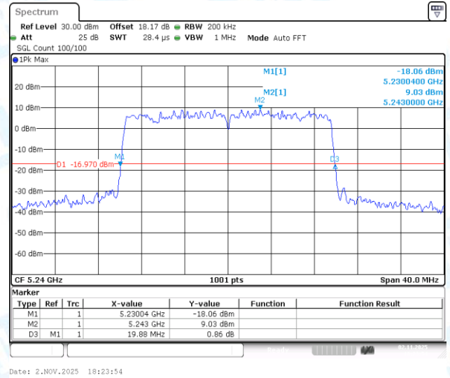
11AX20-CDD-Ant2-5240
