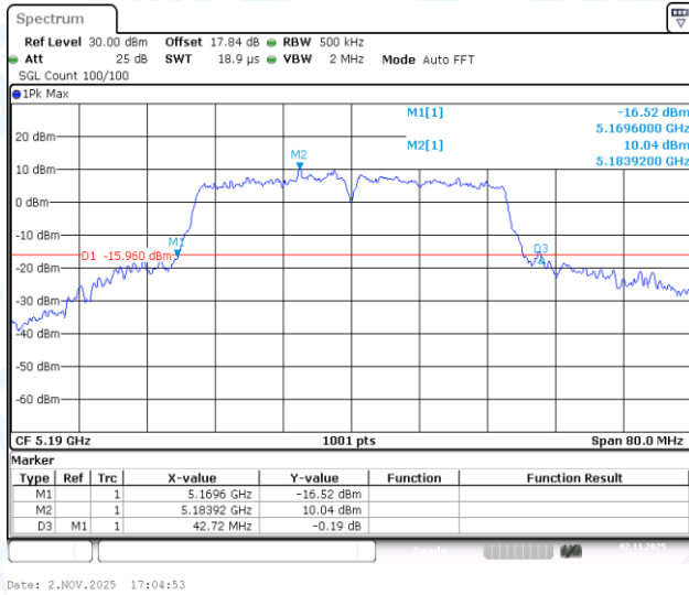
11AC40-CDD-Ant1-5190
