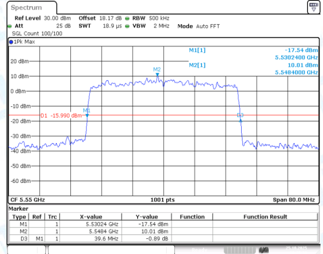
11AX40-CDD-Ant2-5550
