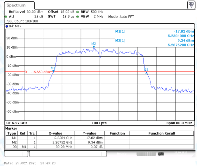
11AC40-CDD-Ant2-5270
