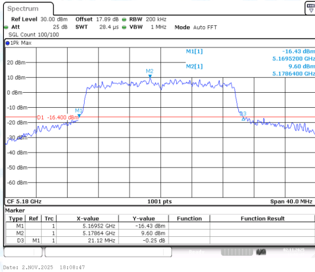
11AX20-CDD-Ant2-5180
