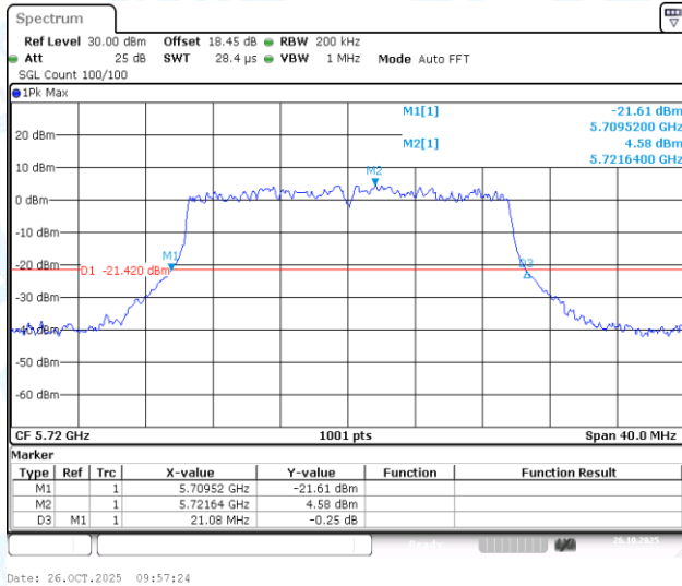
11AX20-CDD-Ant3-5720
