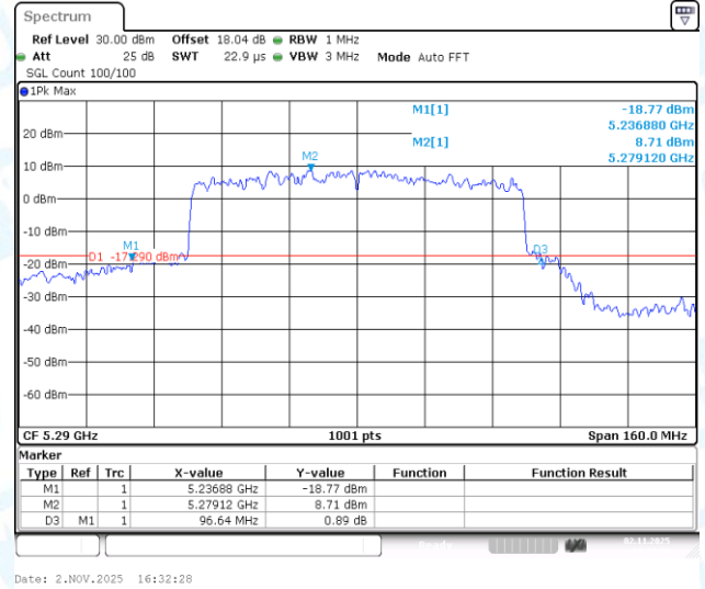
11AX80-CDD-Ant1-5290
