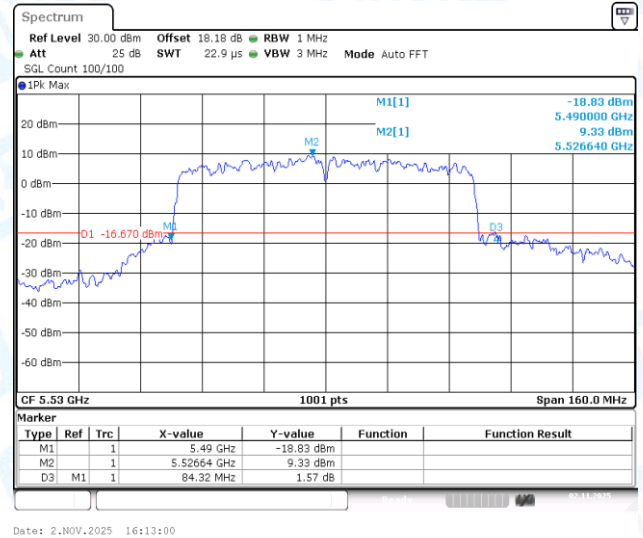
11AC80-CDD-Ant3-5530
