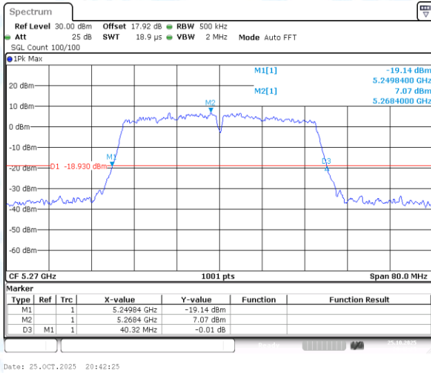
11AC40-CDD-Ant1-5270
