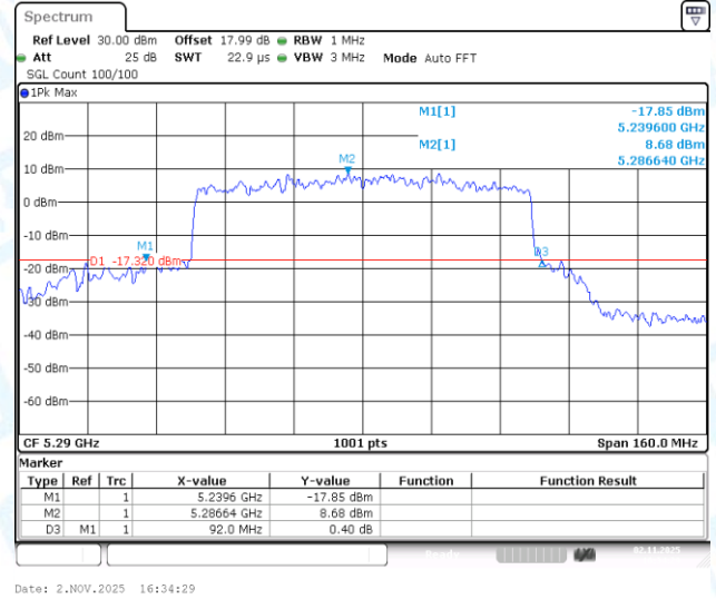
11AX80-CDD-Ant3-5290
