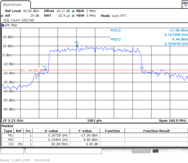
11AX80-CDD-Ant3-5210
