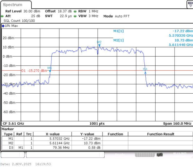
11AC80-CDD-Ant3-5610
