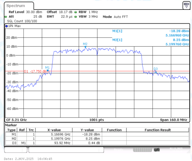
11AC80-CDD-Ant3-5210
