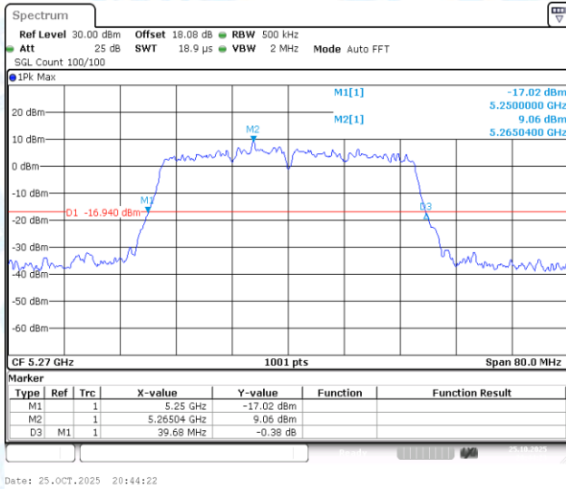
11AC40-CDD-Ant3-5270
