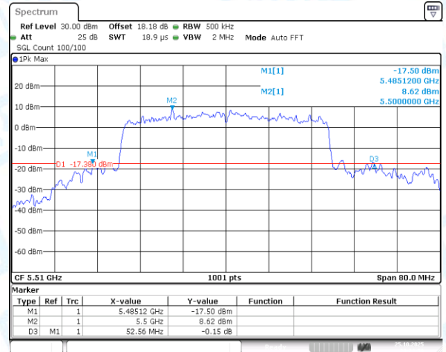
11AX40-CDD-Ant1-5510
