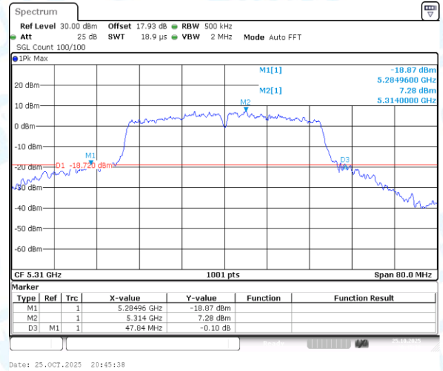
11AC40-CDD-Ant1-5310
