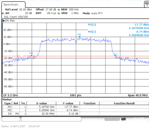
11AX20-CDD-Ant2-5200
