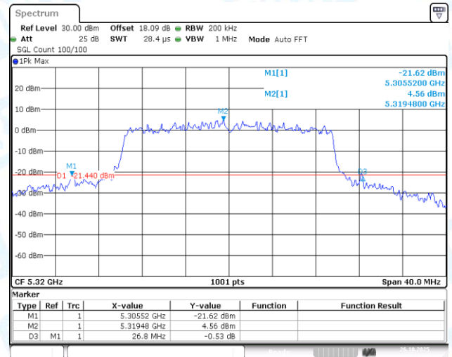
11AX20-CDD-Ant1-5320
