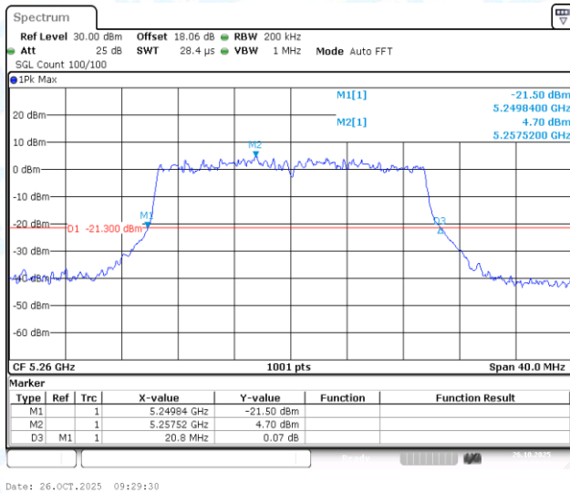
11AX20-CDD-Ant2-5260
