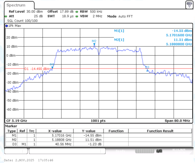
11AC40-CDD-Ant2-5190
