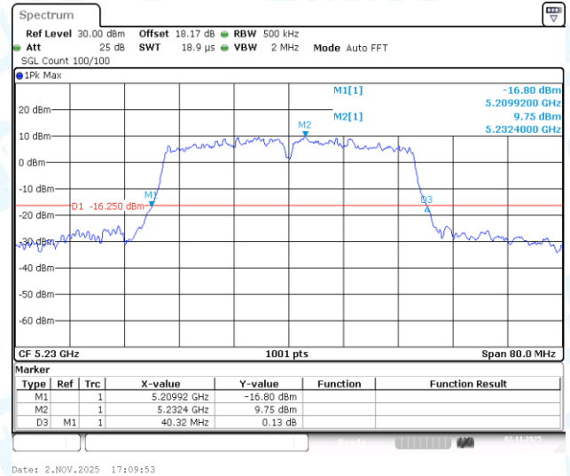
11AC40-CDD-Ant3-5230
