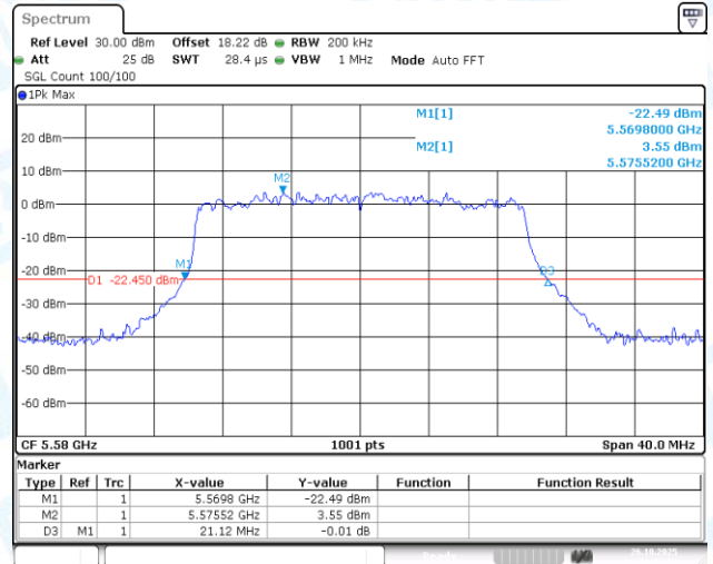
11AX20-CDD-Ant1-5580
