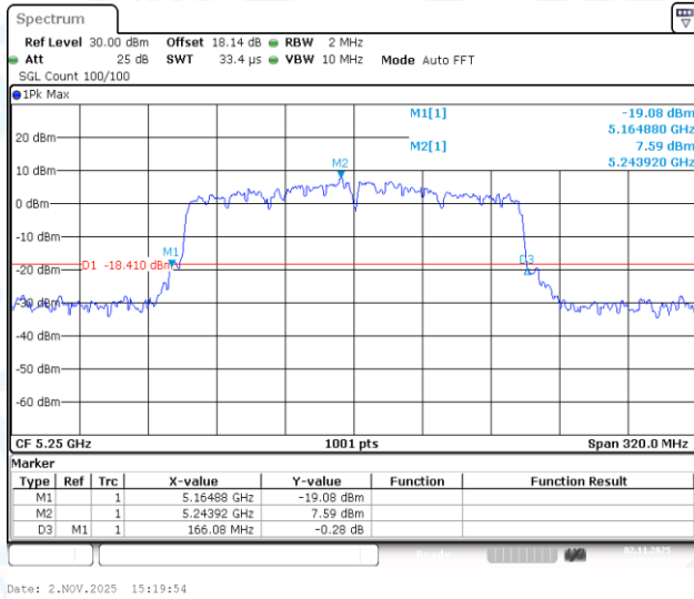
11AC160-CDD-Ant1-5250
