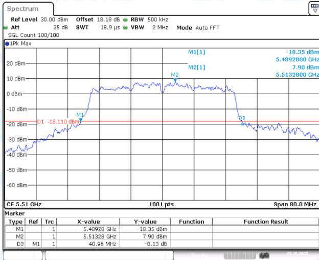
11AC40-CDD-Ant1-5510
