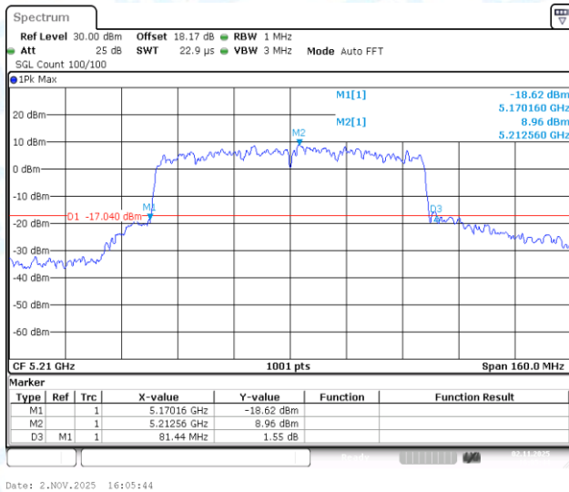
11AC80-CDD-Ant2-5210
