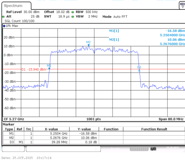
11AX40-CDD-Ant2-5270
