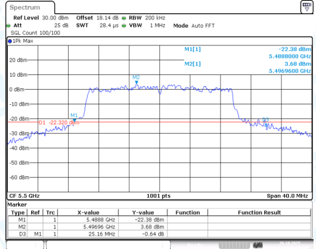
11AX20-CDD-Ant2-5500
