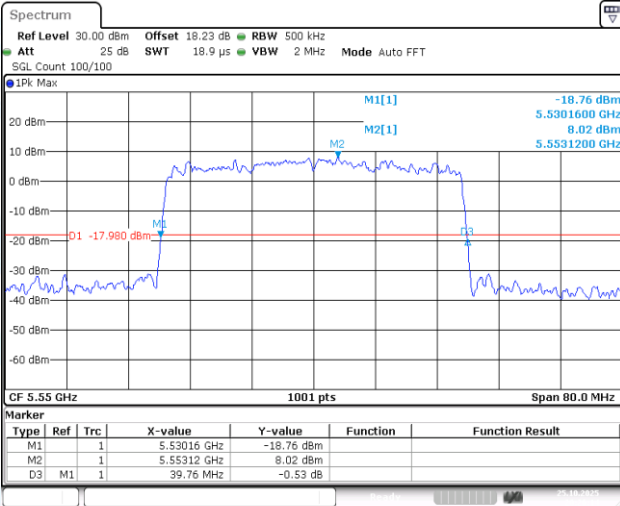
11AX40-CDD-Ant1-5550
