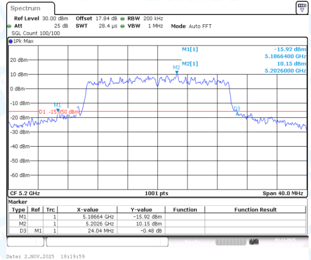
11AX20-CDD-Ant1-5200
