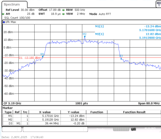
11AC40-CDD-Ant3-5190
