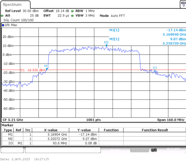
11AX80-CDD-Ant1-5210
