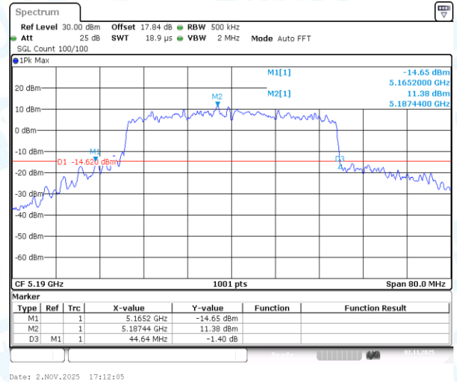
11AX40-CDD-Ant1-5190
