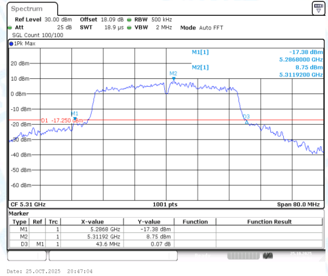
11AC40-CDD-Ant3-5310
