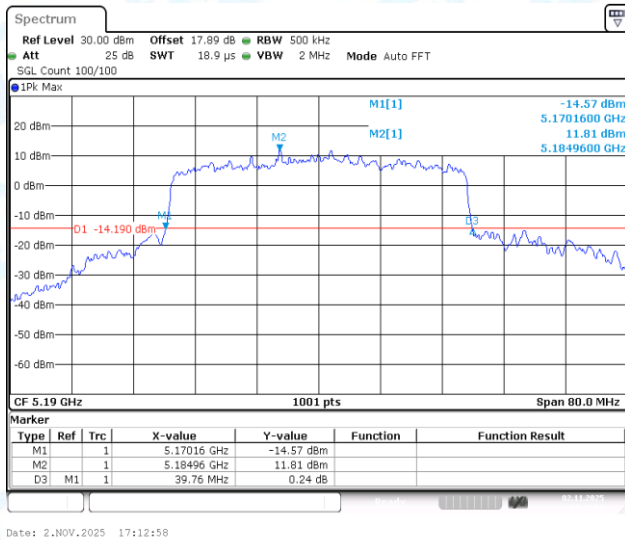
11AX40-CDD-Ant2-5190
