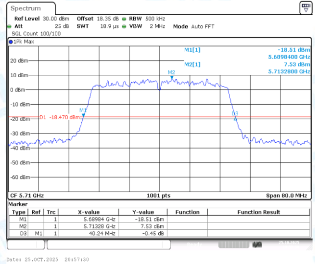
11AC40-CDD-Ant2-5710
