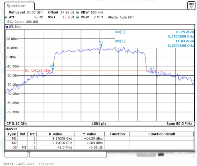
11AX40-CDD-Ant3-5190
