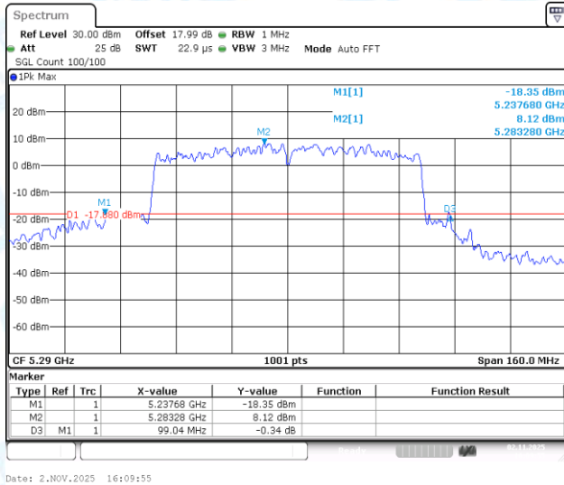
11AC80-CDD-Ant3-5290
