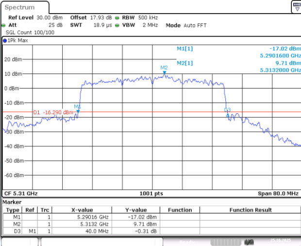
11AX40-CDD-Ant1-5310
