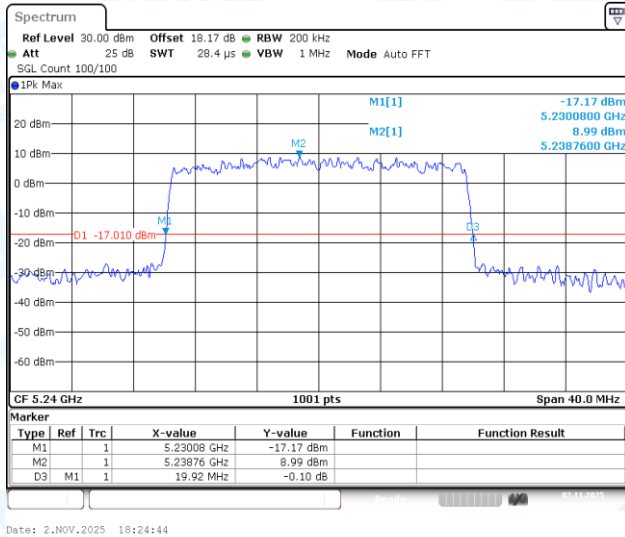
11AX20-CDD-Ant3-5240
