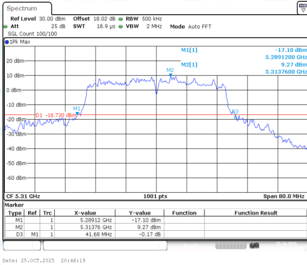
11AC40-CDD-Ant2-5310
