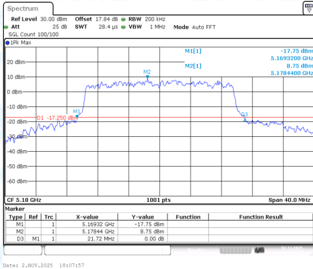
11AX20-CDD-Ant1-5180
