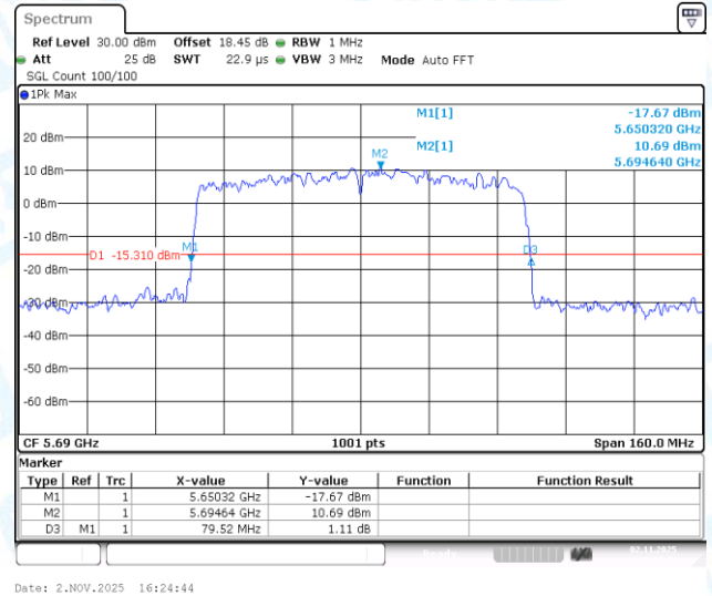
11AC80-CDD-Ant3-5690
