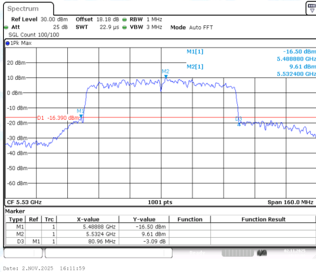
11AC80-CDD-Ant2-5530
