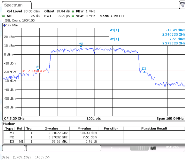
11AC80-CDD-Ant1-5290
