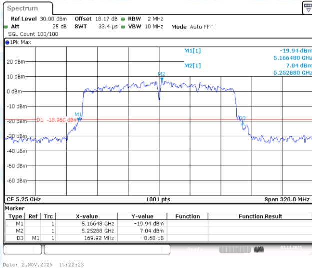
11AC160-CDD-Ant3-5250
