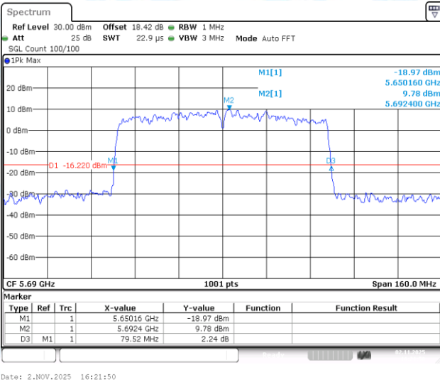
11AC80-CDD-Ant1-5690
