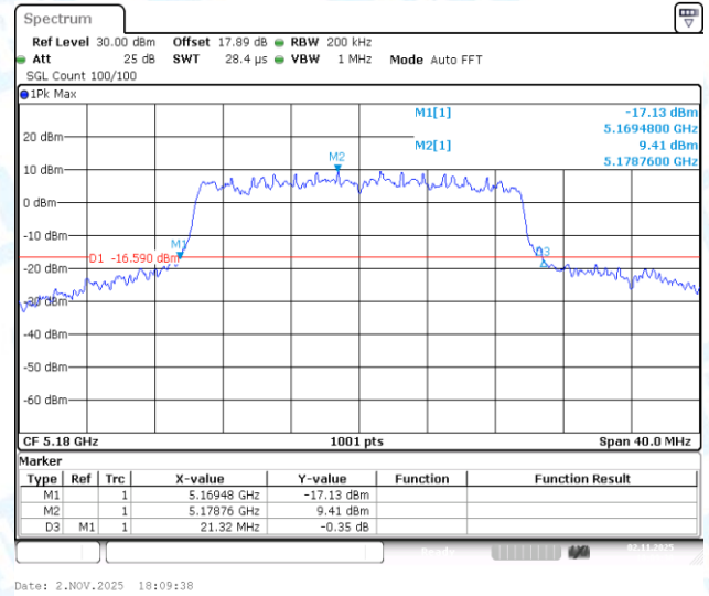
11AX20-CDD-Ant3-5180
