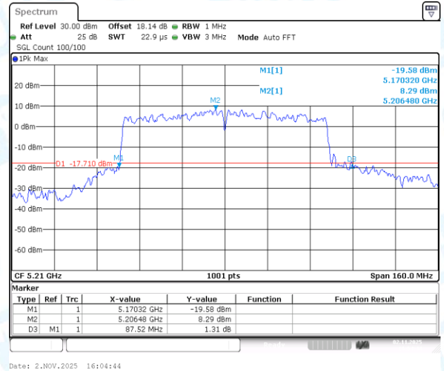
11AC80-CDD-Ant1-5210
