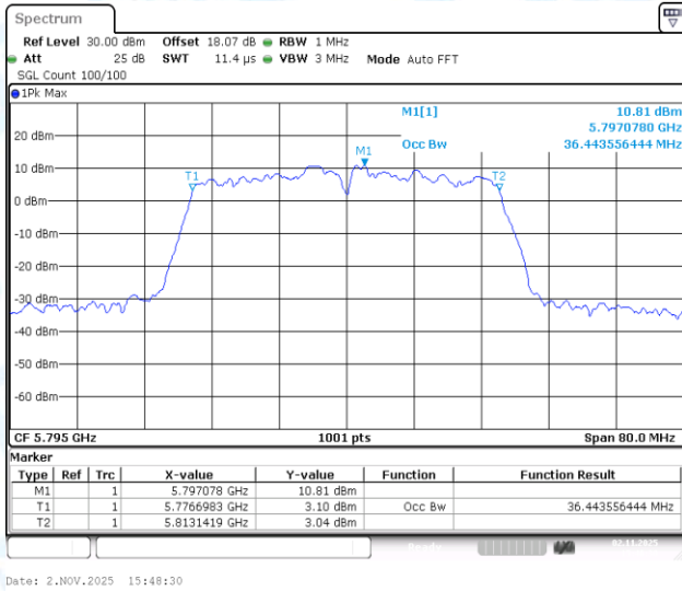
11N40-CDD-Ant1-5795
