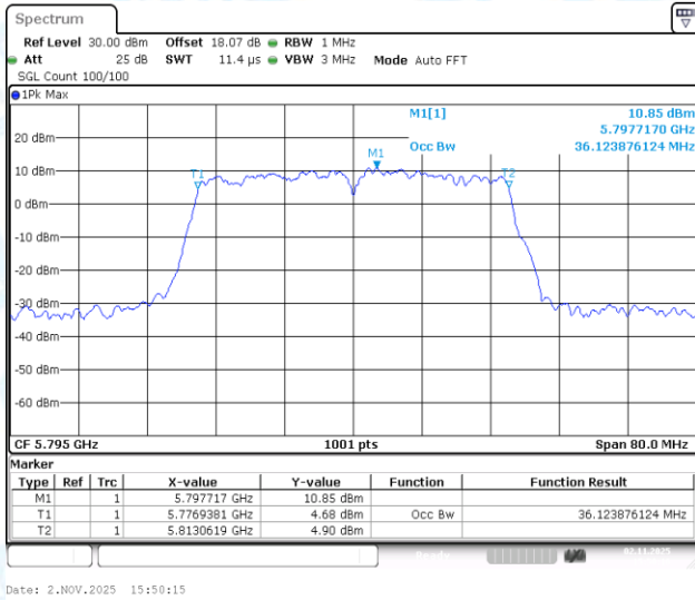
11N40-CDD-Ant3-5795
