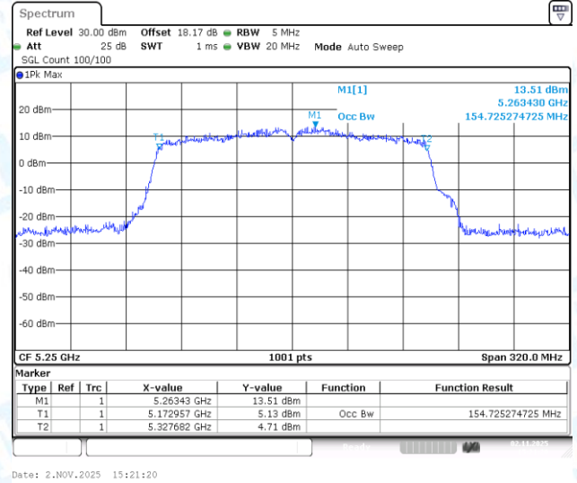
11AC160-CDD-Ant2-5250
