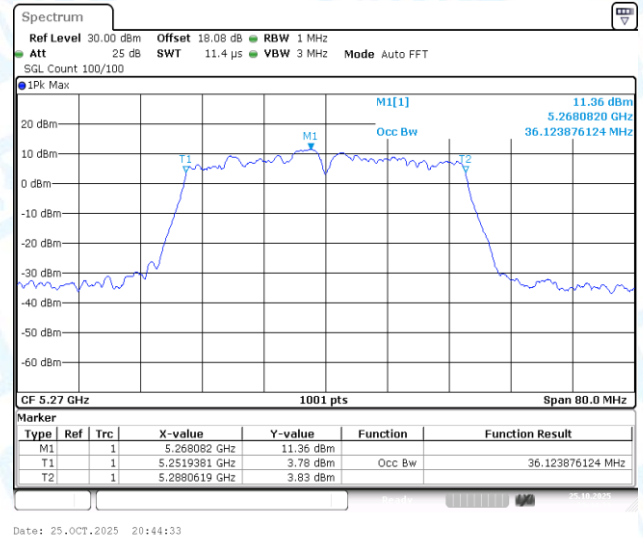
11AC40-CDD-Ant3-5270
