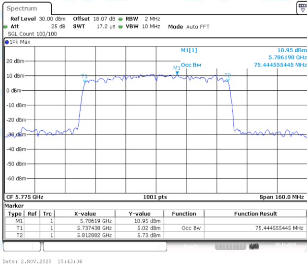
11AC80-CDD-Ant2-5775
