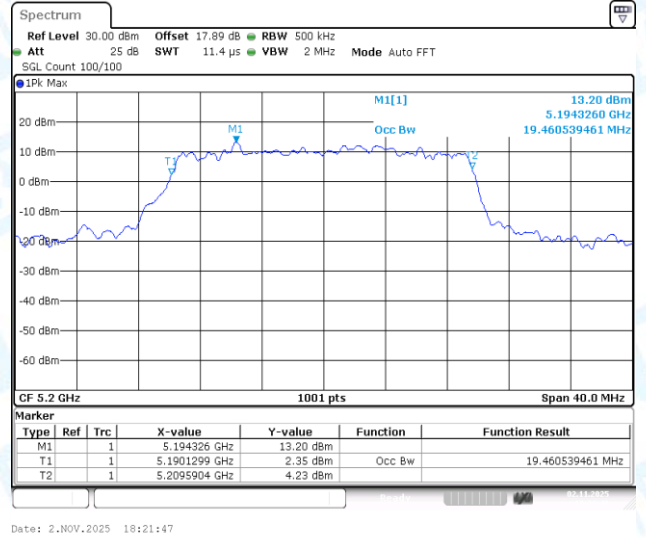
11AX20-CDD-Ant3-5200
