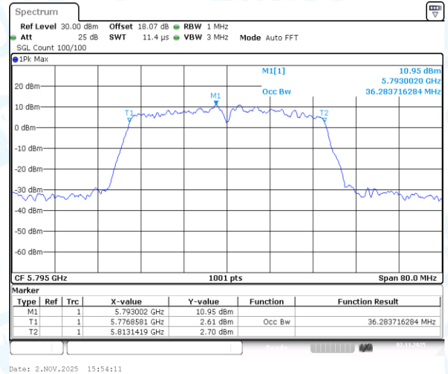
11AC40-CDD-Ant1-5795
