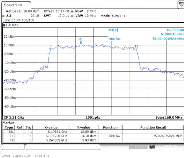
11AC80-CDD-Ant3-5210
