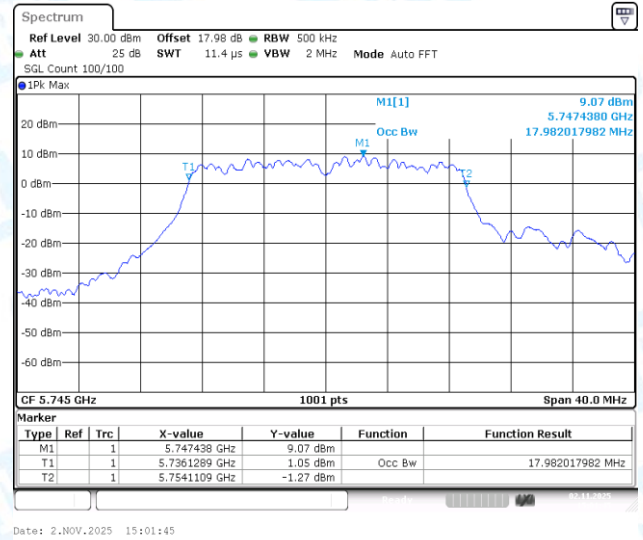
11AC20-CDD-Ant2-5745
