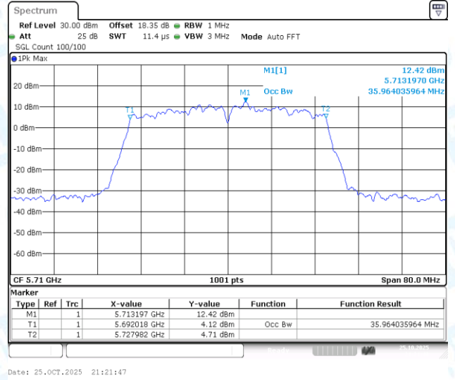
11N40-CDD-Ant2-5710
