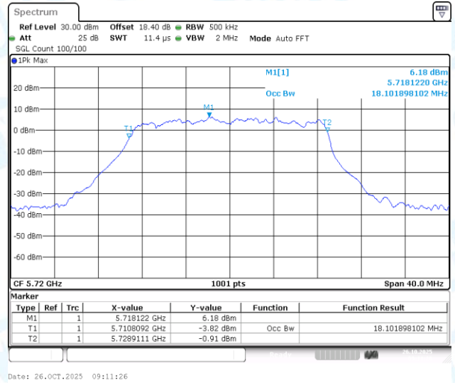
11AC20-CDD-Ant1-5720
