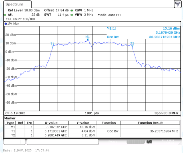
11AC40-CDD-Ant1-5190
