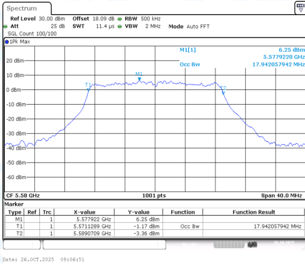
11AC20-CDD-Ant1-5580
