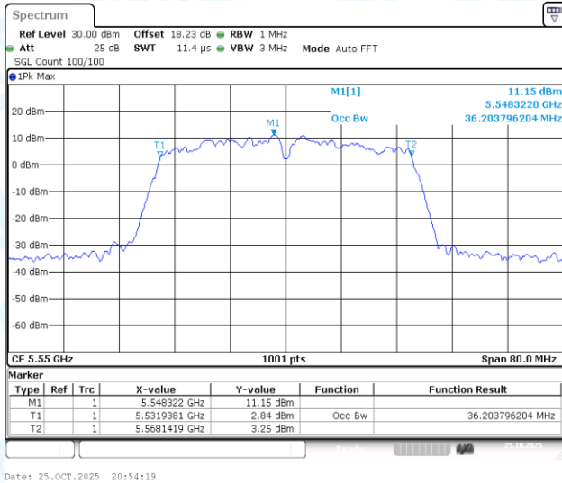
11AC40-CDD-Ant3-5550
