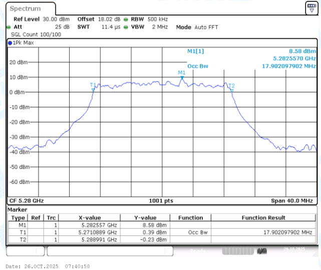
11AC20-CDD-Ant2-5280
