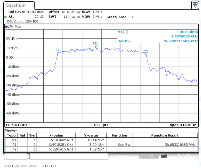
11AC40-CDD-Ant3-5510
