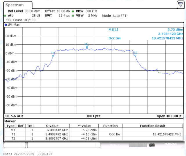
11AC20-CDD-Ant1-5500
