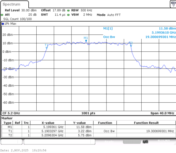
11AX20-CDD-Ant2-5200
