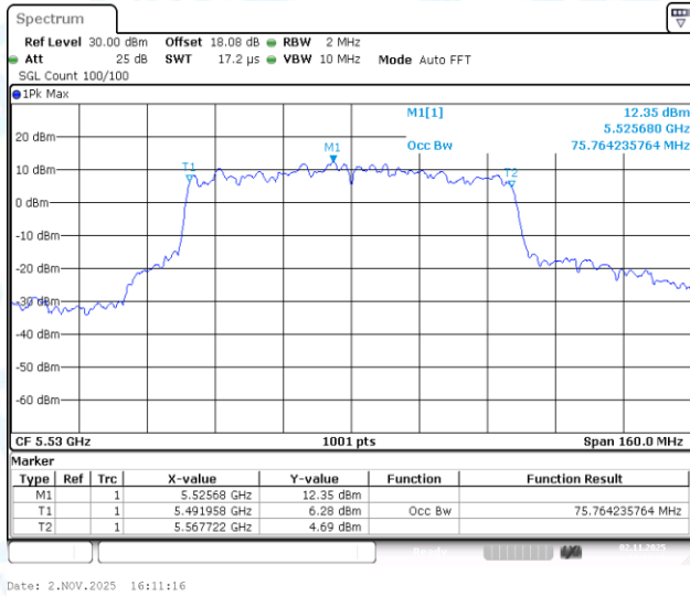
11AC80-CDD-Ant1-5530
