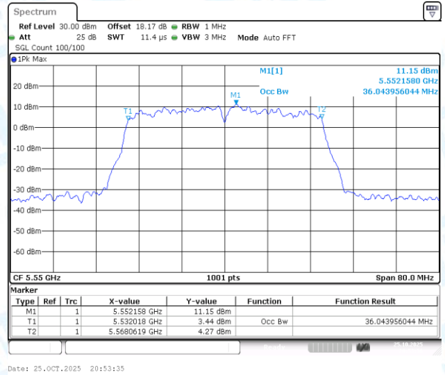
11AC40-CDD-Ant2-5550
