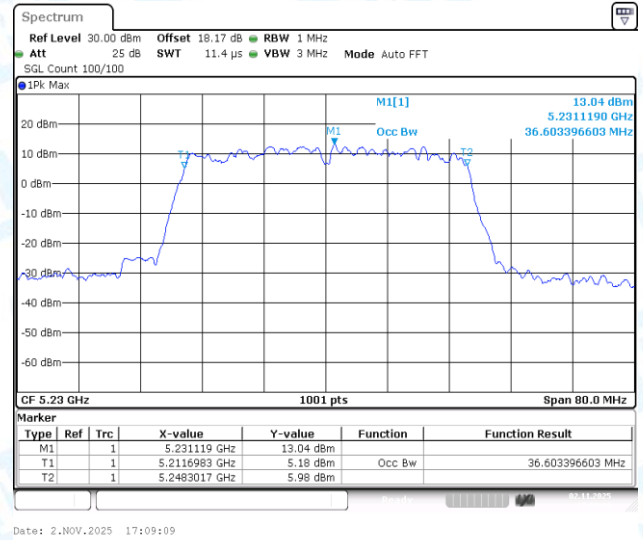
11AC40-CDD-Ant2-5230
