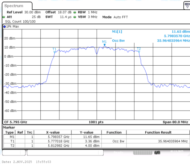
11AC40-CDD-Ant2-5795
