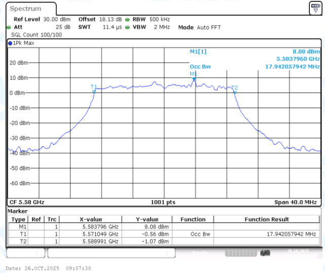
11AC20-CDD-Ant2-5580
