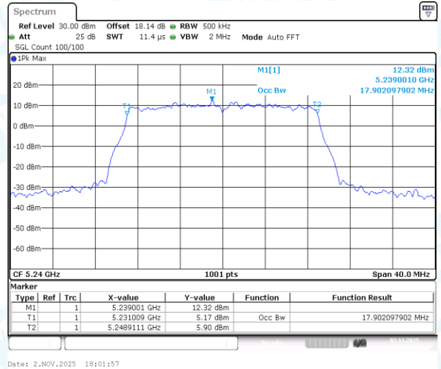
11AC20-CDD-Ant1-5240
