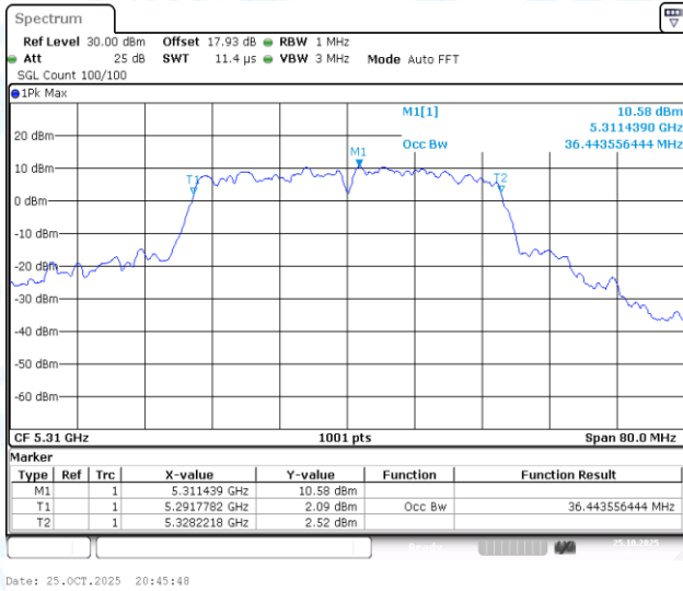
11AC40-CDD-Ant1-5310
