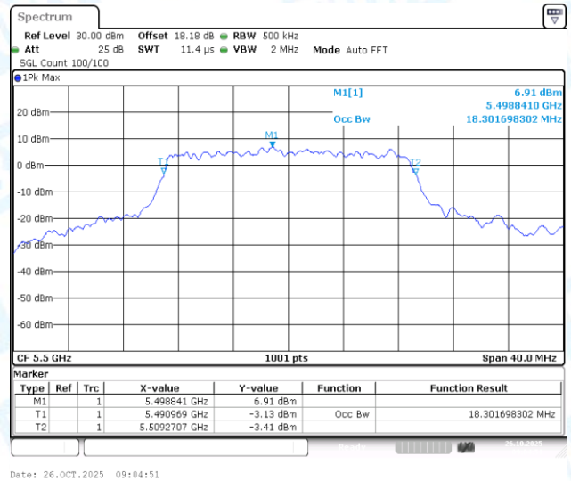
11AC20-CDD-Ant3-5500
