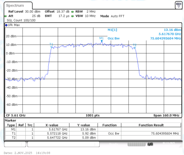
11AC80-CDD-Ant2-5610
