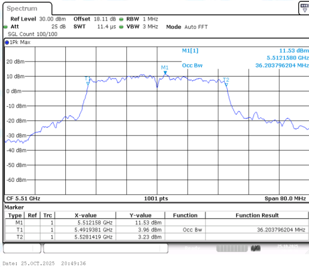
11AC40-CDD-Ant2-5510
