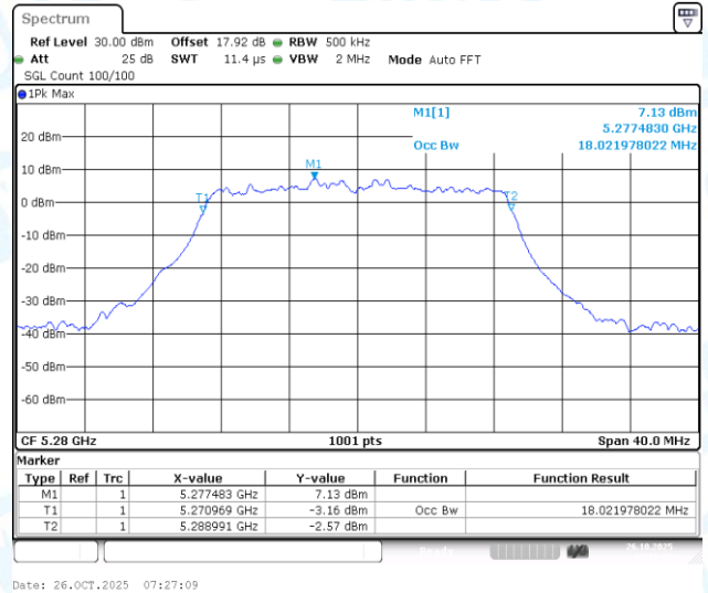
11AC20-CDD-Ant1-5280
