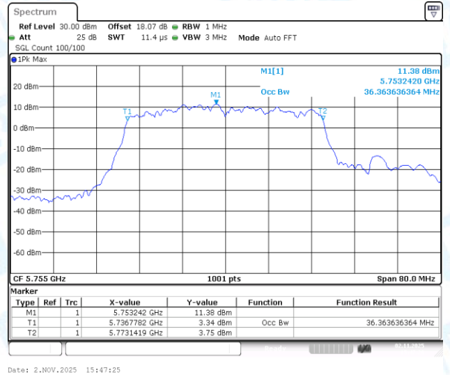
11N40-CDD-Ant3-5755
