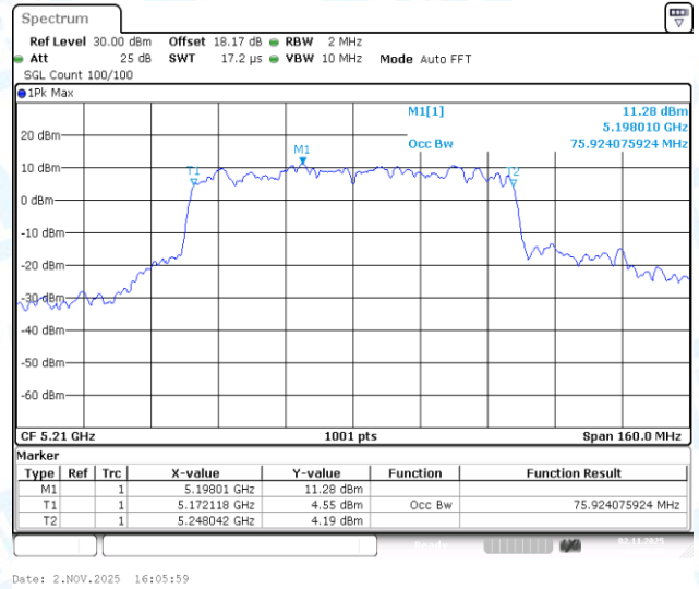
11AC80-CDD-Ant2-5210
