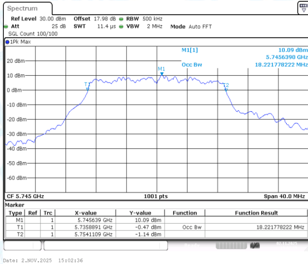
11AC20-CDD-Ant3-5745
