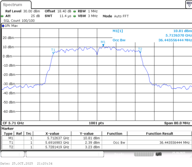
11N40-CDD-Ant1-5710
