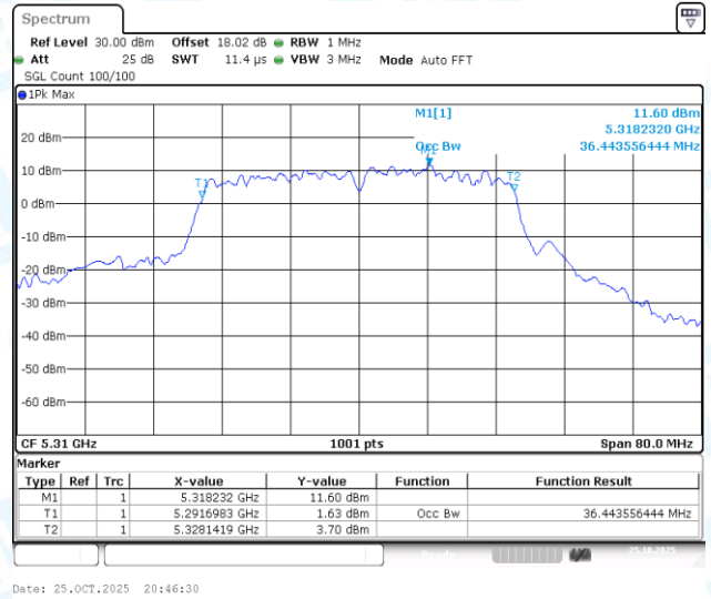
11AC40-CDD-Ant2-5310
