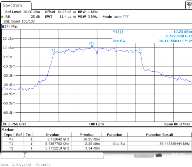
11N40-CDD-Ant2-5755
