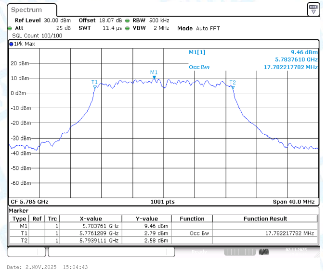
11AC20-CDD-Ant2-5785
