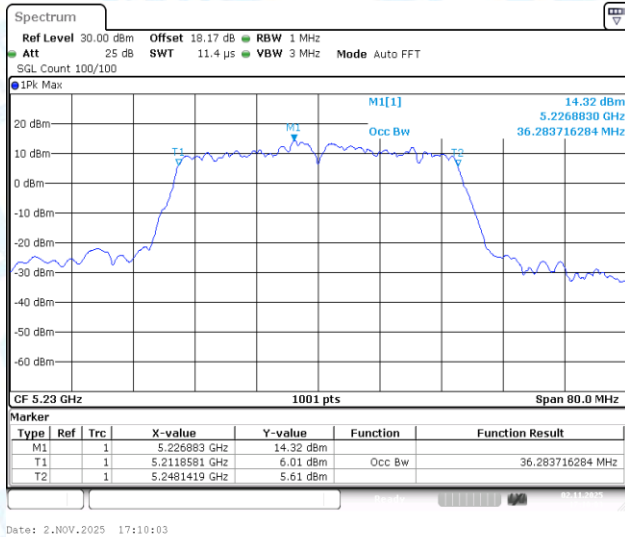
11AC40-CDD-Ant3-5230
