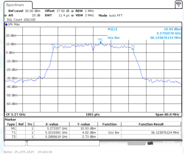
11AC40-CDD-Ant1-5270
