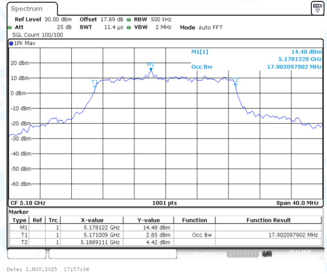
11AC20-CDD-Ant3-5180
