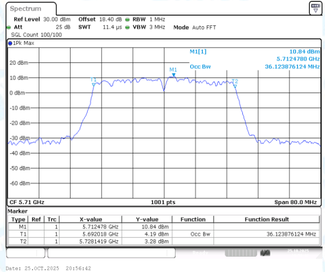
11AC40-CDD-Ant1-5710
