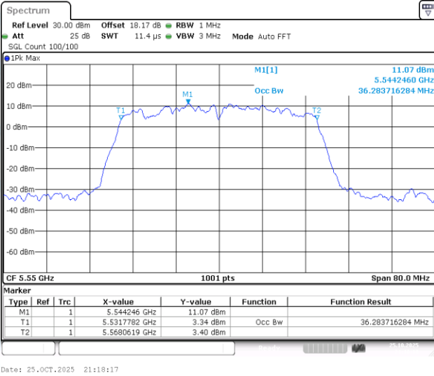
11N40-CDD-Ant2-5550
