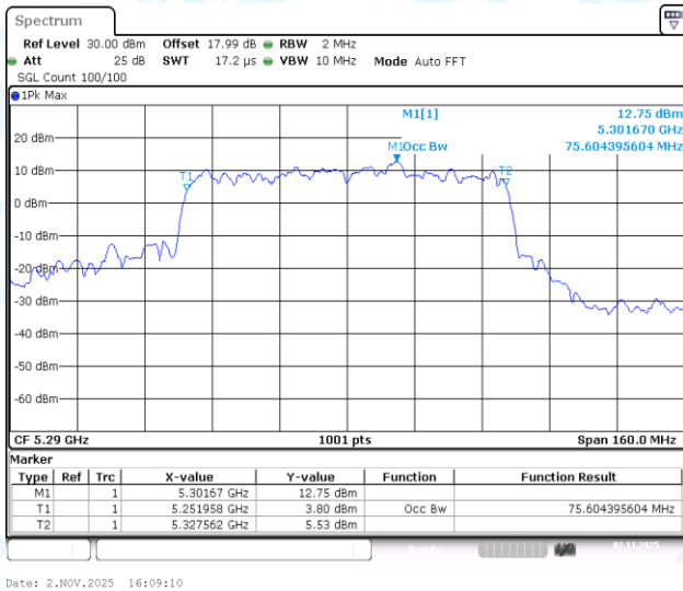
11AC80-CDD-Ant2-5290
