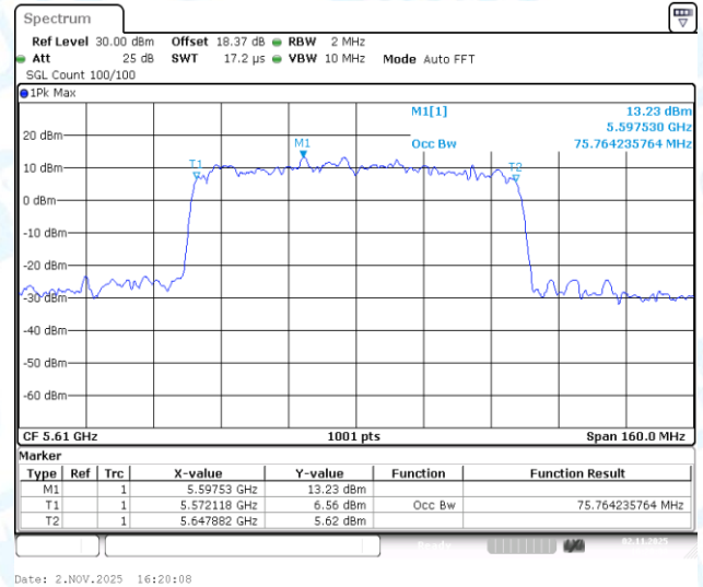
11AC80-CDD-Ant3-5610
