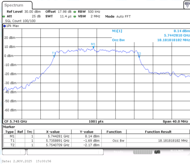
11AC20-CDD-Ant1-5745
