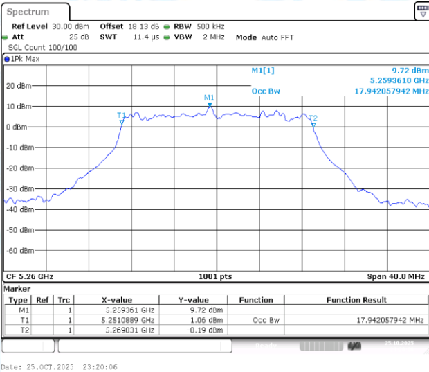
11AC20-CDD-Ant3-5260
