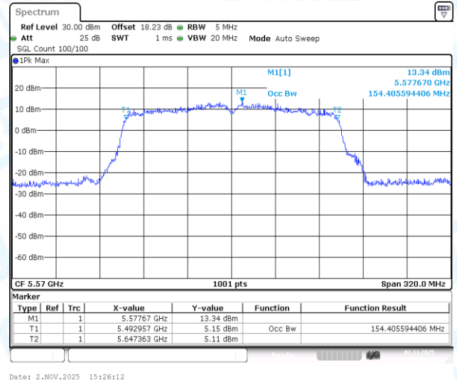
11AC160-CDD-Ant3-5570
