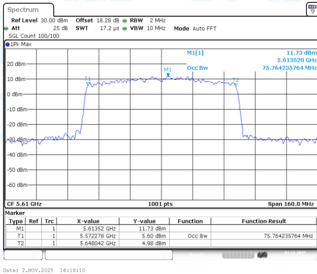
11AC80-CDD-Ant1-5610
