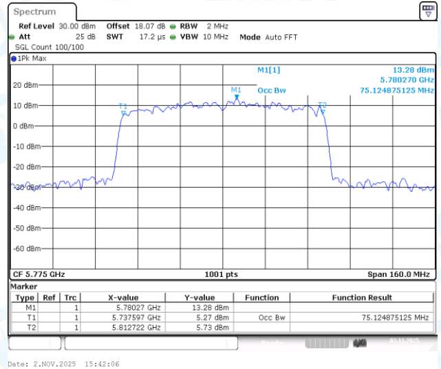
11AC80-CDD-Ant1-5775
