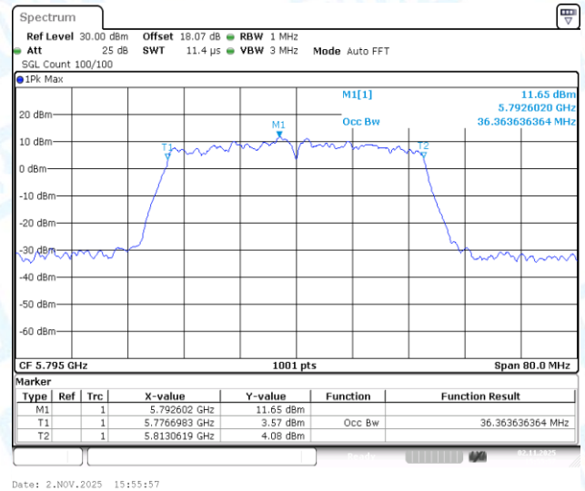
11AC40-CDD-Ant3-5795
