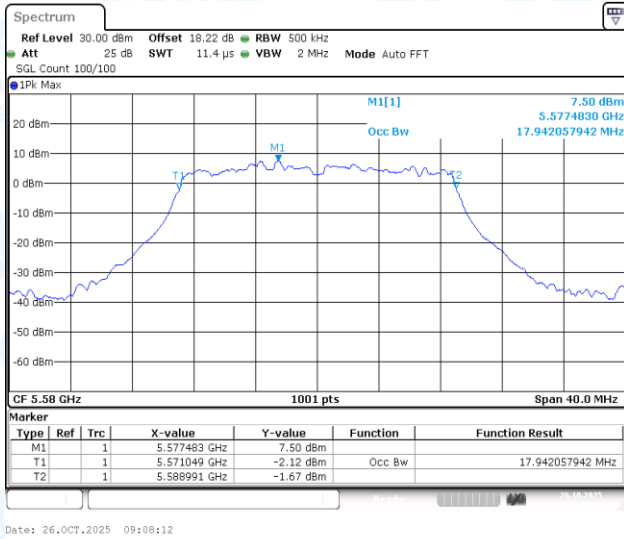
11AC20-CDD-Ant3-5580
