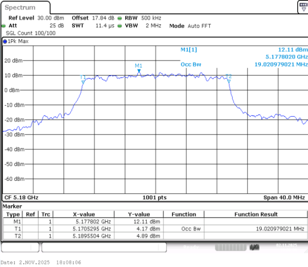
11AX20-CDD-Ant1-5180
