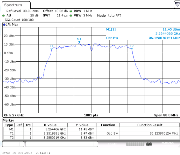
11AC40-CDD-Ant2-5270
