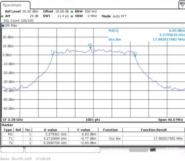
11AC20-CDD-Ant3-5280
