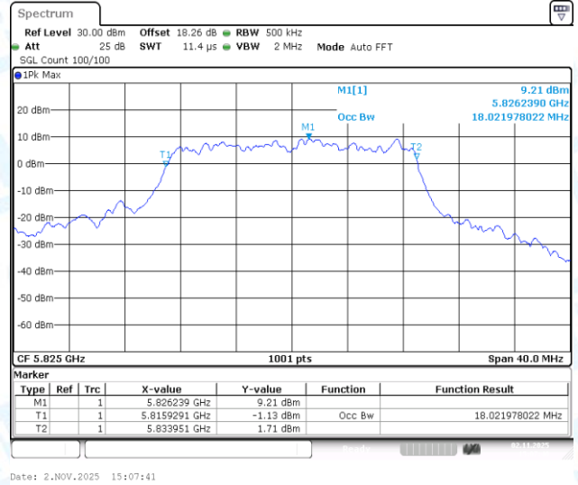
11AC20-CDD-Ant2-5825
