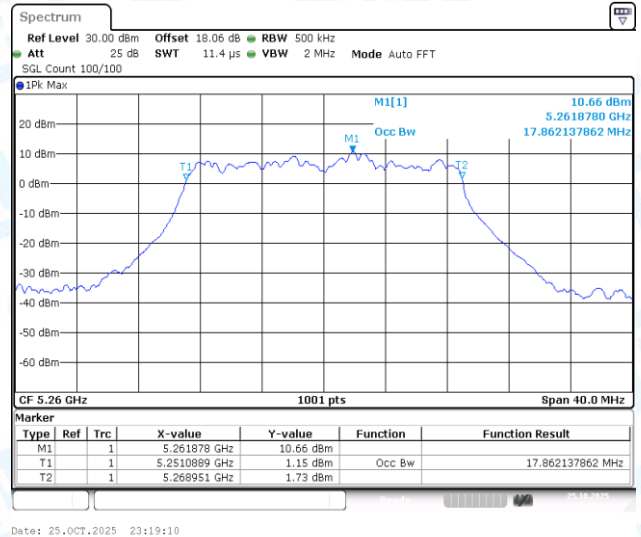
11AC20-CDD-Ant2-5260
