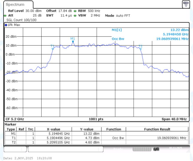
11AX20-CDD-Ant1-5200
