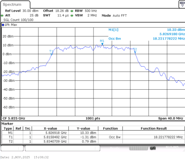
11AC20-CDD-Ant3-5825
