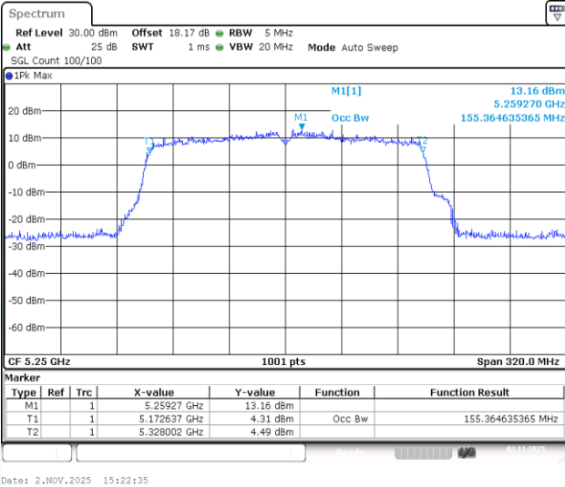
11AC160-CDD-Ant3-5250
