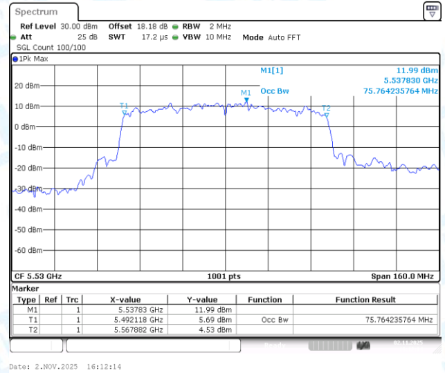
11AC80-CDD-Ant2-5530
