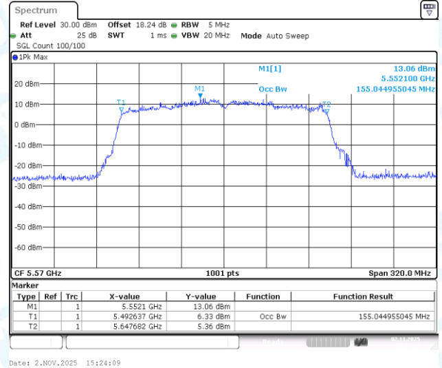
11AC160-CDD-Ant1-5570
