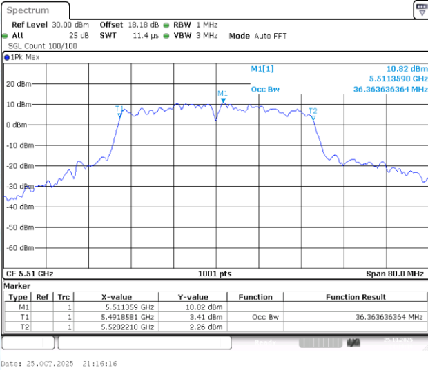
11N40-CDD-Ant3-5510
