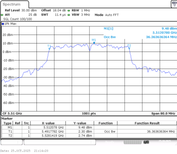
11N40-CDD-Ant1-5510
