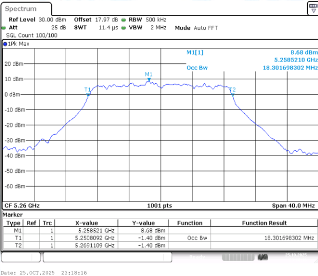
11AC20-CDD-Ant1-5260
