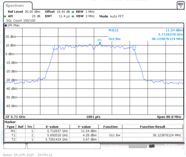
11AC40-CDD-Ant3-5710
