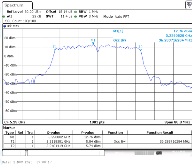
11AC40-CDD-Ant1-5230
