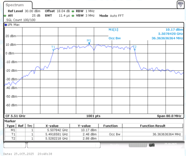
11AC40-CDD-Ant1-5510
