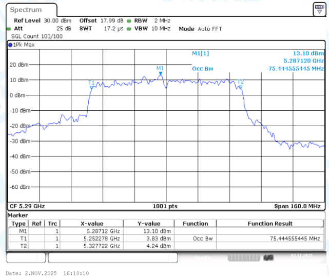
11AC80-CDD-Ant3-5290
