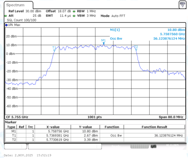
11AC40-CDD-Ant2-5755
