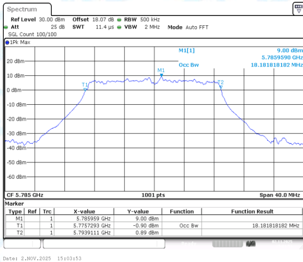
11AC20-CDD-Ant1-5785
