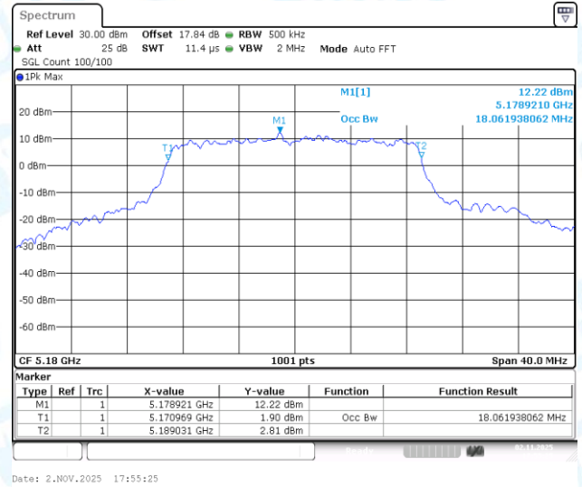
11AC20-CDD-Ant1-5180
