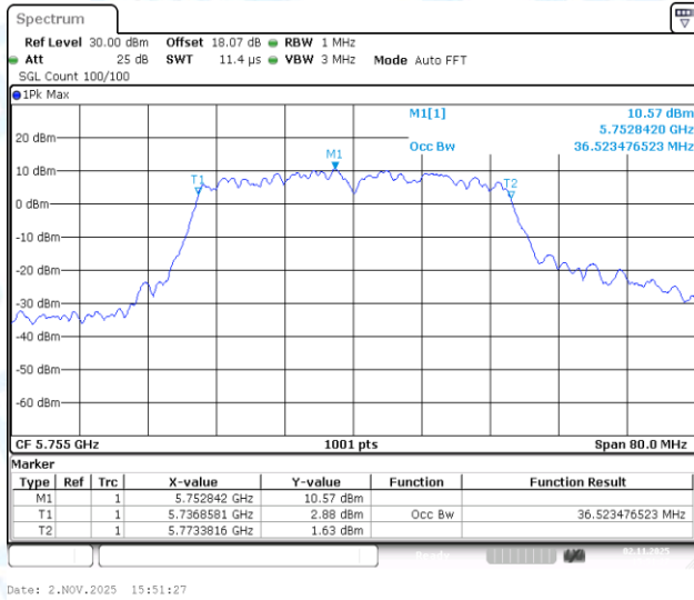
11AC40-CDD-Ant1-5755
