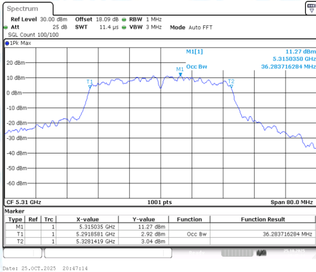
11AC40-CDD-Ant3-5310
