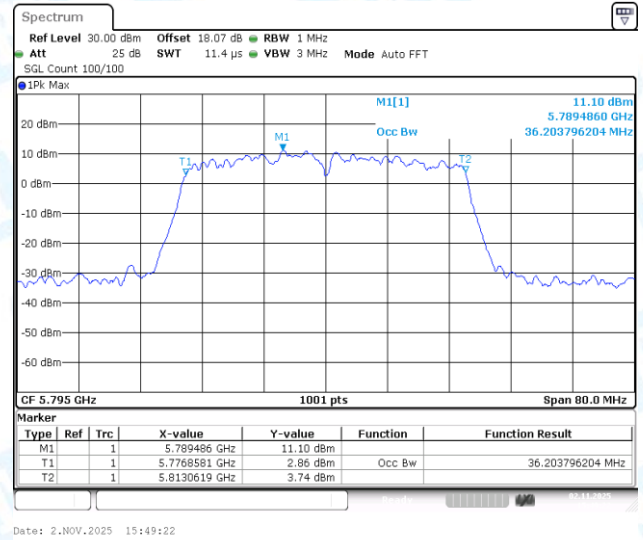
11N40-CDD-Ant2-5795
