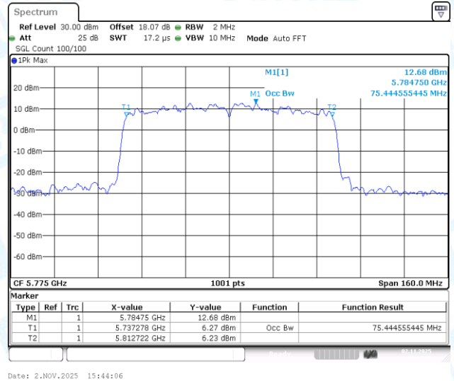
11AC80-CDD-Ant3-5775
