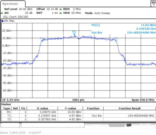
11AC160-CDD-Ant1-5250
