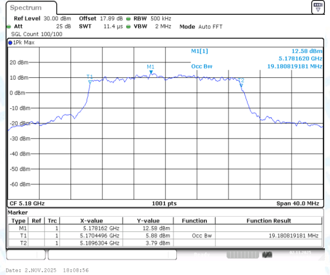
11AX20-CDD-Ant2-5180
