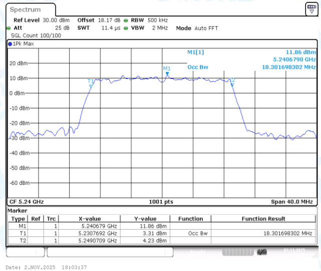
11AC20-CDD-Ant3-5240
