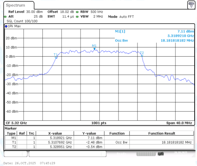
11AC20-CDD-Ant2-5320
