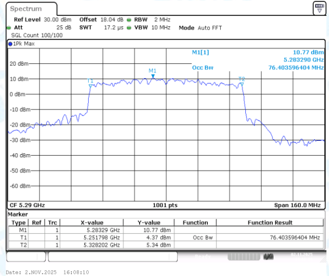
11AC80-CDD-Ant1-5290
