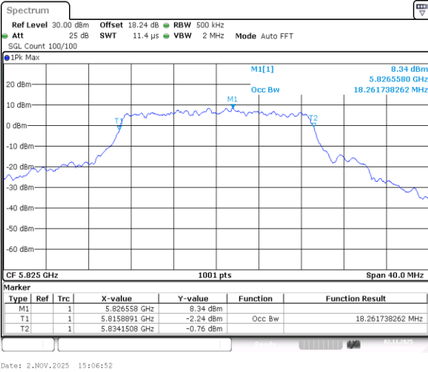
11AC20-CDD-Ant1-5825
