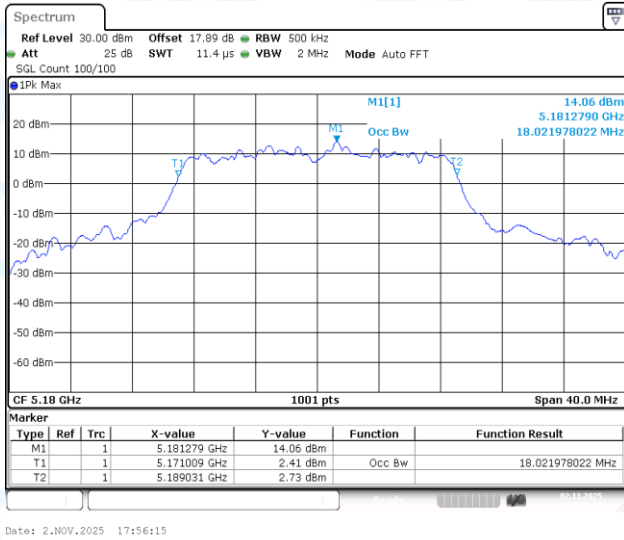
11AC20-CDD-Ant2-5180
