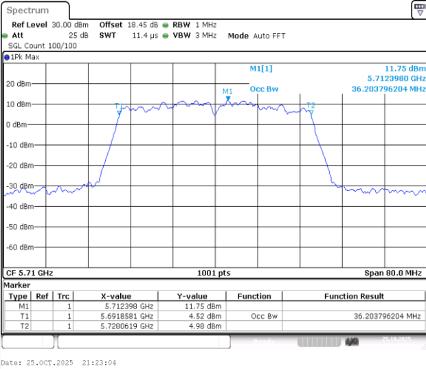
11N40-CDD-Ant3-5710
