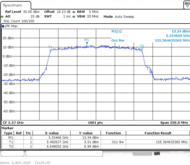
11AC160-CDD-Ant2-5570
