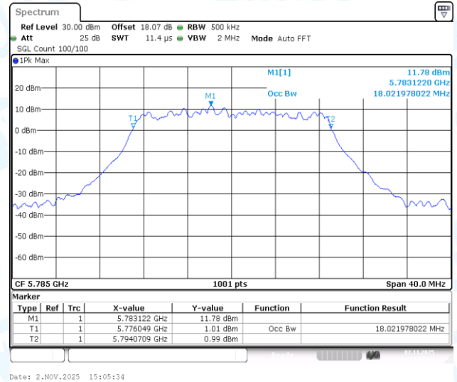
11AC20-CDD-Ant3-5785
