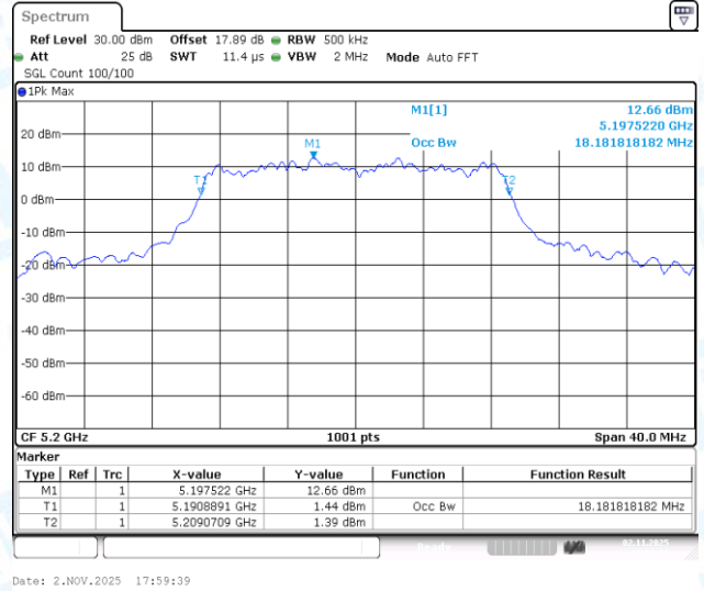
11AC20-CDD-Ant2-5200
