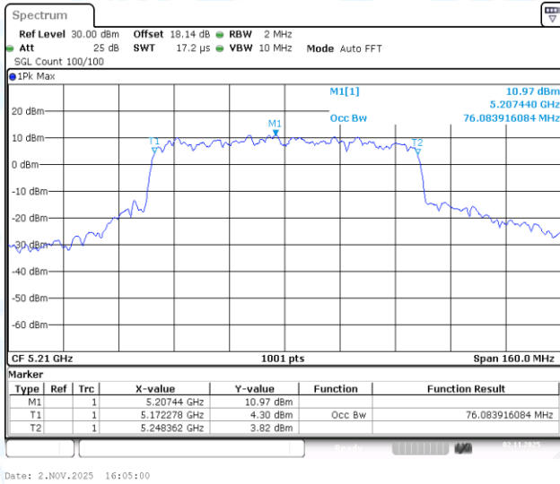
11AC80-CDD-Ant1-5210
