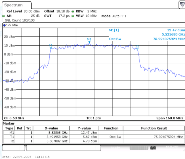
11AC80-CDD-Ant3-5530
