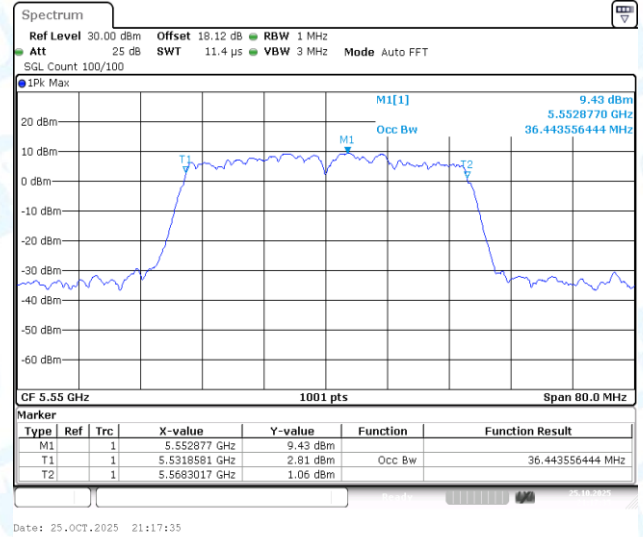
11N40-CDD-Ant1-5550
