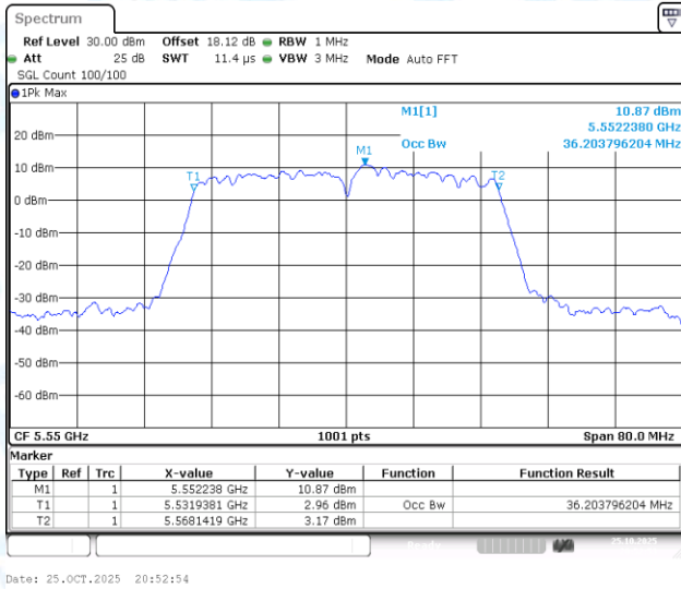
11AC40-CDD-Ant1-5550
