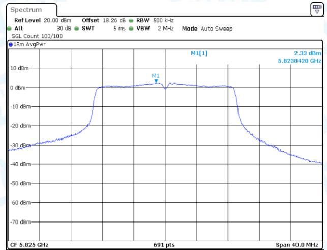
11N20-CDD-Ant1-5825-PASS
