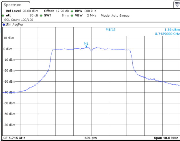
11AC20-CDD-Ant1-5745-PASS
