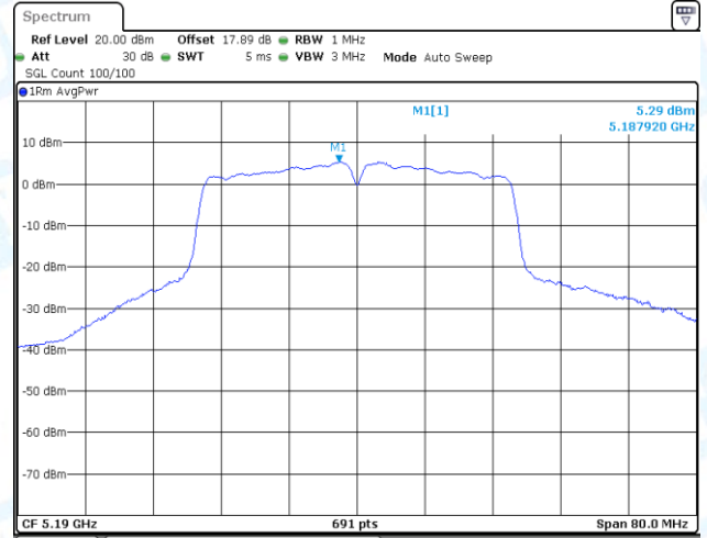
11N40-CDD-Ant2-5190-PASS
