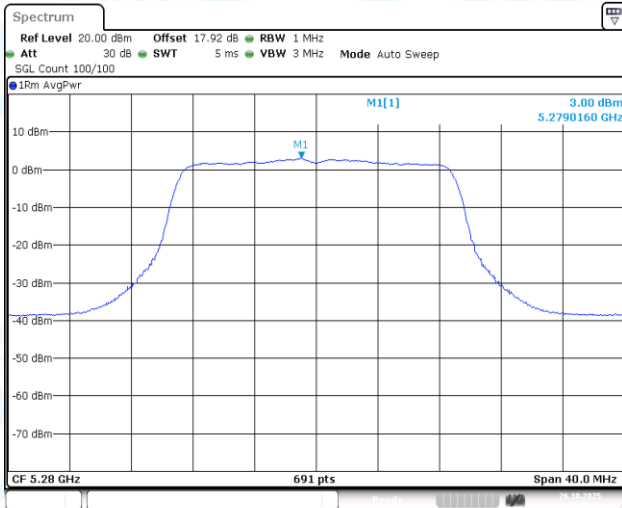
11AC20-CDD-Ant1-5280-PASS
