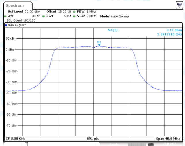
11AC20-CDD-Ant1-5580-PASS
