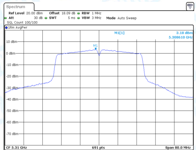
11N40-CDD-Ant1-5310-PASS
