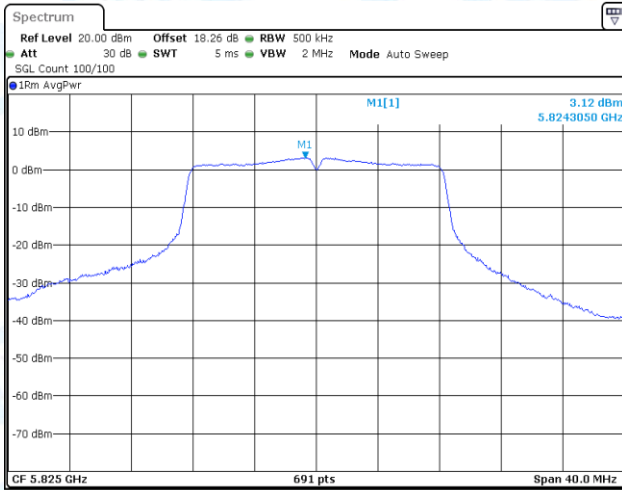
11A-CDD-Ant3-5825-PASS
