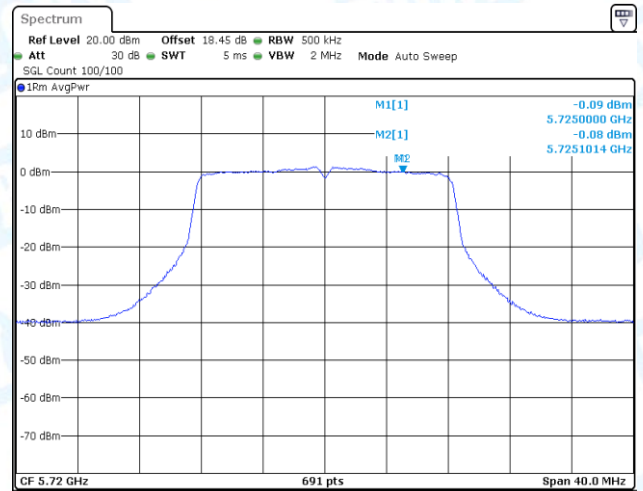
11A-CDD-Ant1-5720_UNII-3-PASS
