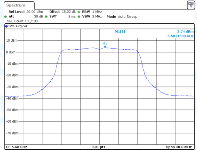
11A-CDD-Ant1-5580-PASS
