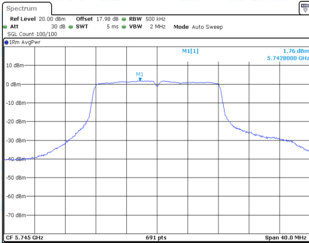
11A-CDD-Ant1-5745-PASS
