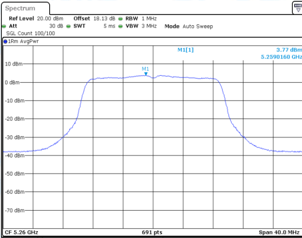
11N20-CDD-Ant1-5260-PASS
