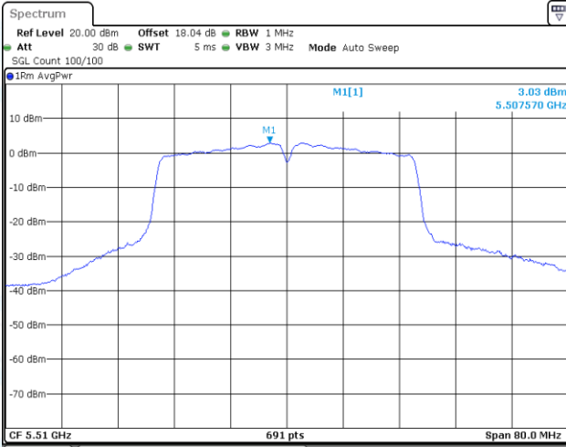
11N40-CDD-Ant1-5510-PASS
