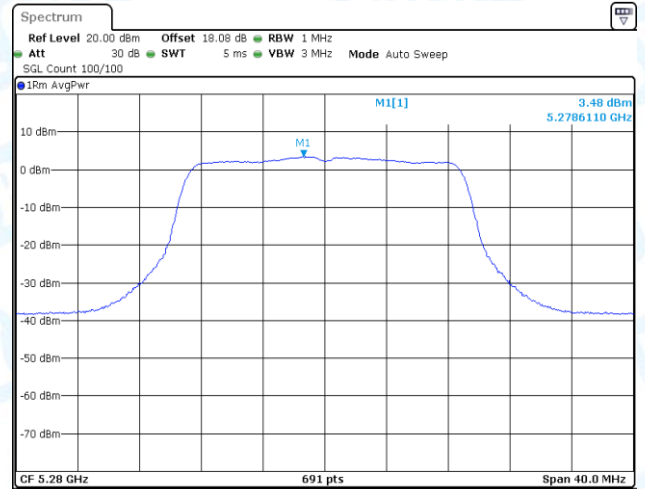
11N20-CDD-Ant1-5280-PASS
