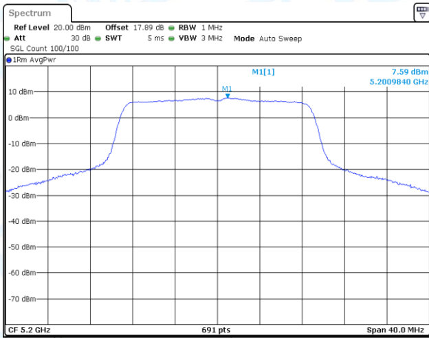
11N20-CDD-Ant1-5200-PASS
