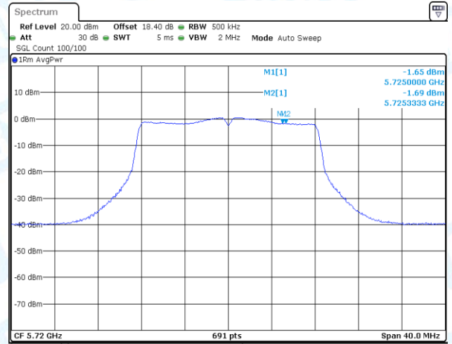
11A-CDD-Ant2-5720_UNII-2C-PASS
