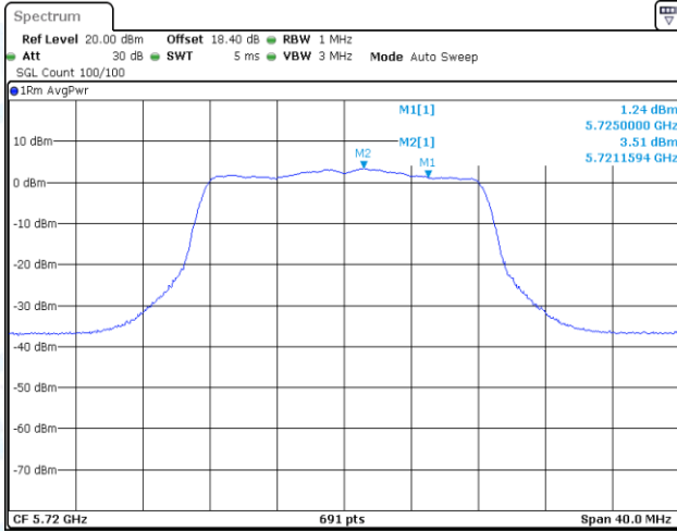
11A-CDD-Ant1-5720_UNII-2C-PASS
