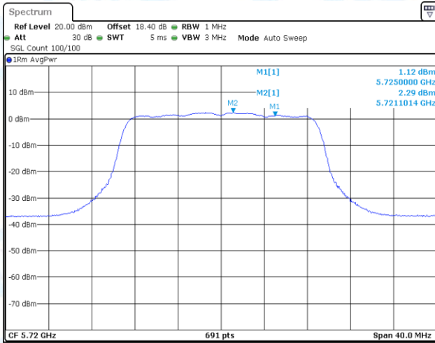
11AC20-CDD-Ant1-5720_UNII-2C-PASS
