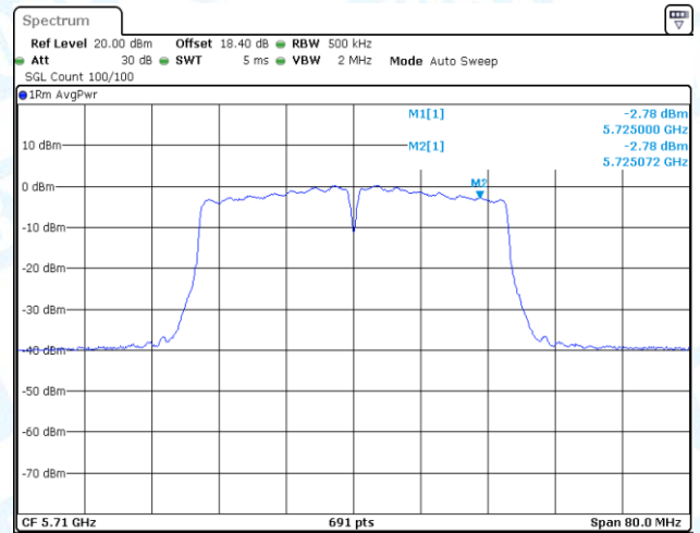
11N40-CDD-Ant2-5710_UNII-2C-PASS
