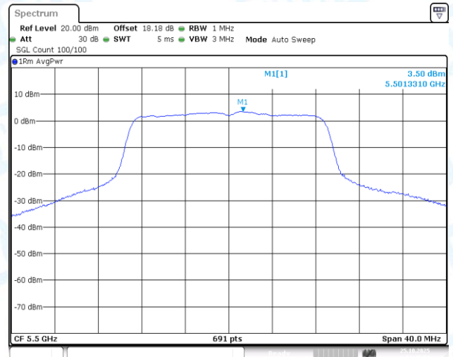
11N20-CDD-Ant1-5500-PASS
