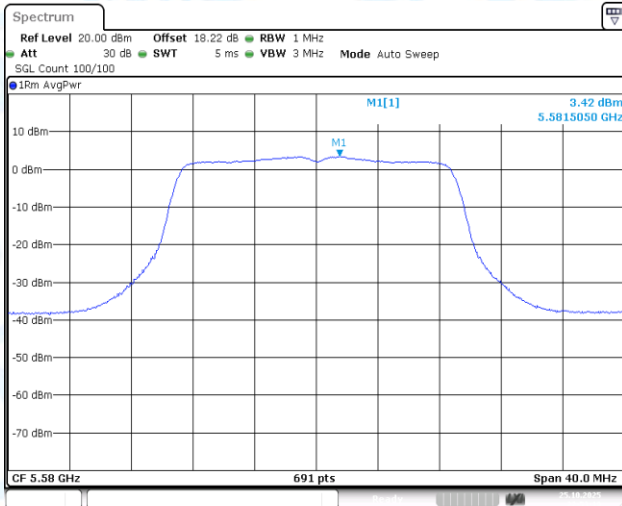
11N20-CDD-Ant1-5580-PASS
