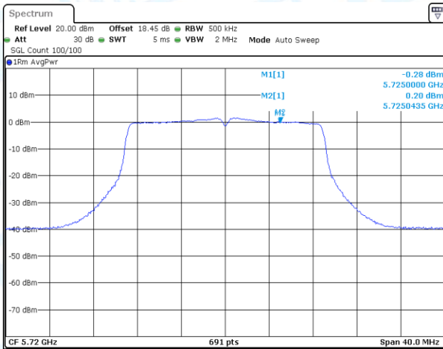
11N20-CDD-Ant1-5720_UNII-3-PASS
