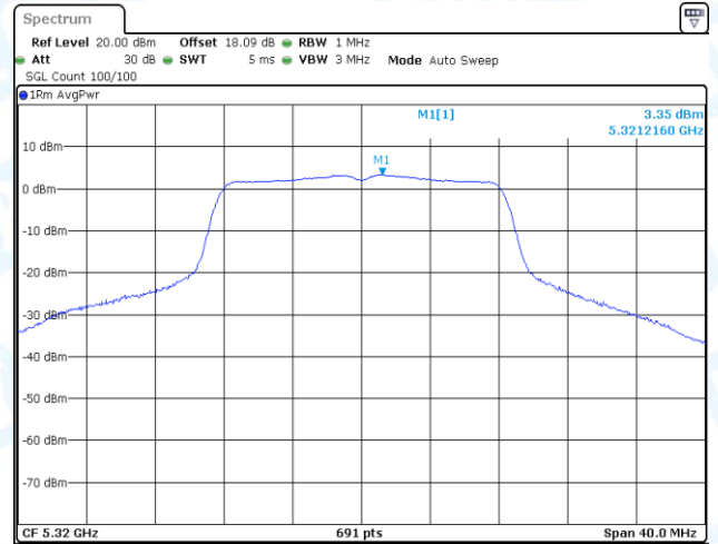
11A-CDD-Ant1-5320-PASS
