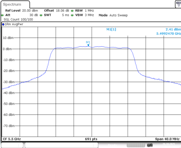
11AC20-CDD-Ant1-5500-PASS
