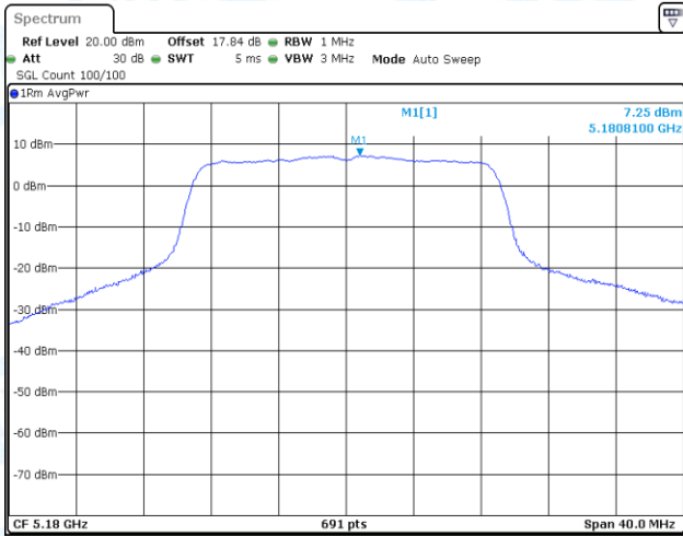
11AC20-CDD-Ant1-5180-PASS
