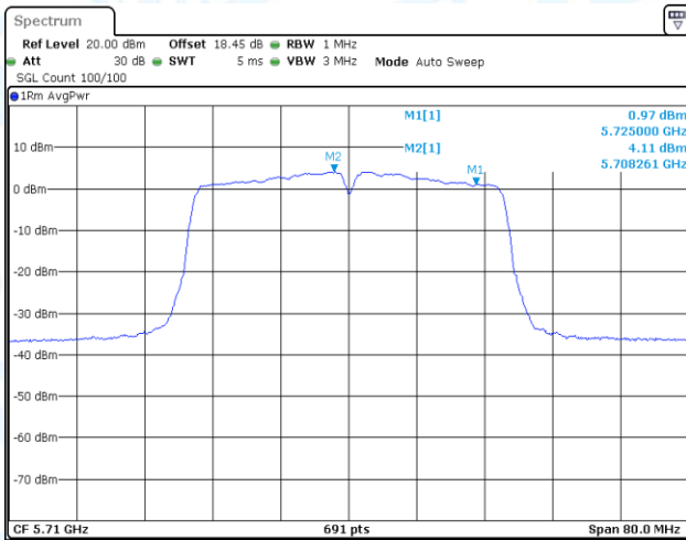
11N40-CDD-Ant1-5710_UNII-2C-PASS
