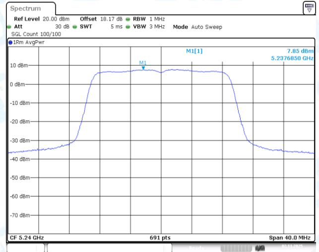
11AC20-CDD-Ant2-5240-PASS
