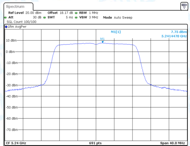
11N20-CDD-Ant1-5240-PASS
