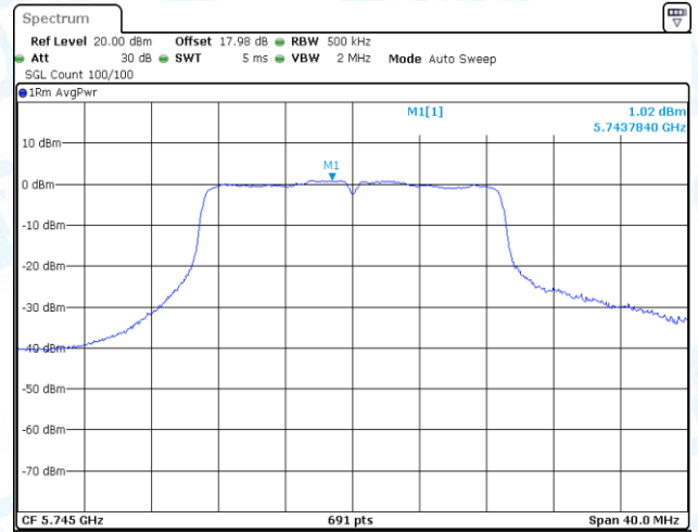
11AC20-CDD-Ant2-5745-PASS
