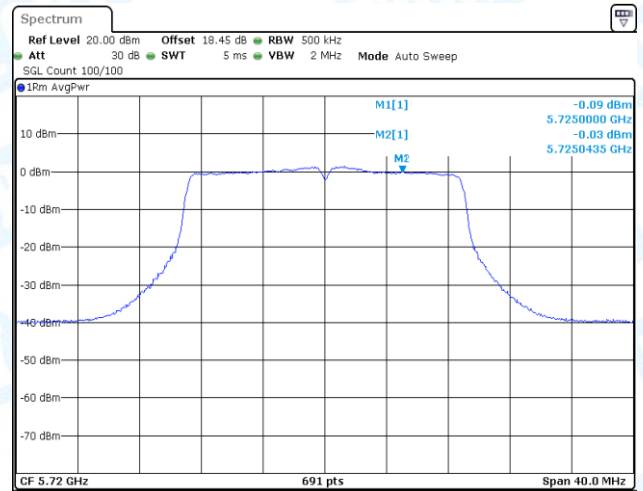
11AC20-CDD-Ant1-5720_UNII-3-PASS
