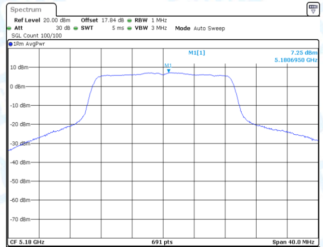
11N20-CDD-Ant2-5180-PASS
