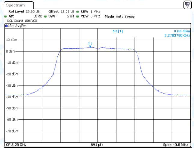
11A-CDD-Ant2-5280-PASS
