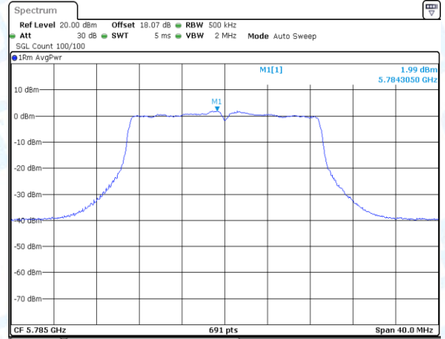
11N20-CDD-Ant1-5785-PASS
