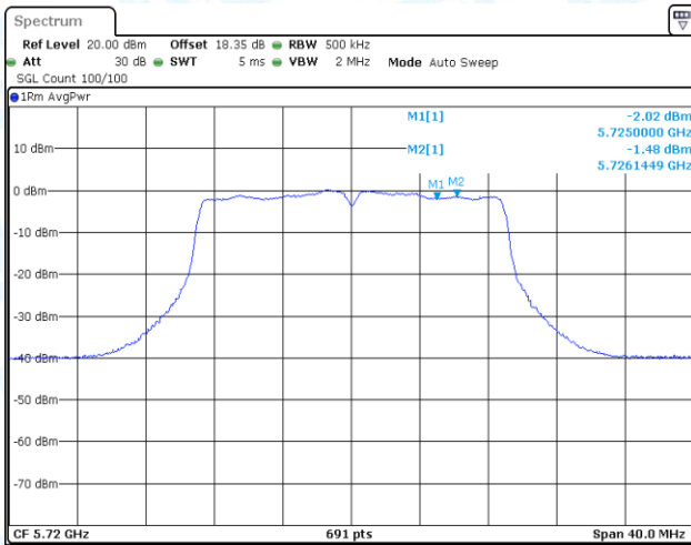
11AC20-CDD-Ant3-5720_UNII-2C-PASS
