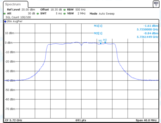
11N20-CDD-Ant2-5720_UNII-3-PASS
