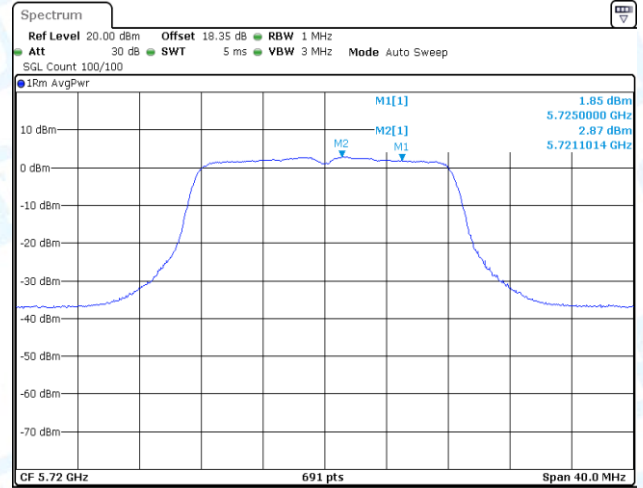
11A-CDD-Ant2-5720_UNII-2C-PASS
