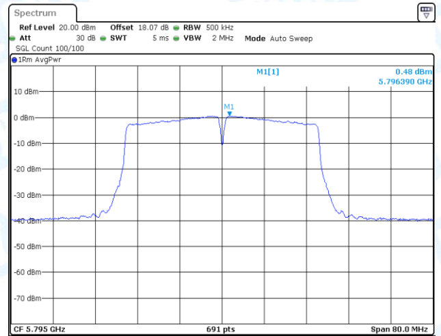
11N40-CDD-Ant1-5795-PASS
