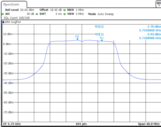
11A-CDD-Ant1-5720_UNII-2C-PASS
