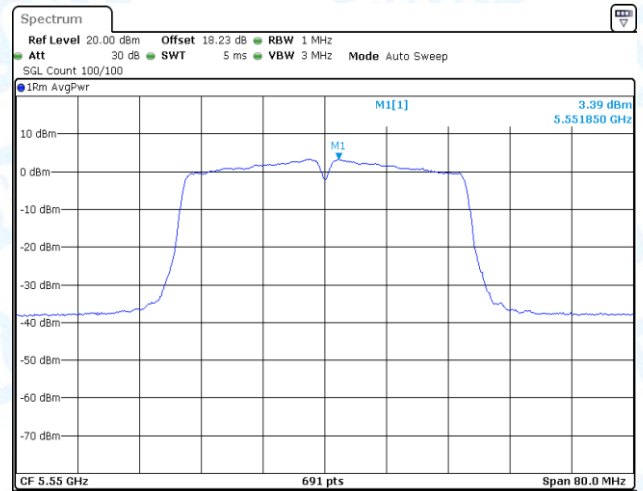
11N40-CDD-Ant1-5550-PASS
