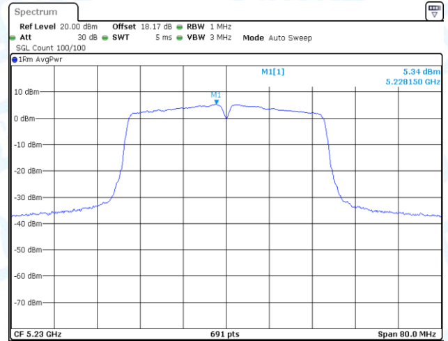
11N40-CDD-Ant1-5230-PASS
