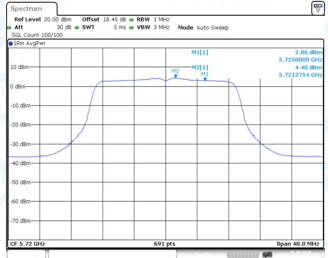
11N20-CDD-Ant1-5720_UNII-2C-PASS
