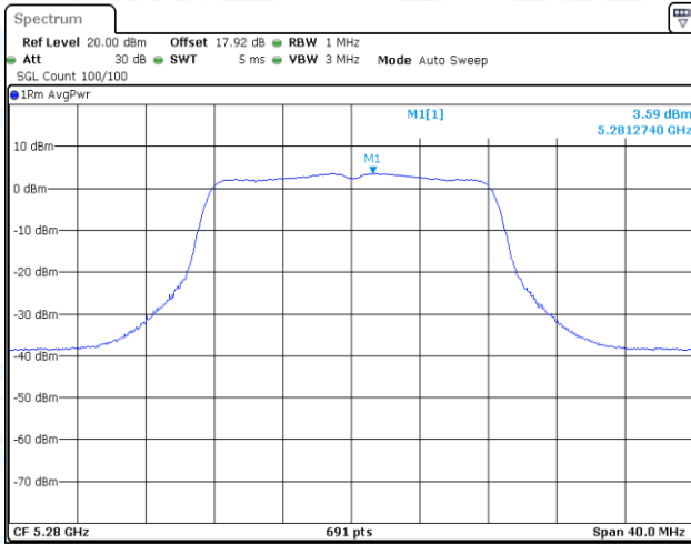
11A-CDD-Ant1-5280-PASS
