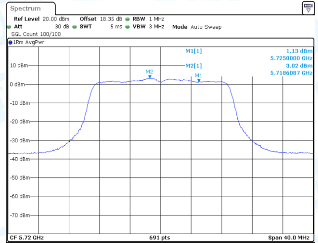
11AC20-CDD-Ant2-5720_UNII-2C-PASS
