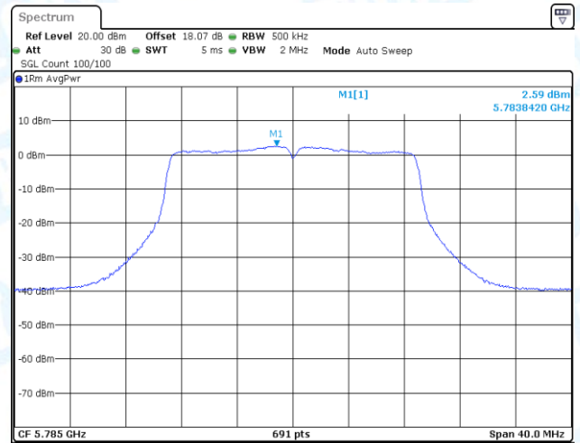
11AC20-CDD-Ant1-5785-PASS
