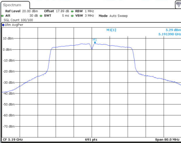
11N40-CDD-Ant1-5190-PASS
