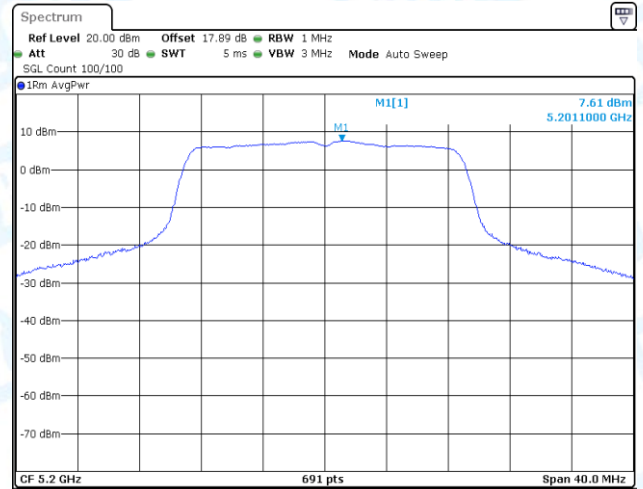
11AC20-CDD-Ant1-5200-PASS
