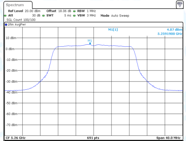
11N20-CDD-Ant2-5260-PASS
