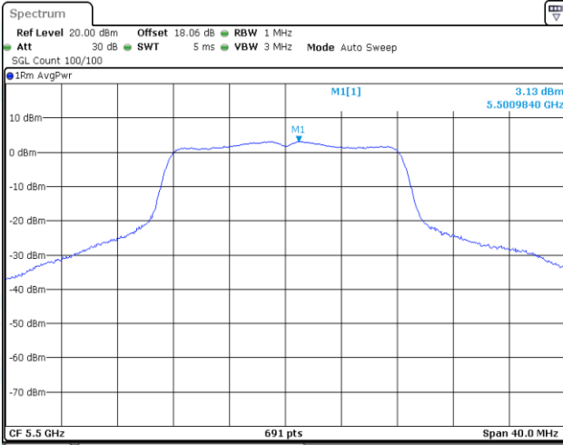
11A-CDD-Ant1-5500-PASS
