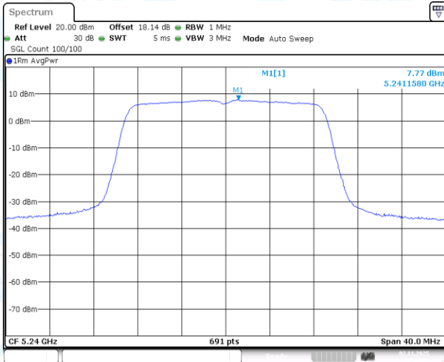
11AC20-CDD-Ant1-5240-PASS
