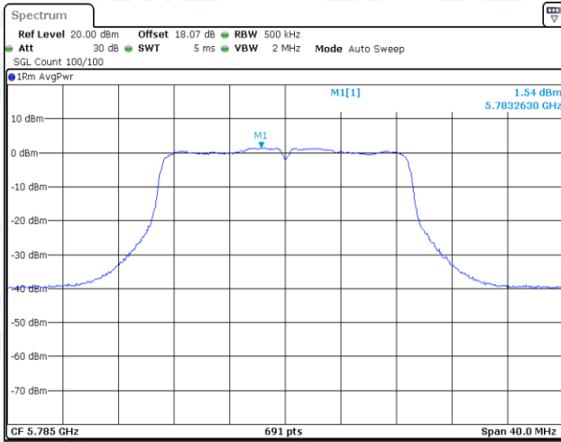
11N20-CDD-Ant3-5785-PASS
