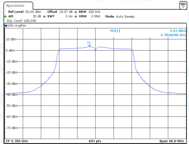
11A-CDD-Ant1-5785-PASS
