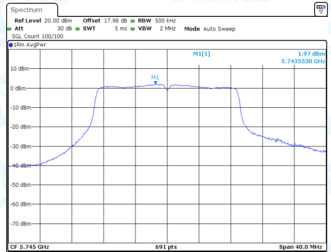
11N20-CDD-Ant1-5745-PASS
