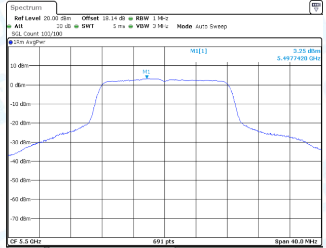
11A-CDD-Ant2-5500-PASS
