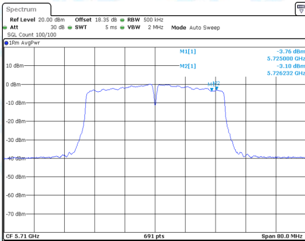
11N40-CDD-Ant3-5710_UNII-2C-PASS
