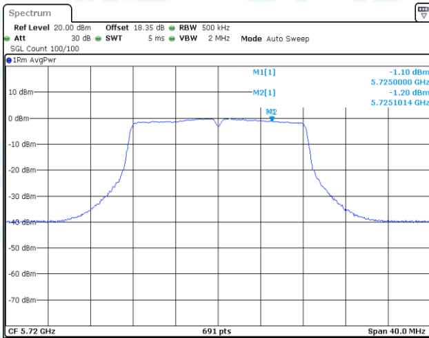
11A-CDD-Ant3-5720_UNII-2C-PASS
