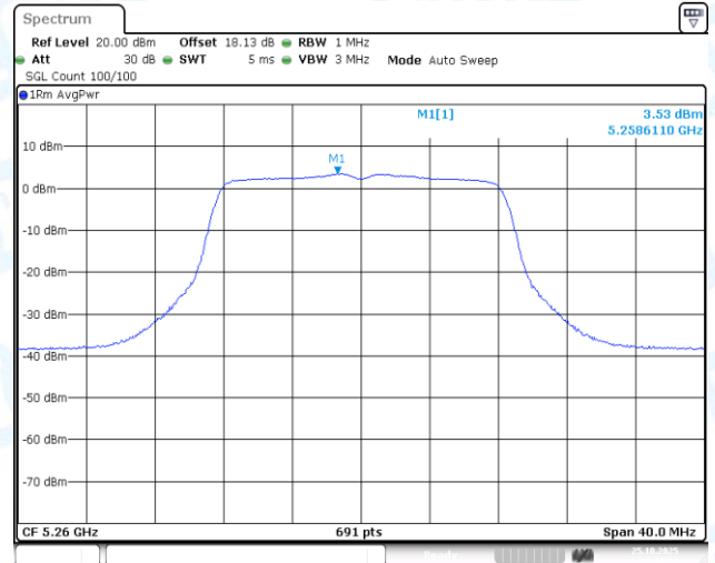
11A-CDD-Ant1-5260-PASS
