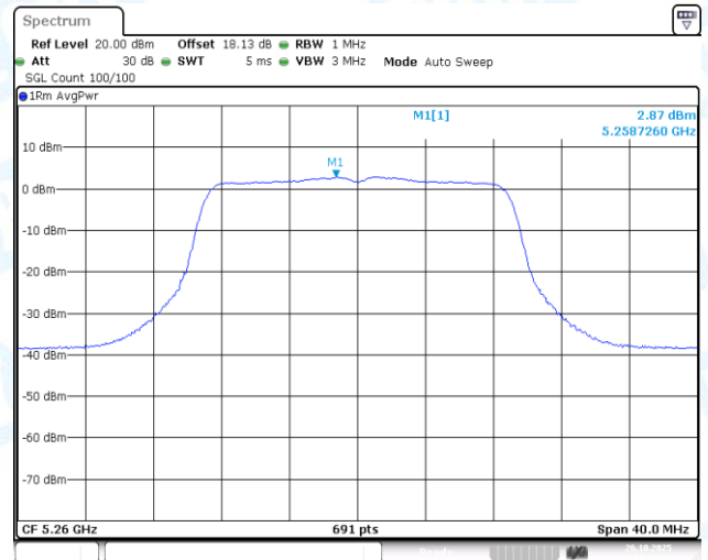
11AC20-CDD-Ant1-5260-PASS
