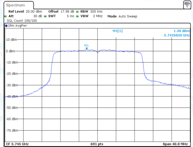
11AX20-CDD-Ant1-5745-PASS
