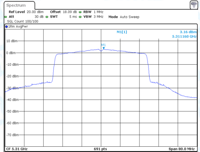
11AX40-CDD-Ant1-5310-PASS
