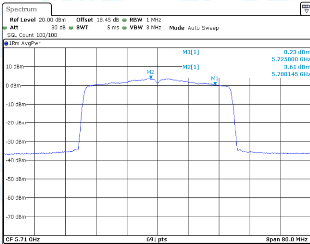
11AX40-CDD-Ant1-5710_UNII-2C-PASS
