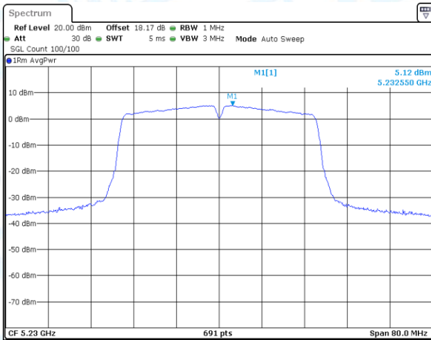
11AC40-CDD-Ant1-5230-PASS
