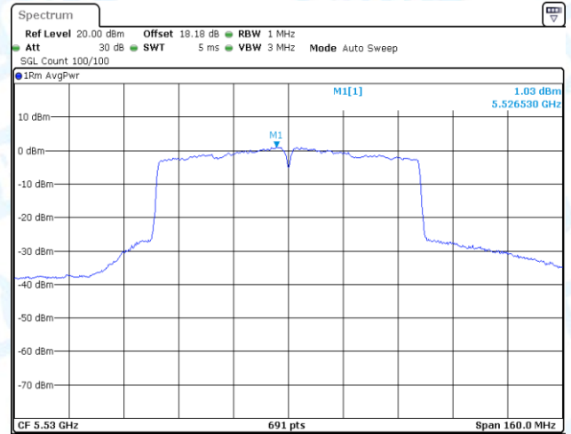
11AC80-CDD-Ant1-5530-PASS
