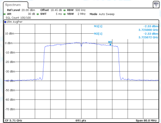
11AX40-CDD-Ant1-5710_UNII-3-PASS
