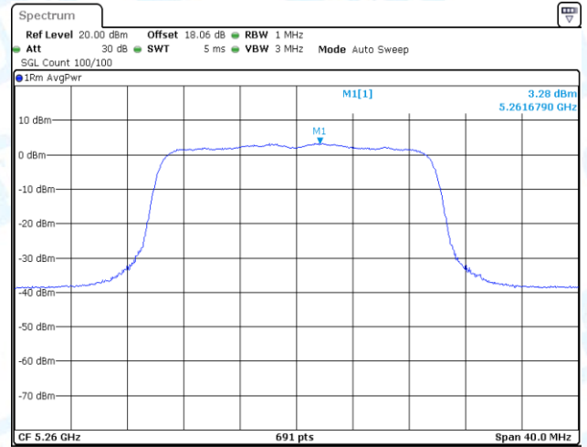
11AX20-CDD-Ant2-5260-PASS
