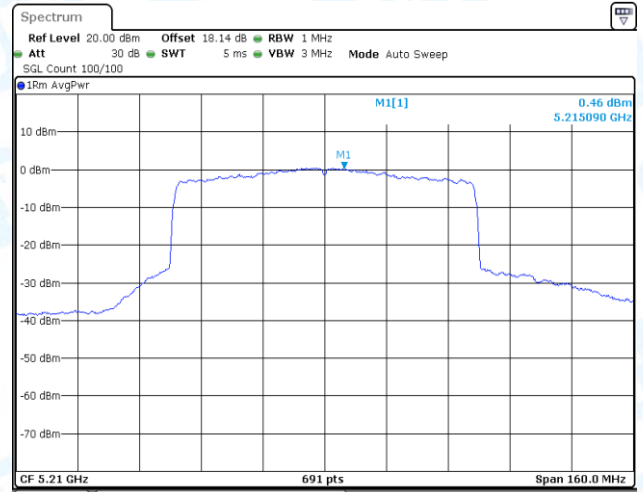
11AX80-CDD-Ant1-5210-PASS
