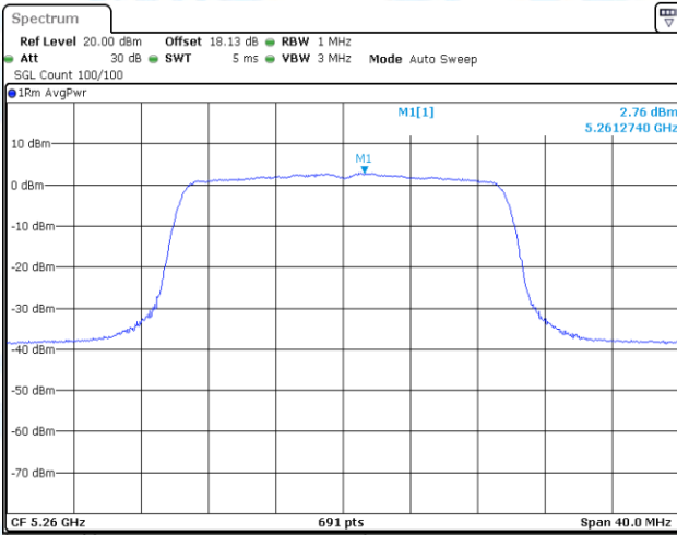
11AX20-CDD-Ant1-5260-PASS
