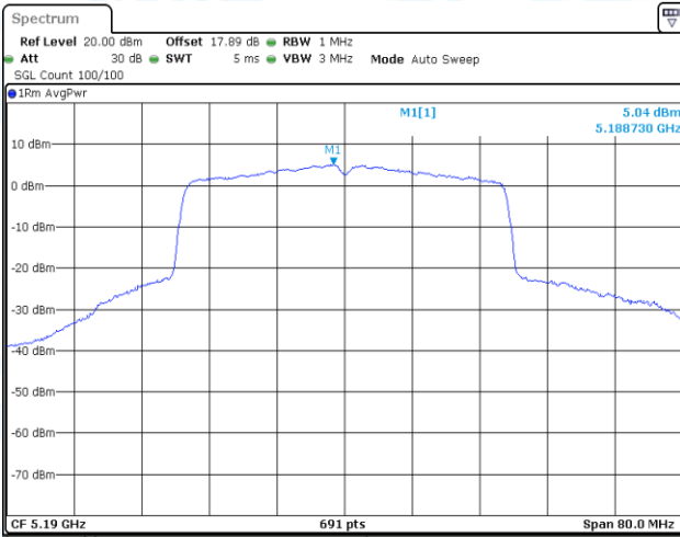
11AX40-CDD-Ant1-5190-PASS
