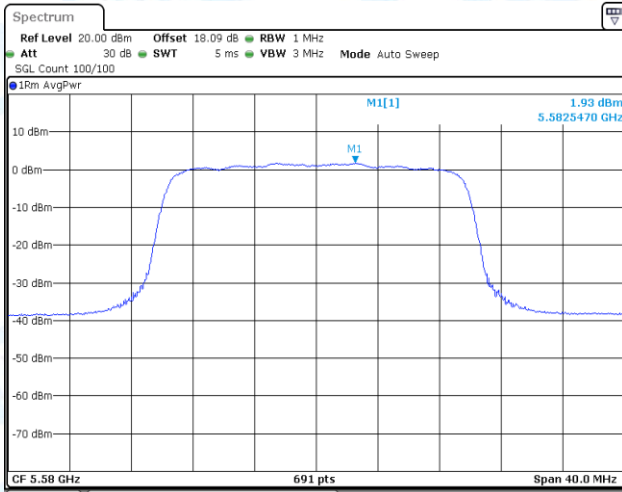
11AX20-CDD-Ant1-5580-PASS
