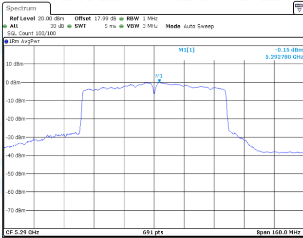
11AC80-CDD-Ant1-5290-PASS
