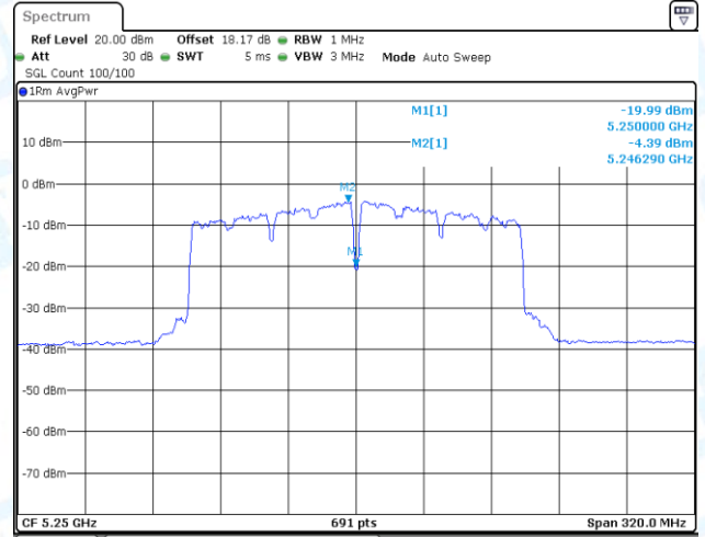
11AC160-CDD-Ant2-5250_UNII-1-PASS
