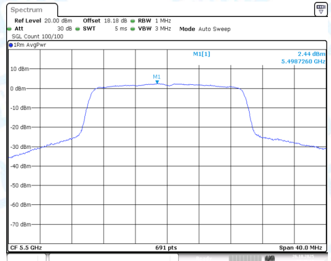
11AX20-CDD-Ant1-5500-PASS
