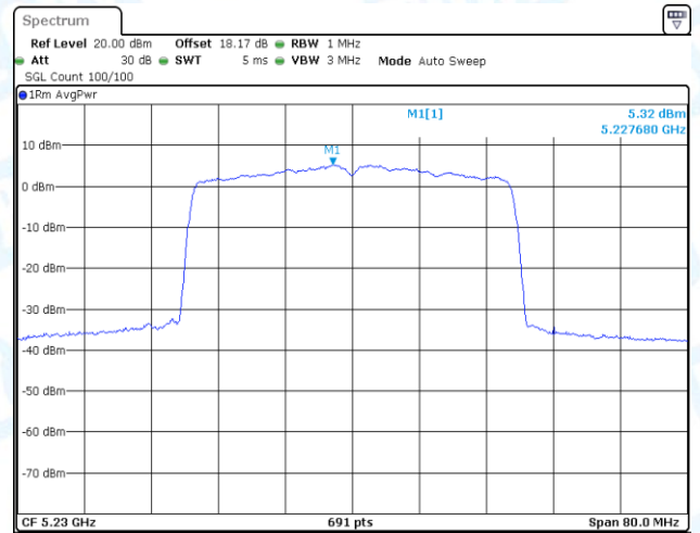
11AX40-CDD-Ant3-5230-PASS
