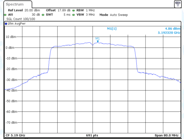
11AX40-CDD-Ant2-5190-PASS
