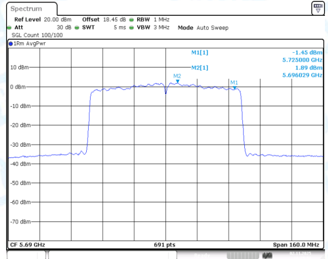
11AC80-CDD-Ant1-5690_UNII-2C-PASS
