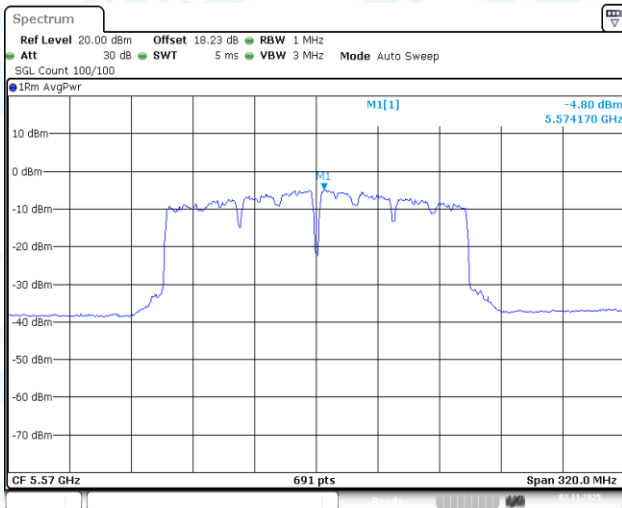
11AC160-CDD-Ant3-5570-PASS
