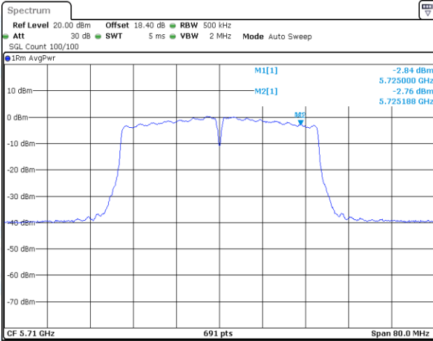
11AC40-CDD-Ant1-5710_UNII-3-PASS
