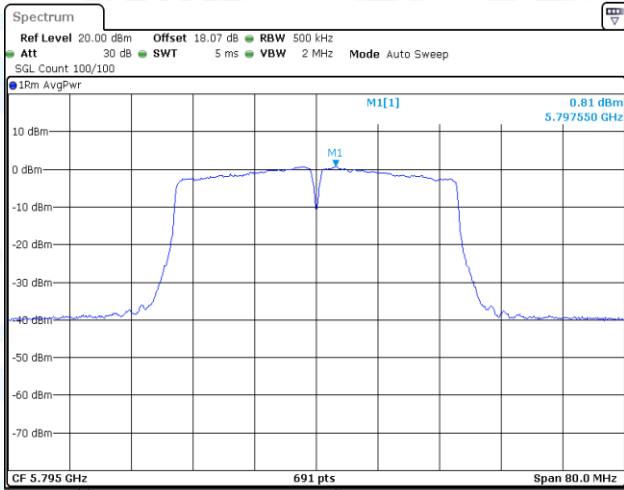
11AC40-CDD-Ant1-5795-PASS
