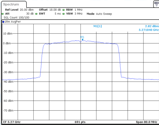
11AX40-CDD-Ant1-5270-PASS
