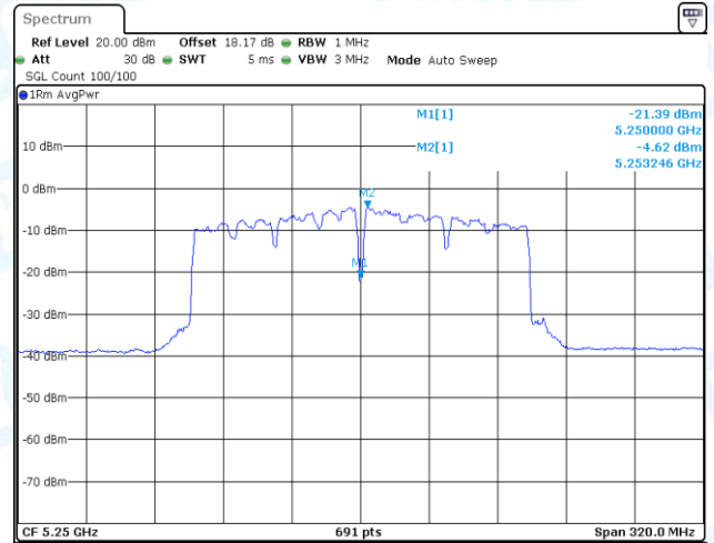
11AC160-CDD-Ant1-5250_UNII-2A-PASS
