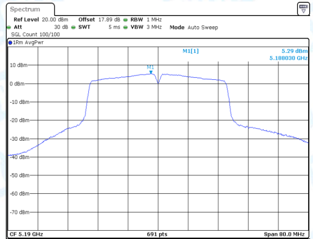
11AC40-CDD-Ant1-5190-PASS
