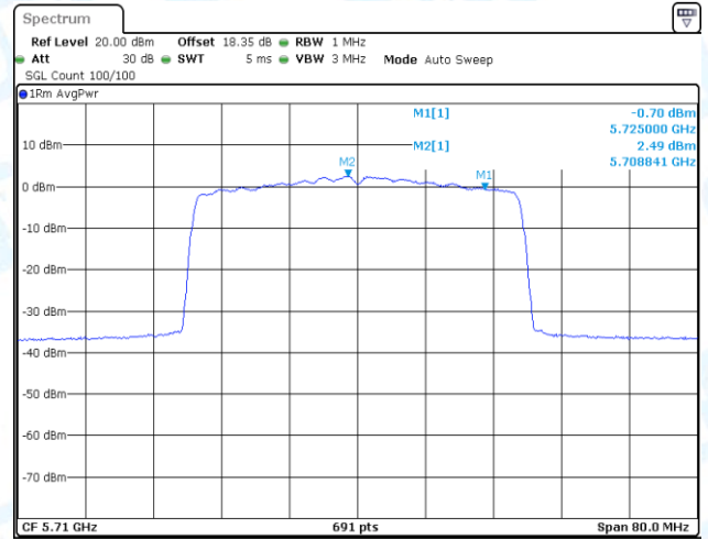
11AX40-CDD-Ant2-5710_UNII-2C-PASS
