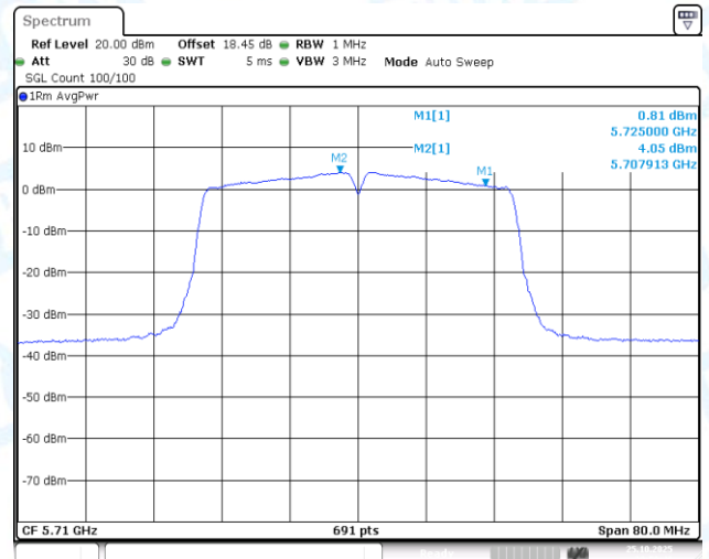
11AC40-CDD-Ant1-5710_UNII-2C-PASS
