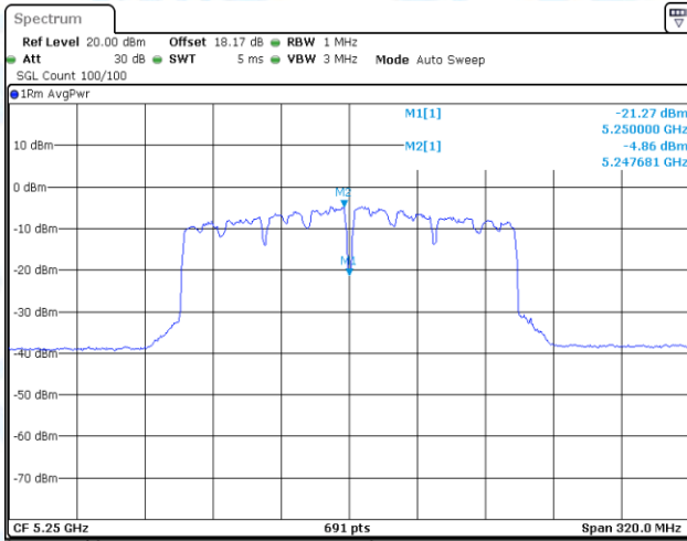
11AC160-CDD-Ant1-5250_UNII-1-PASS
