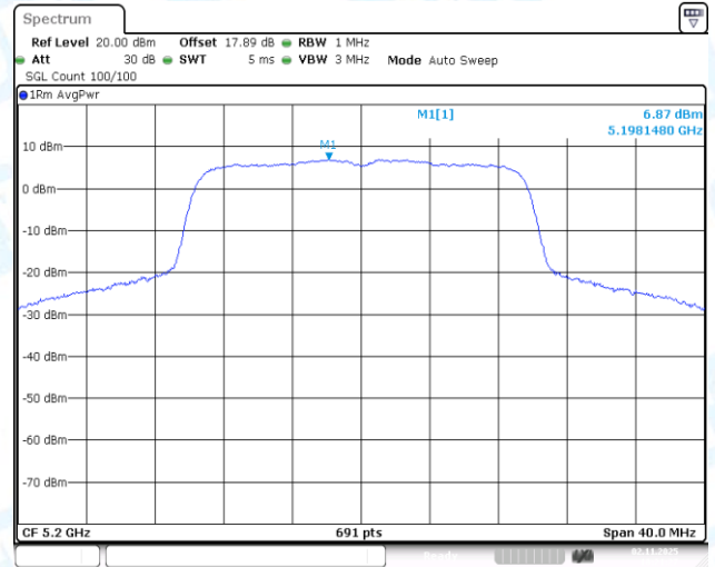
11AX20-CDD-Ant2-5200-PASS
