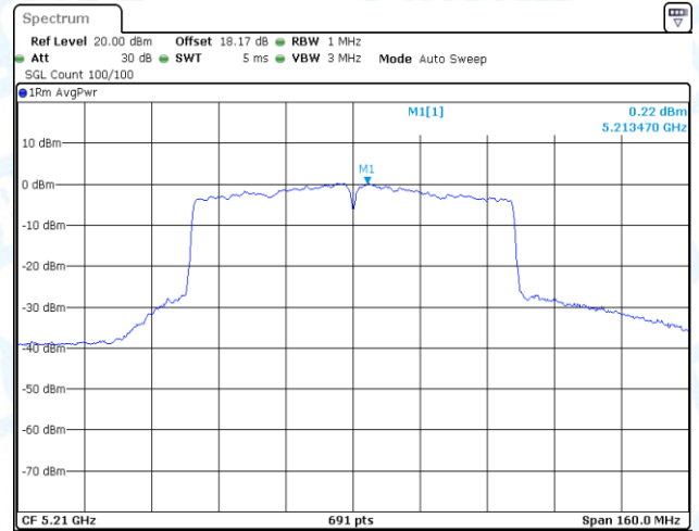
11AC80-CDD-Ant1-5210-PASS
