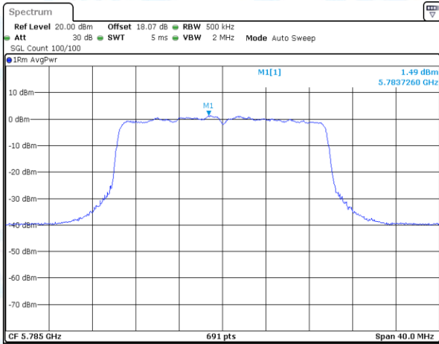
11AX20-CDD-Ant1-5785-PASS
