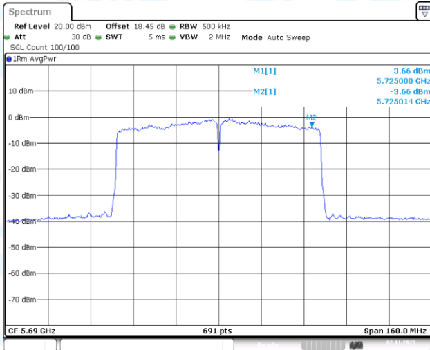
11AC80-CDD-Ant1-5690_UNII-3-PASS
