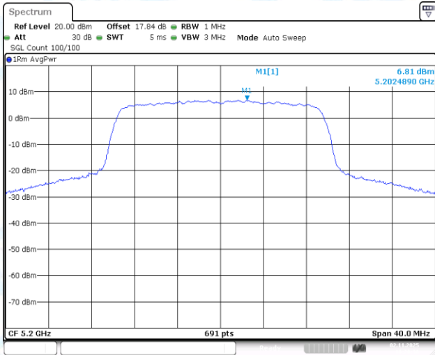
11AX20-CDD-Ant1-5200-PASS
