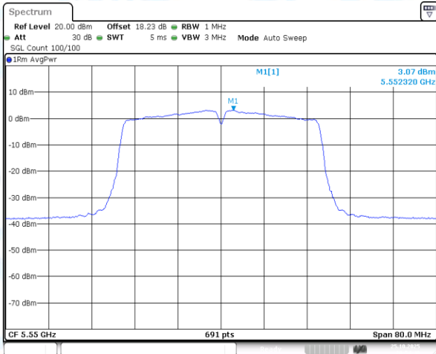
11AC40-CDD-Ant1-5550-PASS
