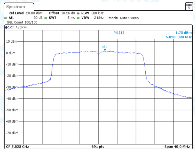
11AX20-CDD-Ant1-5825-PASS
