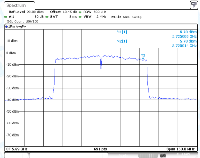
11AC80-CDD-Ant2-5690_UNII-3-PASS
