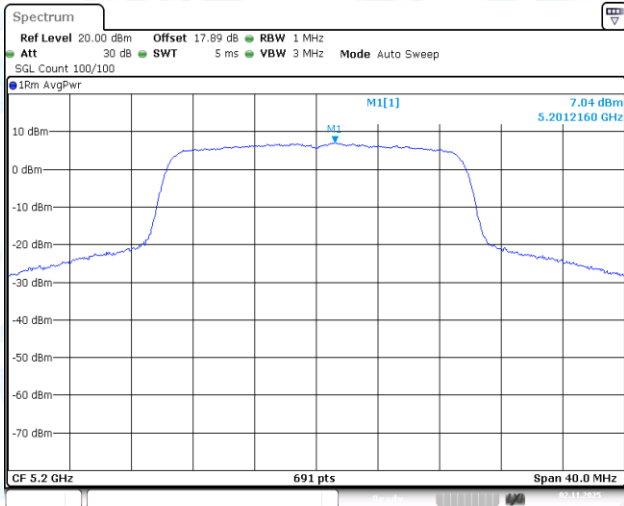
11AX20-CDD-Ant1-5200-PASS
