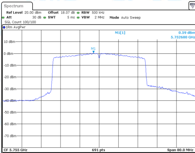
11AX40-CDD-Ant1-5755-PASS
