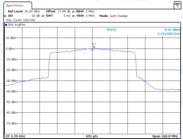
11AX80-CDD-Ant1-5290-PASS
