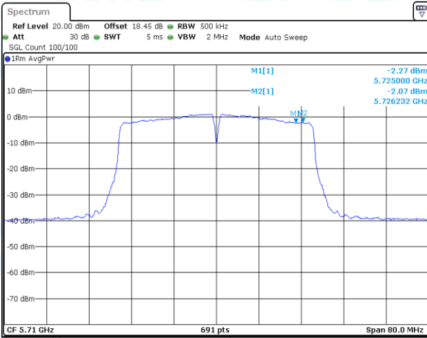
11AC40-CDD-Ant1-5710_UNII-3-PASS
