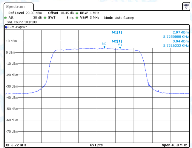
11AX20-CDD-Ant1-5720_UNII-2C-PASS
