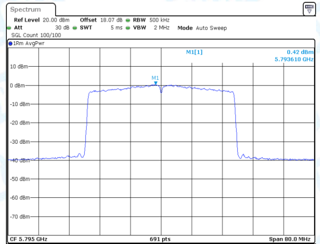
11AX40-CDD-Ant1-5795-PASS
