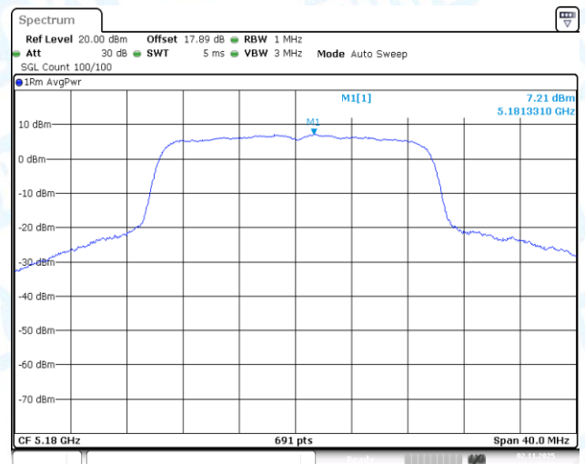
11AX20-CDD-Ant1-5180-PASS
