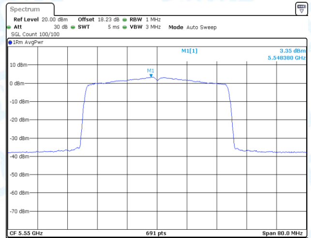
11AX40-CDD-Ant1-5550-PASS
