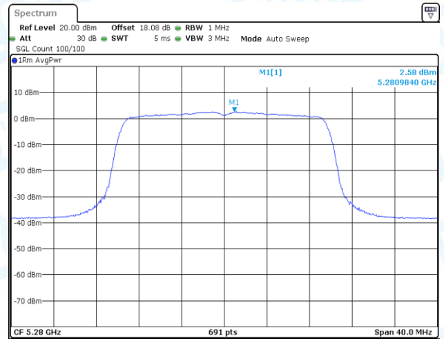
11AX20-CDD-Ant1-5280-PASS
