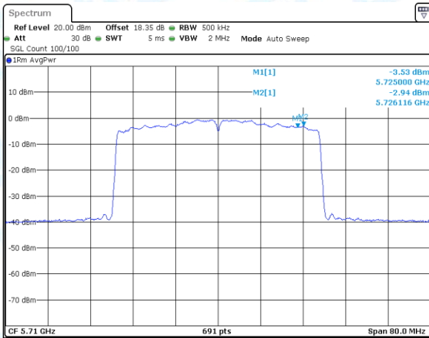
11AX40-CDD-Ant3-5710_UNII-2C-PASS
