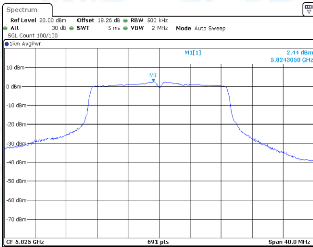
11AC20-CDD-Ant1-5825-PASS
