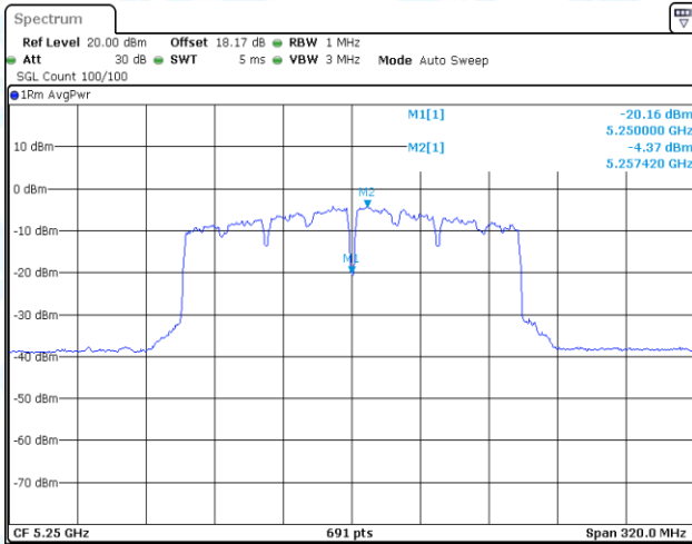
11AC160-CDD-Ant3-5250_UNII-1-PASS
