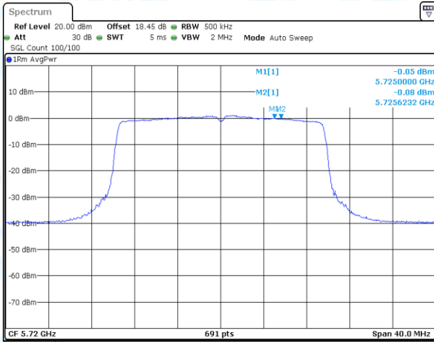
11AX20-CDD-Ant1-5720_UNII-3-PASS
