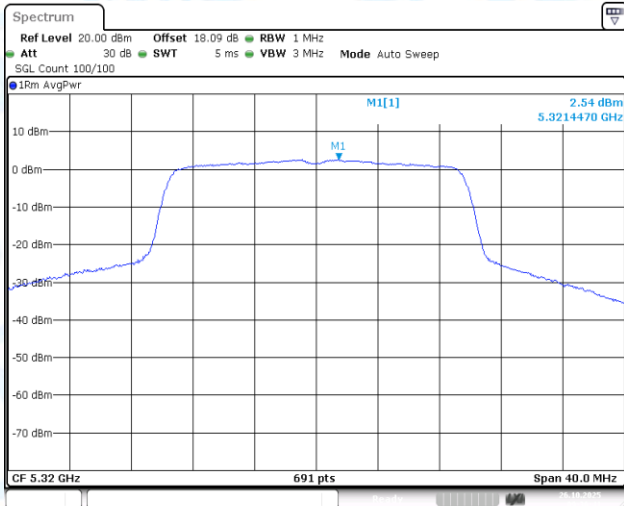
11AX20-CDD-Ant1-5320-PASS
