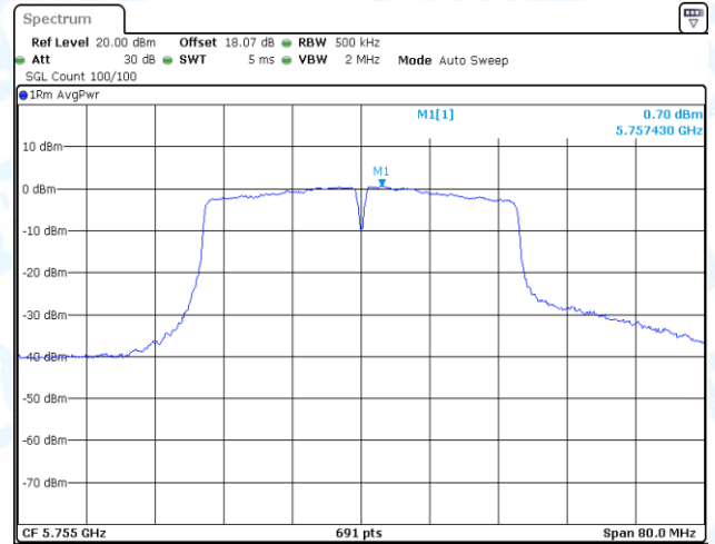
11AC40-CDD-Ant1-5755-PASS
