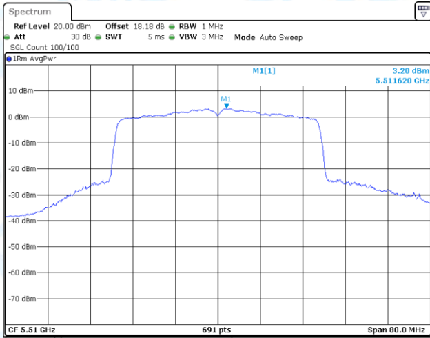
11AX40-CDD-Ant1-5510-PASS
