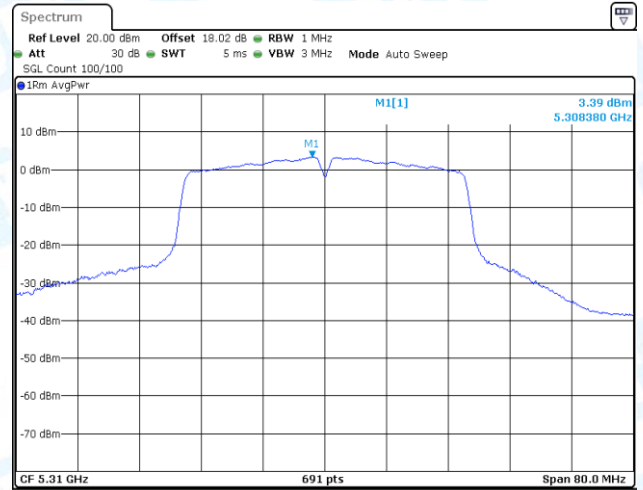
11AC40-CDD-Ant2-5310-PASS
