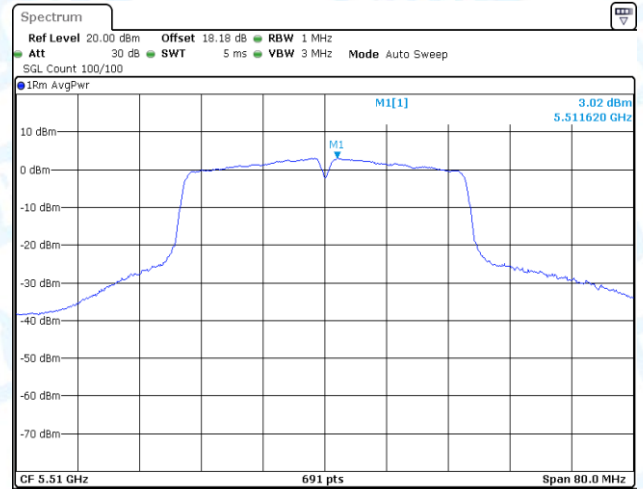
11AC40-CDD-Ant1-5510-PASS
