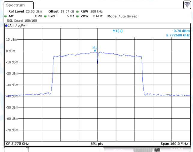
11AC80-CDD-Ant1-5775-PASS
