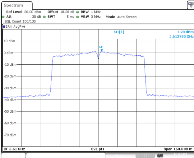
11AC80-CDD-Ant1-5610-PASS
