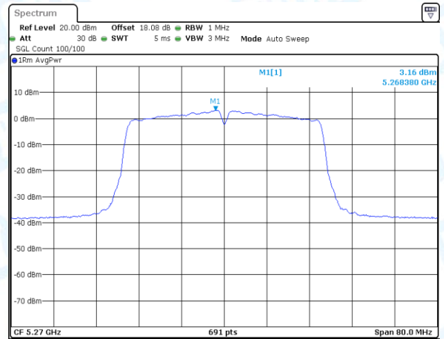
11AC40-CDD-Ant1-5270-PASS
