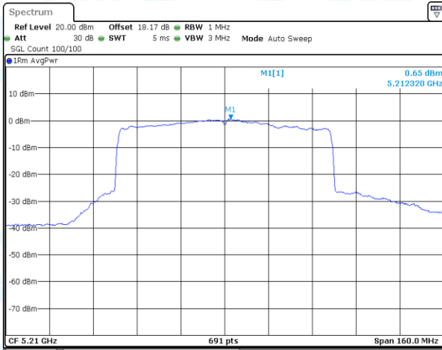
11AX80-CDD-Ant3-5210-PASS
