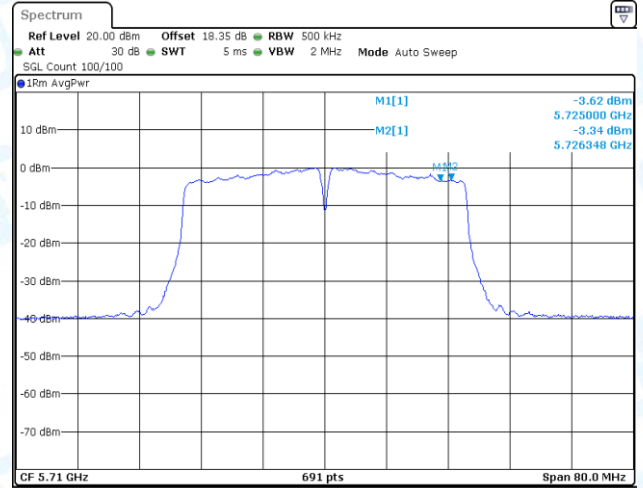
11AC40-CDD-Ant2-5710_UNII-3-PASS
