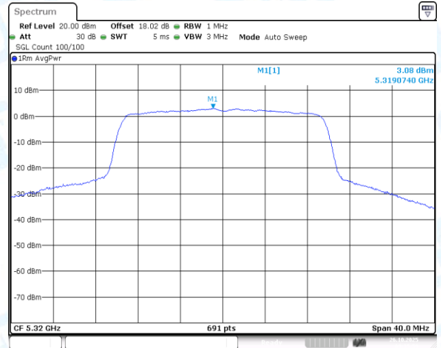
11AX20-CDD-Ant2-5320-PASS
