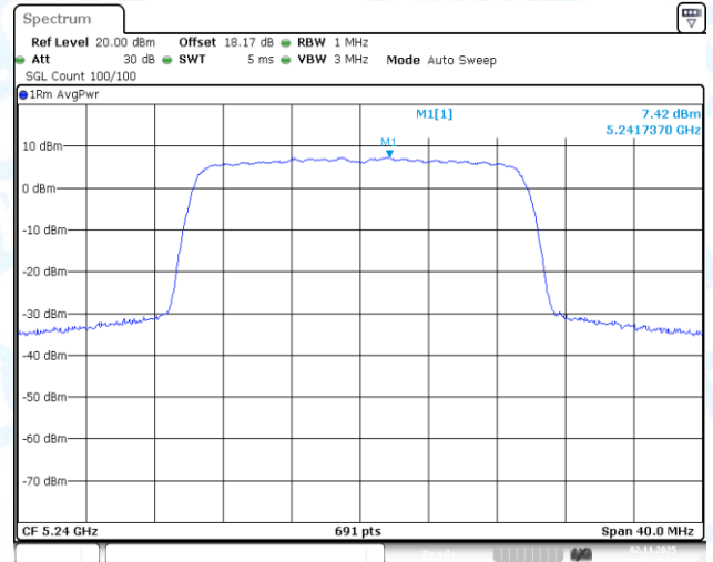
11AX20-CDD-Ant1-5240-PASS
