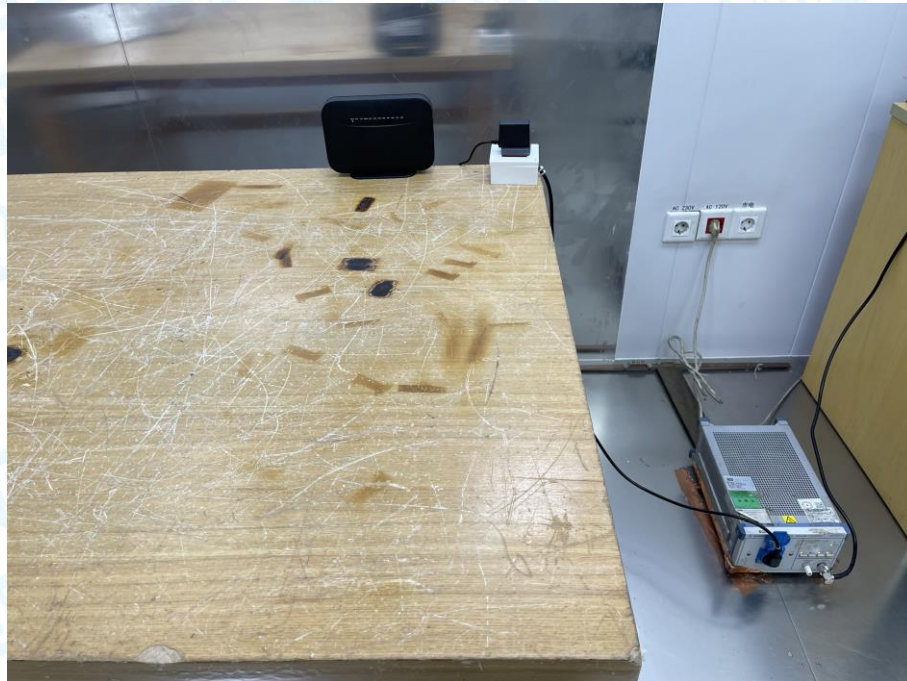
Photo of Setup for RF Conducted Measurements
