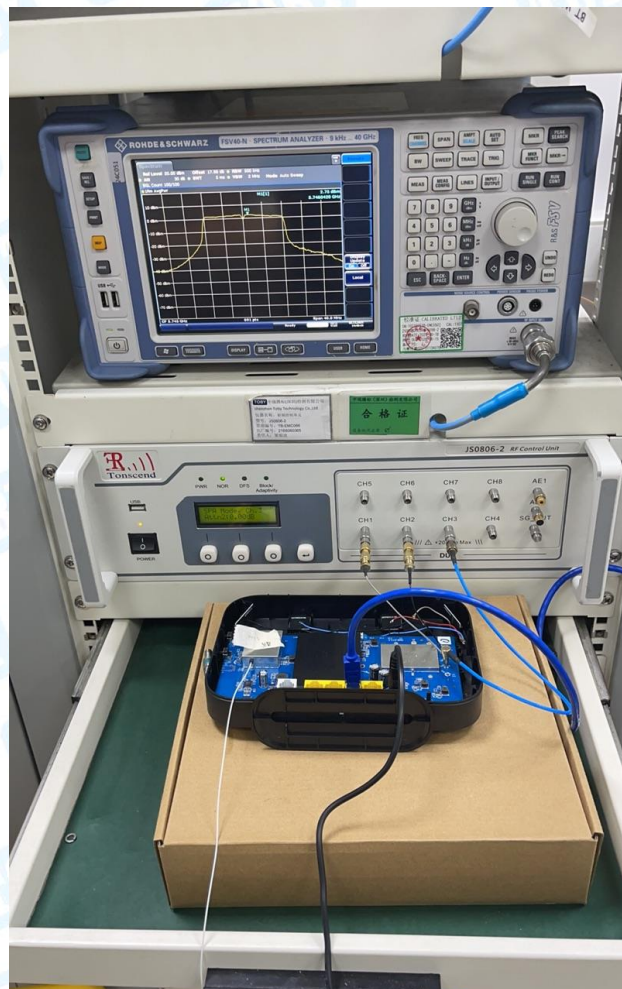
Photo of Setup for RF Conducted Measurements
