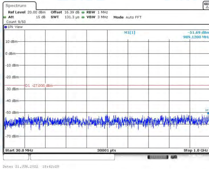
11A_Ant2_5300_30~1000
