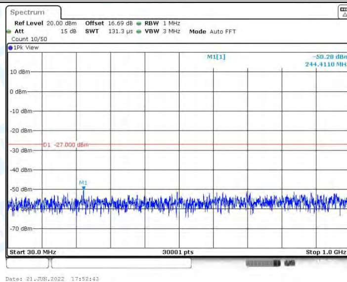
11A_Ant1_5700_30~1000
