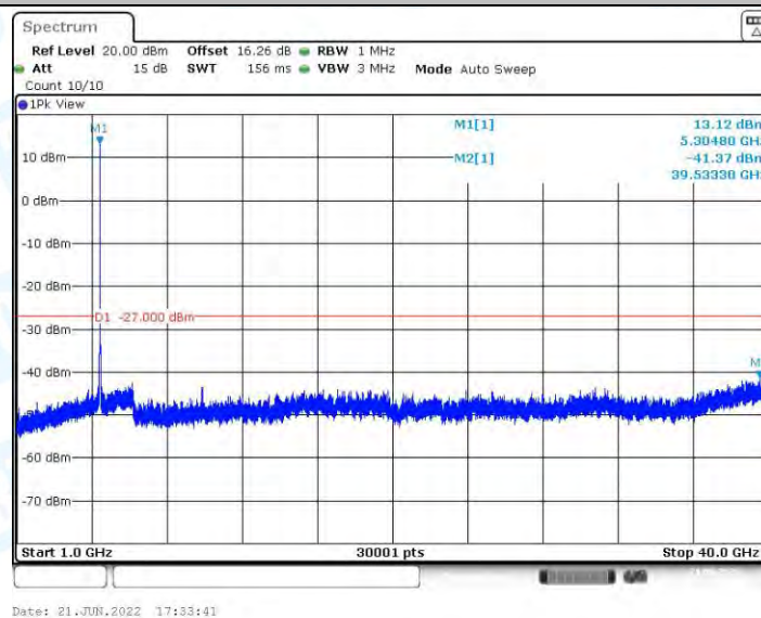
11A_Ant1_5300_1000~40000
