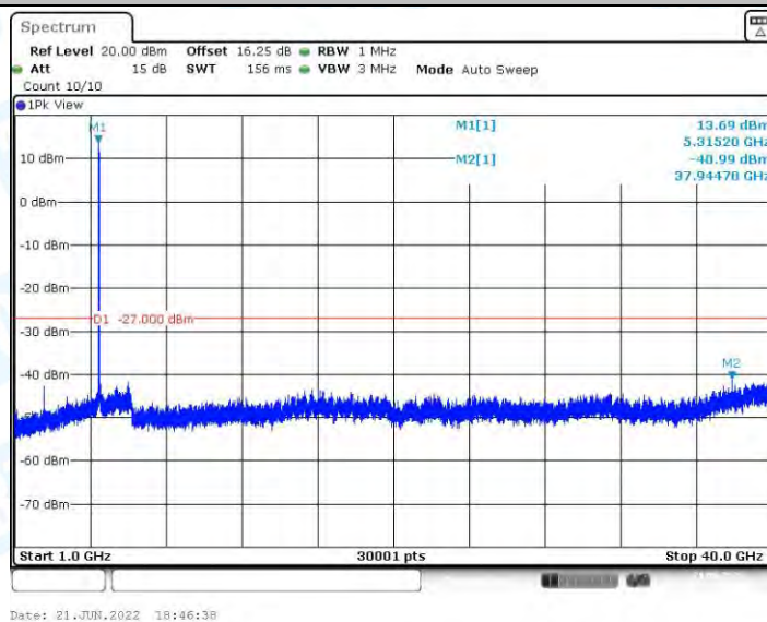
11A_Ant2_5320_1000~40000
