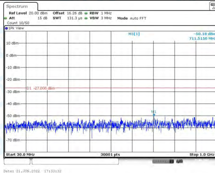
11A_Ant1_5300_30~1000
