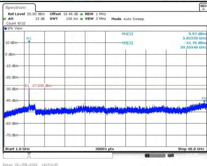
11AC20MIMO_Ant1_5825_1000~40000
