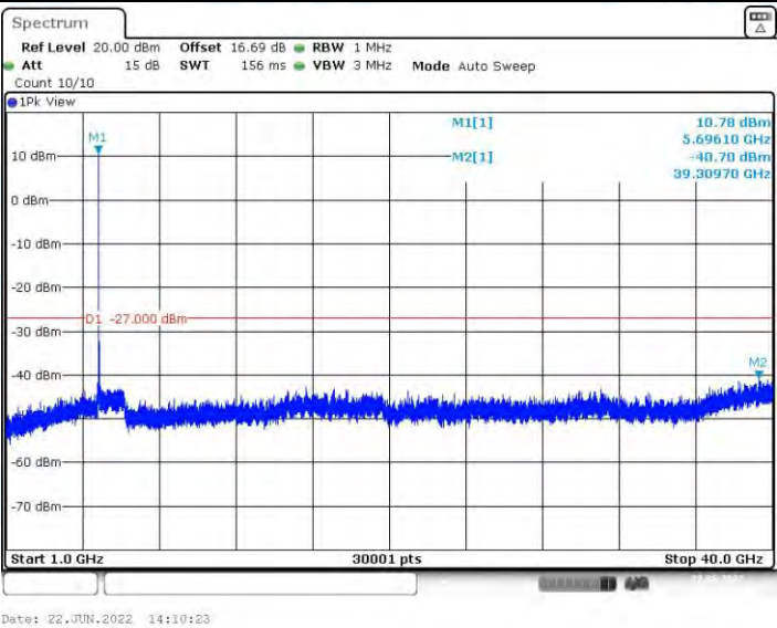
11AC20MIMO_Ant1_5700_1000~40000
