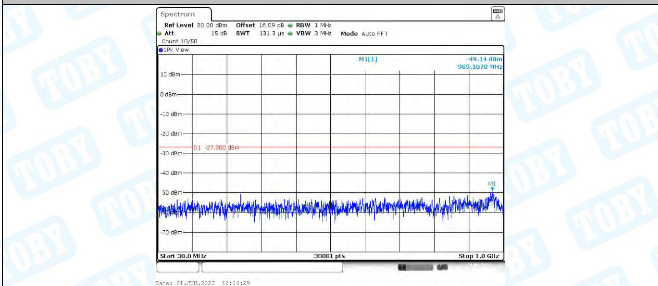
11A_Ant2_5180_30~1000
