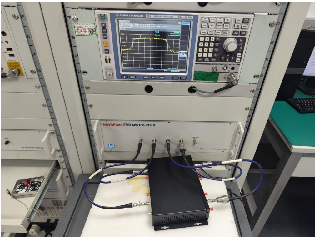
Conducted Measurement Photo at Antenna Port
