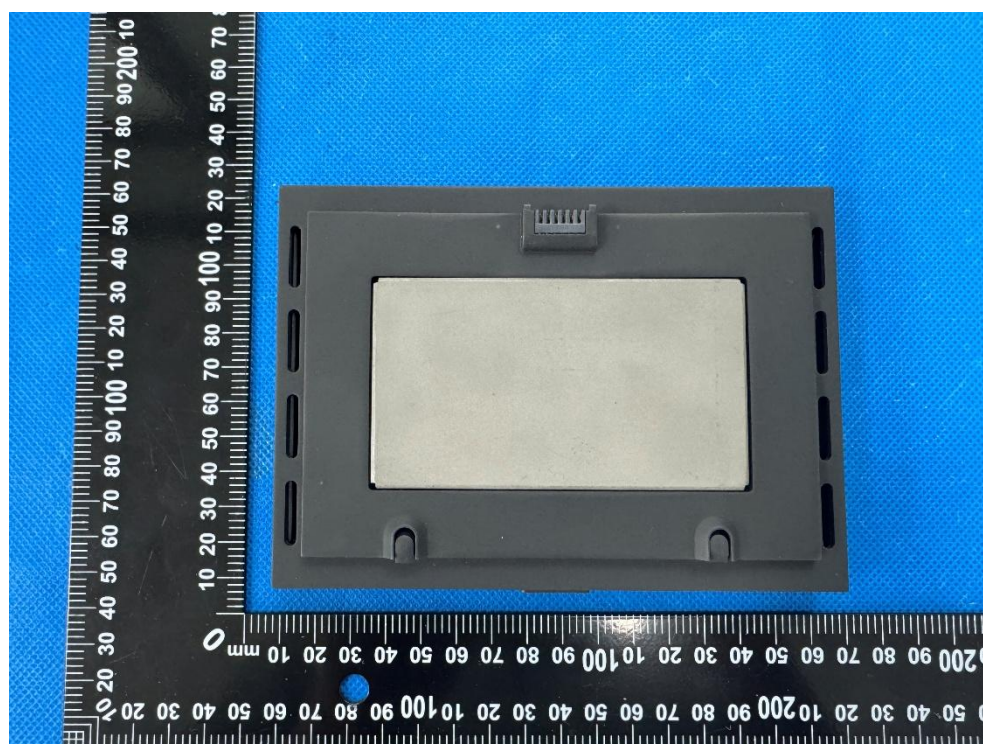
Photo 14 (battery base)
