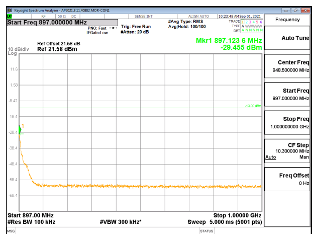
Plot 2: 16QAM – 895.24MHz
