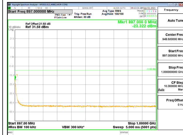
Plot 1: 64QAM – 895.24MHz
