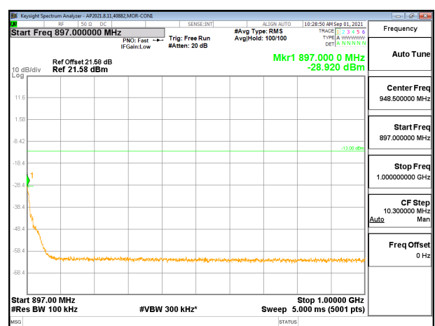
Plot 2: QPSK – 895.27MHz
