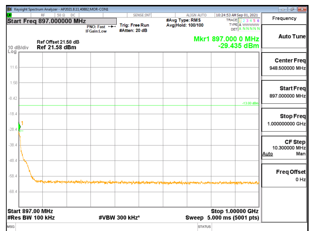
Plot 2: 64QAM – 895.24MHz
