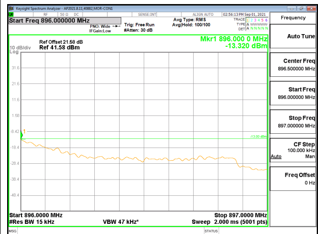
Plot 2: 64QAM – 895.27MHz
