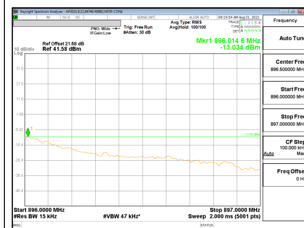
Plot 1: 64QAM – 895.27MHz
