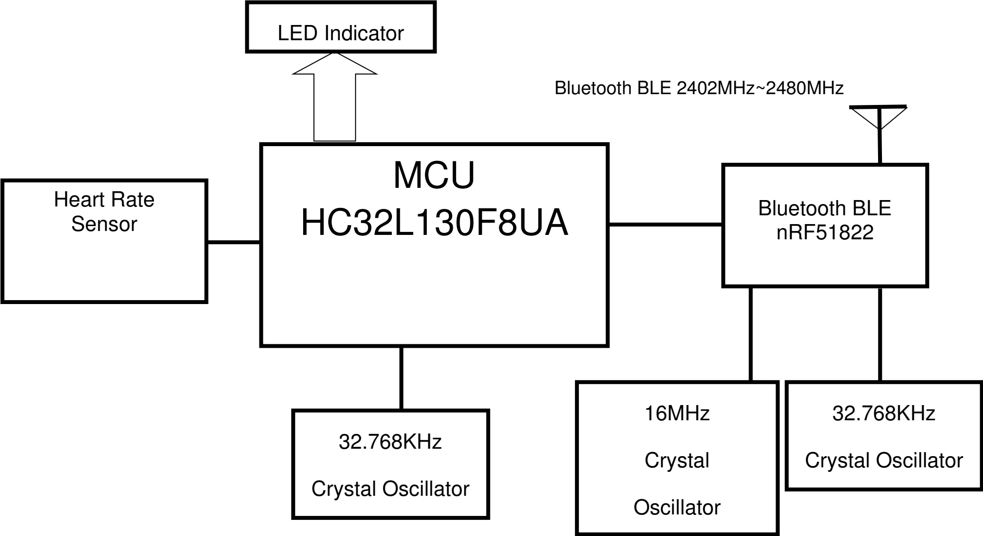
Baby Tracker (Sensor) Block Diagram
