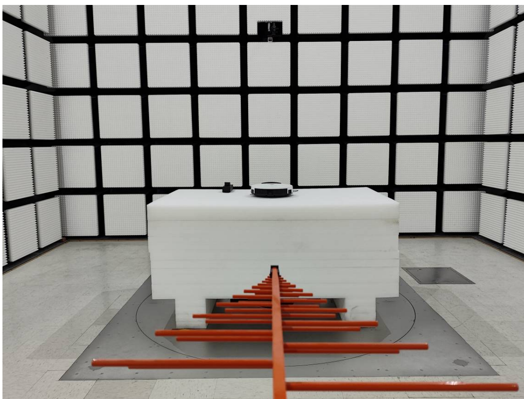
Radiated Emission Below 1GHz View Adapter 2 + Charging Dock
